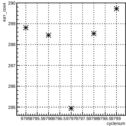
4aY_coil4:cyclenum {run == 7913}
