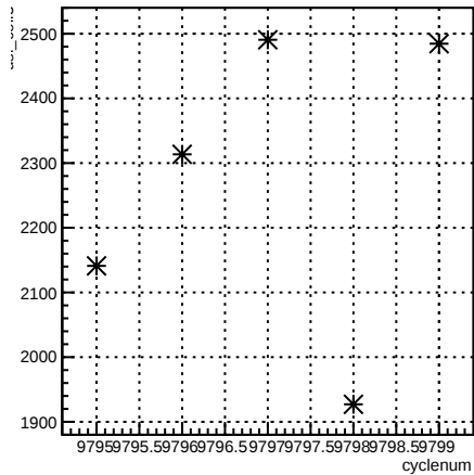
usl_coil7:cyclenum {run == 7913}
