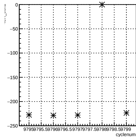
4eX_coil1:cyclenum {run == 7913}
