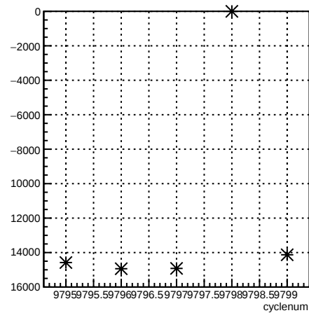
usr_coil1:cyclenum {run == 7913}
