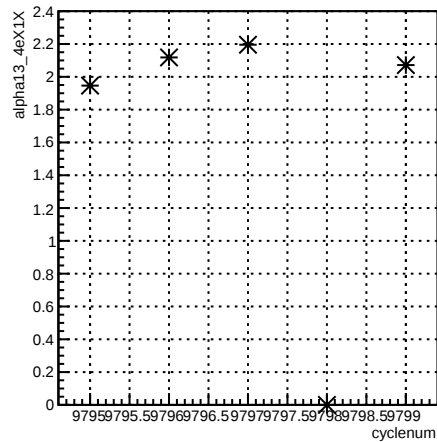
alpha13_4eX1X:cyclenum {run == 7913}
