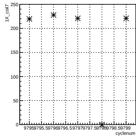
1X_coil7:cyclenum {run == 7913}
