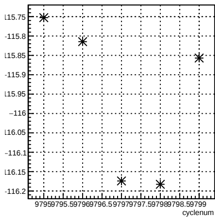
4aY_coil6:cyclenum {run == 7913}
