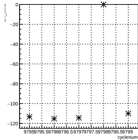
1X_coil1:cyclenum {run == 7913}
