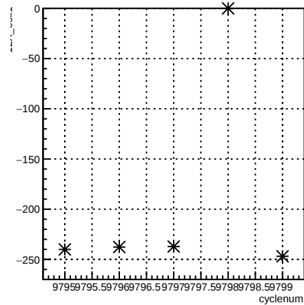
12X_coil1:cyclenum {run == 7913}
