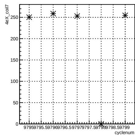
4eX_coil7:cyclenum {run == 7913}
