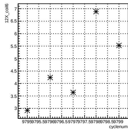
12X_coil6:cyclenum {run == 7913}
