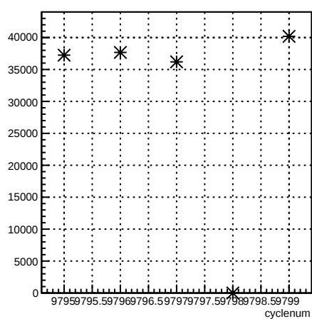
usr_coil7:cyclenum {run == 7913}
