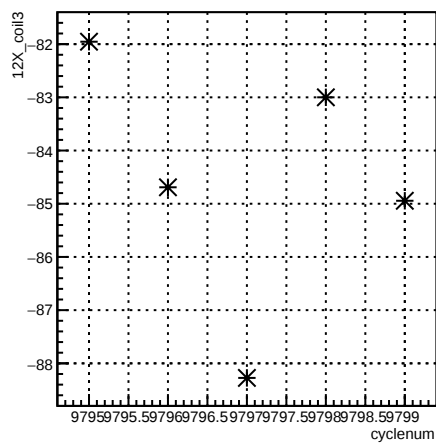
12X_coil3:cyclenum {run == 7913}
