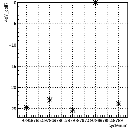
4eY_coil7:cyclenum {run == 7913}
