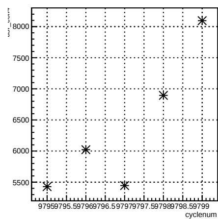
usr_coil4:cyclenum {run == 7913}
