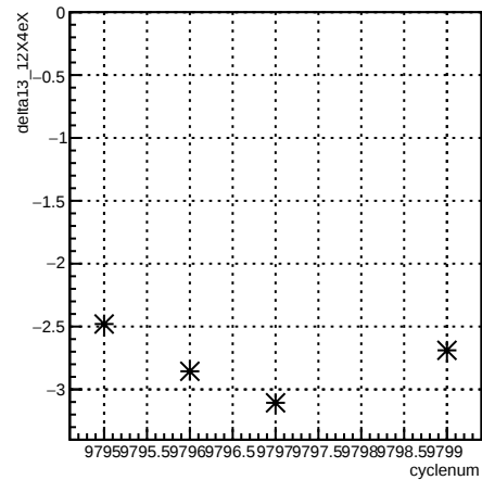
delta13_12X4eX:cyclenum {run == 7913}
