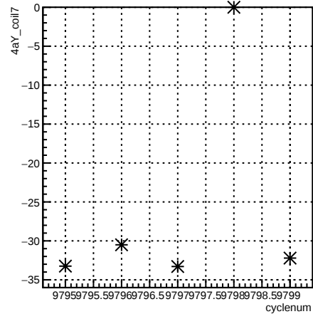
4aY_coil7:cyclenum {run == 7913}
