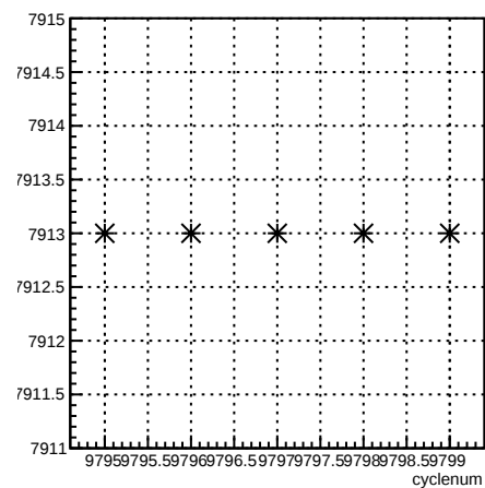
run:cyclenum {run == 7913}
