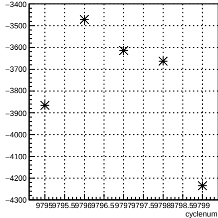
usl_coil6:cyclenum {run == 7913}
