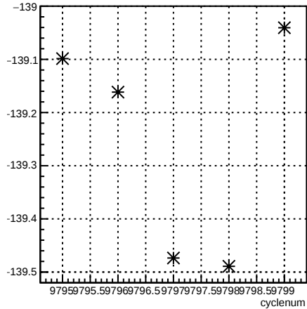
4eY_coil6:cyclenum {run == 7913}
