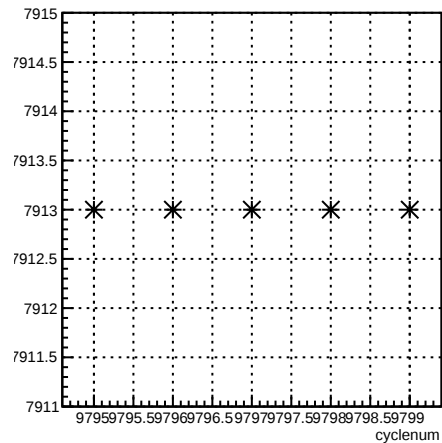
run:cyclenum {run == 7913}
