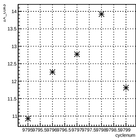
1X_coil3:cyclenum {run == 7913}
