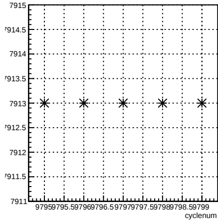
run:cyclenum {run == 7913}
