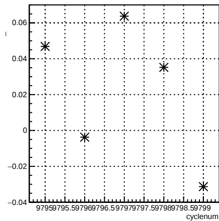
delta46_12X4eY:cyclenum {run == 7913}
