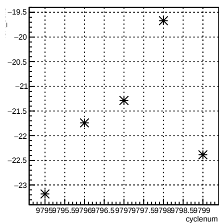
4eX_coil3:cyclenum {run == 7913}
