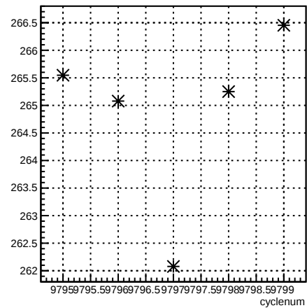
4eY_coil4:cyclenum {run == 7913}
