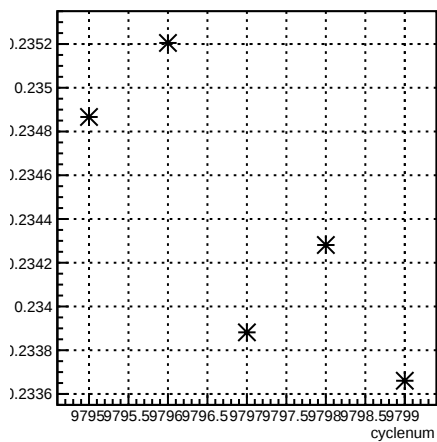
alpha46_4eY4aY:cyclenum {run == 7913}
