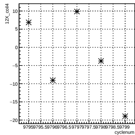
12X_coil4:cyclenum {run == 7913}
