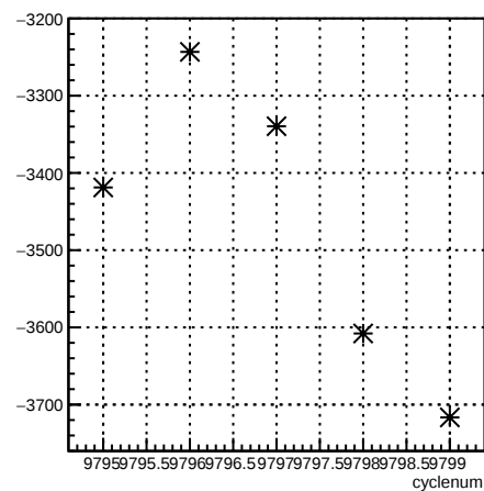
usr_coil6:cyclenum {run == 7913}
