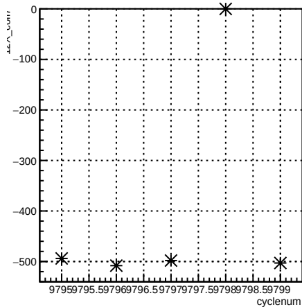
12X_coil7:cyclenum {run == 7913}
