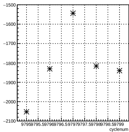
usr_coil3:cyclenum {run == 7913}
