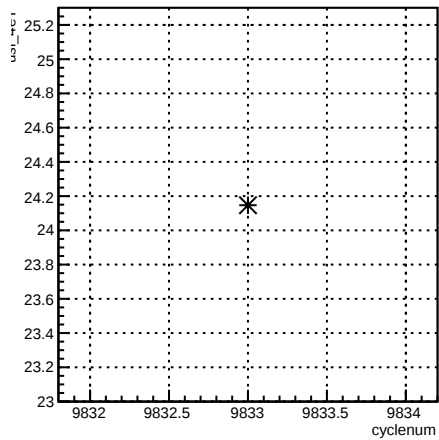
usl_4eY:cyclenum {run == 7921}
