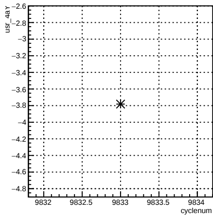
usr_4aY:cyclenum {run == 7921}
