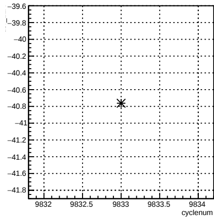
usr_12X:cyclenum {run == 7921}
