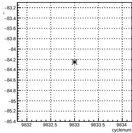
12X_coil7:cyclenum {run == 7921}
