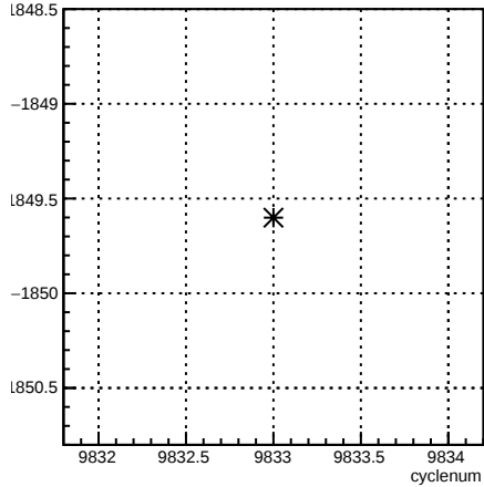
usr_coil7:cyclenum {run == 7921}
