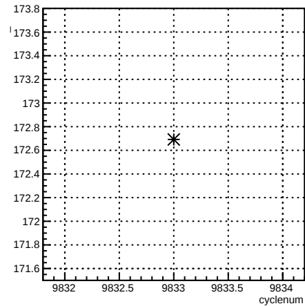
usr_4eX:cyclenum {run == 7921}
