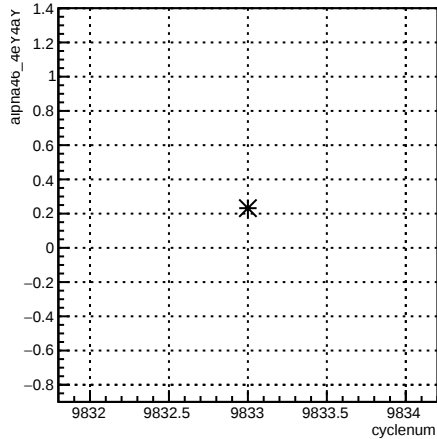
alpha46_4eY4aY:cyclenum {run == 7921}
