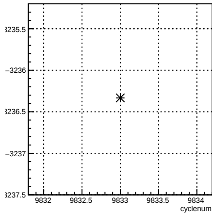
usl_coil6:cyclenum {run == 7921}
