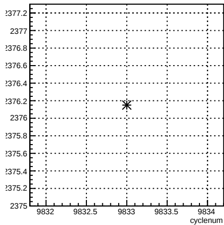
usl_coil7:cyclenum {run == 7921}
