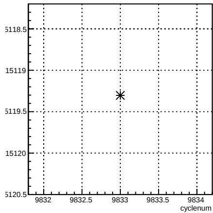
usr_coil6:cyclenum {run == 7921}
