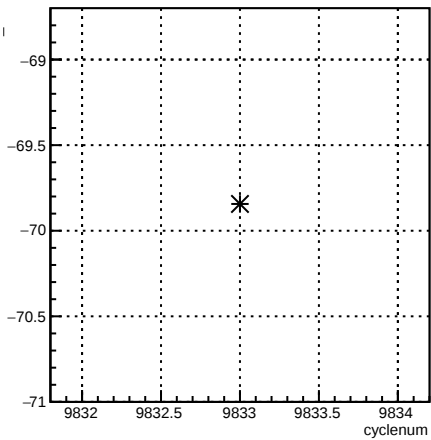
usl_4eY:cyclenum {run == 7921}
