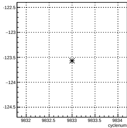
4eX_coil1:cyclenum {run == 7921}
