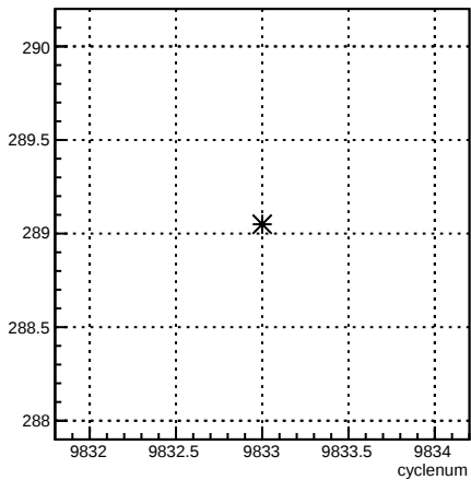
4eY_coil4:cyclenum {run == 7921}
