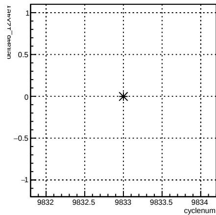
delta46_12X4eY:cyclenum {run == 7921}
