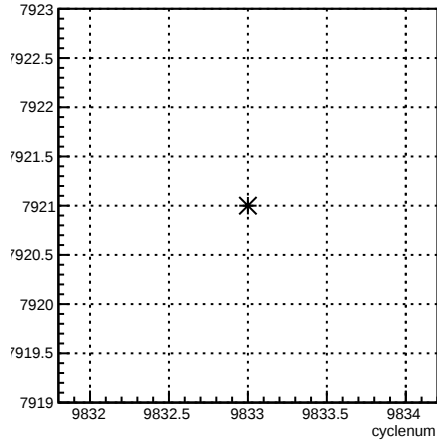
run:cyclenum {run == 7921}
