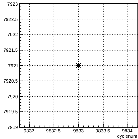
run:cyclenum {run == 7921}
