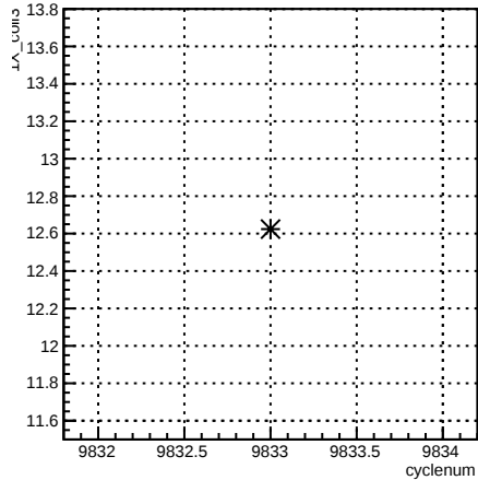
4eX_coil3:cyclenum {run == 7921}
