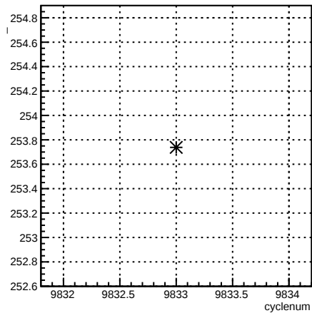
4eX_coil7:cyclenum {run == 7921}
