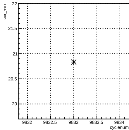
usr_4eY:cyclenum {run == 7921}
