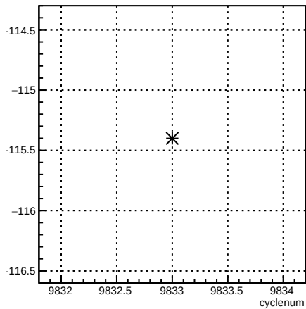
4eY_coil6:cyclenum {run == 7921}
