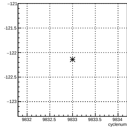
usr_1X:cyclenum {run == 7921}
