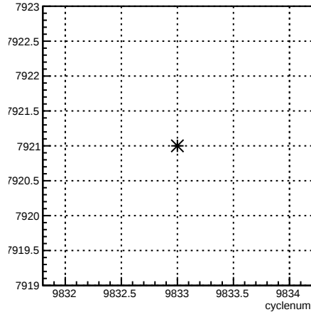
run:cyclenum {run == 7921}
