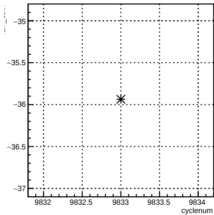
4eY_coil7:cyclenum {run == 7921}
