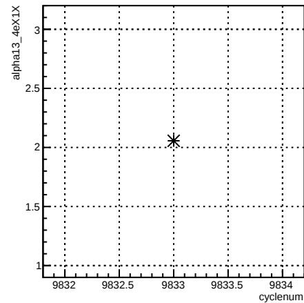
alpha13_4eX1X:cyclenum {run == 7921}
