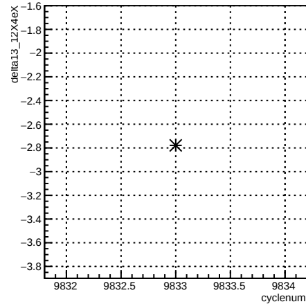
delta13_12X4eX:cyclenum {run == 7921}
