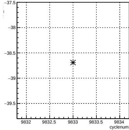
usl_12X:cyclenum {run == 7921}
