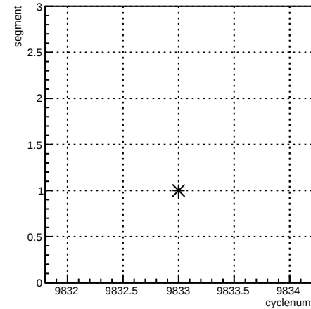
segment:cyclenum {run == 7921}
