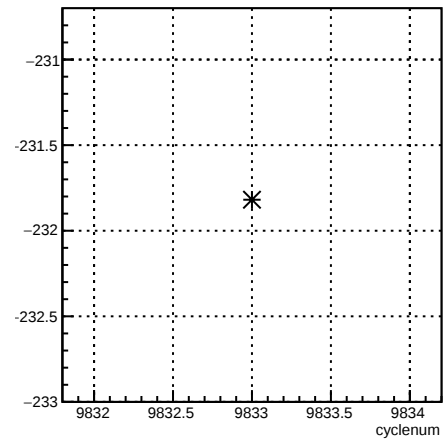
12X_coil6:cyclenum {run == 7921}
