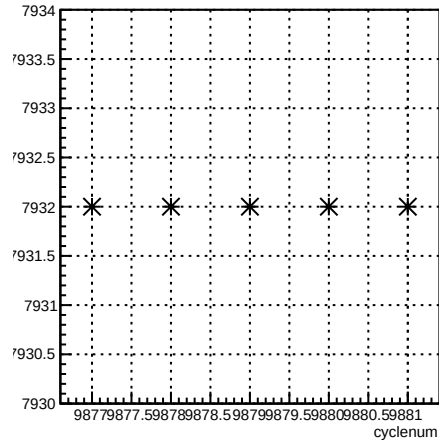
run:cyclenum {run == 7932}
