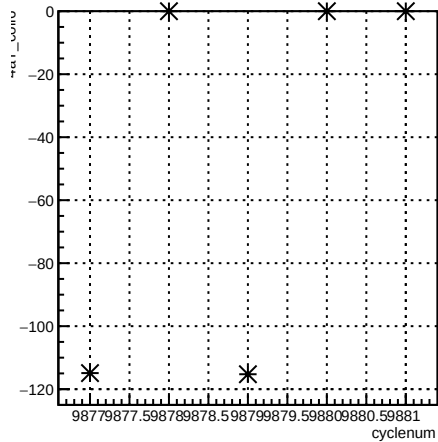
4aY_coil6:cyclenum {run == 7932}
