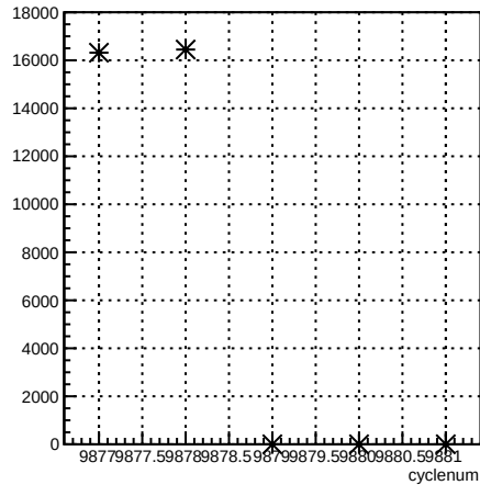
usl_coil1:cyclenum {run == 7932}
