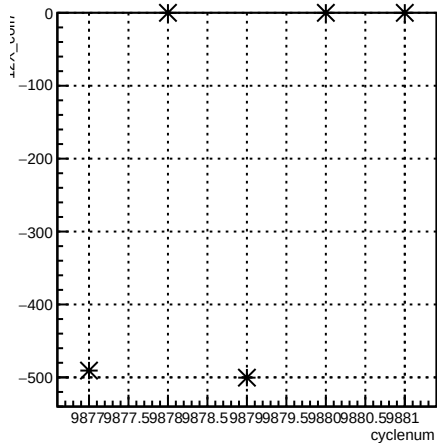
12X_coil7:cyclenum {run == 7932}
