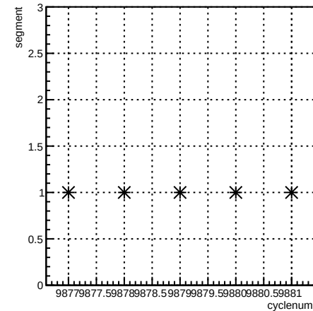
segment:cyclenum {run == 7932}
