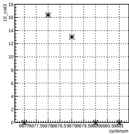
1X_coil3:cyclenum {run == 7932}
