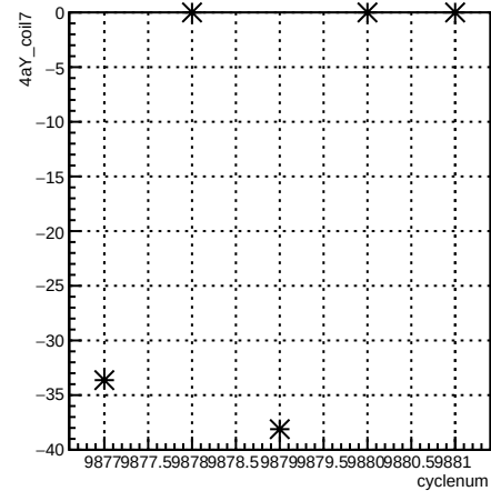
4aY_coil7:cyclenum {run == 7932}
