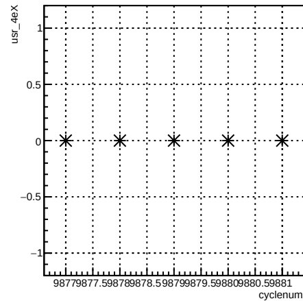
run:cyclenum {run == 7932}
