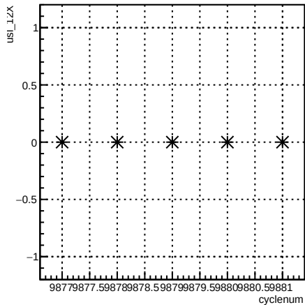
usl_12X:cyclenum {run == 7932}
