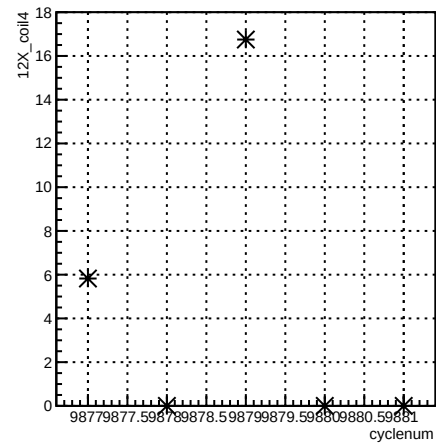
12X_coil4:cyclenum {run == 7932}
