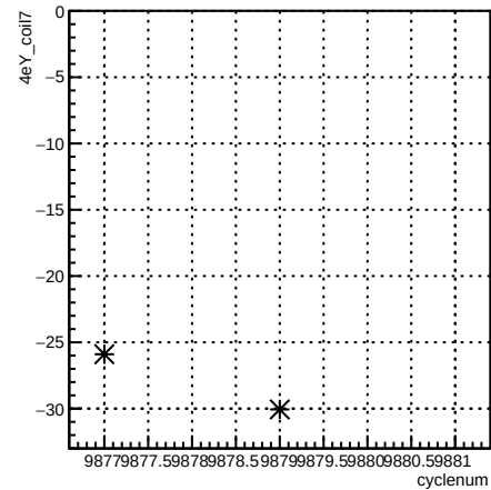
4eY_coil7:cyclenum {run == 7932}
