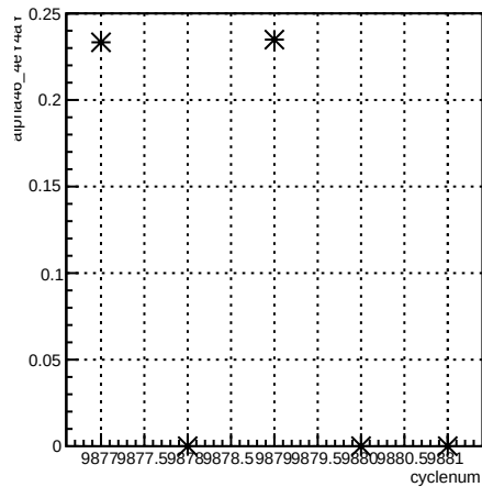
alpha46_4eY4aY:cyclenum {run == 7932}
