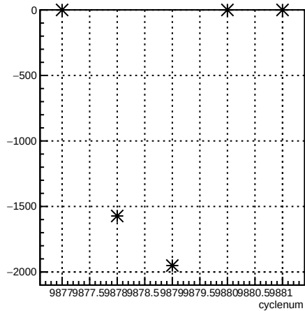
usr_coil3:cyclenum {run == 7932}
