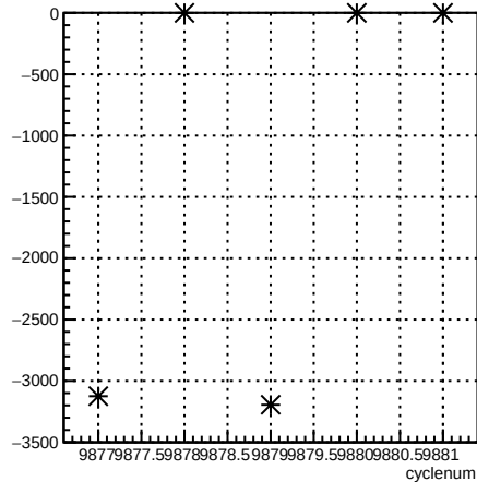
usl_coil6:cyclenum {run == 7932}
