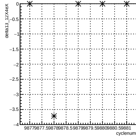
delta13_12X4eX:cyclenum {run == 7932}
