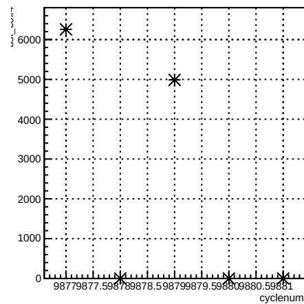
usl_coil4:cyclenum {run == 7932}
