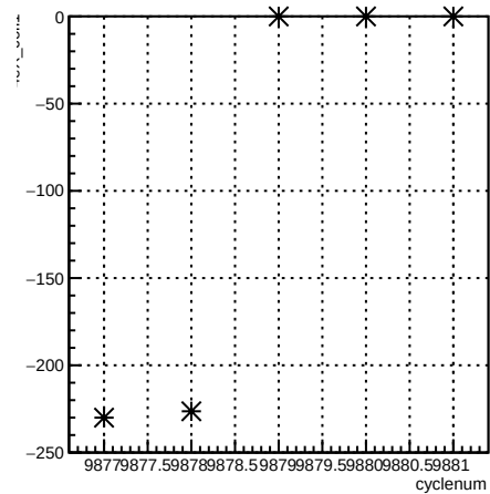
4eX_coil1:cyclenum {run == 7932}
