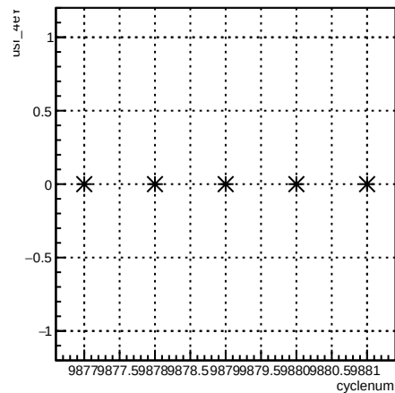
usr_4eY:cyclenum {run == 7932}
