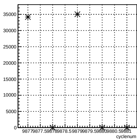
usr_coil7:cyclenum {run == 7932}
