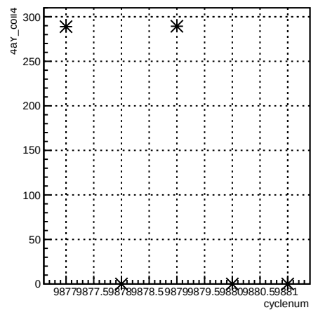
4aY_coil4:cyclenum {run == 7932}
