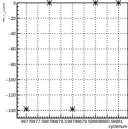
4eY_coil6:cyclenum {run == 7932}
