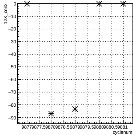
12X_coil3:cyclenum {run == 7932}
