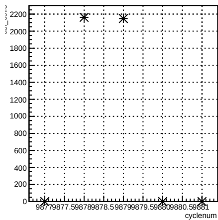
usl_coil3:cyclenum {run == 7932}
