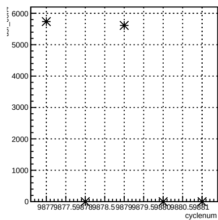
usr_coil4:cyclenum {run == 7932}
