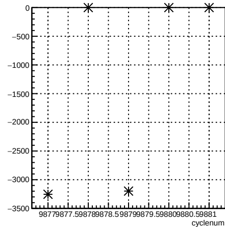
usr_coil6:cyclenum {run == 7932}
