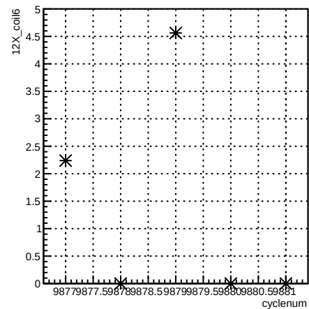
12X_coil6:cyclenum {run == 7932}
