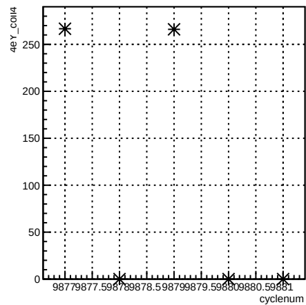
4eY_coil4:cyclenum {run == 7932}
