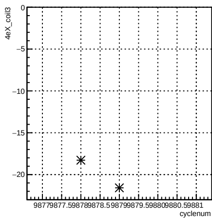
4eX_coil3:cyclenum {run == 7932}
