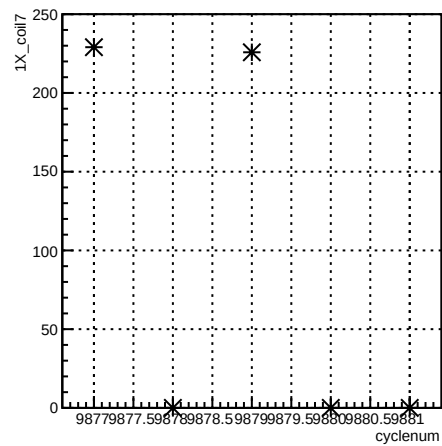
1X_coil7:cyclenum {run == 7932}
