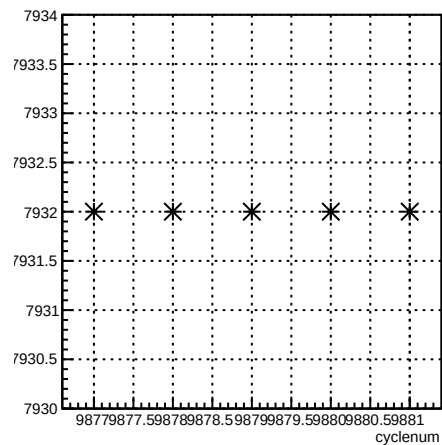
run:cyclenum {run == 7932}
