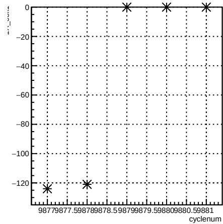
1X_coil1:cyclenum {run == 7932}
