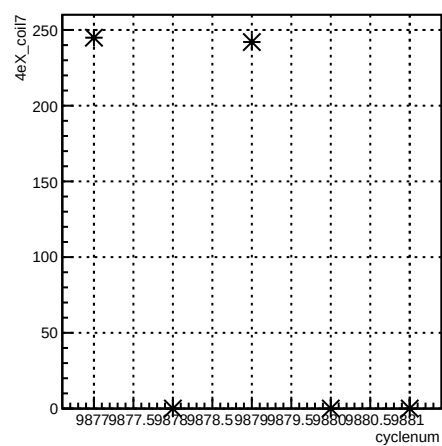
4eX_coil7:cyclenum {run == 7932}
