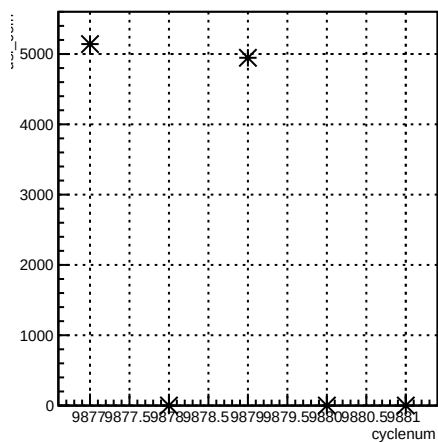
usl_coil7:cyclenum {run == 7932}
