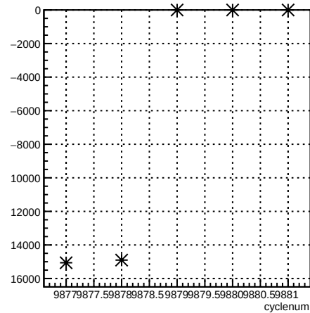
usr_coil1:cyclenum {run == 7932}
