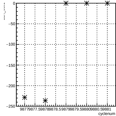
12X_coil1:cyclenum {run == 7932}
