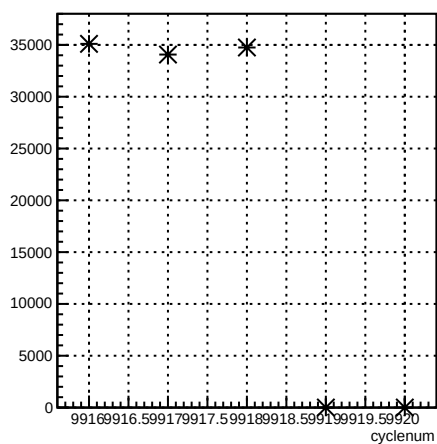
usr_coil7:cyclenum {run == 7940}
