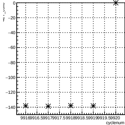
4eY_coil6:cyclenum {run == 7940}
