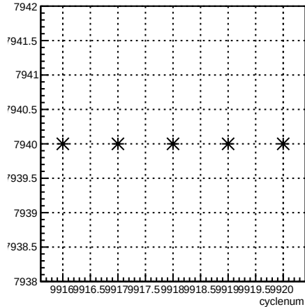
run:cyclenum {run == 7940}
