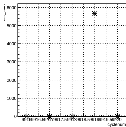
usr_coil4:cyclenum {run == 7940}
