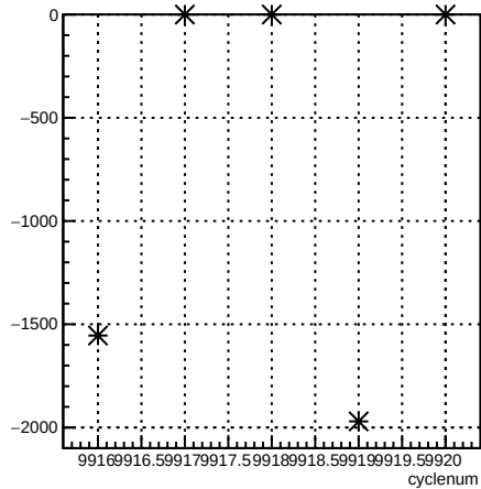
usr_coil3:cyclenum {run == 7940}
