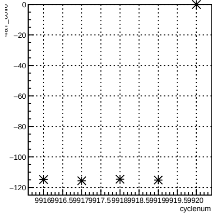
4aY_coil6:cyclenum {run == 7940}
