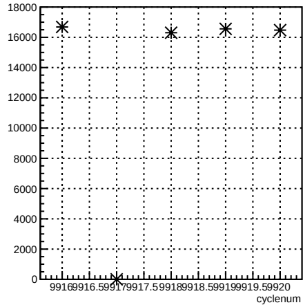
usl_coil1:cyclenum {run == 7940}
