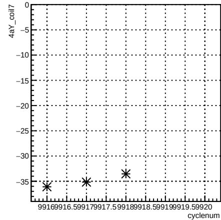
4aY_coil7:cyclenum {run == 7940}
