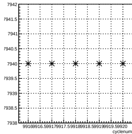
run:cyclenum {run == 7940}
