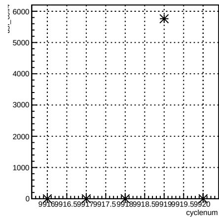
usl_coil4:cyclenum {run == 7940}
