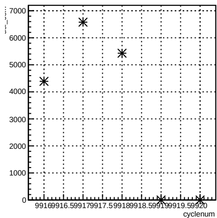
usl_coil7:cyclenum {run == 7940}
