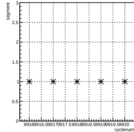
segment:cyclenum {run == 7940}
