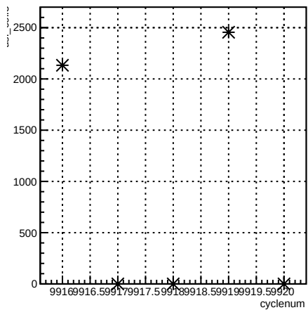
usl_coil3:cyclenum {run == 7940}
