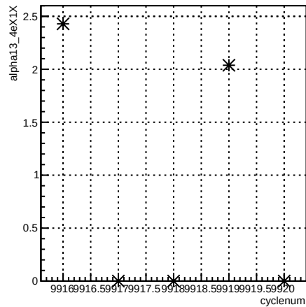
alpha13_4eX1X:cyclenum {run == 7940}
