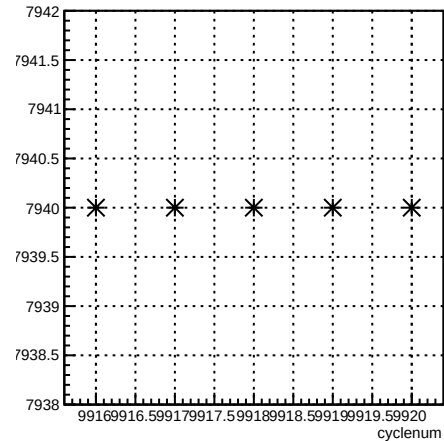
run:cyclenum {run == 7940}
