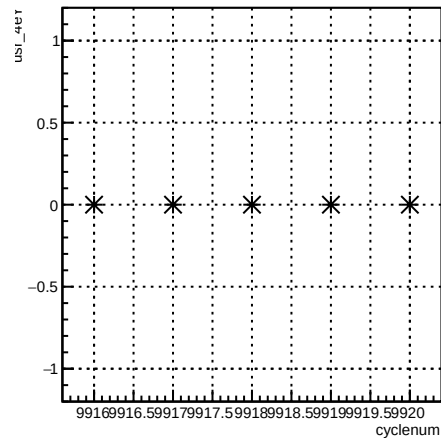
usr_4eY:cyclenum {run == 7940}
