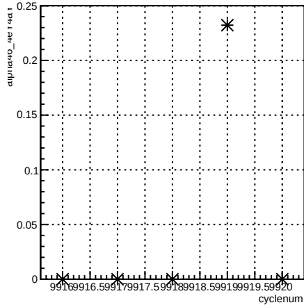
alpha46_4eY4aY:cyclenum {run == 7940}
