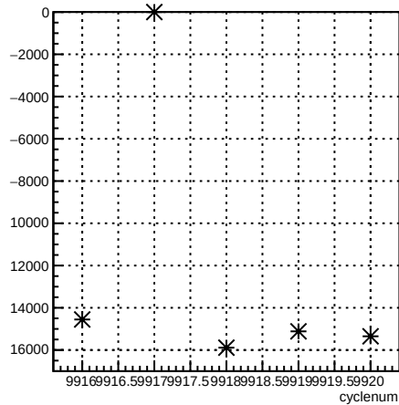
usr_coil1:cyclenum {run == 7940}
