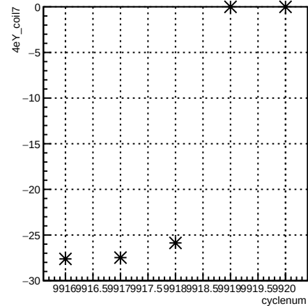
4eY_coil7:cyclenum {run == 7940}
