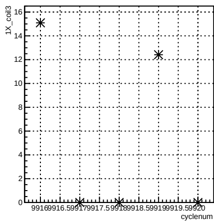
1X_coil3:cyclenum {run == 7940}
