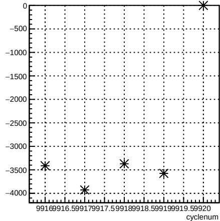
usl_coil6:cyclenum {run == 7940}
