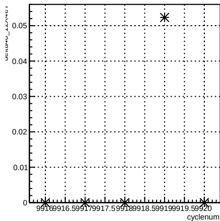
delta46_12X4eY:cyclenum {run == 7940}
