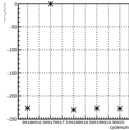
4eX_coil1:cyclenum {run == 7940}
