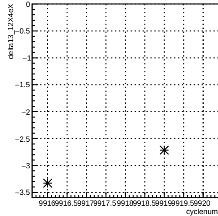
delta13_12X4eX:cyclenum {run == 7940}
