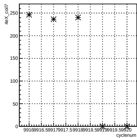
4eX_coil7:cyclenum {run == 7940}
