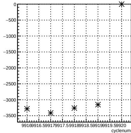
usr_coil6:cyclenum {run == 7940}
