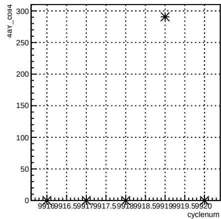
4aY_coil4:cyclenum {run == 7940}
