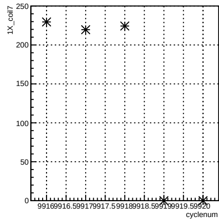
1X_coil7:cyclenum {run == 7940}
