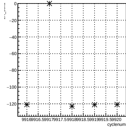
1X_coil1:cyclenum {run == 7940}
