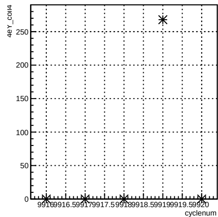
4eY_coil4:cyclenum {run == 7940}
