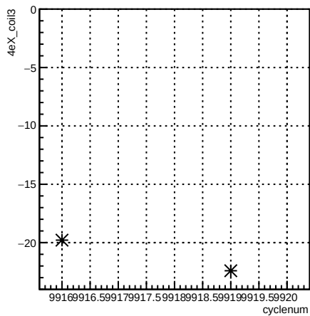
4eX_coil3:cyclenum {run == 7940}
