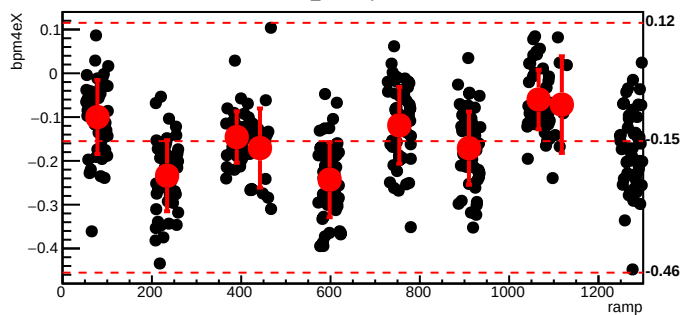
bmod_trim3,cyc=9916
