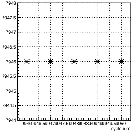
run:cyclenum {run == 7946}
