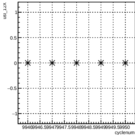
usl_12X:cyclenum {run == 7946}
