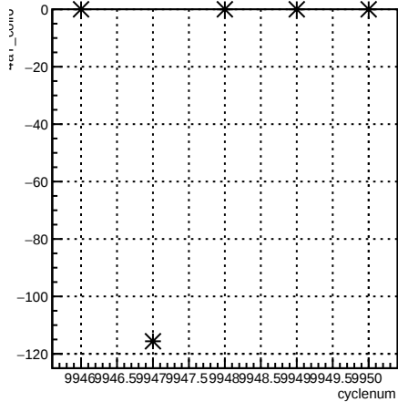
4aY_coil6:cyclenum {run == 7946}
