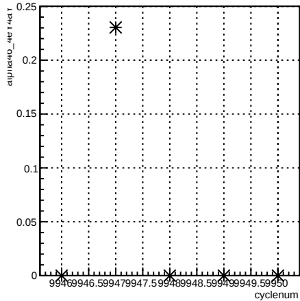
alpha46_4eY4aY:cyclenum {run == 7946}
