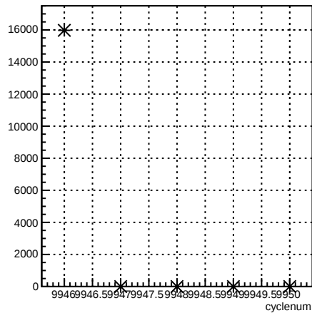
usl_coil6:cyclenum {run == 7946}
