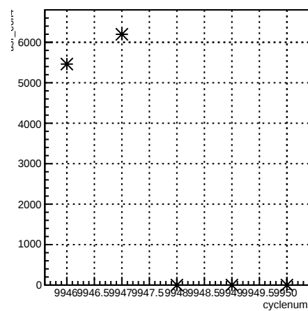
usr_coil4:cyclenum {run == 7946}
