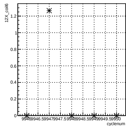
12X_coil6:cyclenum {run == 7946}
