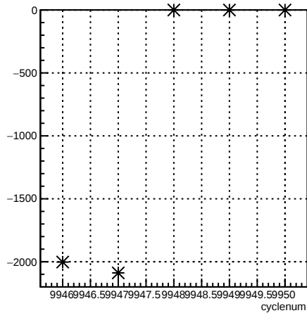
usr_coil3:cyclenum {run == 7946}
