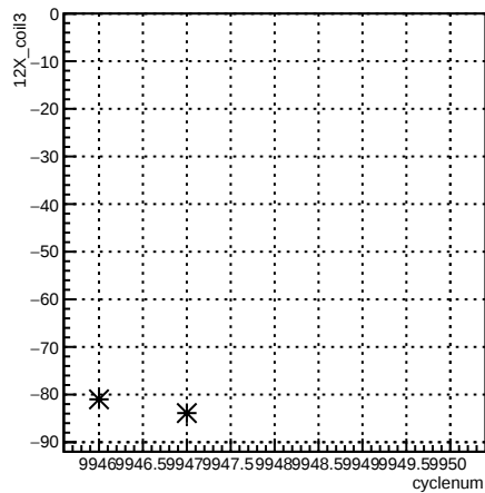
12X_coil3:cyclenum {run == 7946}
