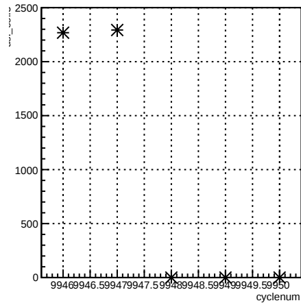
usl_coil3:cyclenum {run == 7946}
