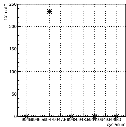
1X_coil7:cyclenum {run == 7946}
