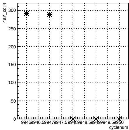
4aY_coil4:cyclenum {run == 7946}
