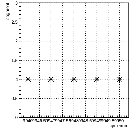
segment:cyclenum {run == 7946}
