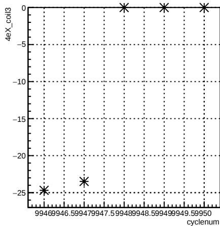
4eX_coil3:cyclenum {run == 7946}
