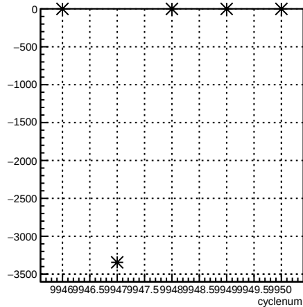
usl_coil6:cyclenum {run == 7946}
