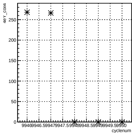
4eY_coil4:cyclenum {run == 7946}
