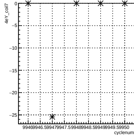
4eY_coil7:cyclenum {run == 7946}
