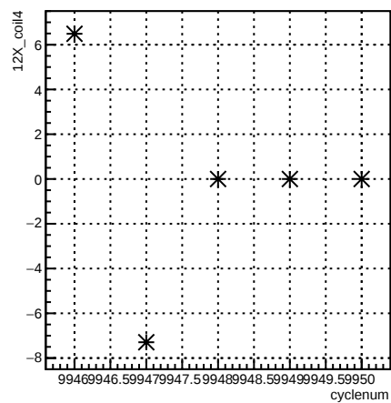
12X_coil4:cyclenum {run == 7946}
