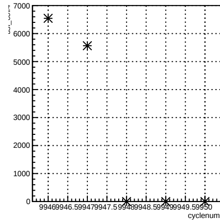
usl_coil4:cyclenum {run == 7946}
