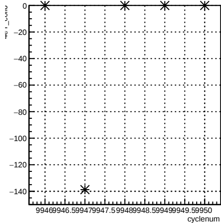
4eY_coil6:cyclenum {run == 7946}
