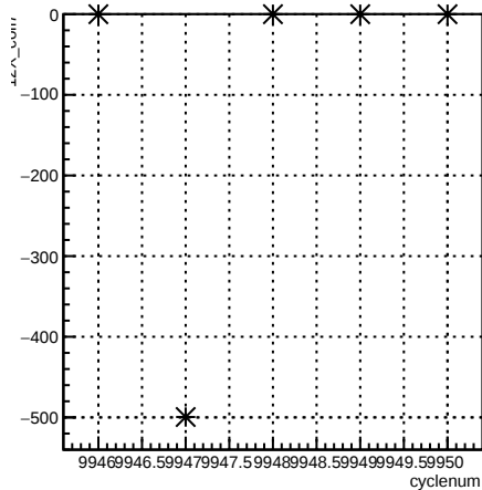
12X_coil7:cyclenum {run == 7946}
