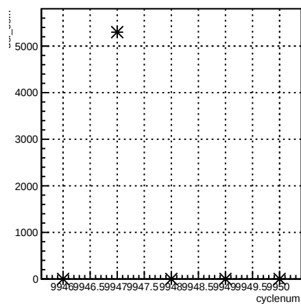
usl_coil7:cyclenum {run == 7946}
