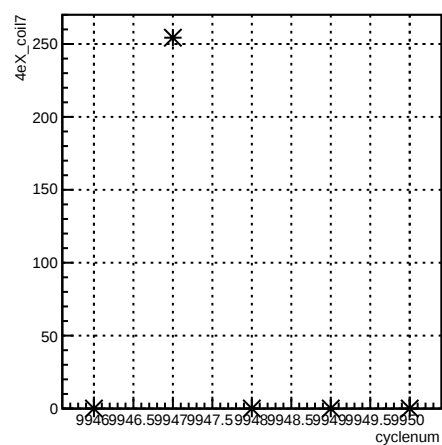
4eX_coil7:cyclenum {run == 7946}
