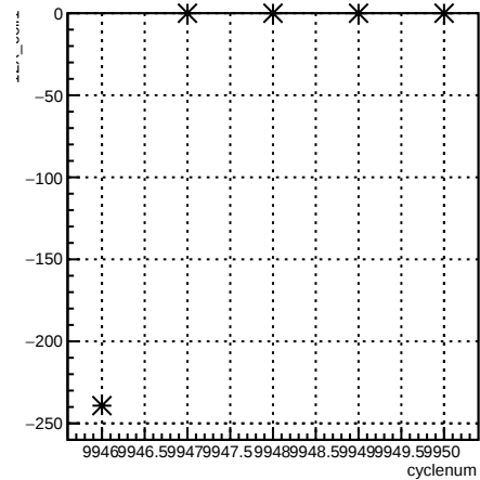
12X_coil1:cyclenum {run == 7946}
