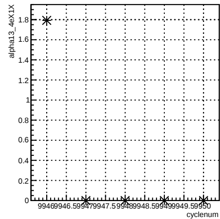
alpha13_4eX1X:cyclenum {run == 7946}
