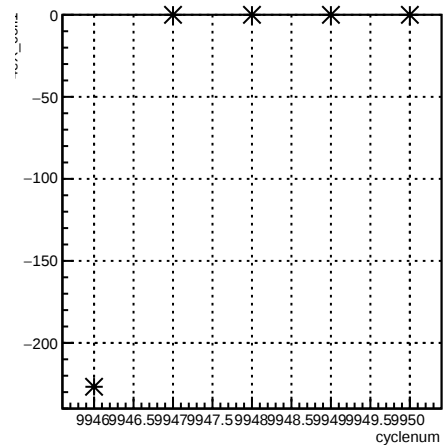
4eX_coil1:cyclenum {run == 7946}
