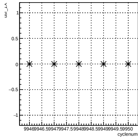
usr_4eY:cyclenum {run == 7946}
