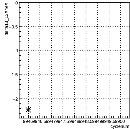
delta13_12X4eX:cyclenum {run == 7946}
