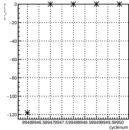
1X_coil1:cyclenum {run == 7946}
