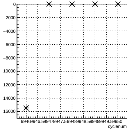
usr_coil1:cyclenum {run == 7946}
