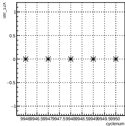
usr_12X:cyclenum {run == 7946}
