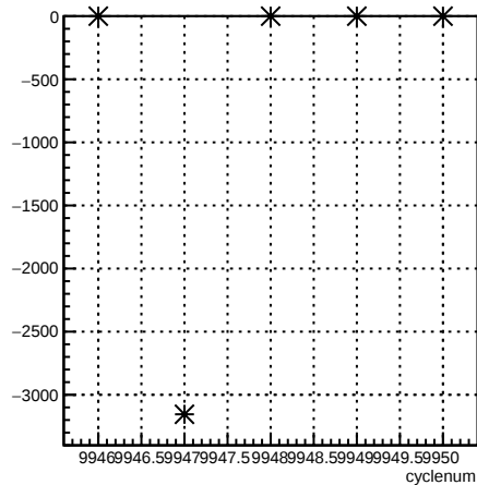
usr_coil6:cyclenum {run == 7946}
