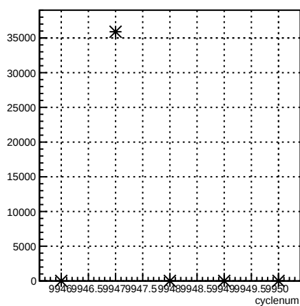
usr_coil7:cyclenum {run == 7946}
