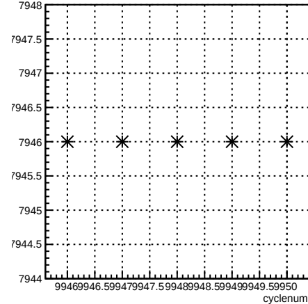
run:cyclenum {run == 7946}
