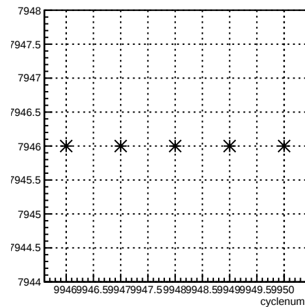
run:cyclenum {run == 7946}
