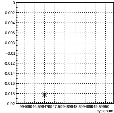
delta46_12X4eY:cyclenum {run == 7946}
