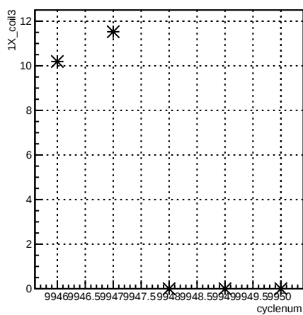
1X_coil3:cyclenum {run == 7946}
