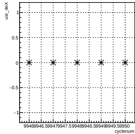
run:cyclenum {run == 7946}
