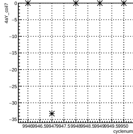
4aY_coil7:cyclenum {run == 7946}
