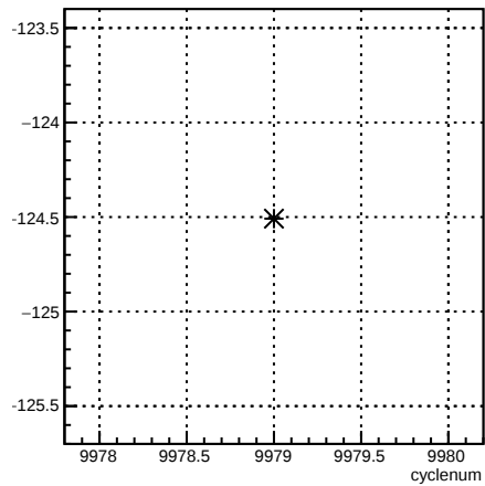
usr_4eY:cyclenum {run == 7953}
