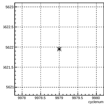
usr_coil4:cyclenum {run == 7953}
