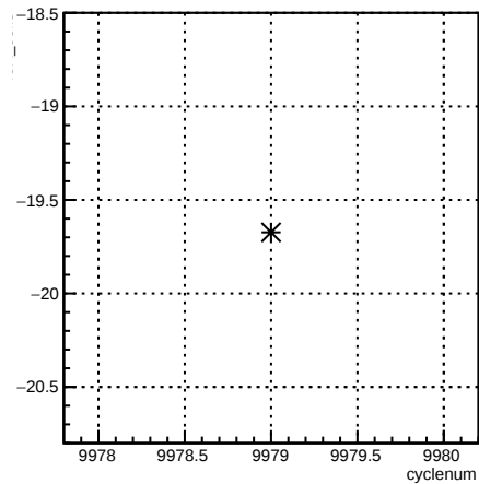
4eX_coil3:cyclenum {run == 7953}
