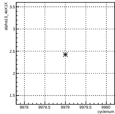
alpha13_4eX1X:cyclenum {run == 7953}
