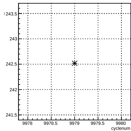
1X_coil7:cyclenum {run == 7953}
