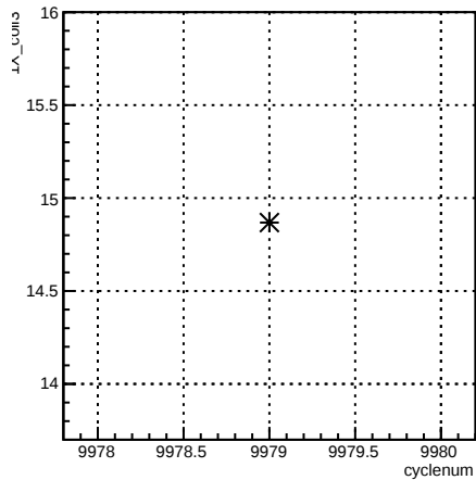
1X_coil3:cyclenum {run == 7953}
