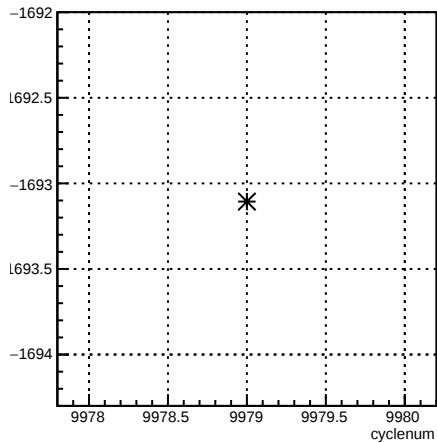
usr_coil3:cyclenum {run == 7953}
