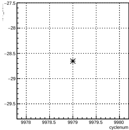
4eY_coil7:cyclenum {run == 7953}
