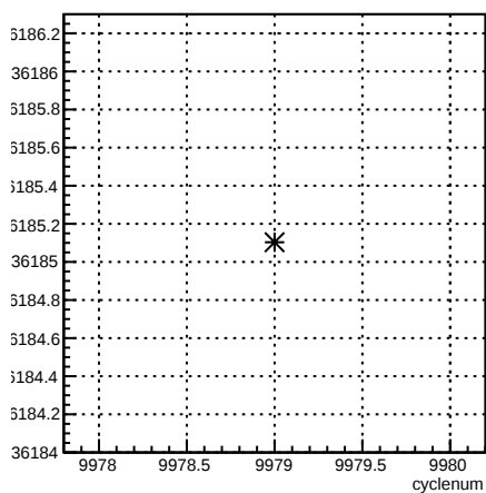
usr_coil7:cyclenum {run == 7953}
