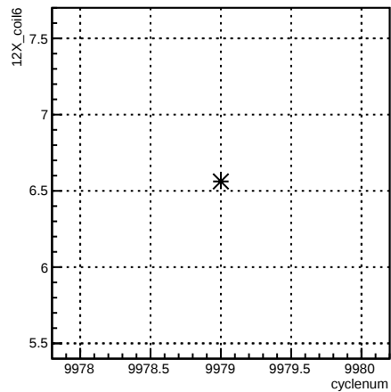
12X_coil6:cyclenum {run == 7953}
