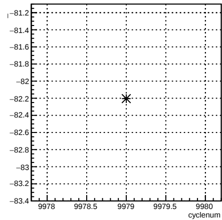
usl_4eY:cyclenum {run == 7953}
