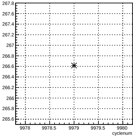
4eY_coil4:cyclenum {run == 7953}
