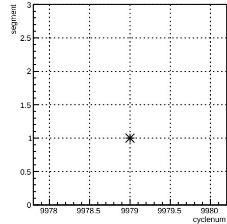
segment:cyclenum {run == 7953}
