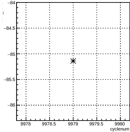
12X_coil7:cyclenum {run == 7953}
