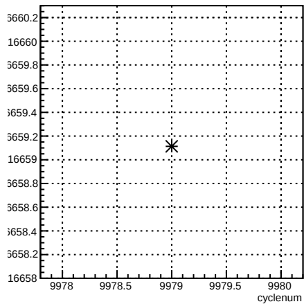
usl_coil6:cyclenum {run == 7953}
