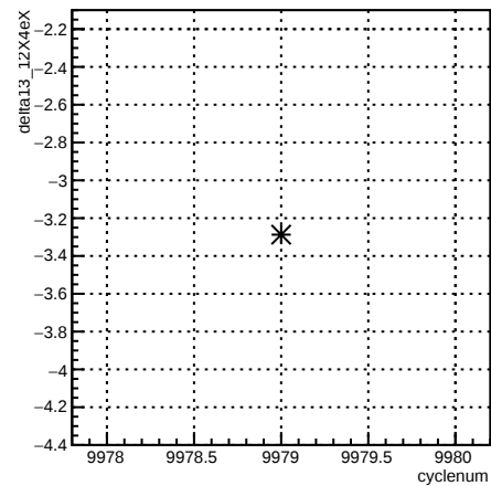
delta13_12X4eX:cyclenum {run == 7953}
