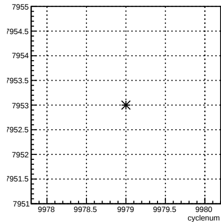
run:cyclenum {run == 7953}
