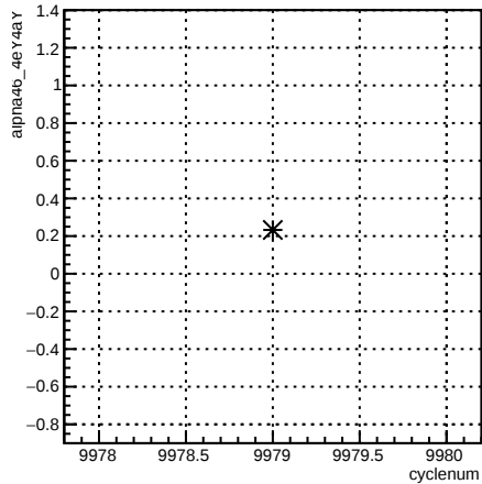
alpha46_4eY4aY:cyclenum {run == 7953}
