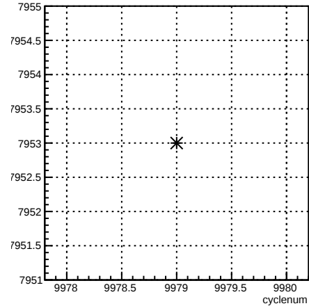
run:cyclenum {run == 7953}
