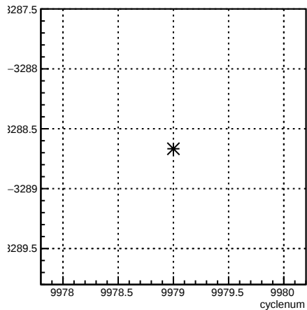
usr_coil6:cyclenum {run == 7953}
