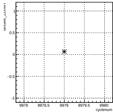
delta46_12X4eY:cyclenum {run == 7953}
