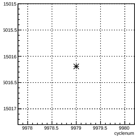
usr_coil1:cyclenum {run == 7953}
