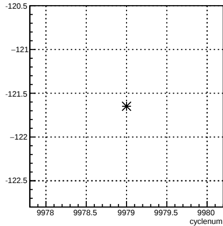
1X_coil1:cyclenum {run == 7953}
