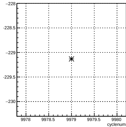
4eX_coil1:cyclenum {run == 7953}
