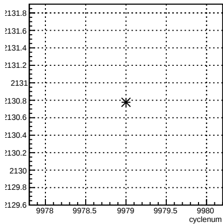
usl_coil7:cyclenum {run == 7953}
