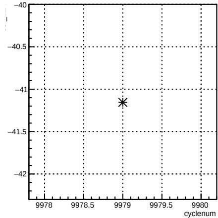
usr_12X:cyclenum {run == 7953}
