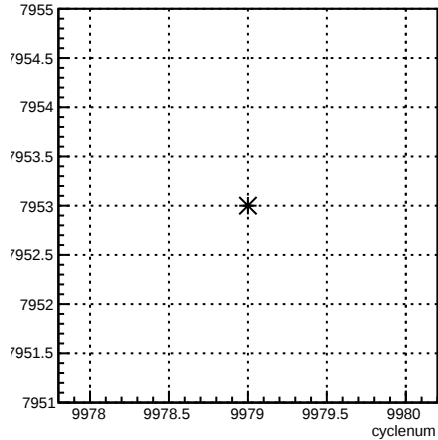
run:cyclenum {run == 7953}
