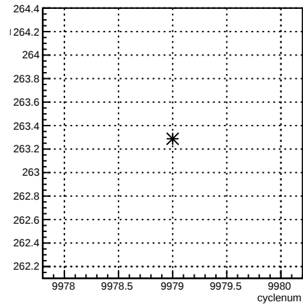
4eX_coil7:cyclenum {run == 7953}
