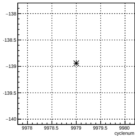
4eY_coil6:cyclenum {run == 7953}
