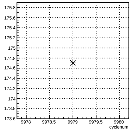
run:cyclenum {run == 7953}
