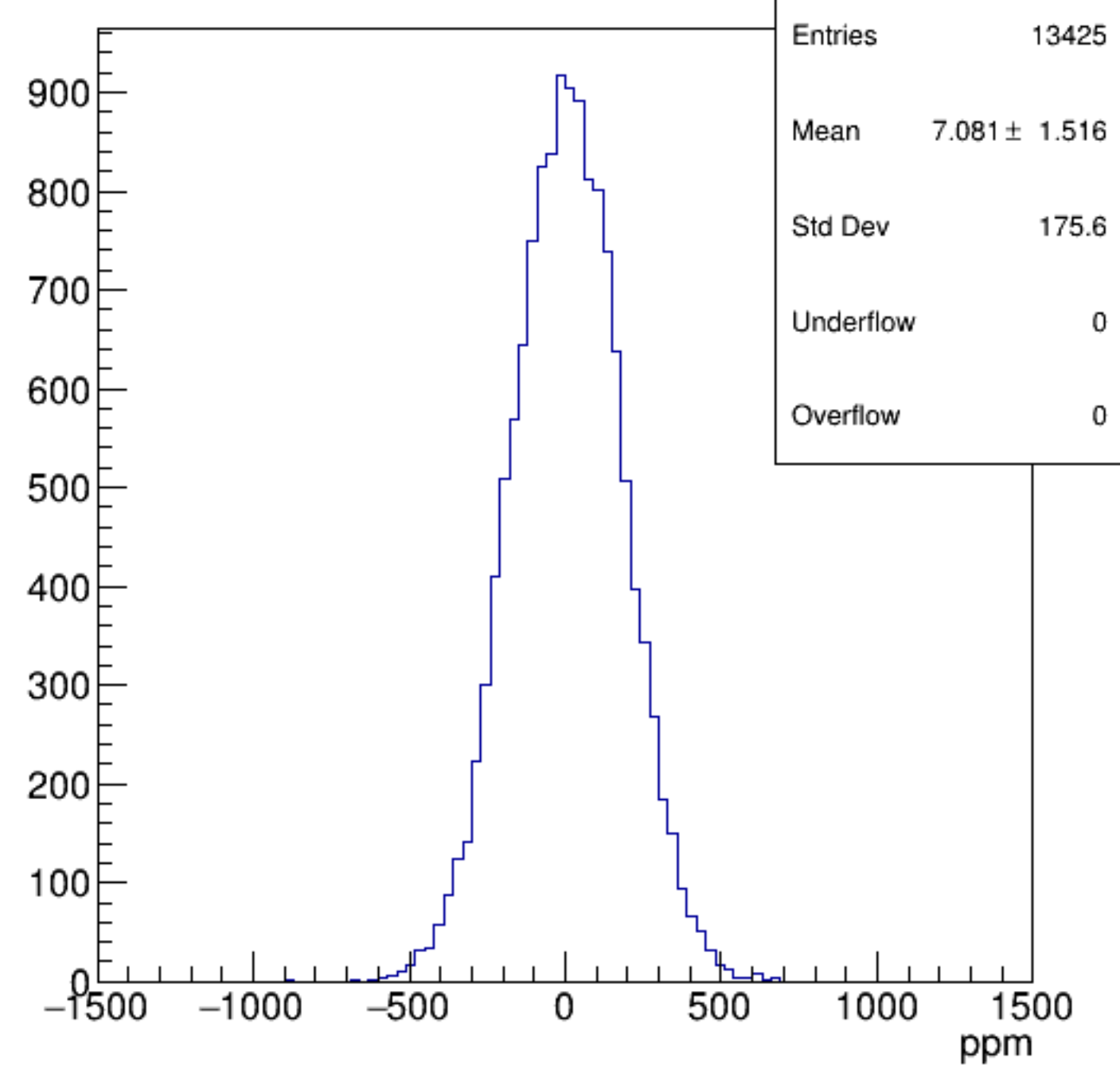
asym_bcm0l02
