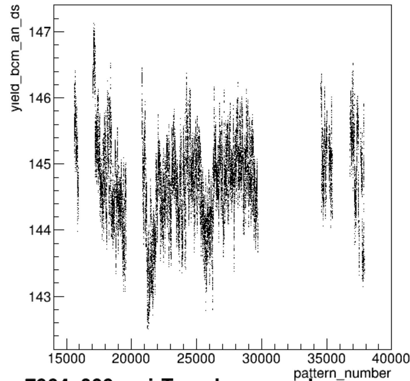
yield_bcm_an_ds:pattern_number {ErrorFlag==0}
