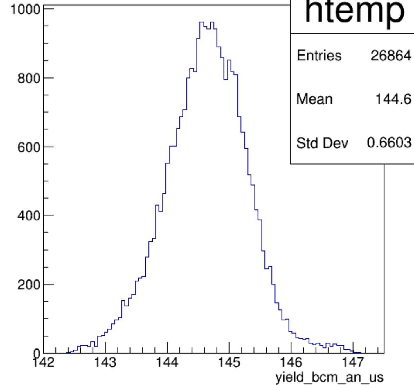
yield_bcm_an_us {ErrorFlag==0}
