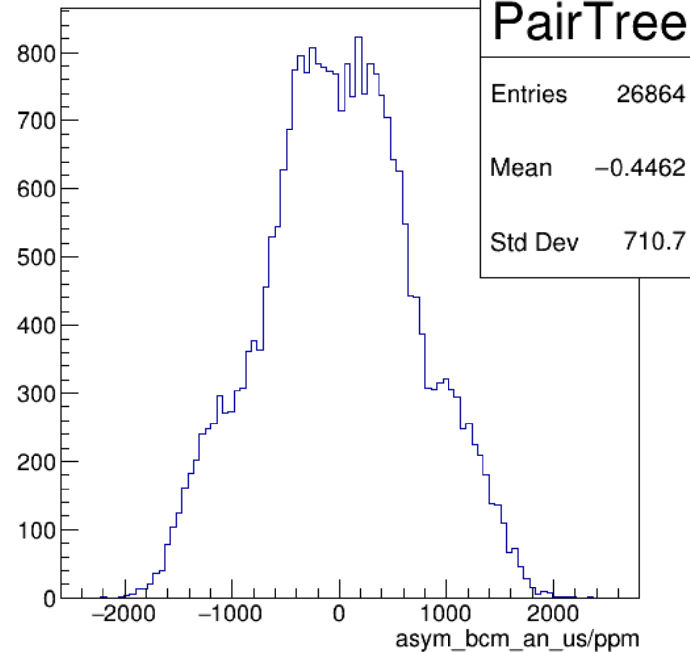
asym_bcm_an_us/ppm {ErrorFlag==0}
