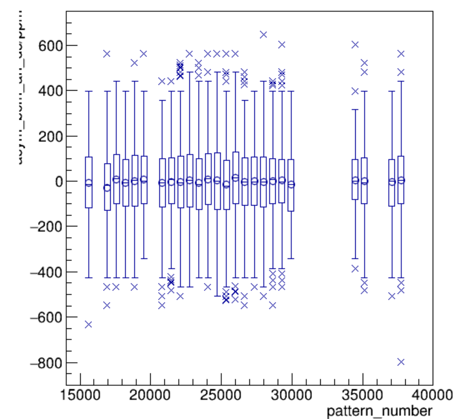
asym_bcm_an_ds/ppm:pattern_number {ErrorFlag==0}
