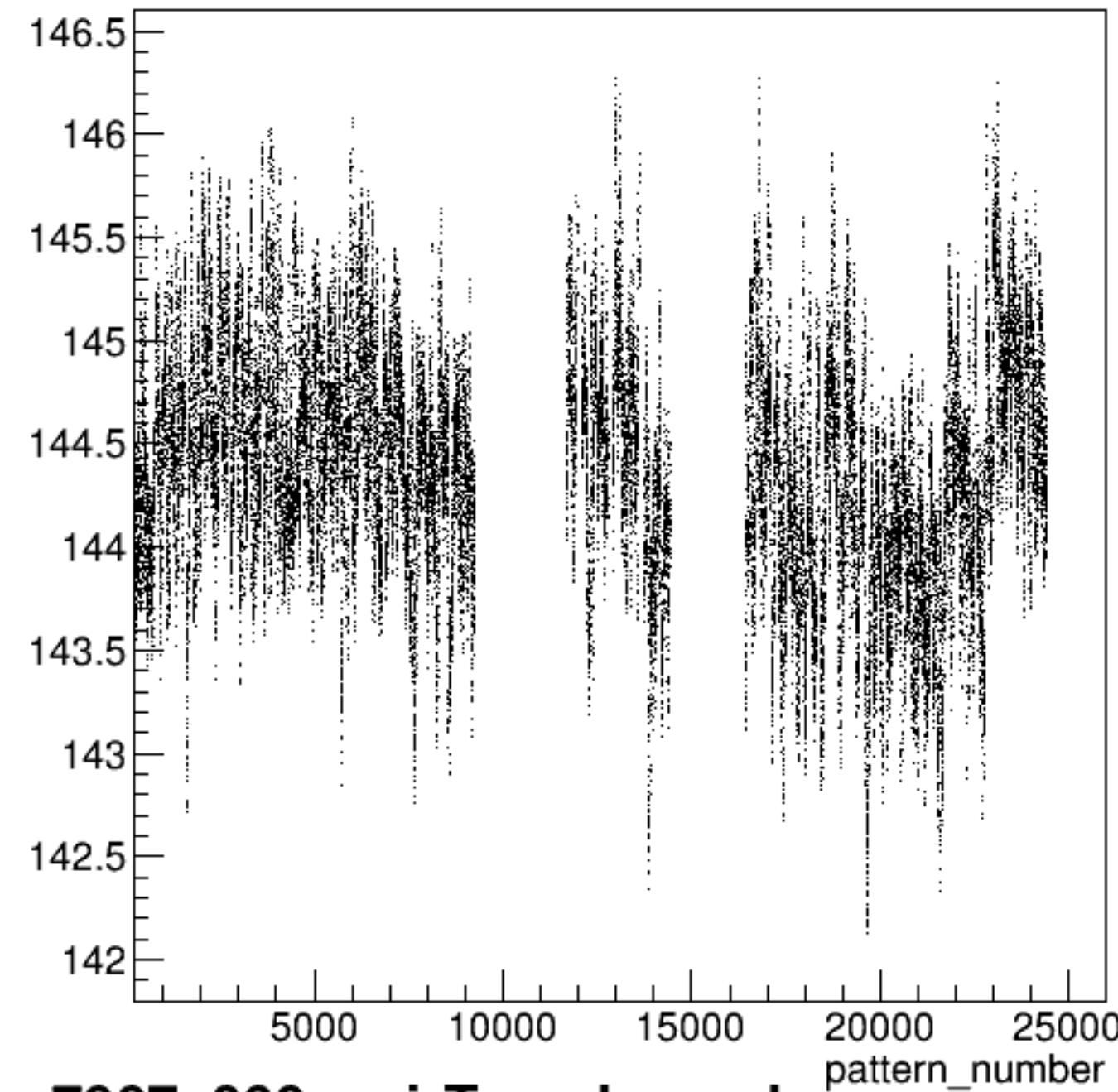
yield_bcm_dg_us:pattern_number {ErrorFlag==0}
