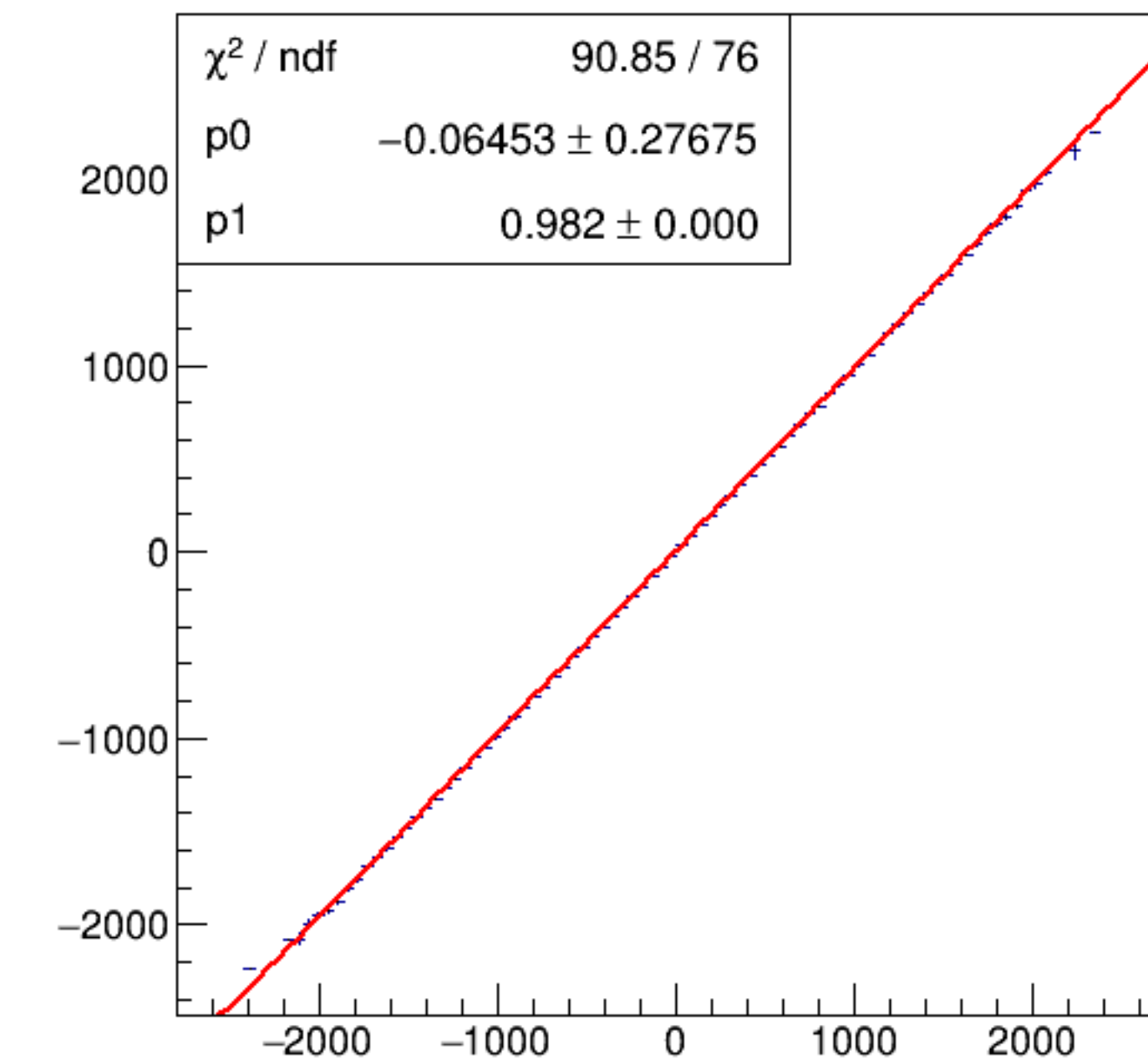
run7967_000_asym_bcm_dg_ds_vs_asym_bcm_an_us_pr.png
