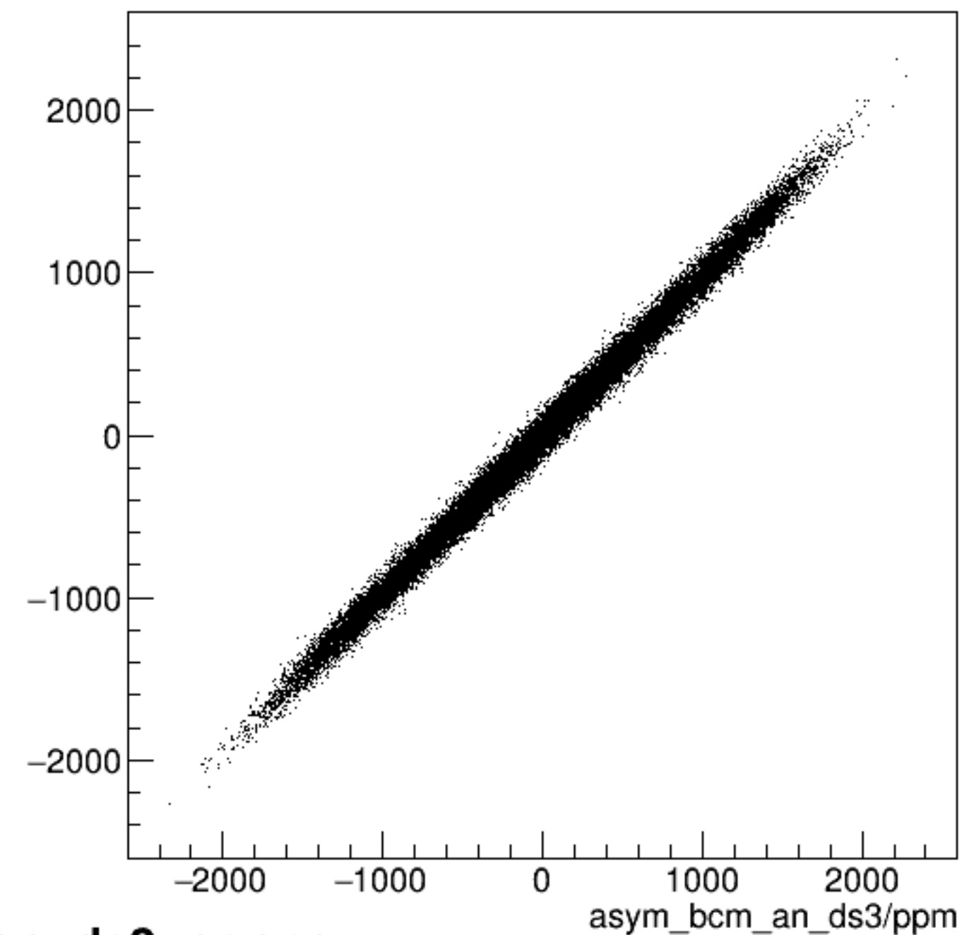
run7967_000_asym_bcm_dg_us_vs_asym_bcm_an_ds3_pr.png
