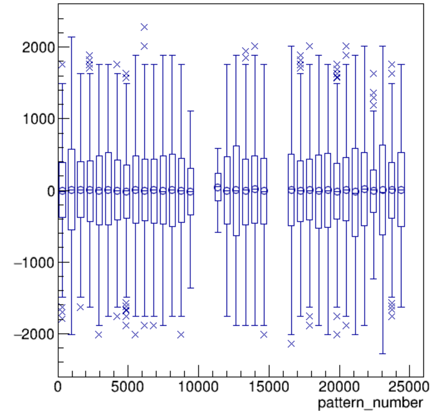
asym_bcm_dg_us/ppm:pattern_number {ErrorFlag==0}
