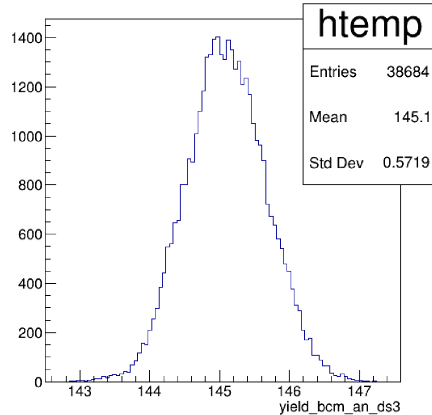
yield_bcm_an_ds3 {ErrorFlag==0}
