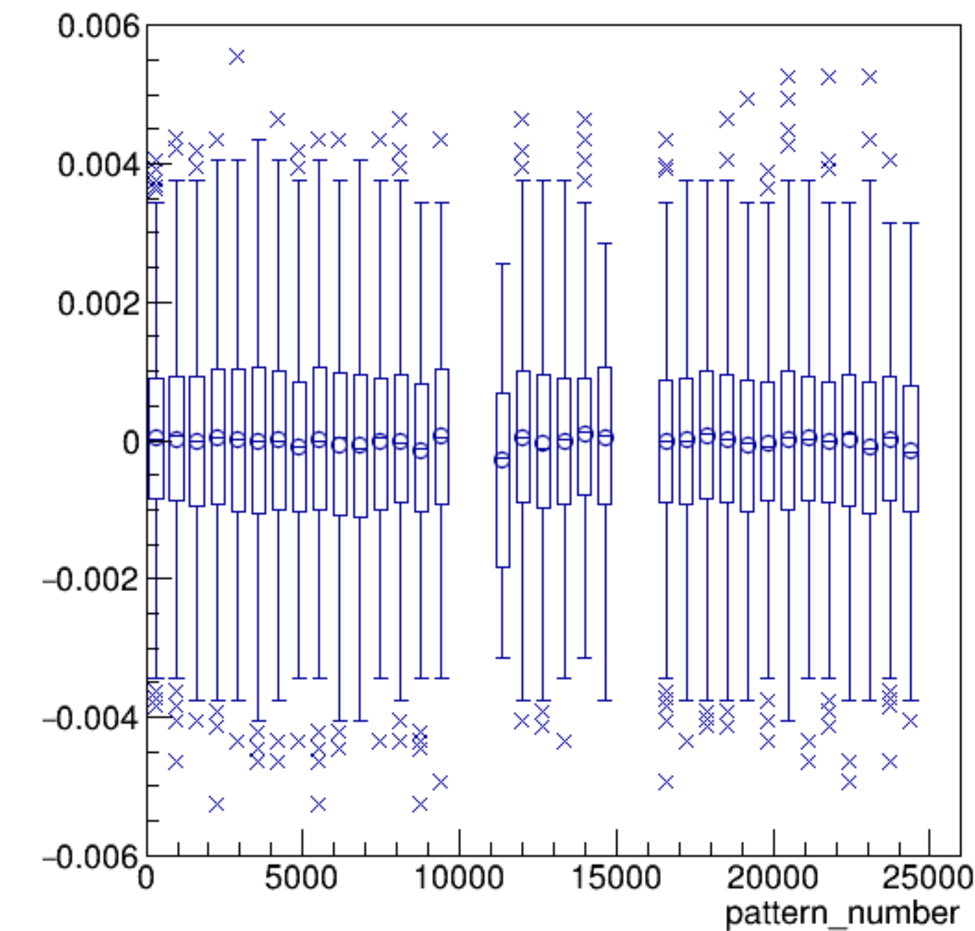
asym_bcm_an_diff*yield_bcm_an_diff:pattern_number {ErrorFlag==0}
