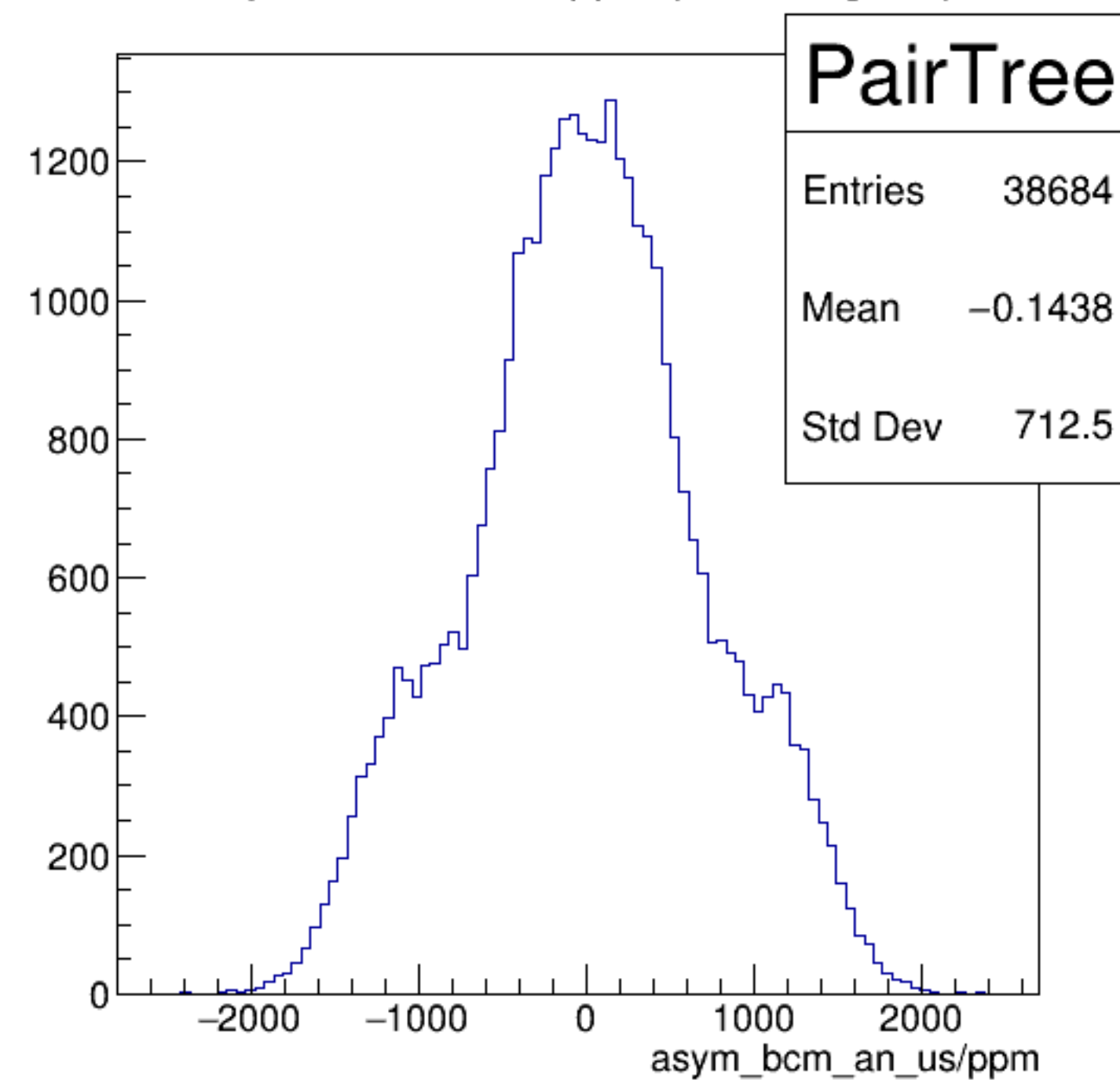
asym_bcm_an_us/ppm {ErrorFlag==0}
