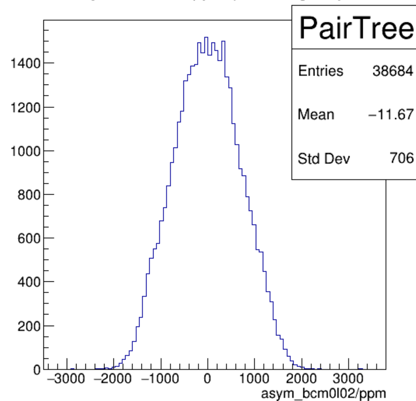
asym_bcm0l02/ppm {ErrorFlag==0}
