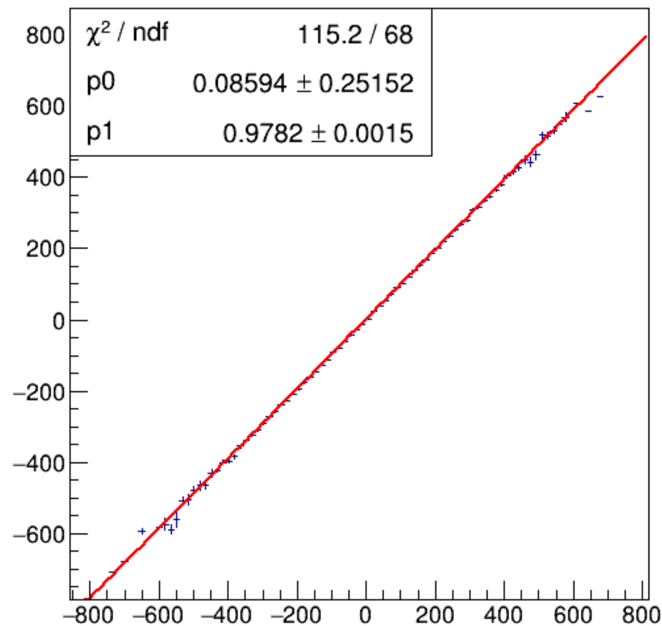
run7967_000_asym_bcm_dg_ds_vs_asym_bcm_an_us_mul.png
