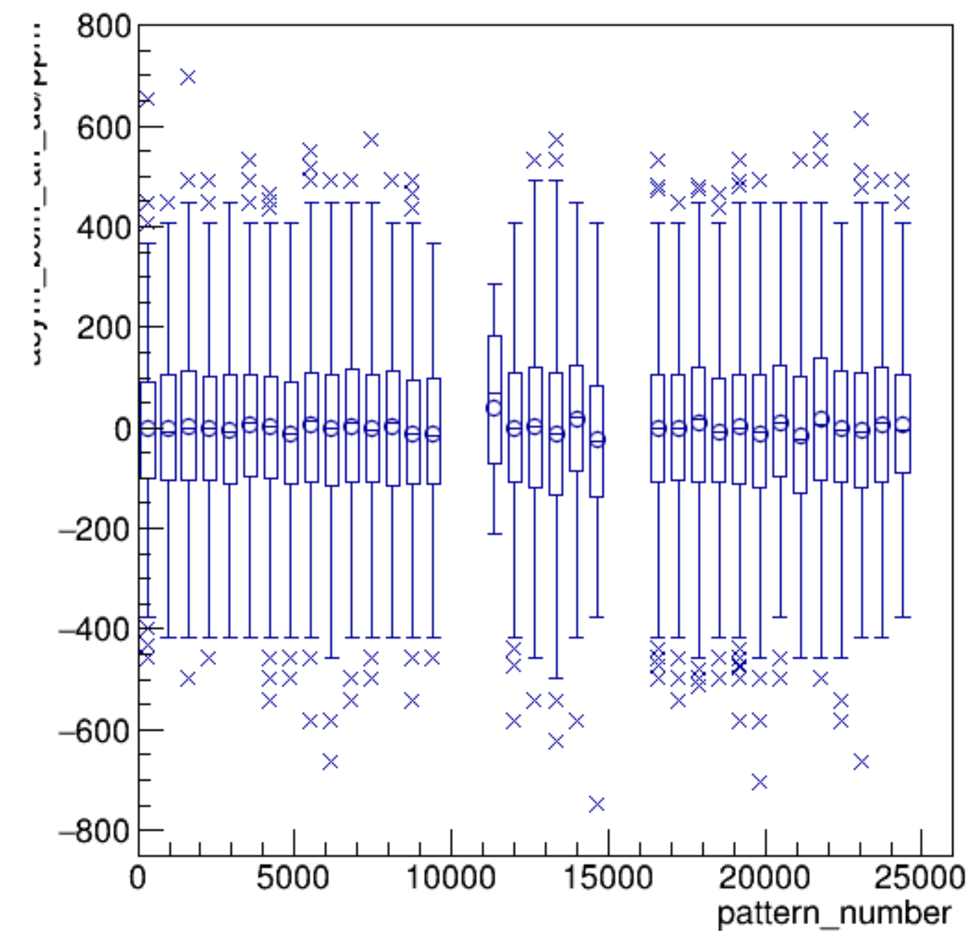
asym_bcm_an_us/ppm:pattern_number {ErrorFlag==0}
