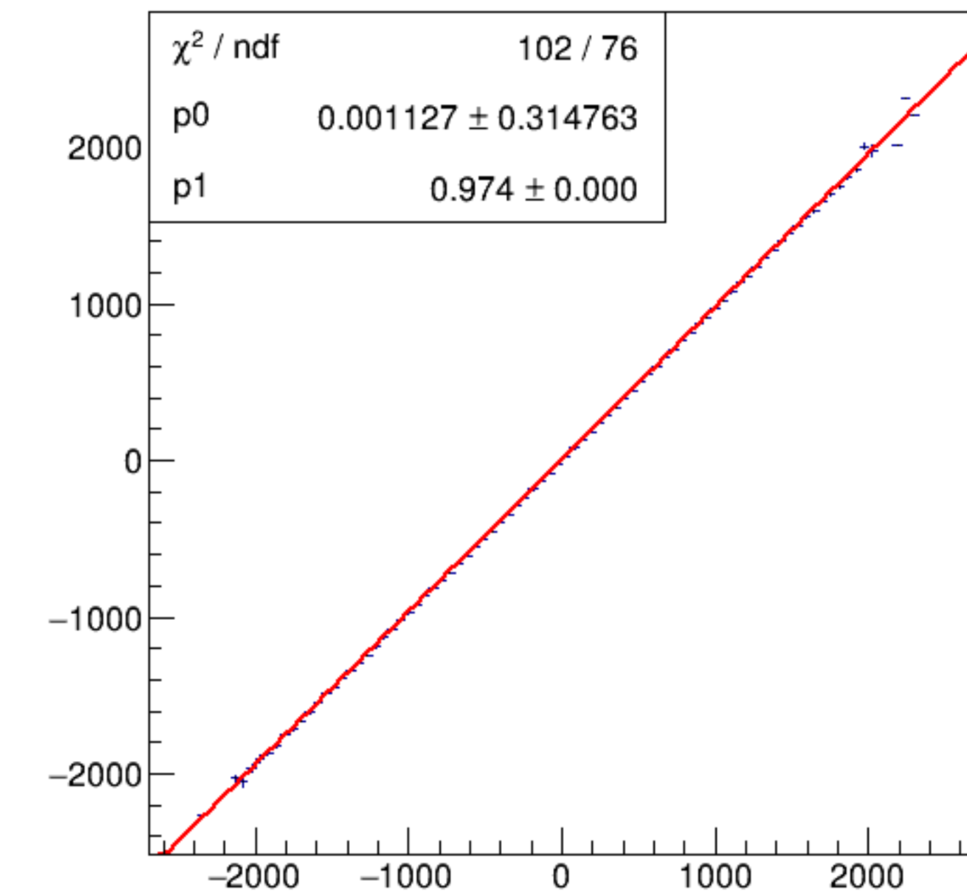
run7967_000_asym_bcm_dg_us_vs_asym_bcm_an_ds3_pr.png
