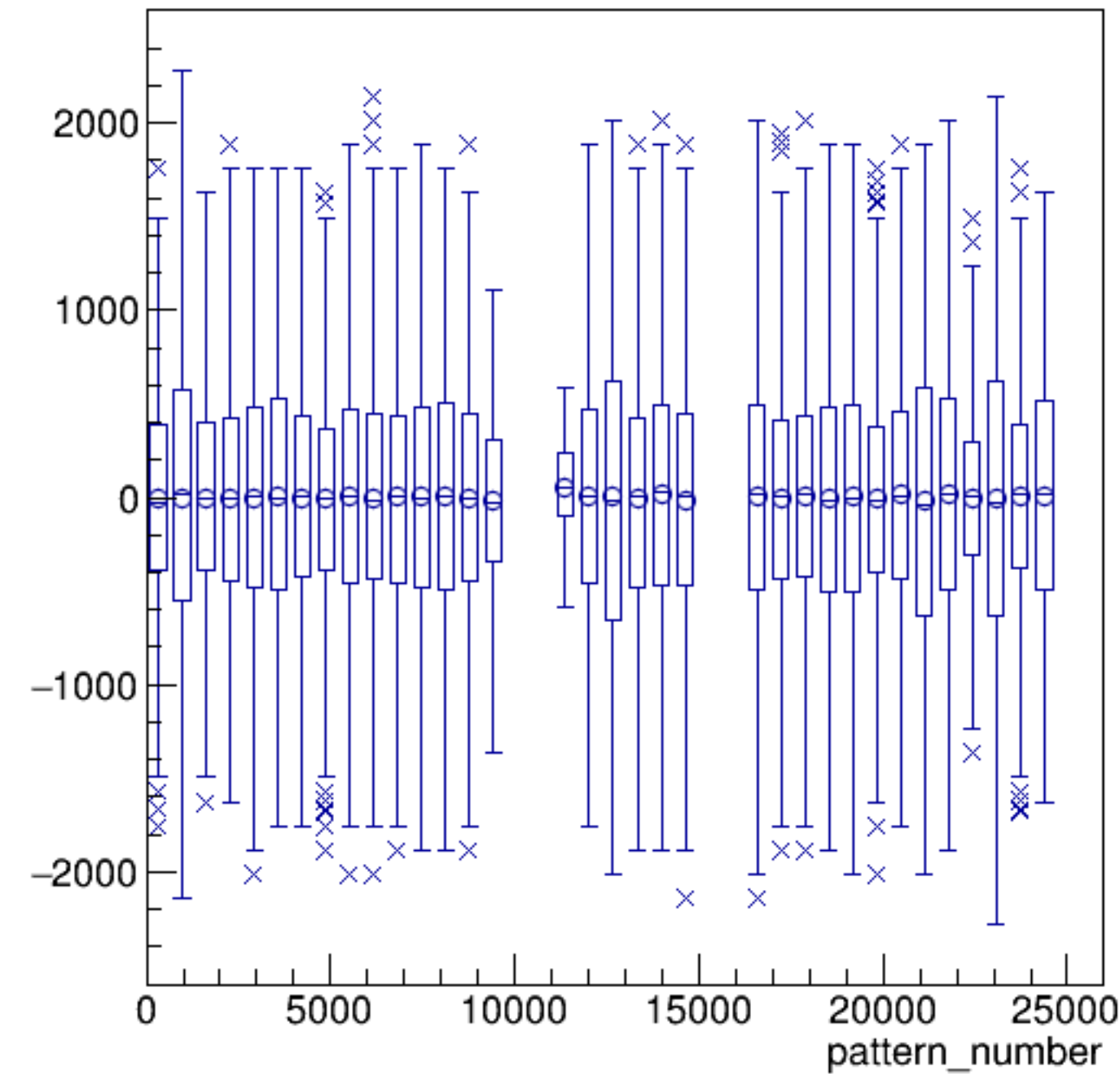
asym_bcm_dg_ds/ppm:pattern_number {ErrorFlag==0}
