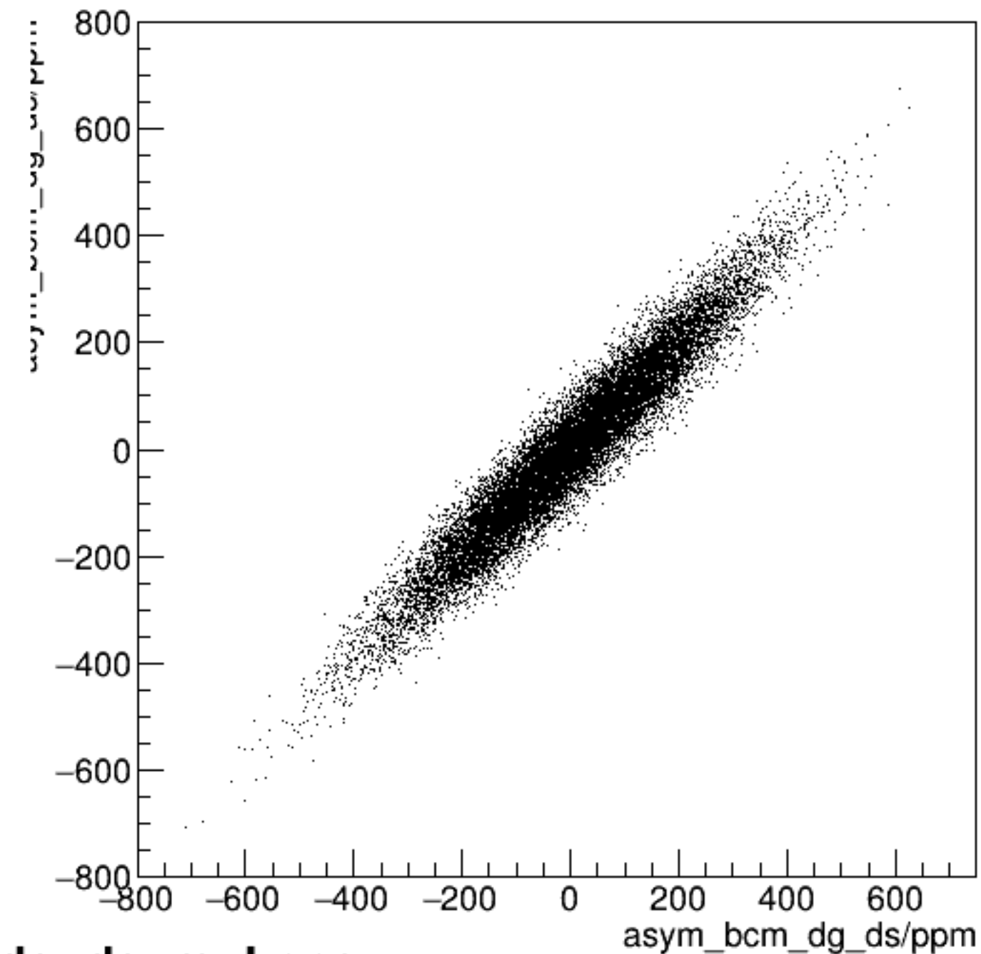
run7967_000_asym_bcm_dg_us_vs_asym_bcm_dg_ds_mul.png
