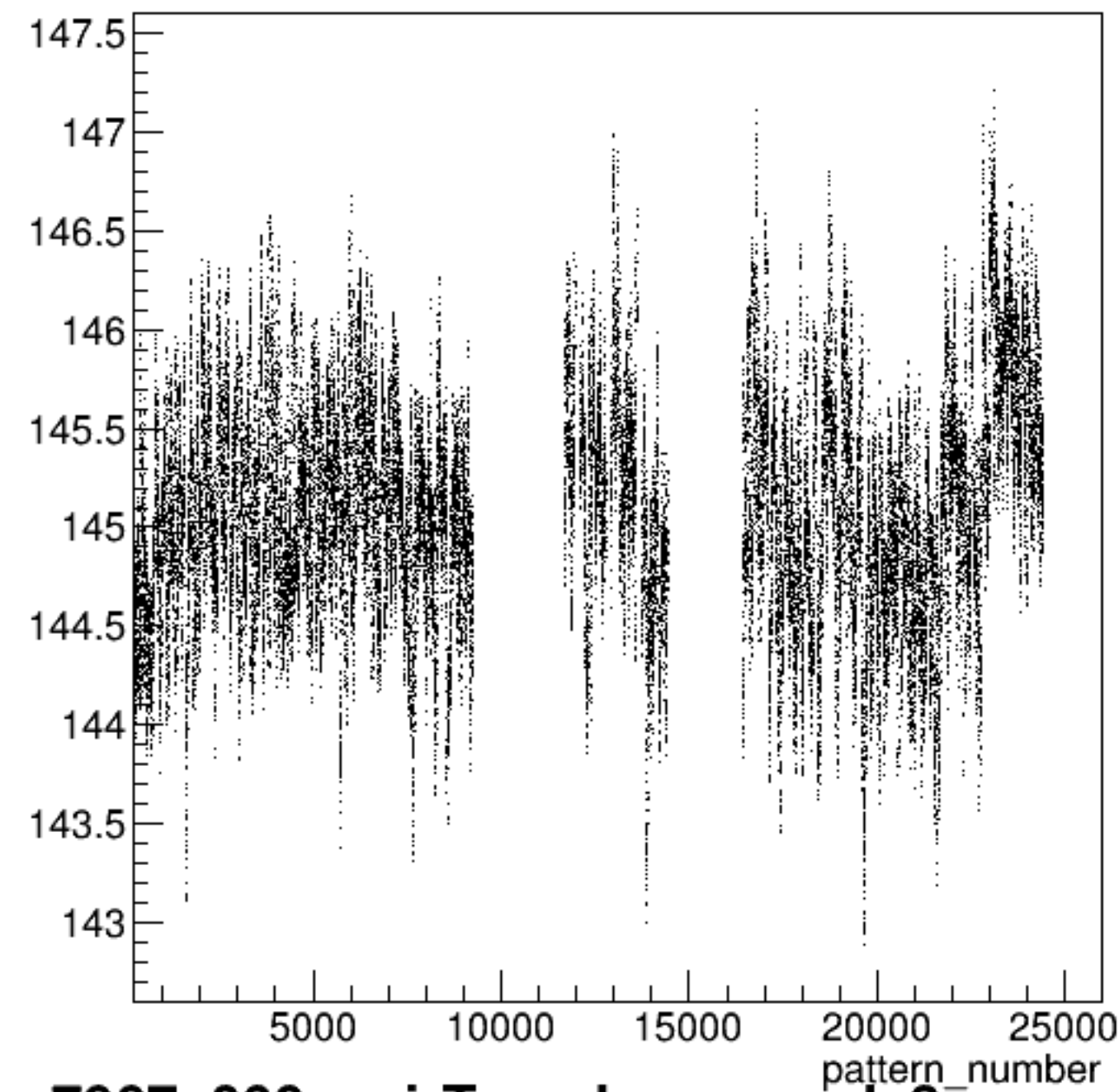
yield_bcm_an_ds3:pattern_number {ErrorFlag==0}
