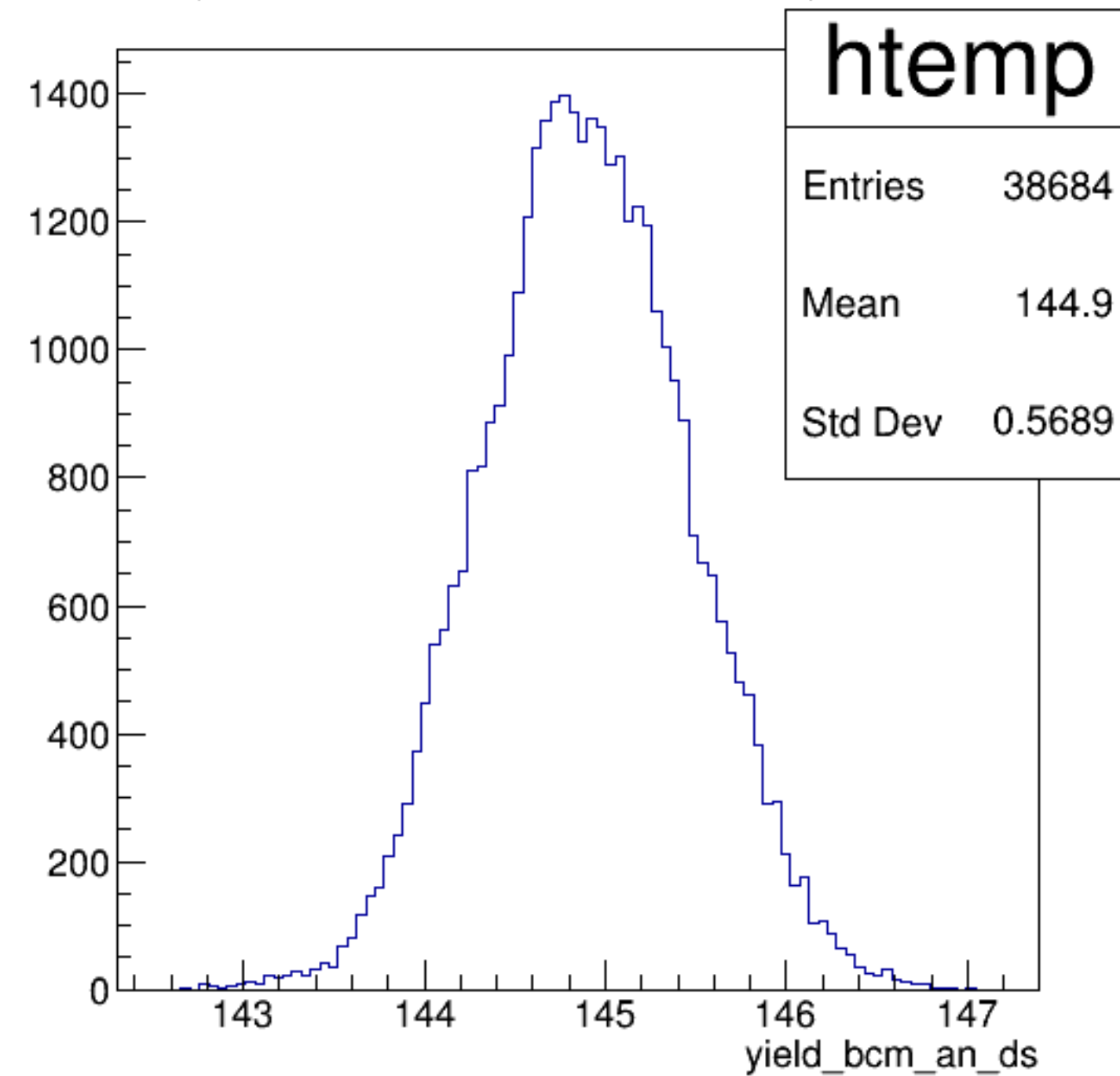
yield_bcm_an_ds {ErrorFlag==0}
