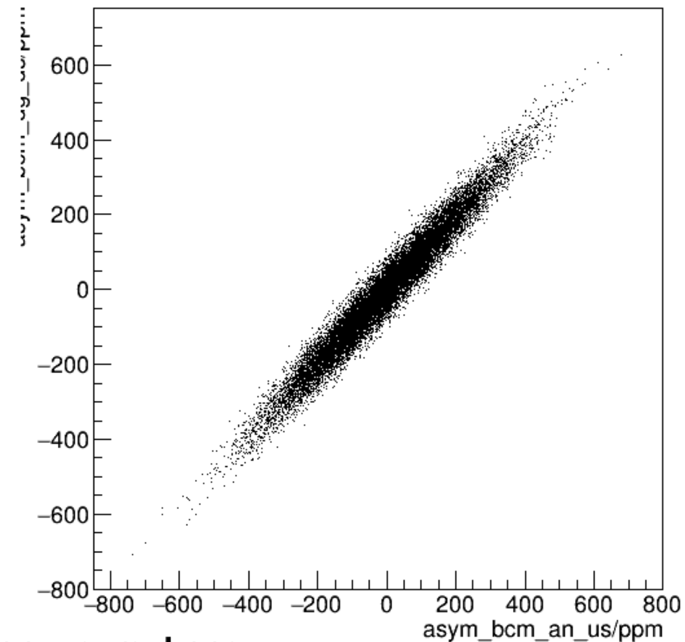
run7967_000_asym_bcm_dg_ds_vs_asym_bcm_an_us_mul.png
