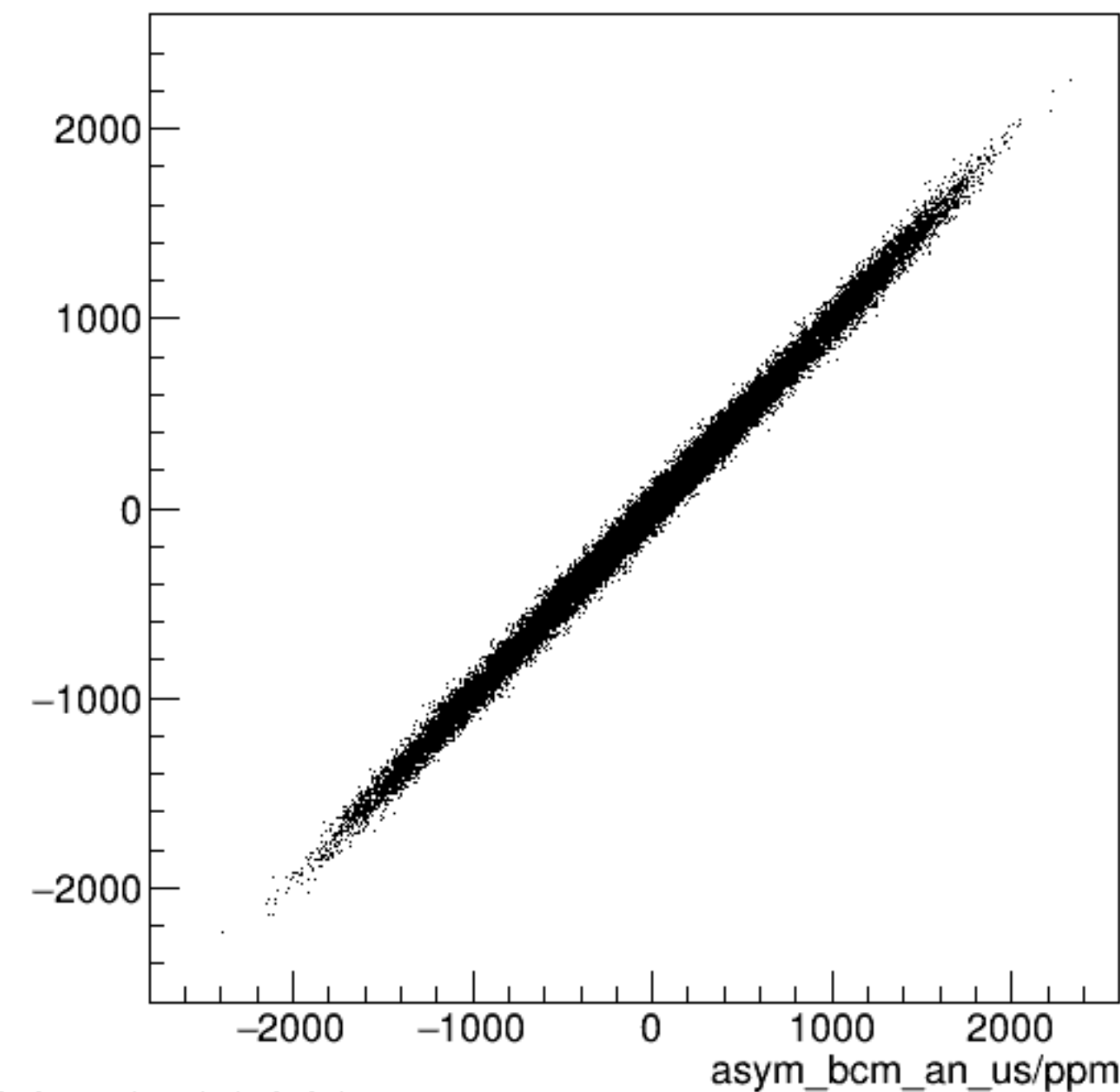
run7967_000_asym_bcm_dg_ds_vs_asym_bcm_an_us_pr.png
