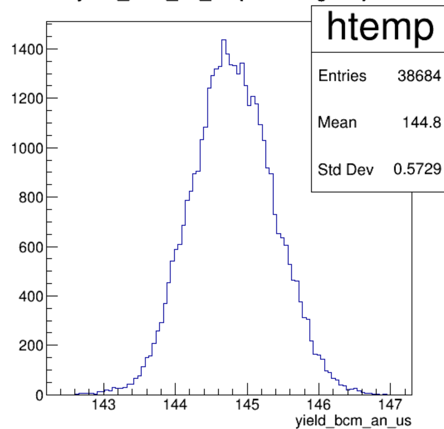
yield_bcm_an_us {ErrorFlag==0}
