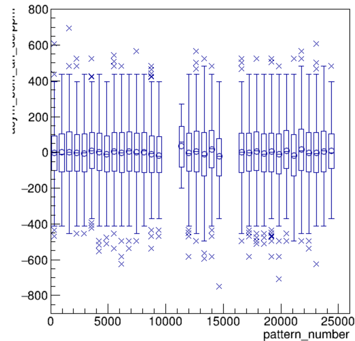
asym_bcm_an_ds/ppm:pattern_number {ErrorFlag==0}
