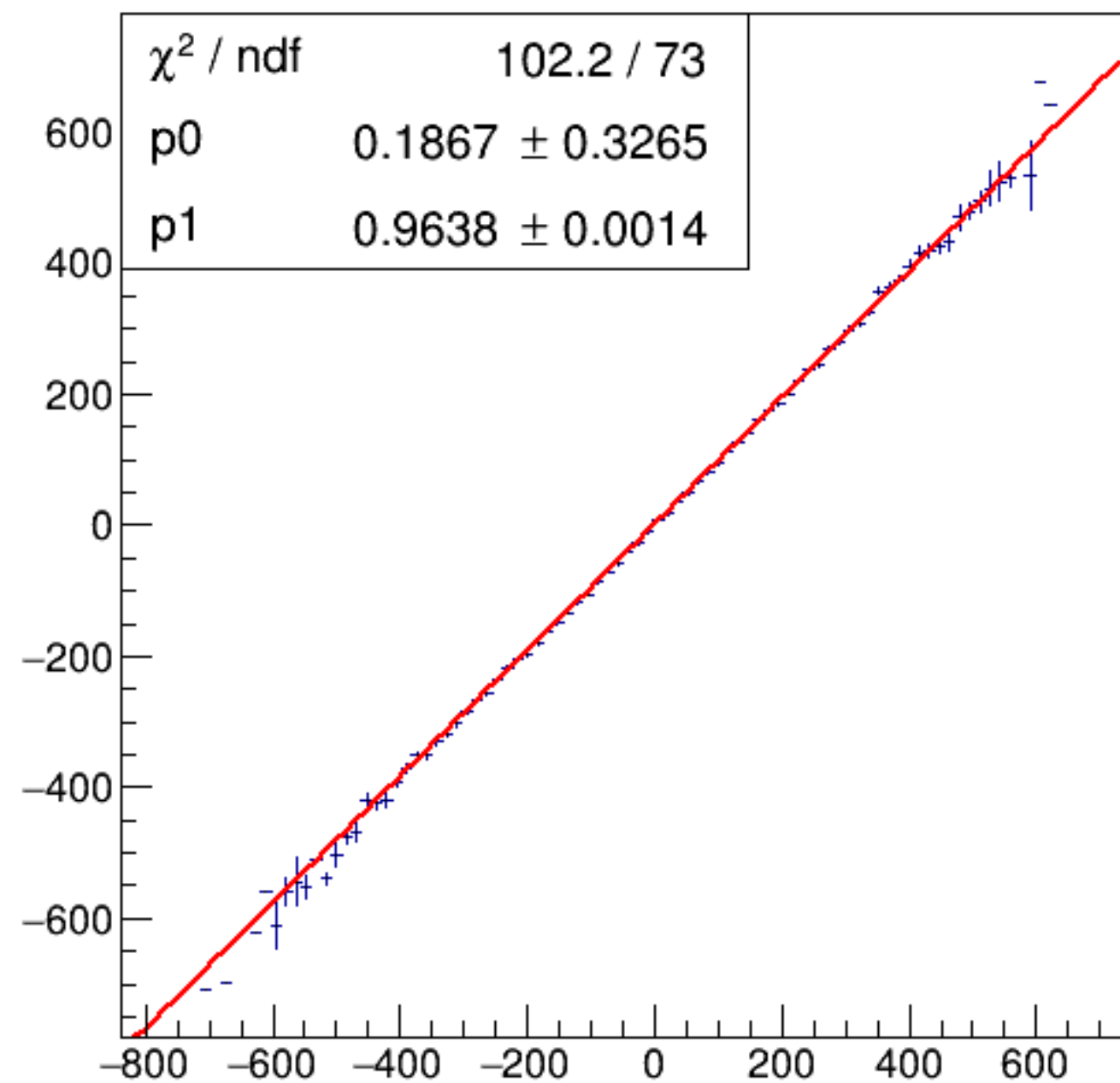
run7967_000_asym_bcm_dg_us_vs_asym_bcm_dg_ds_mul.png
