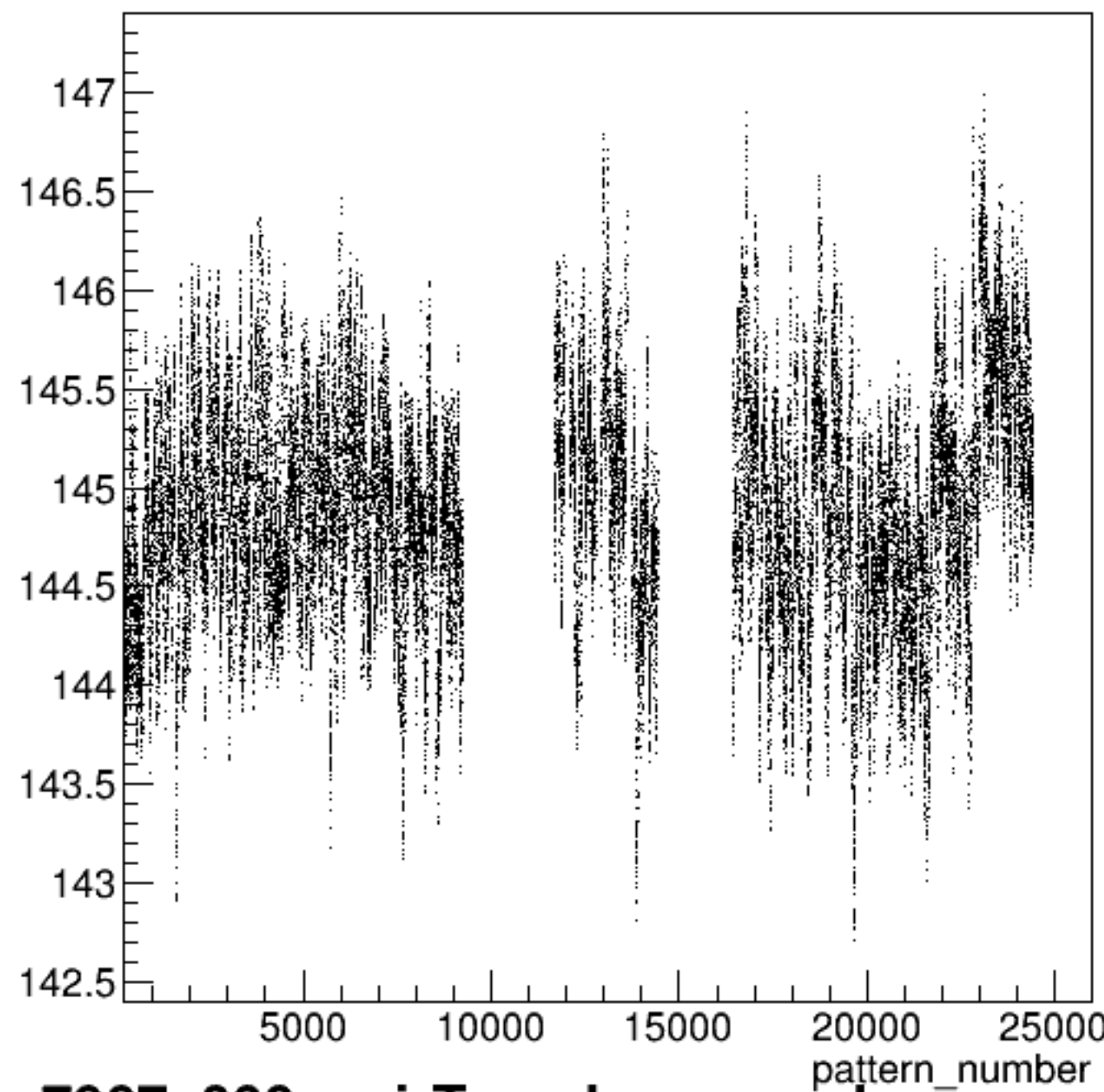
yield_bcm_an_ds:pattern_number {ErrorFlag==0}
