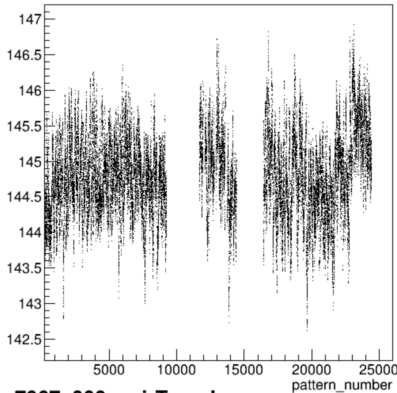
yield_bcm_an_us:pattern_number {ErrorFlag==0}
