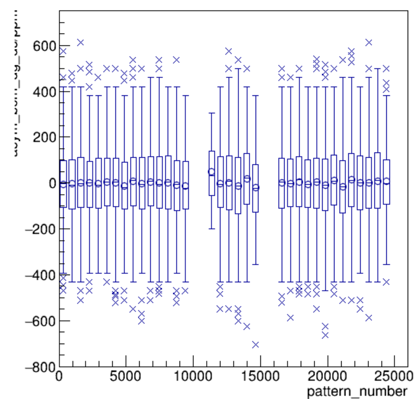
asym_bcm_dg_ds/ppm:pattern_number {ErrorFlag==0}
