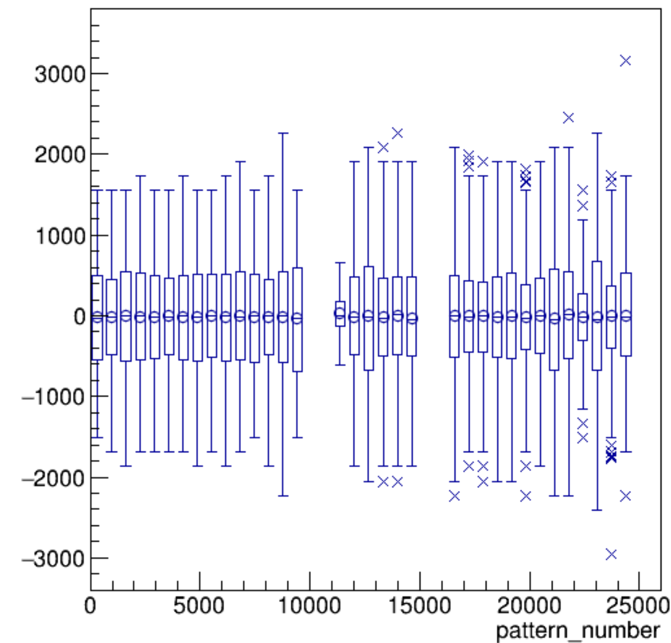
asym_bcm0l02/ppm:pattern_number {ErrorFlag==0}
