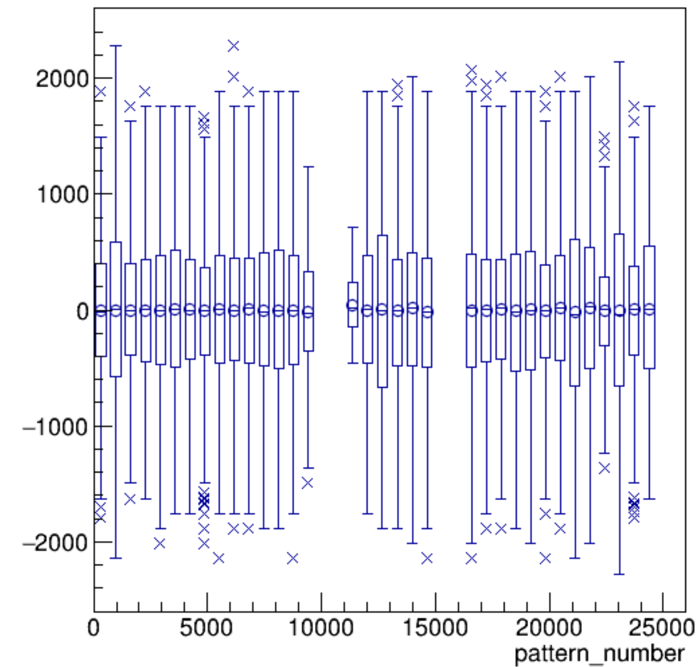
asym_bcm_an_ds3/ppm:pattern_number {ErrorFlag==0}
