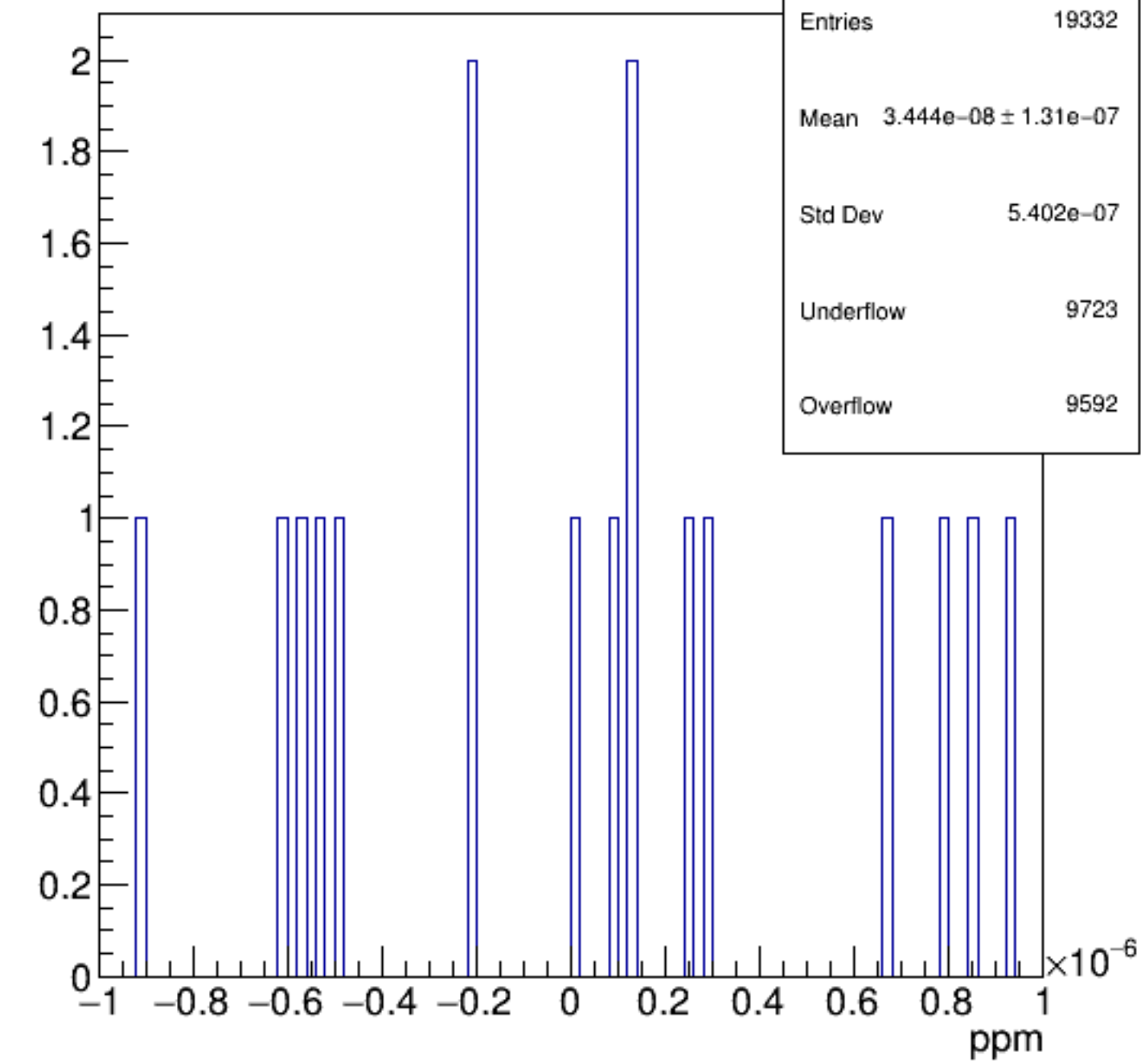
asym_bcm_an_diff
