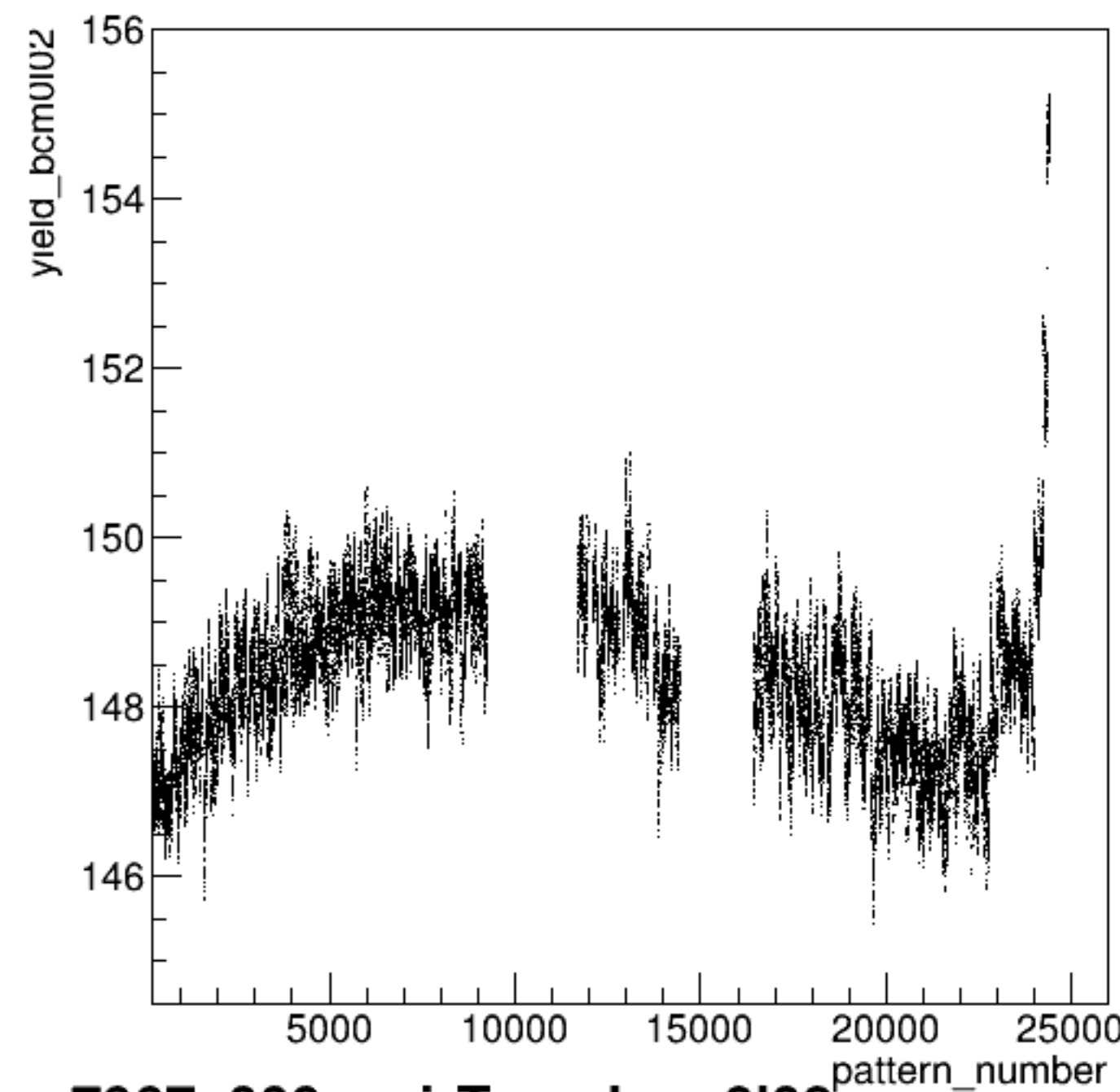
yield_bcm0l02:pattern_number {ErrorFlag==0}
