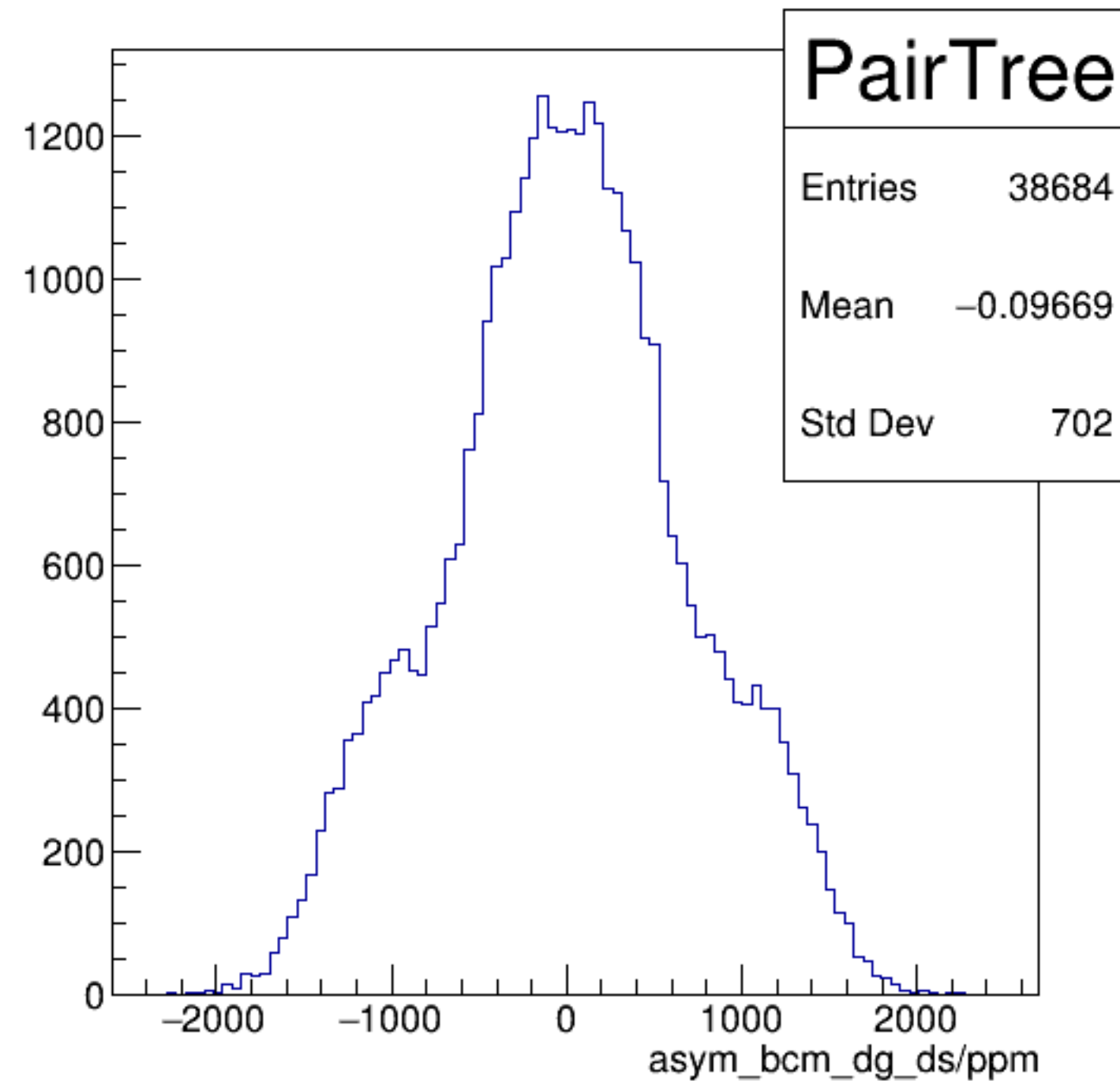
asym_bcm_dg_ds/ppm {ErrorFlag==0}
