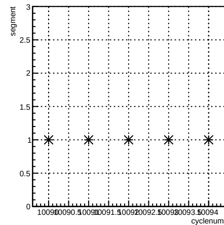
segment:cyclenum {run == 7994}
