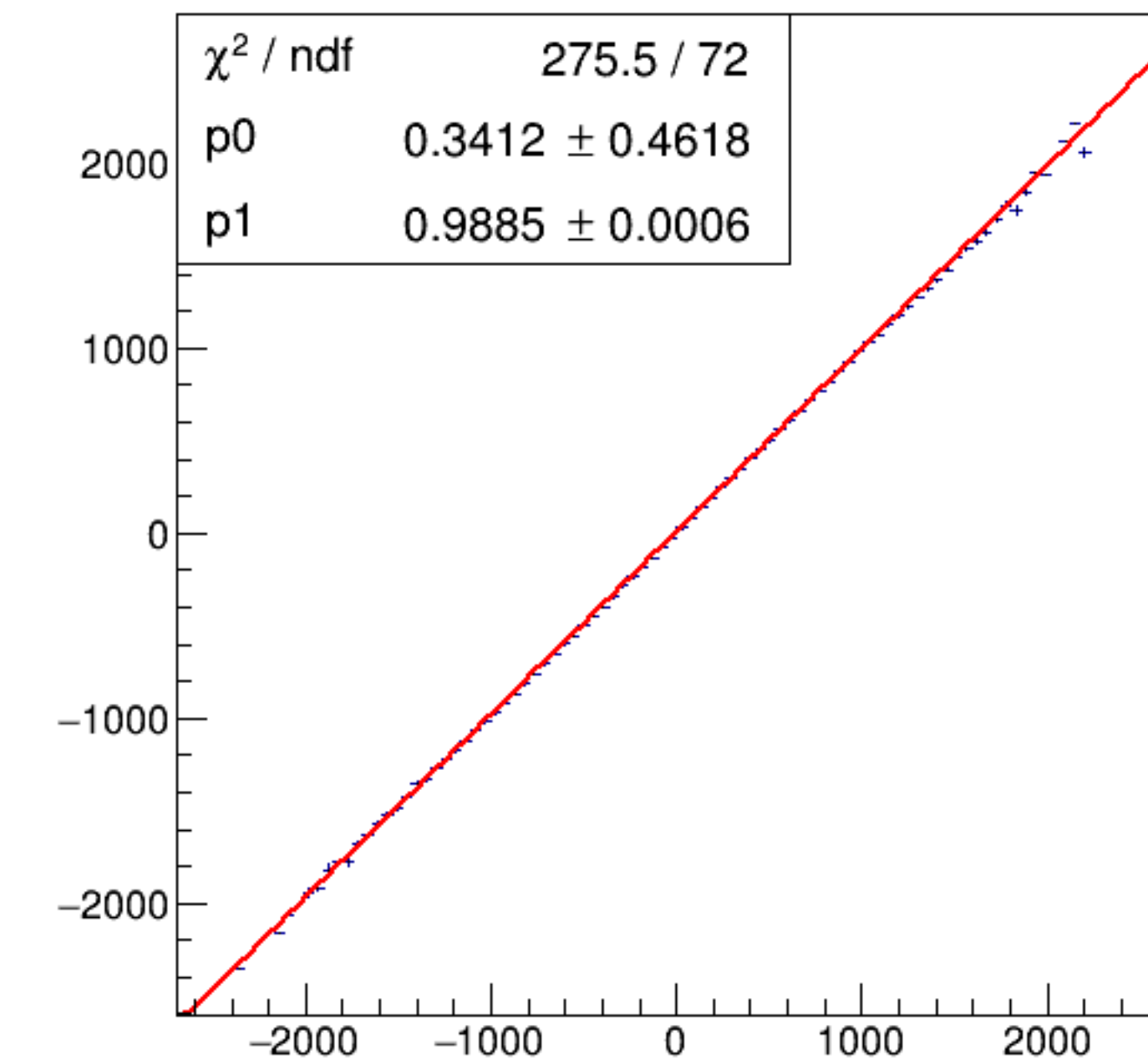
run8001_000_asym_bcm_dg_ds_vs_asym_bcm_an_us_pr.png
