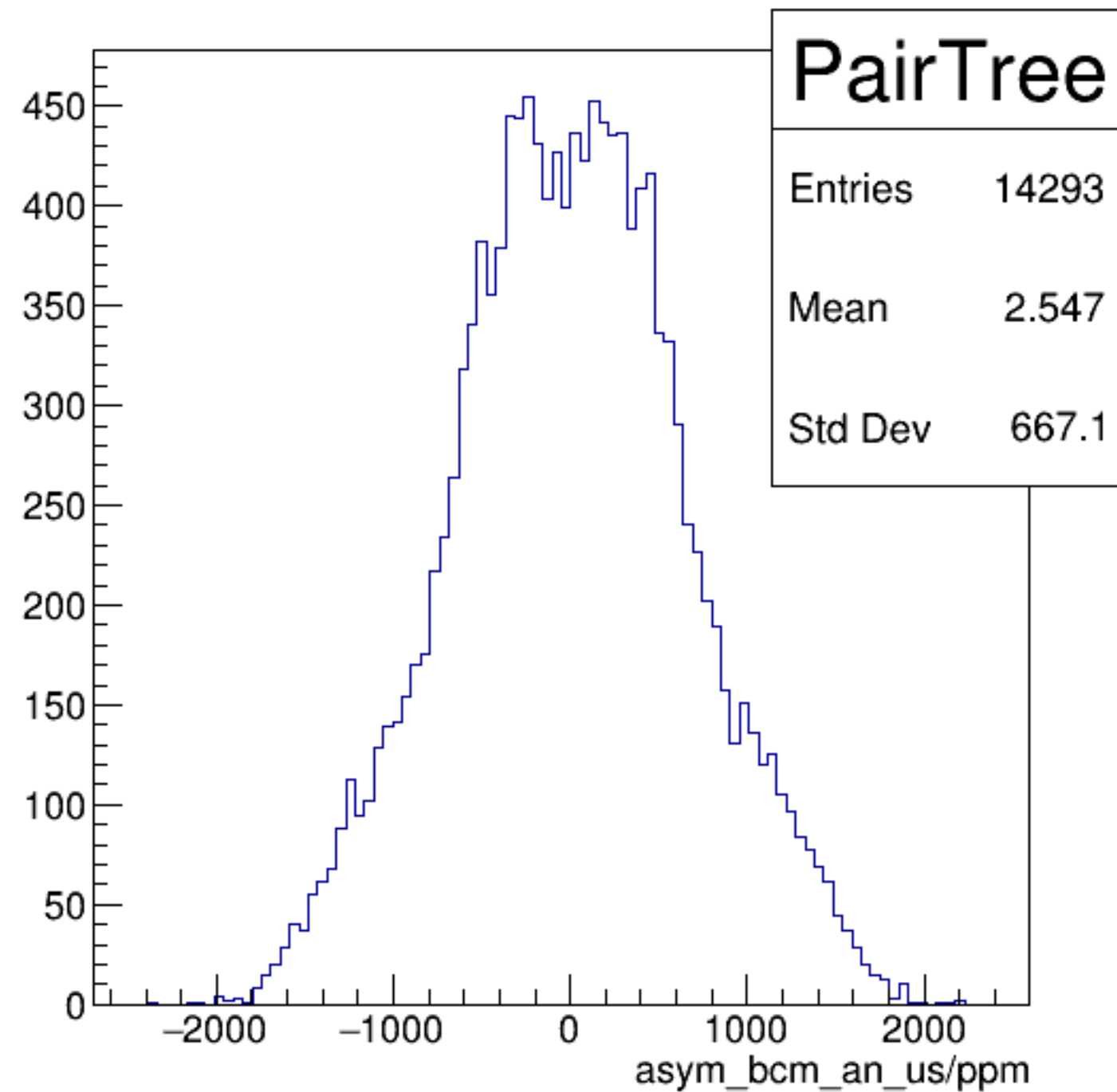
asym_bcm_an_us/ppm {ErrorFlag==0}
