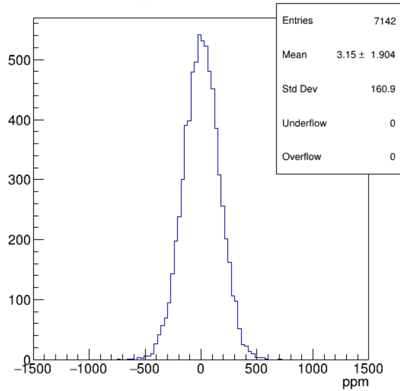
asym_bcm_an_ds
