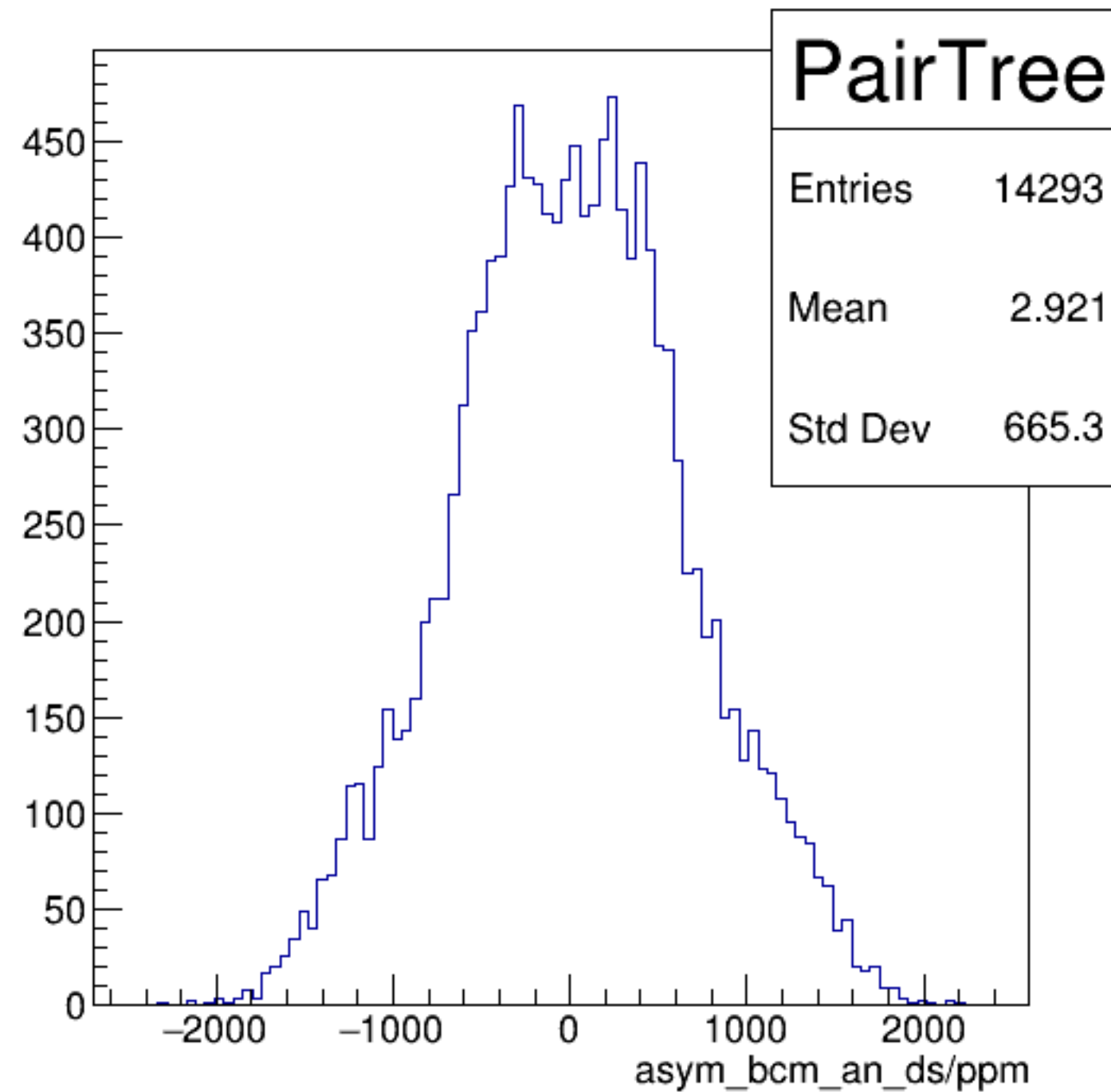
asym_bcm_an_ds/ppm {ErrorFlag==0}
