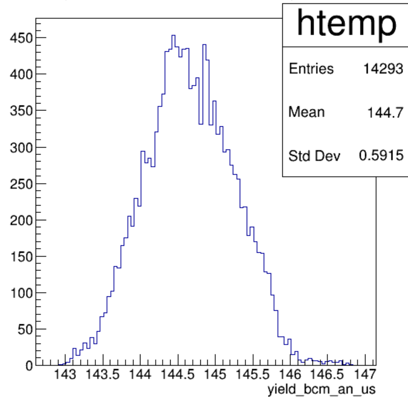
yield_bcm_an_us {ErrorFlag==0}
