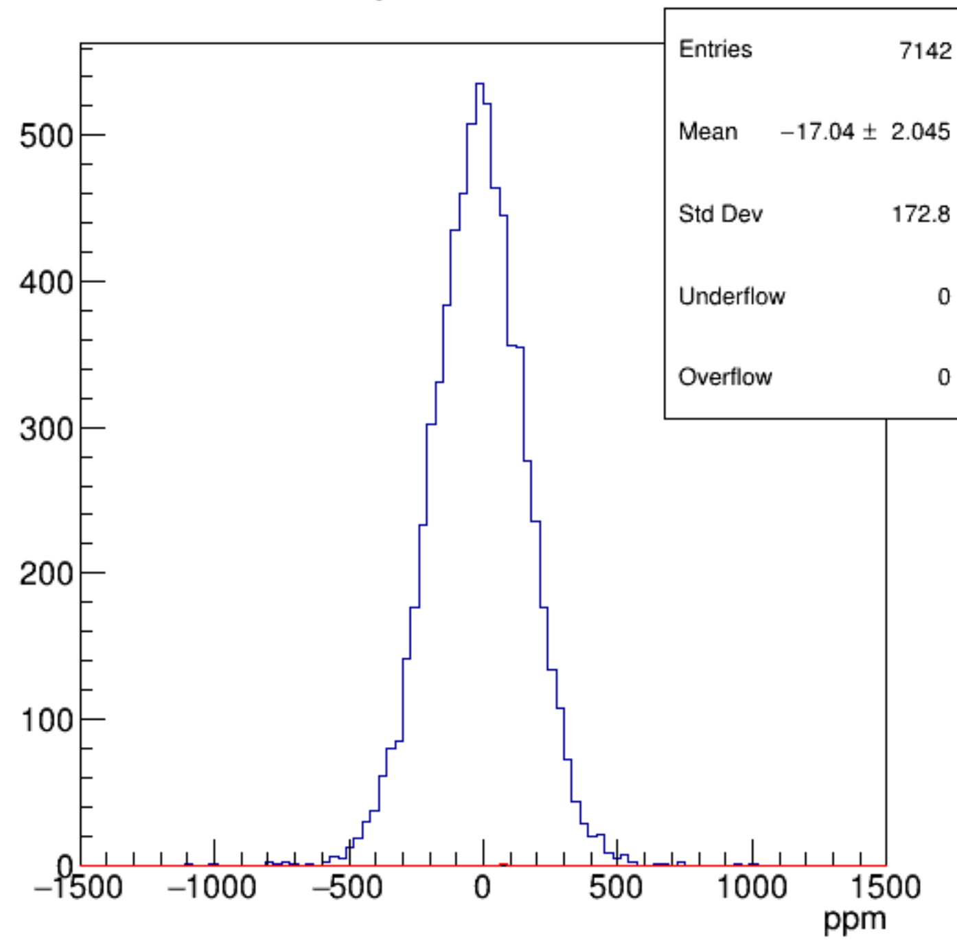
asym_bcm0l02
