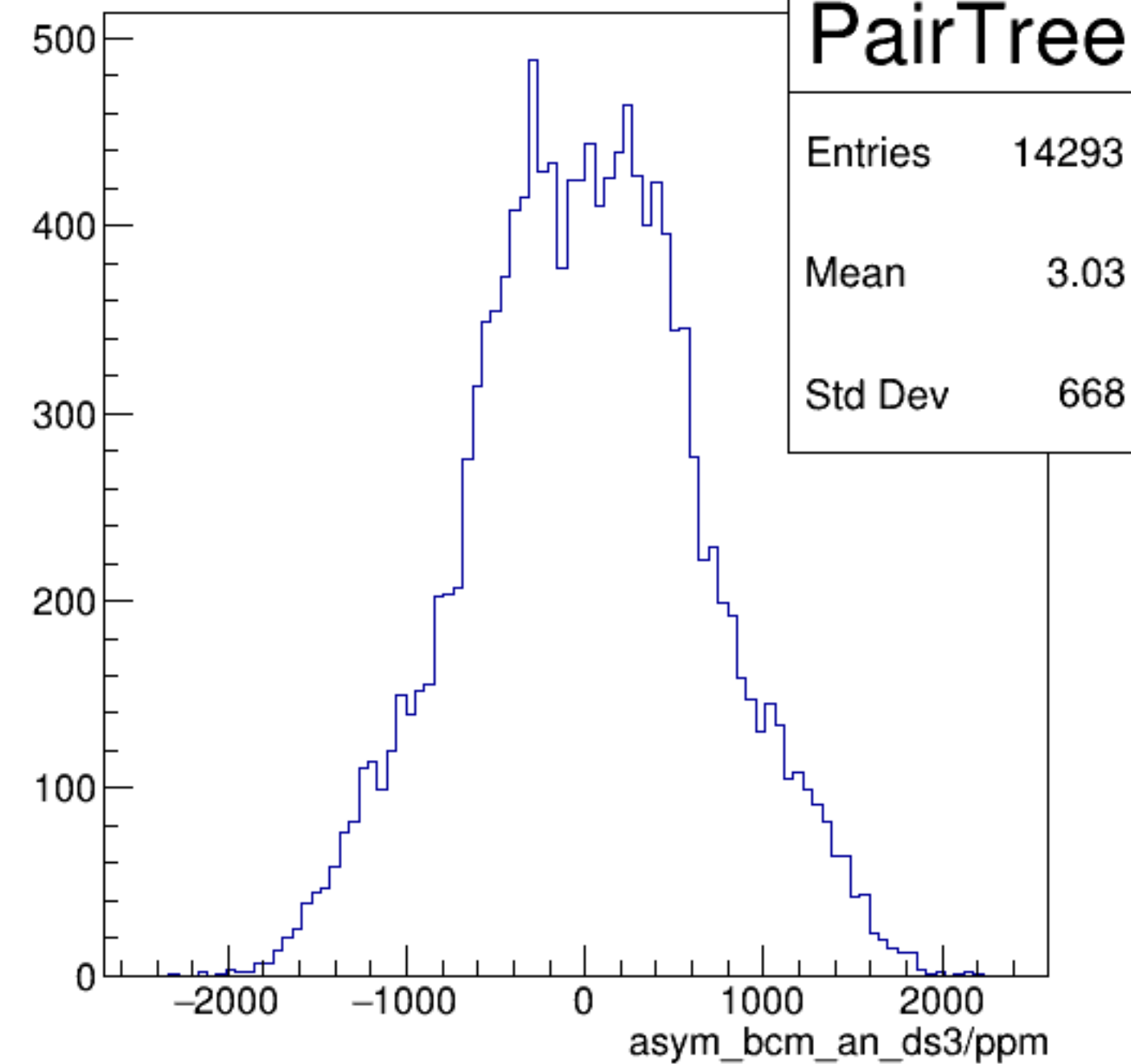
asym_bcm_an_ds3/ppm {ErrorFlag==0}
