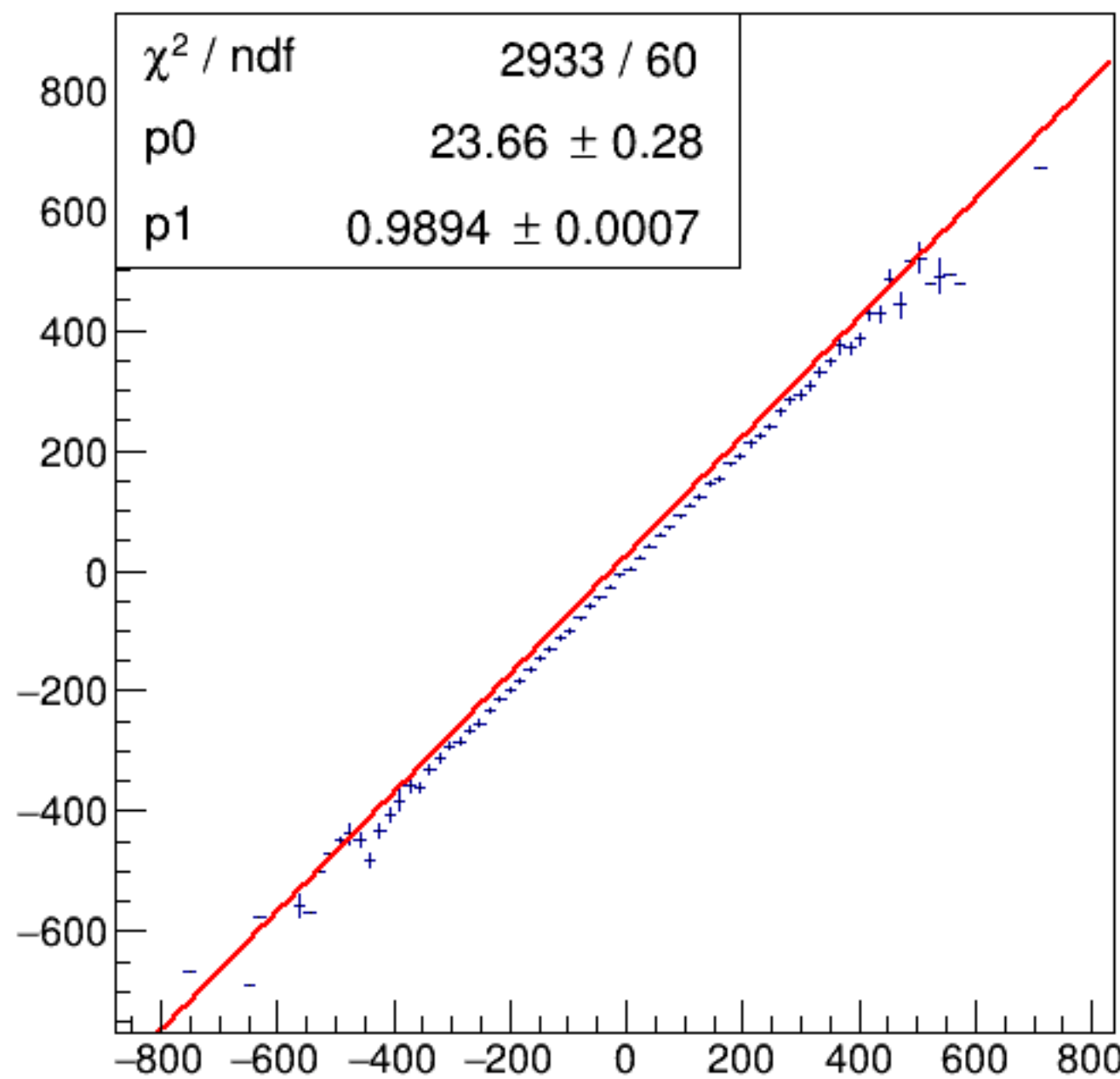
run8001_000_asym_bcm_dg_us_vs_asym_bcm_an_ds_mul.png
