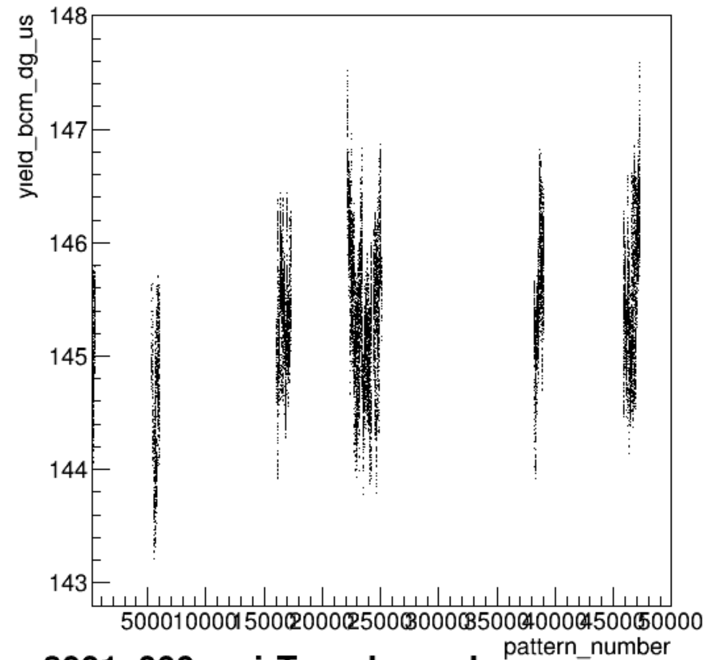
yield_bcm_dg_us:pattern_number {ErrorFlag==0}
