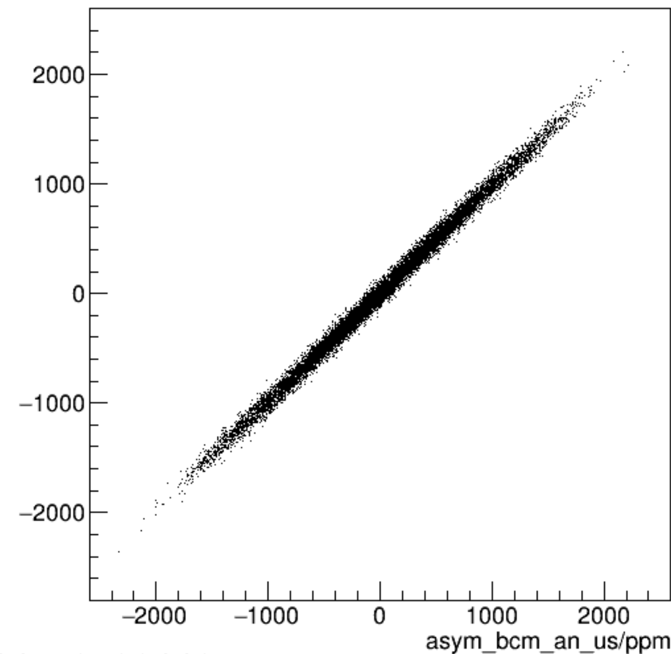
run8001_000_asym_bcm_dg_ds_vs_asym_bcm_an_us_pr.png
