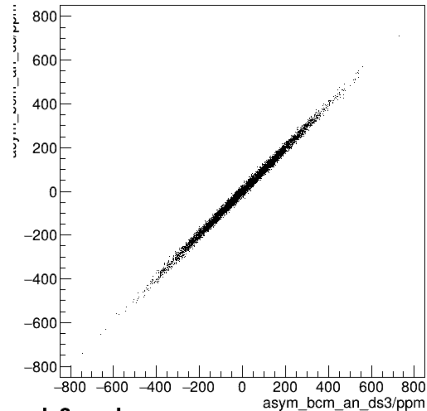
run8001_000_asym_bcm_an_ds_vs_asym_bcm_an_ds3_mul.png
