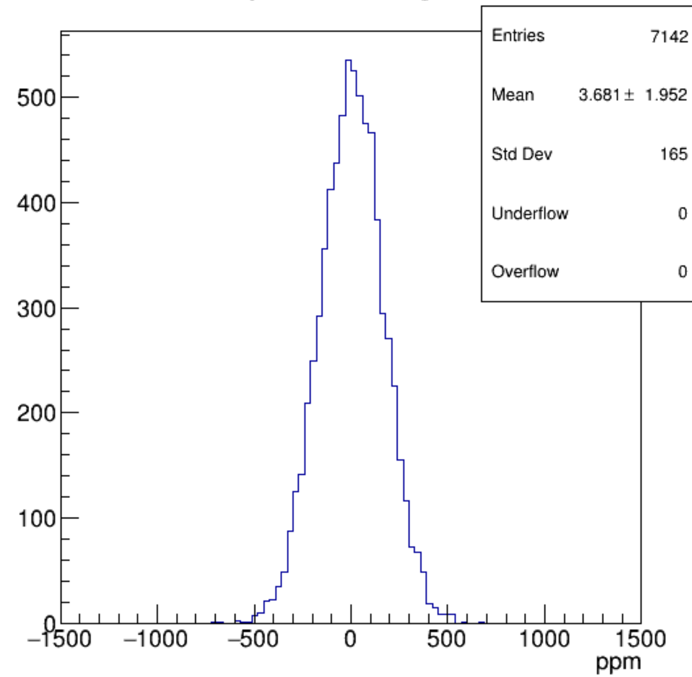
asym_bcm_dg_us
