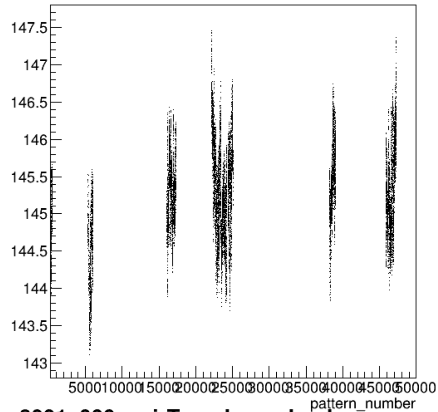
yield_bcm_dg_ds:pattern_number {ErrorFlag==0}
