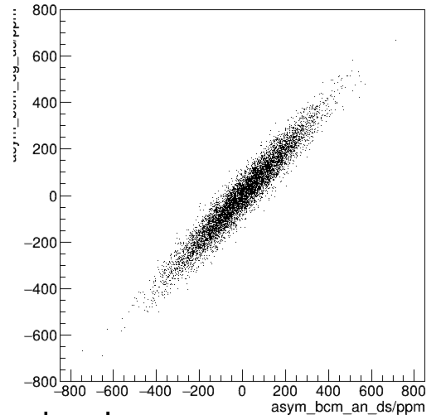
run8001_000_asym_bcm_dg_us_vs_asym_bcm_an_ds_mul.png
