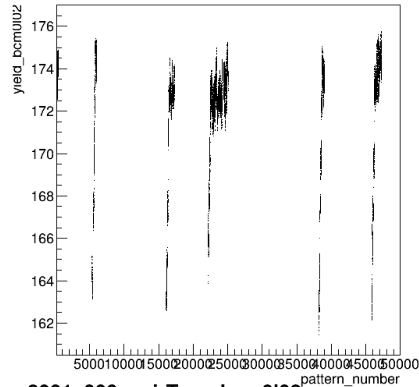
yield_bcm0l02:pattern_number {ErrorFlag==0}
