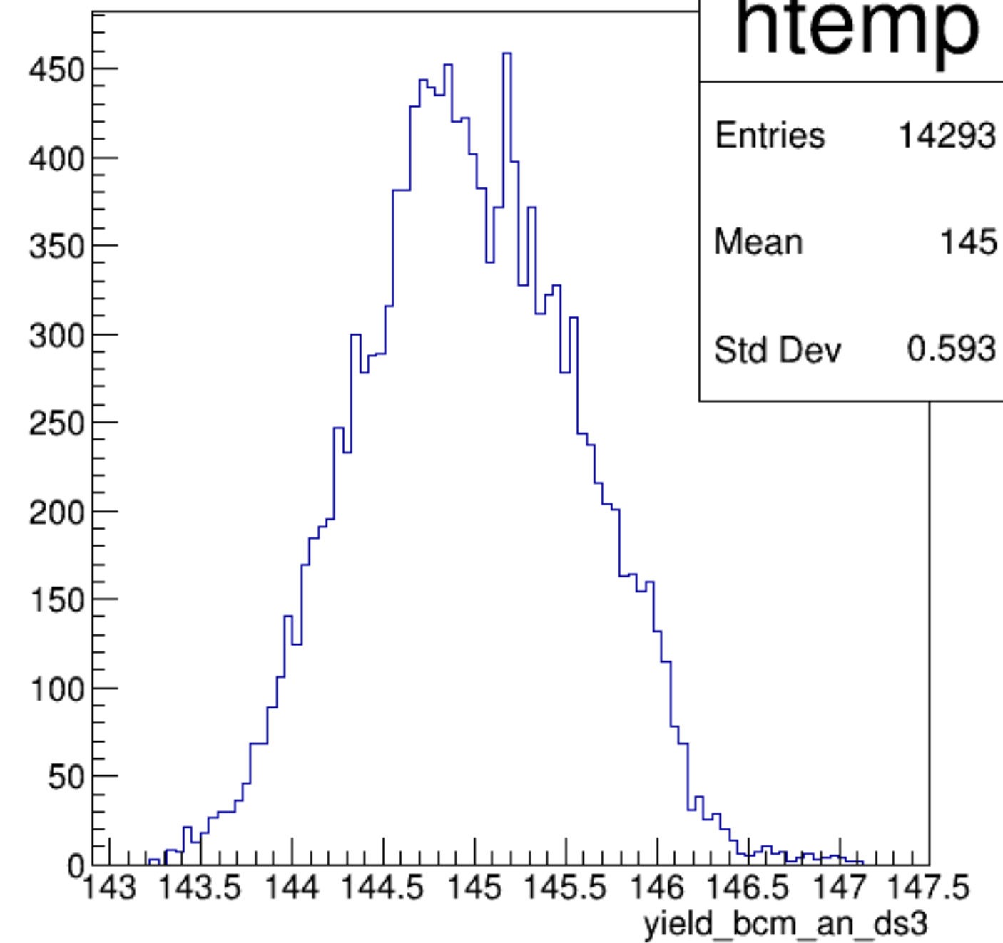
yield_bcm_an_ds3 {ErrorFlag==0}
