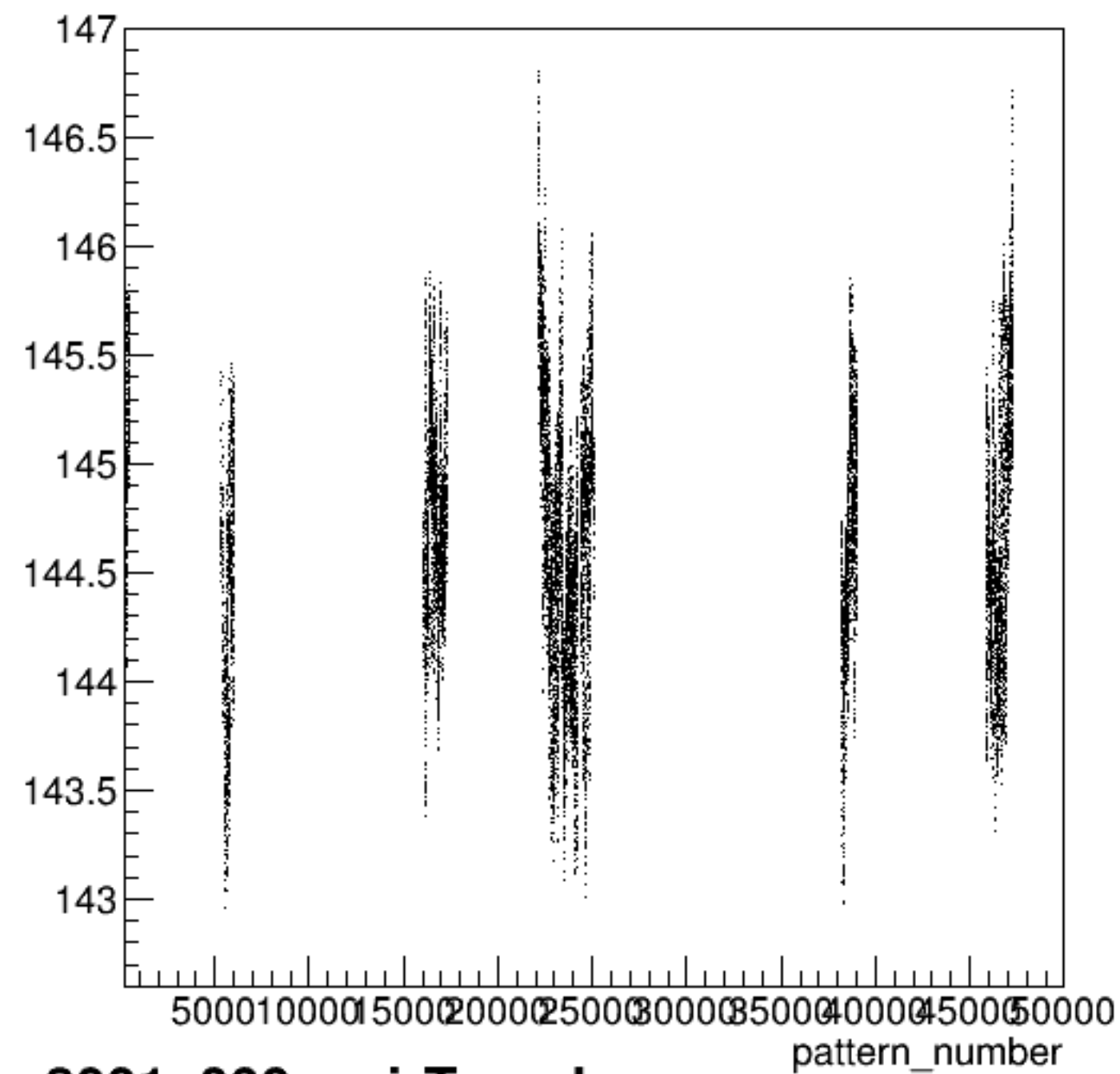
yield_bcm_an_us:pattern_number {ErrorFlag==0}
