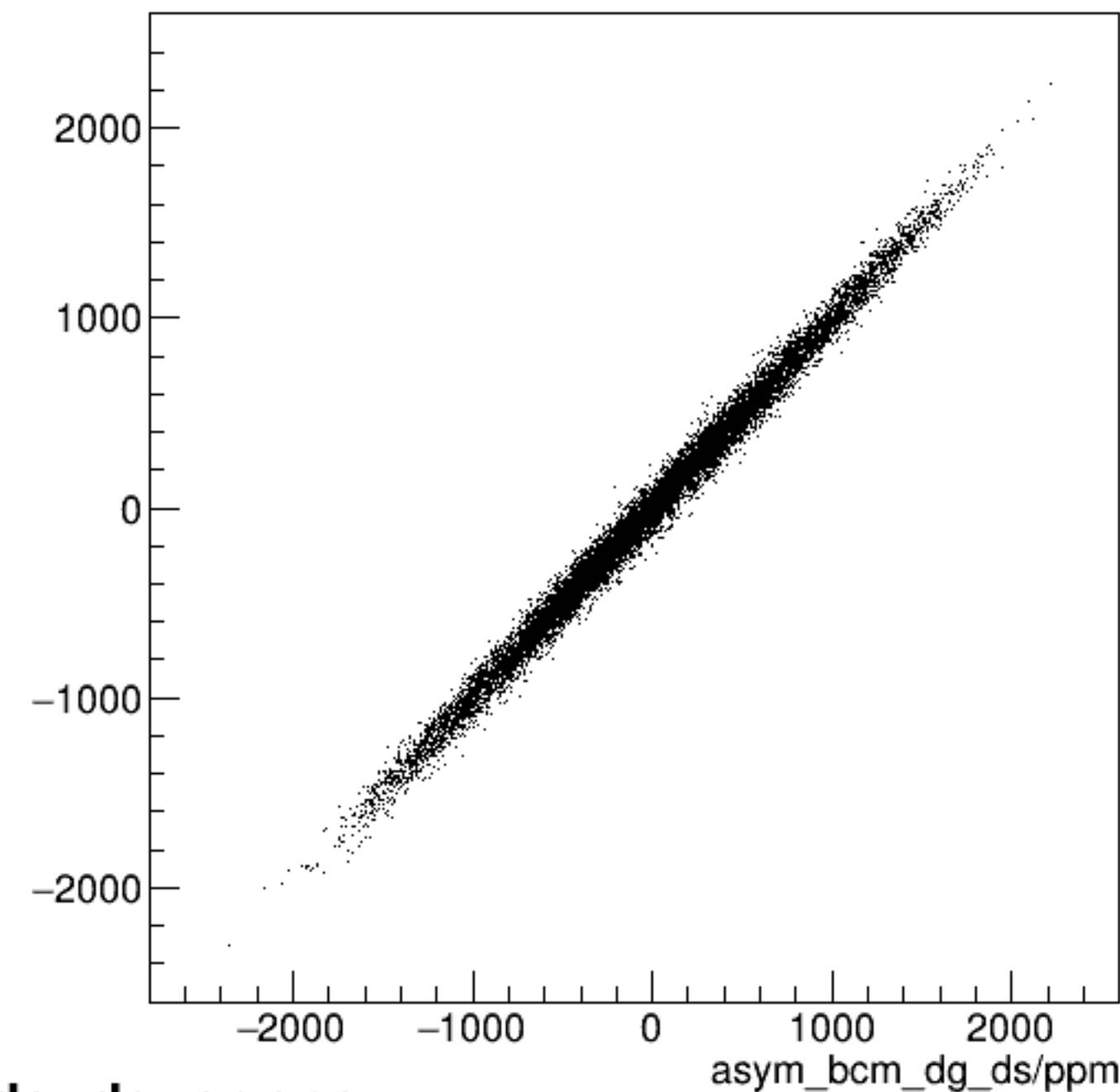
run8001_000_asym_bcm_dg_us_vs_asym_bcm_dg_ds_pr.png
