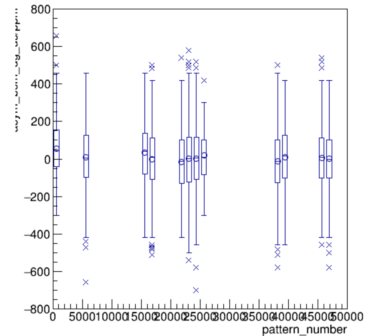
asym_bcm_dg_us/ppm:pattern_number {ErrorFlag==0}
