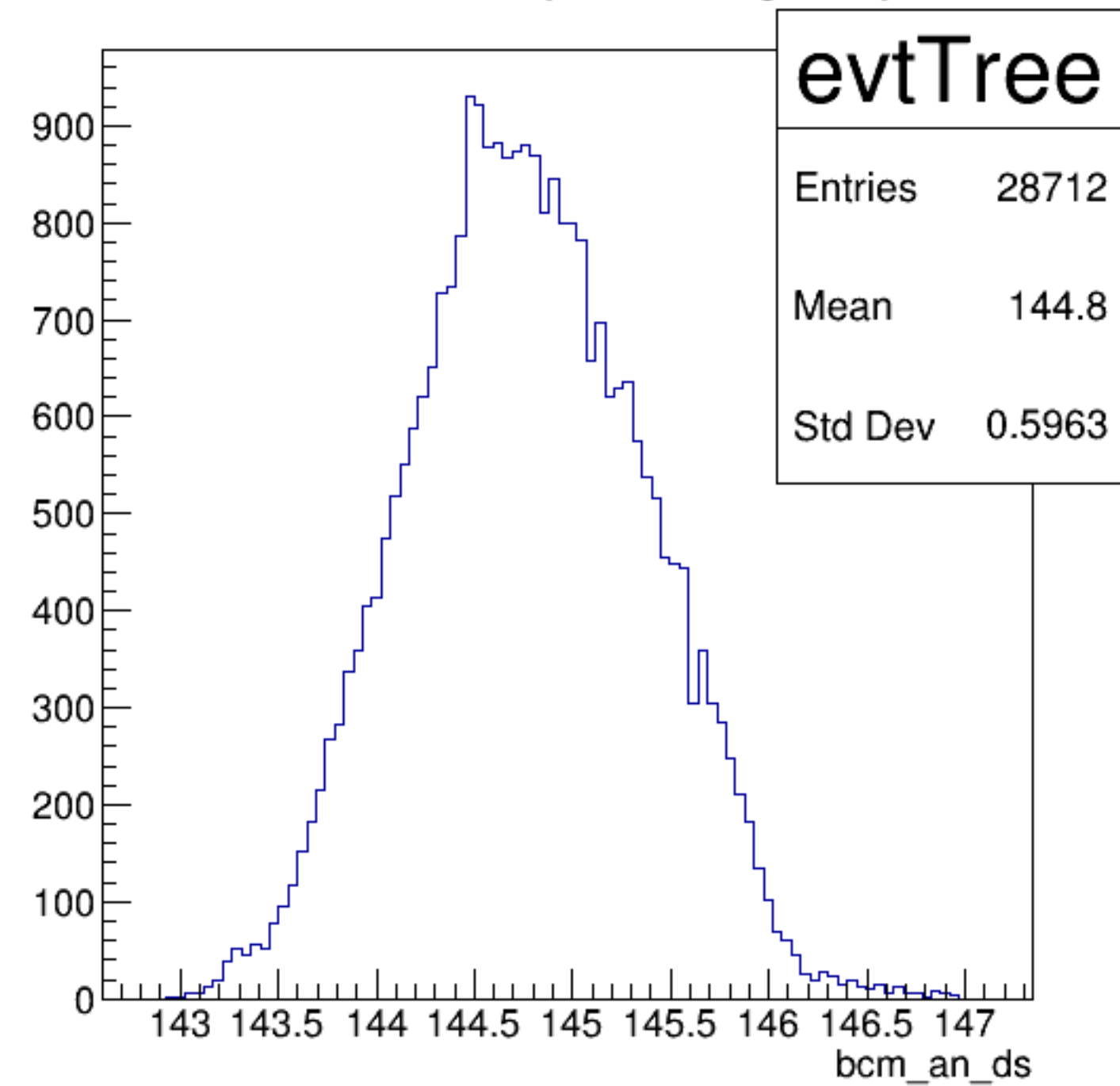
bcm_an_ds {ErrorFlag==0}
