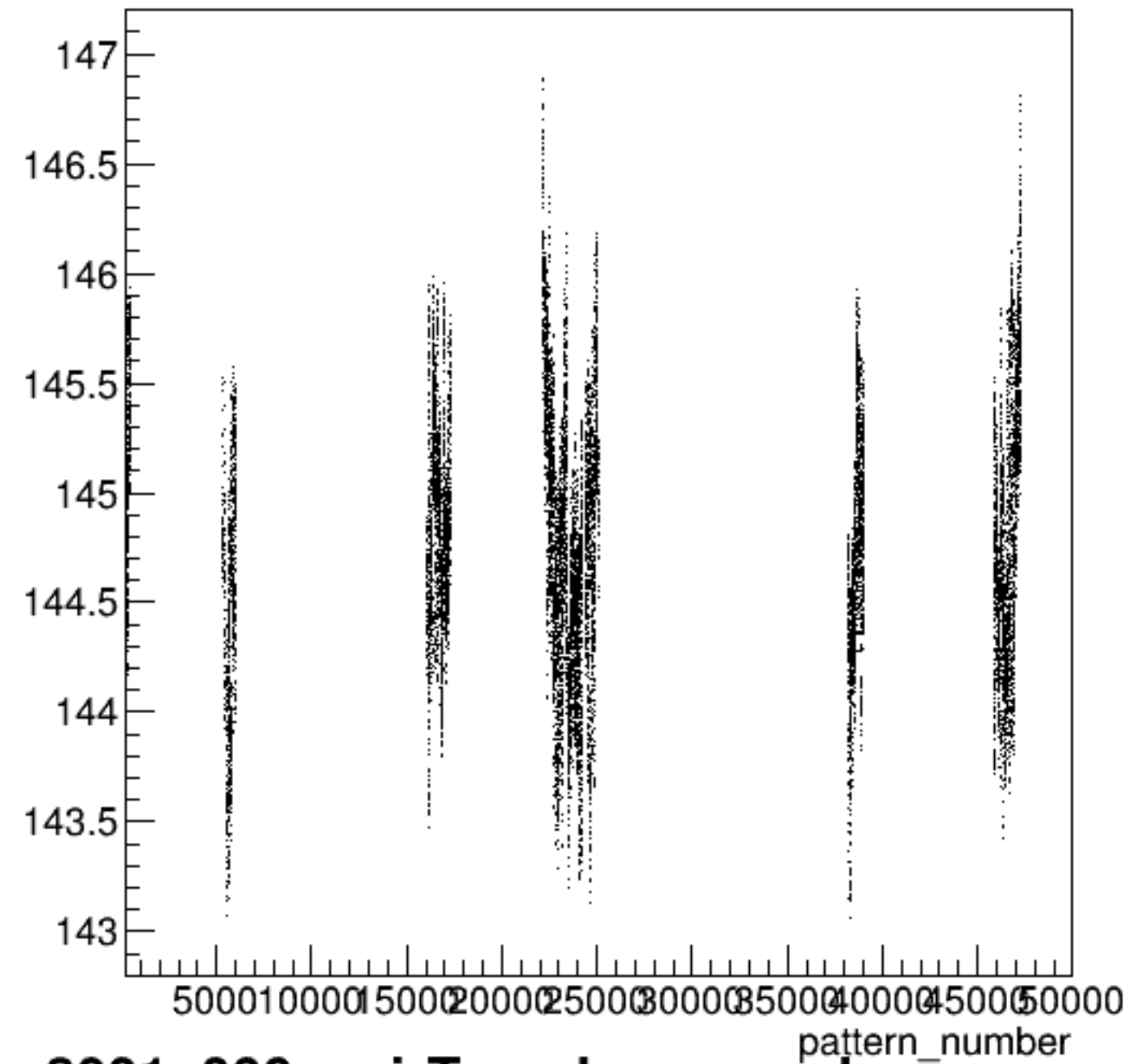
yield_bcm_an_ds:pattern_number {ErrorFlag==0}
