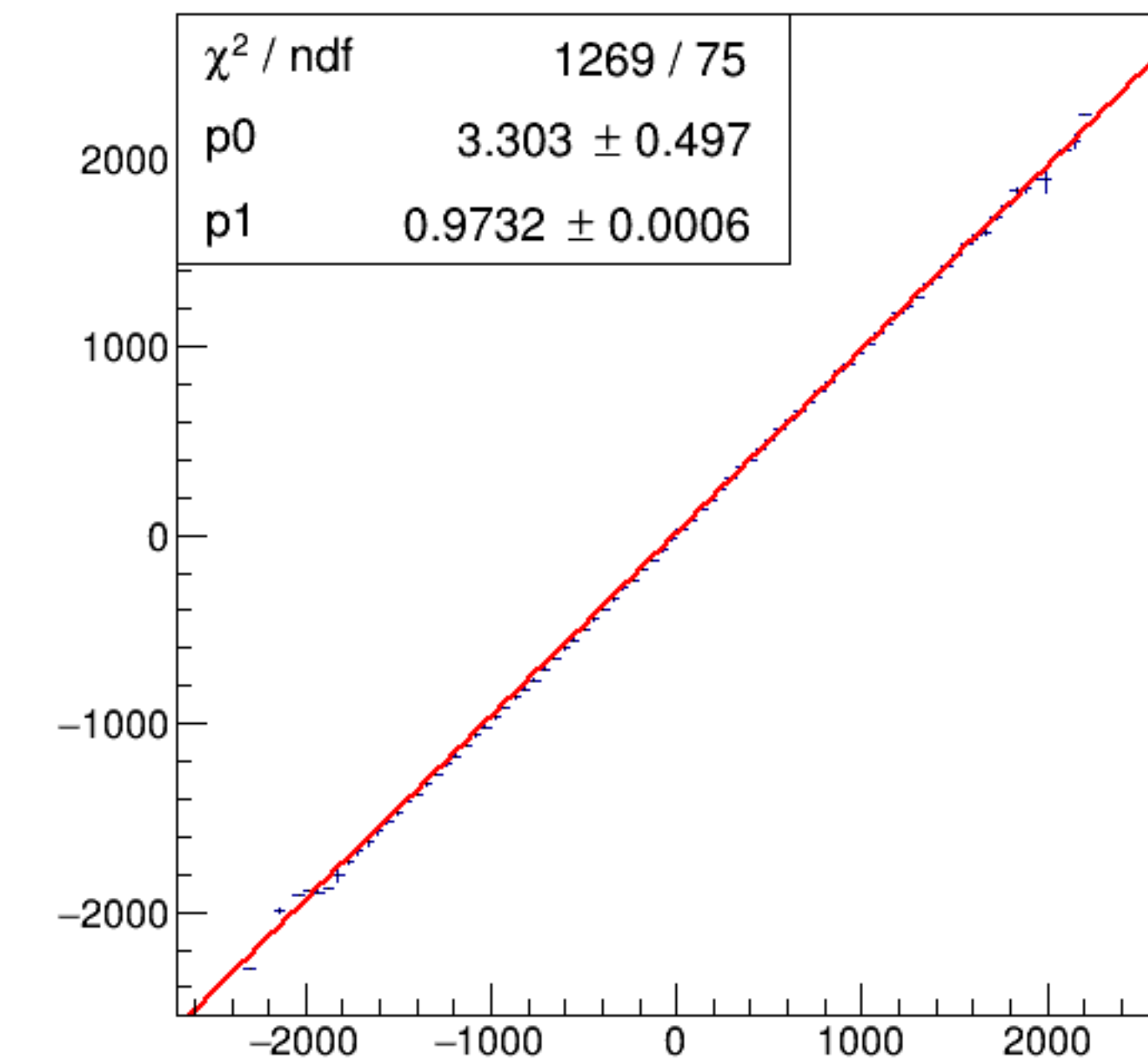
run8001_000_asym_bcm_dg_us_vs_asym_bcm_an_ds3_pr.png
