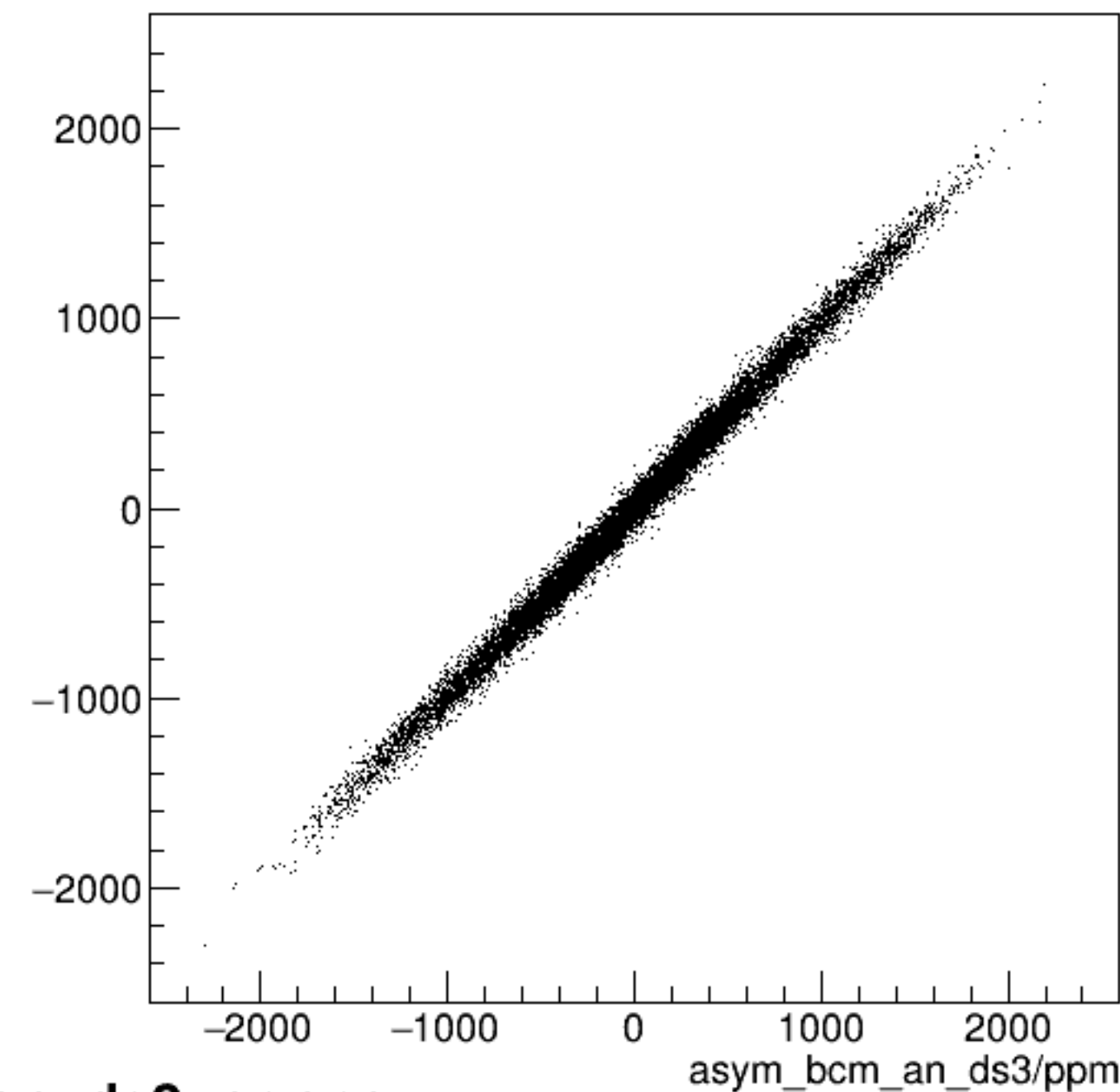
run8001_000_asym_bcm_dg_us_vs_asym_bcm_an_ds3_pr.png
