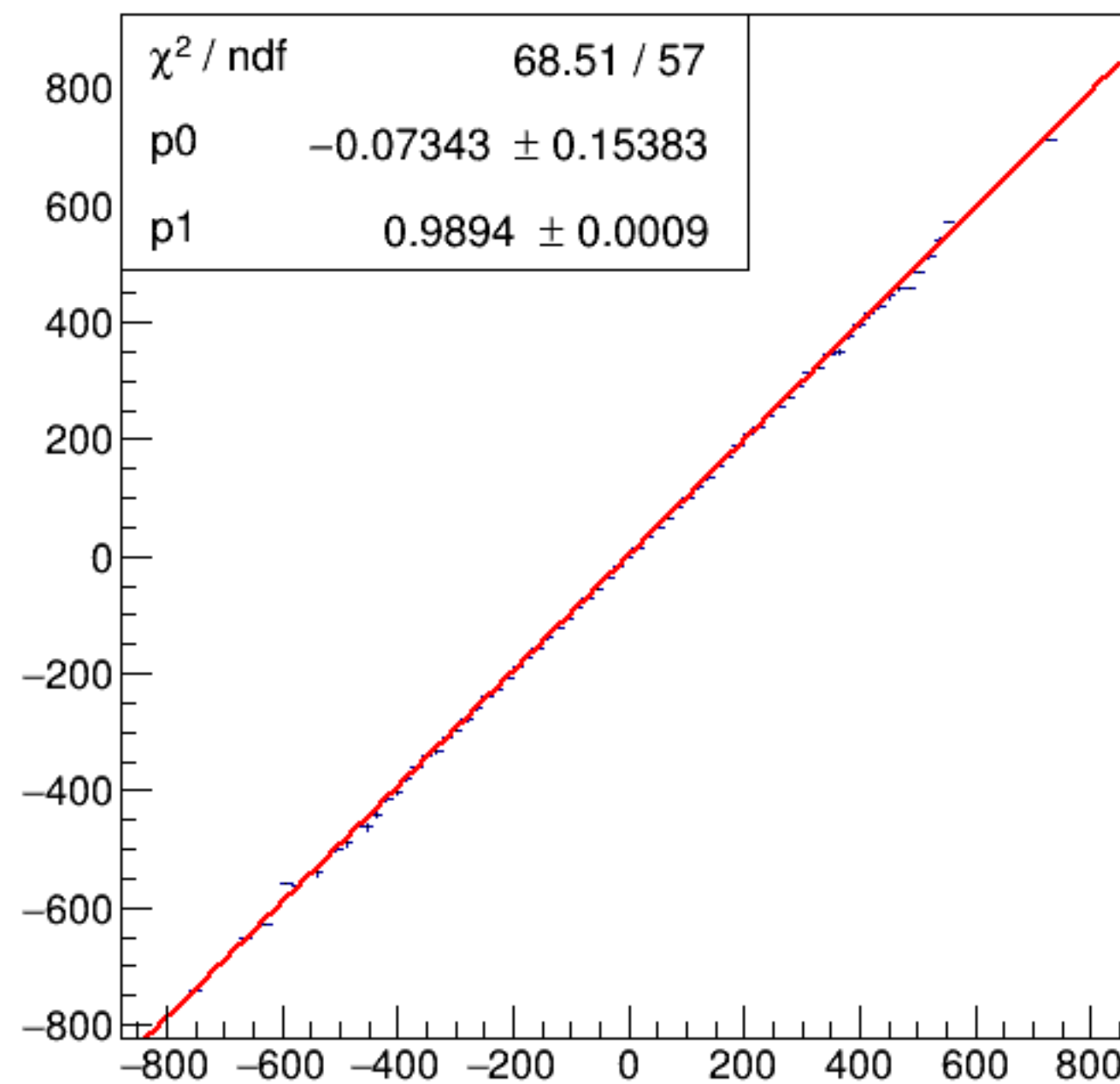
run8001_000_asym_bcm_an_ds_vs_asym_bcm_an_ds3_mul.png
