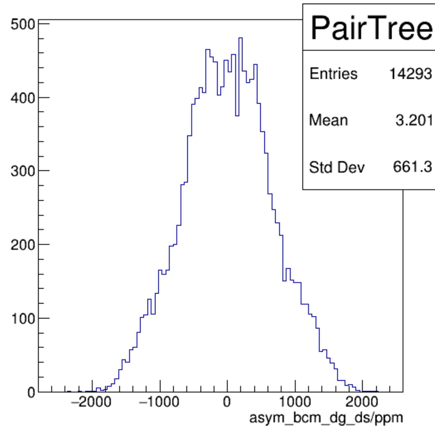
asym_bcm_dg_ds/ppm {ErrorFlag==0}
