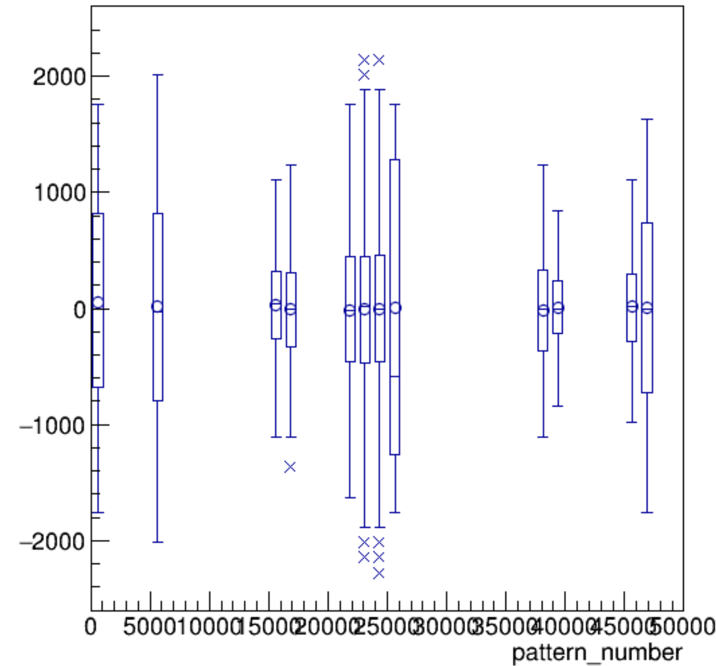
asym_bcm_an_ds/ppm:pattern_number {ErrorFlag==0}
