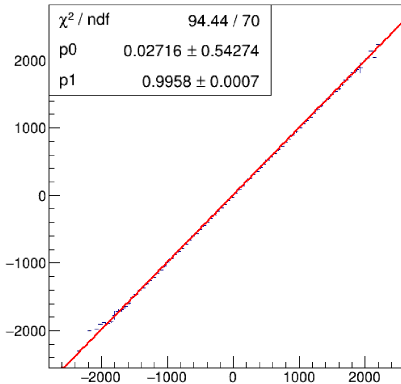
run8001_000_asym_bcm_dg_us_vs_asym_bcm_dg_ds_pr.png
