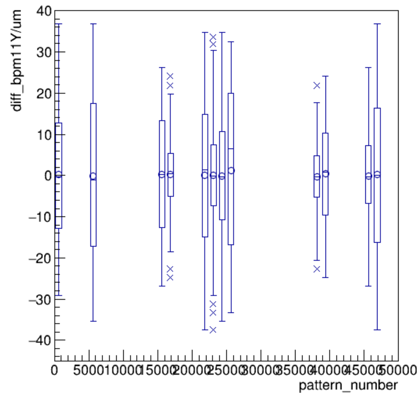
diff_bpm11Y/um:pattern_number {ErrorFlag==0}
