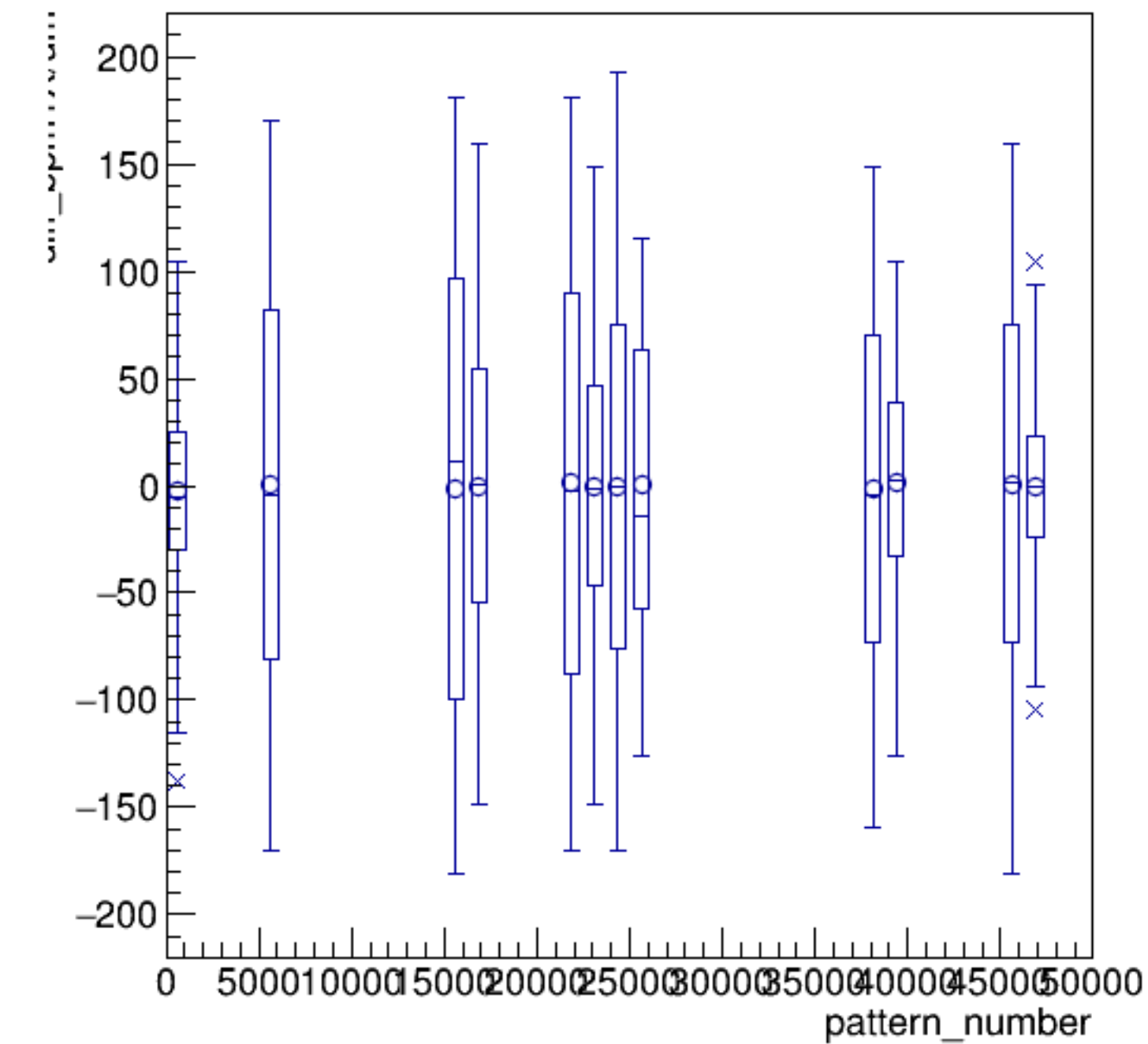
diff_bpm1X/um:pattern_number {ErrorFlag==0}
