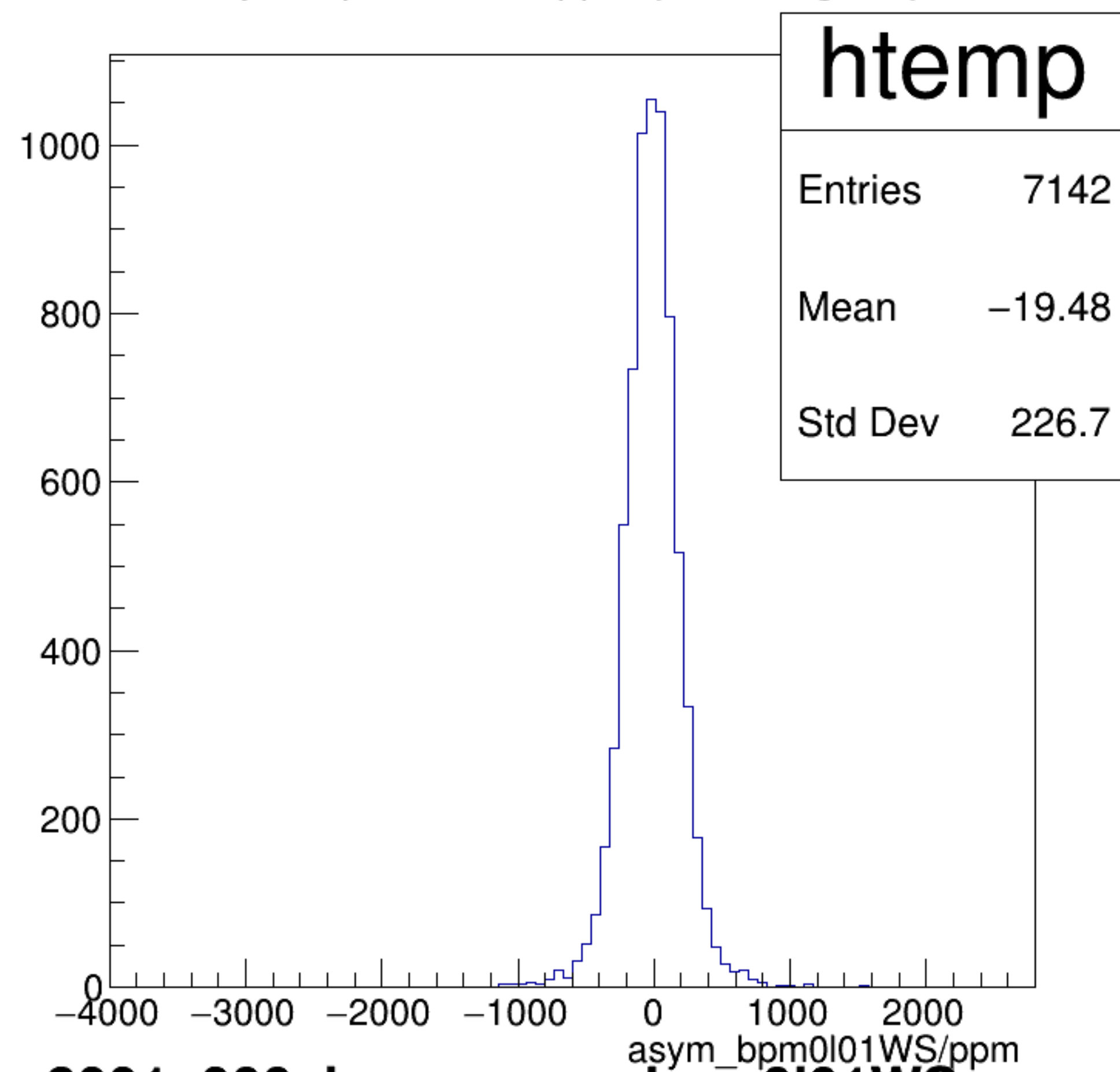
asym_bpm0l01WS/ppm {ErrorFlag==0}
