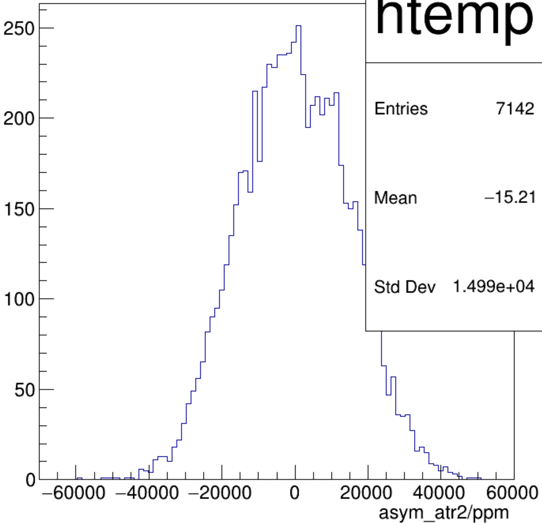
asym_atr2/ppm {ok_cut}
