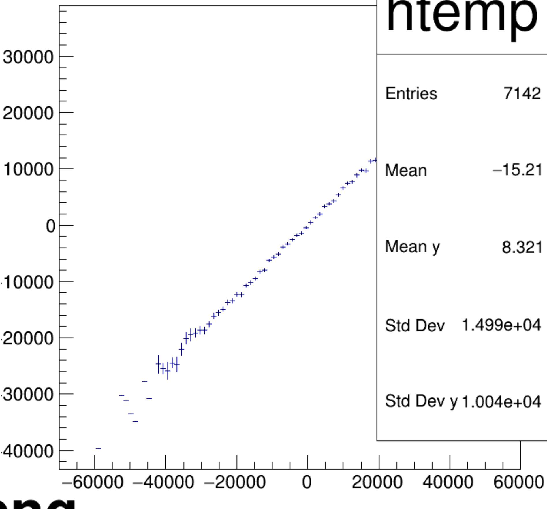
asym_atl2/ppm:asym_atr2/ppm {ok_cut}
