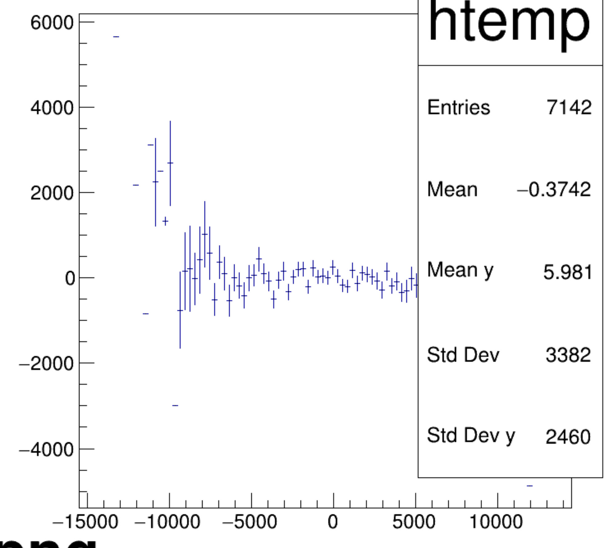
asym_atl1/ppm:asym_atr1/ppm {ok_cut}
