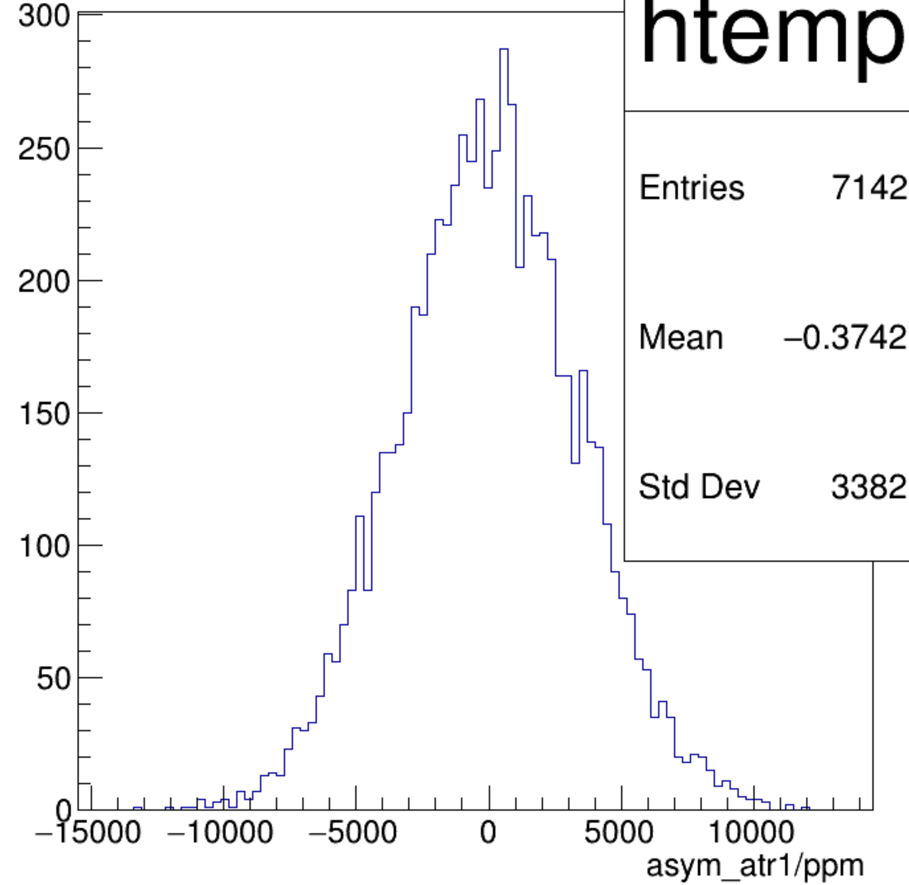
asym_atr1/ppm {ok_cut}
