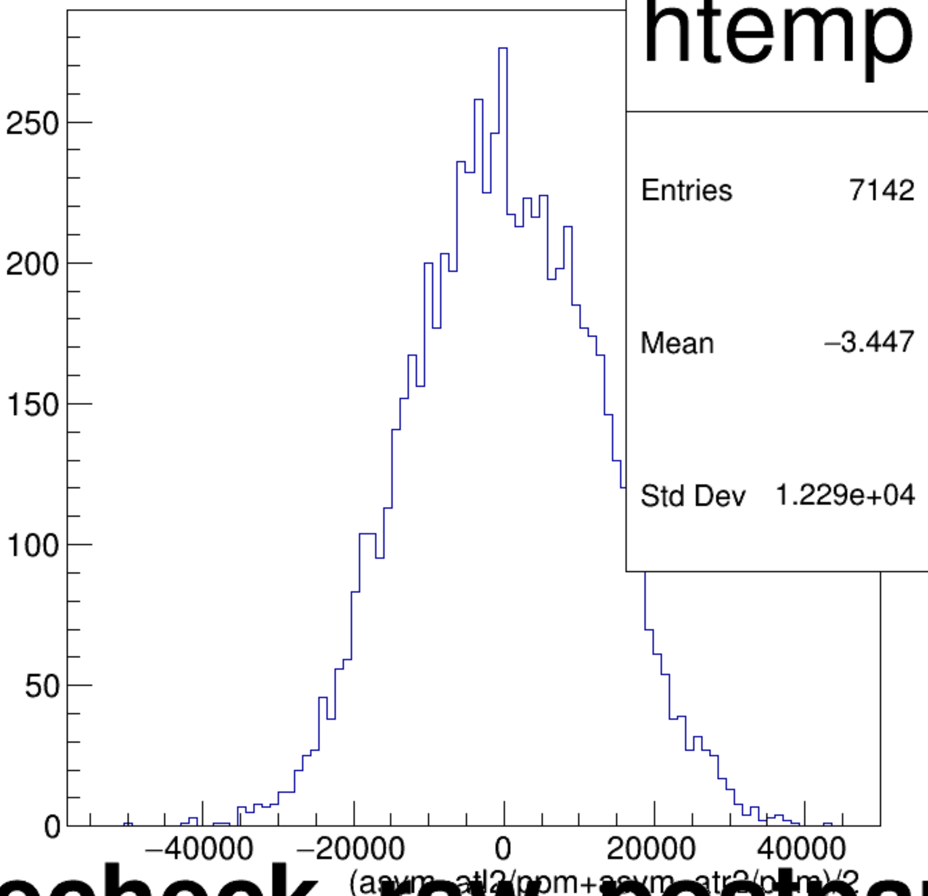
(asym_atl2/ppm+asym_atr2/ppm)/2 {ok_cut}
