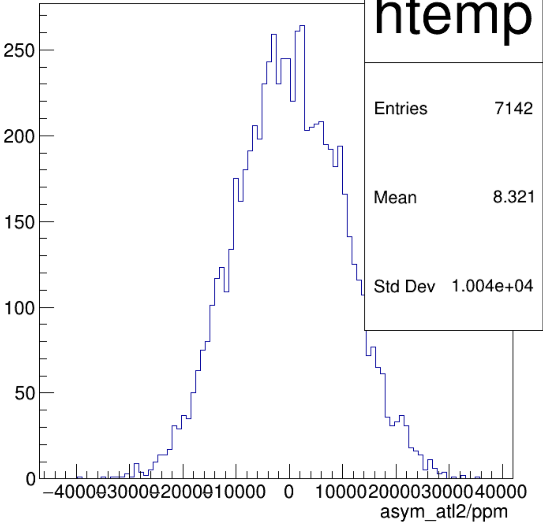
asym_atl2/ppm {ok_cut}
