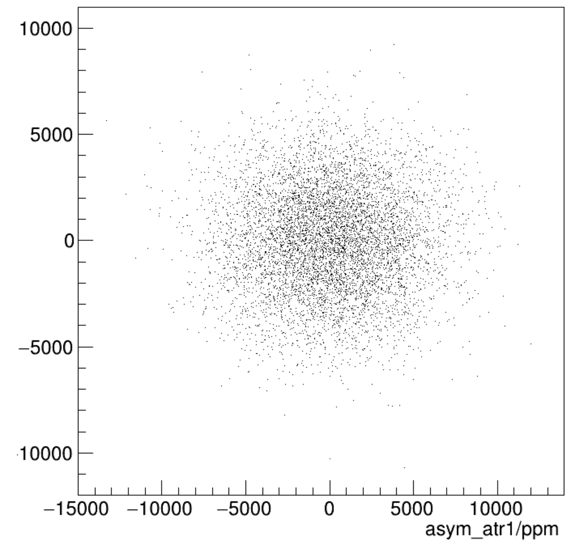
asym_atl1/ppm:asym_atr1/ppm {ok_cut}
