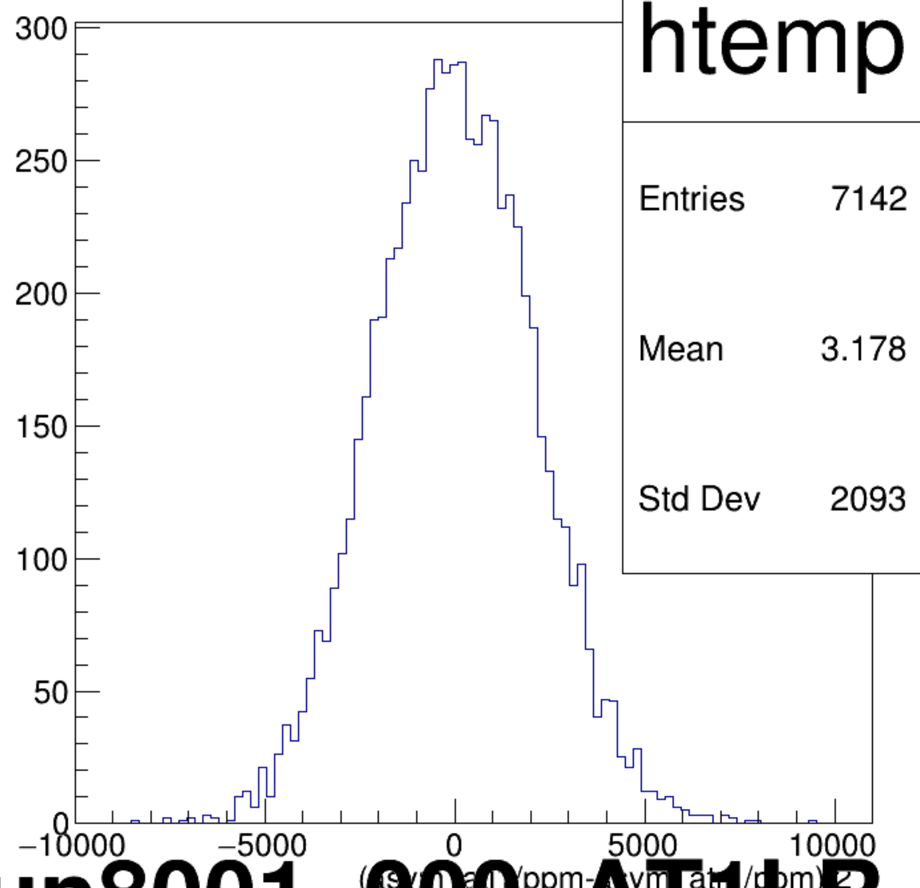
(asym_atl1/ppm-asym_atr1/ppm)/2 {ok_cut}
