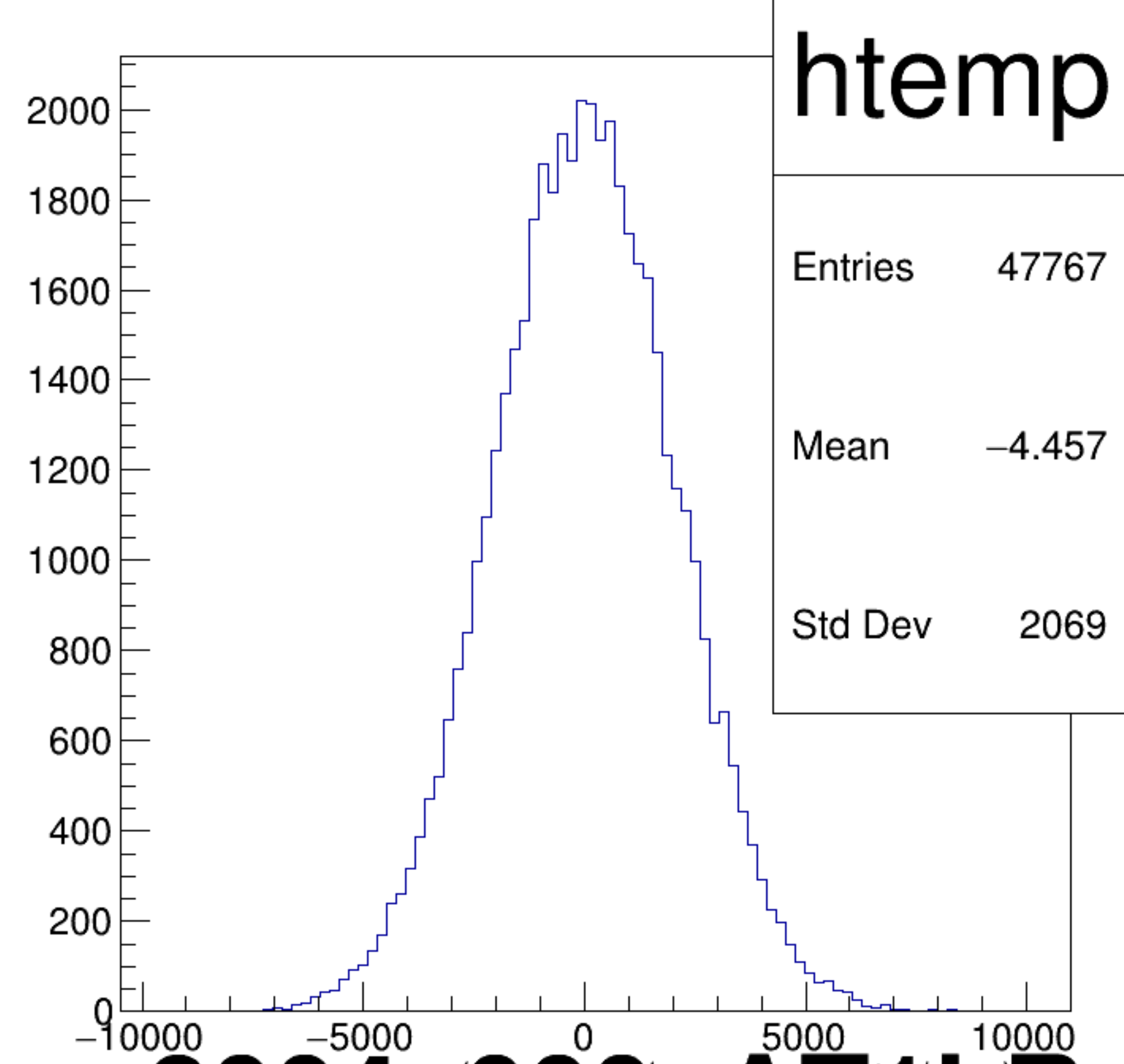
(asym_atl1/ppm-asym_atr1/ppm)/2 {ok_cut}
