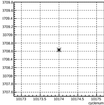
usr_coil7:cyclenum {run == 8020}
