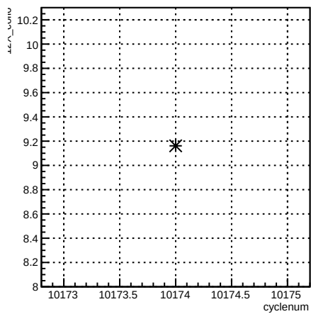
12X_coil6:cyclenum {run == 8020}
