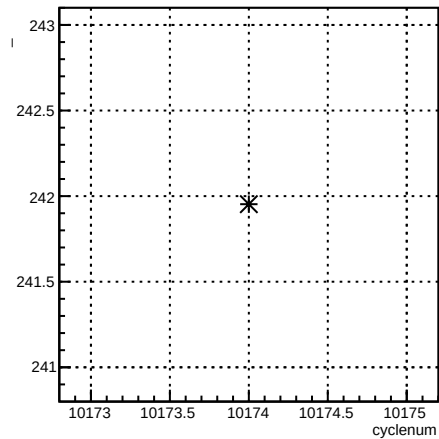
4eX_coil7:cyclenum {run == 8020}
