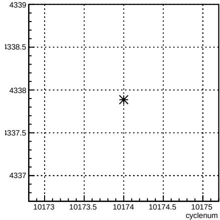
usl_coil7:cyclenum {run == 8020}
