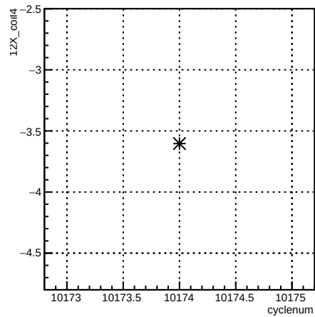
12X_coil4:cyclenum {run == 8020}
