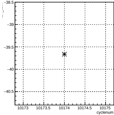
4eY_coil7:cyclenum {run == 8020}
