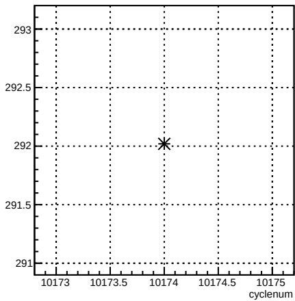
4eY_coil4:cyclenum {run == 8020}
