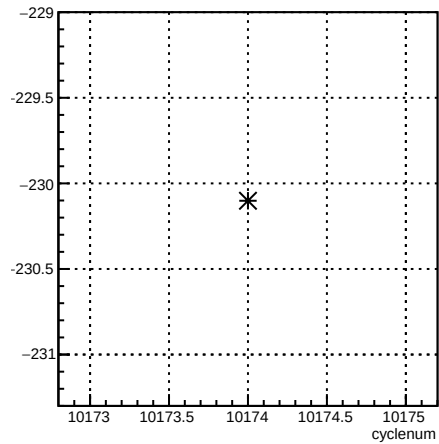
12X_coil1:cyclenum {run == 8020}
