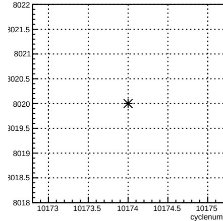
run:cyclenum {run == 8020}
