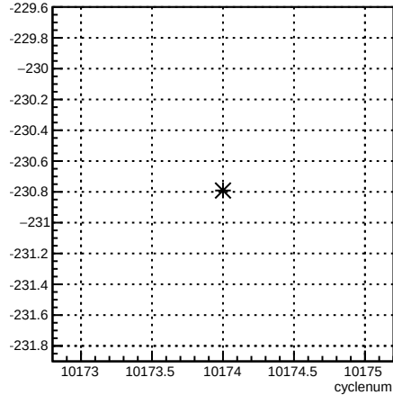
4eX_coil1:cyclenum {run == 8020}
