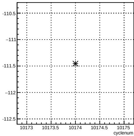
4eY_coil6:cyclenum {run == 8020}
