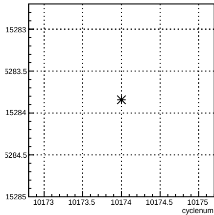
usr_coil1:cyclenum {run == 8020}
