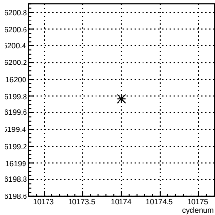
usl_coil6:cyclenum {run == 8020}
