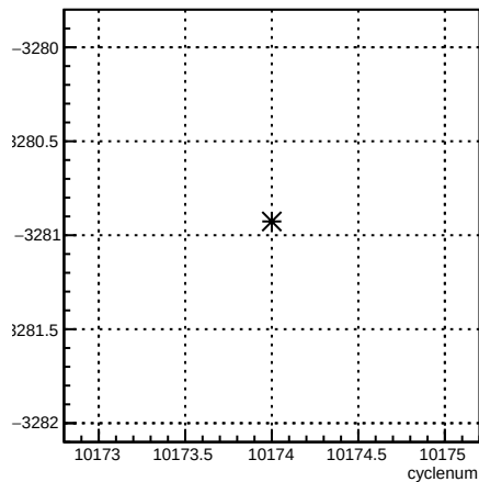
usr_coil6:cyclenum {run == 8020}
