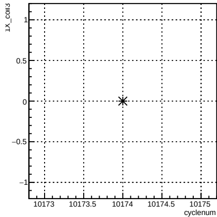
4eX_coil3:cyclenum {run == 8020}
