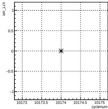
usr_12X:cyclenum {run == 8020}
