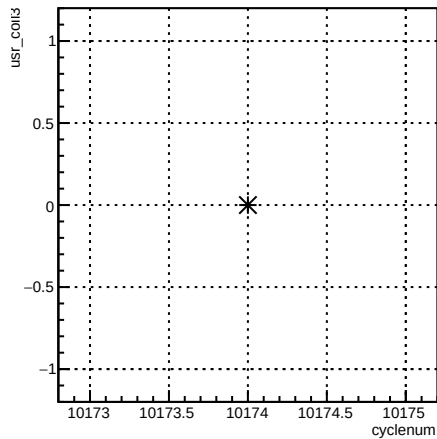
usr_coil3:cyclenum {run == 8020}
