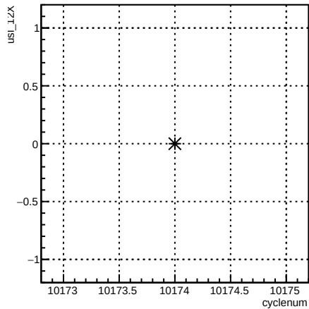
usl_12X:cyclenum {run == 8020}
