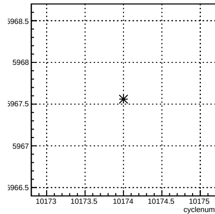
usr_coil4:cyclenum {run == 8020}
