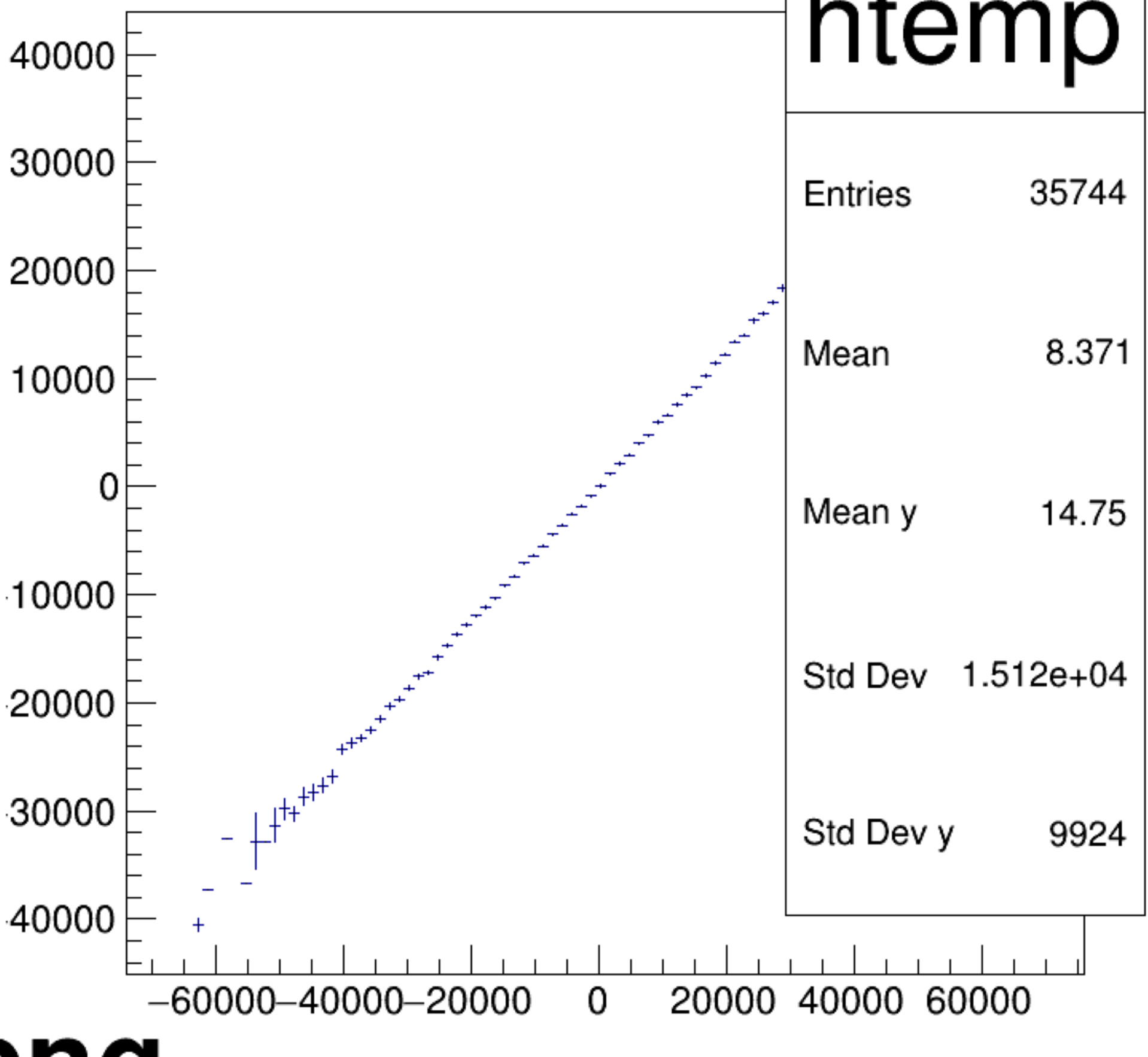
asym_atl2/ppm:asym_atr2/ppm {ok_cut}
