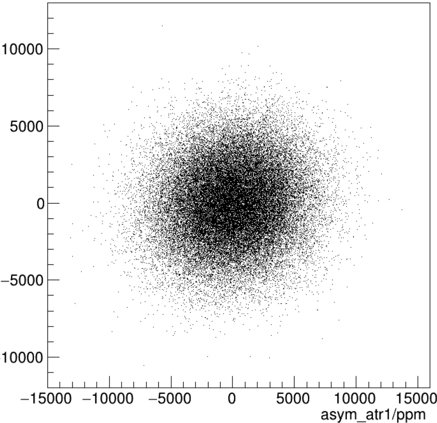
asym_atl1/ppm:asym_atr1/ppm {ok_cut}
