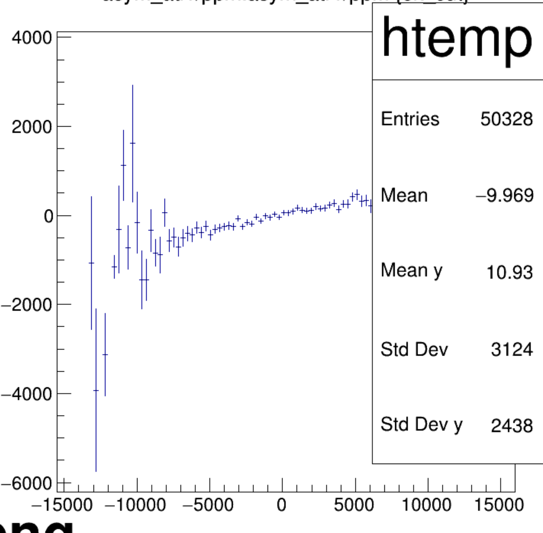
asym_atl1/ppm:asym_atr1/ppm {ok_cut}
