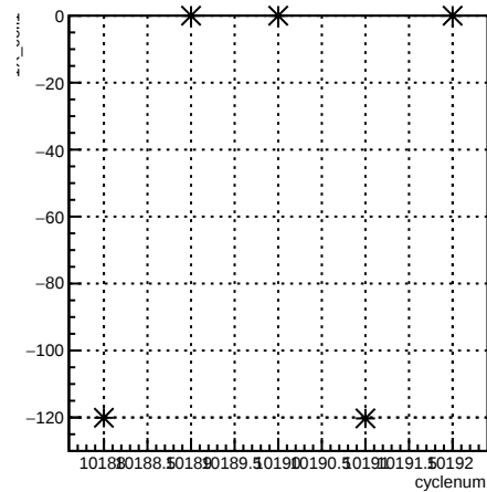
1X_coil1:cyclenum {run == 8023}
