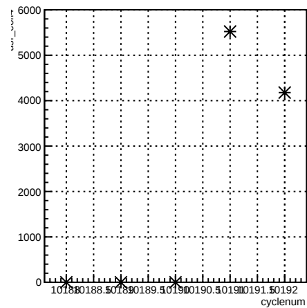
usr_coil4:cyclenum {run == 8023}
