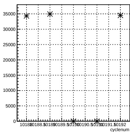
usr_coil7:cyclenum {run == 8023}
