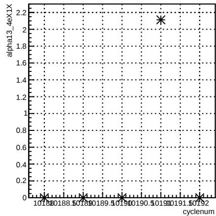
alpha13_4eX1X:cyclenum {run == 8023}
