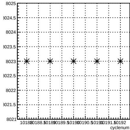
run:cyclenum {run == 8023}
