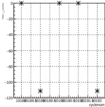
4aY_coil6:cyclenum {run == 8023}
