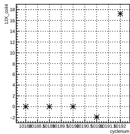
12X_coil4:cyclenum {run == 8023}
