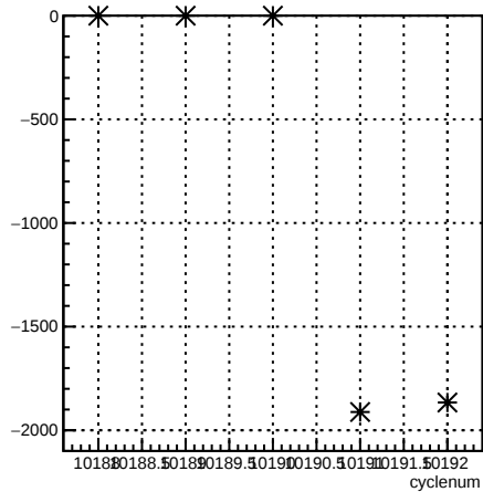
usr_coil3:cyclenum {run == 8023}
