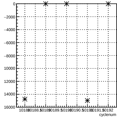
usr_coil1:cyclenum {run == 8023}
