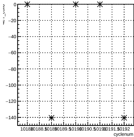
4eY_coil6:cyclenum {run == 8023}
