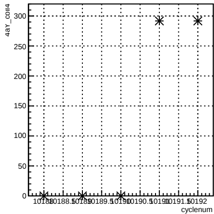
4aY_coil4:cyclenum {run == 8023}
