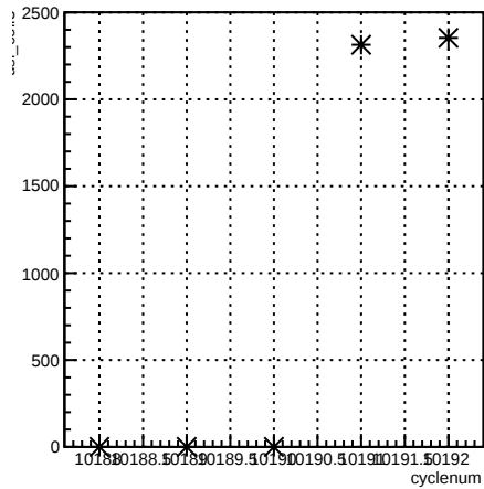
usl_coil3:cyclenum {run == 8023}
