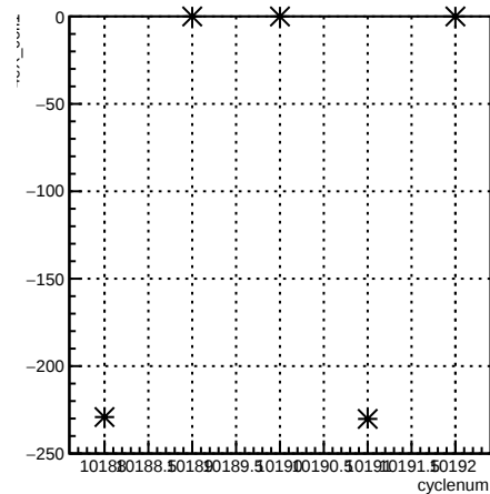
4eX_coil1:cyclenum {run == 8023}
