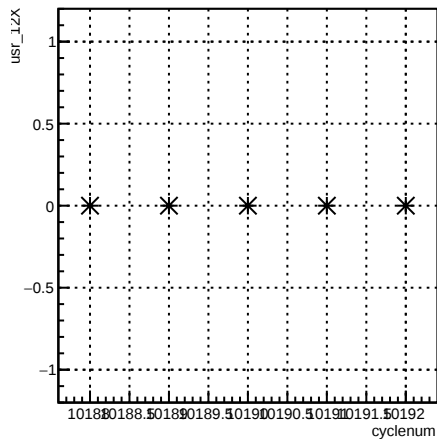
usr_12X:cyclenum {run == 8023}
