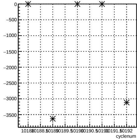
usl_coil6:cyclenum {run == 8023}
