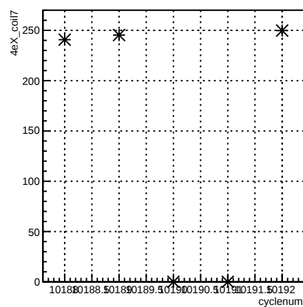
4eX_coil7:cyclenum {run == 8023}
