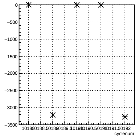
usr_coil6:cyclenum {run == 8023}
