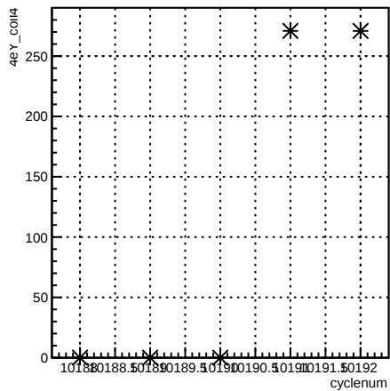
4eY_coil4:cyclenum {run == 8023}
