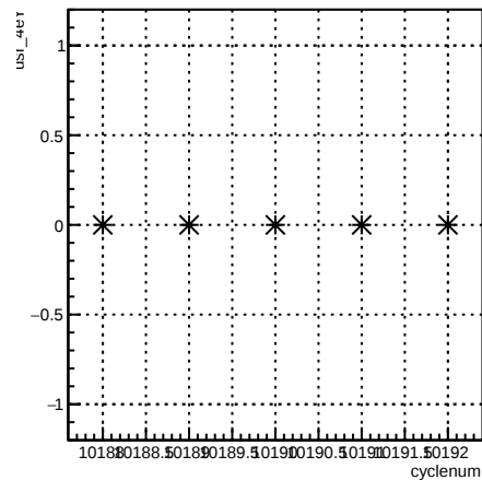
usr_4eY:cyclenum {run == 8023}
