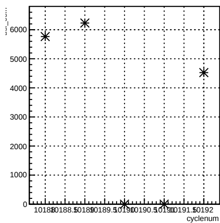
usl_coil7:cyclenum {run == 8023}
