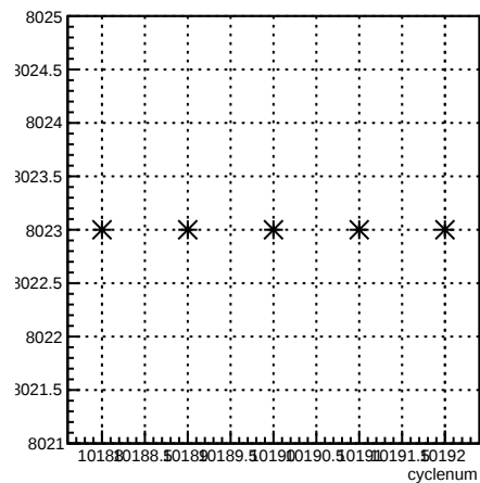
run:cyclenum {run == 8023}
