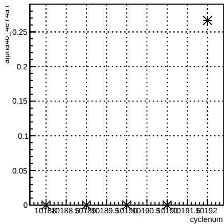
alpha46_4eY4aY:cyclenum {run == 8023}
