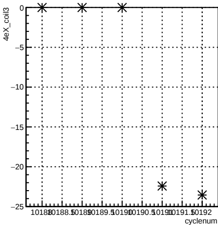
4eX_coil3:cyclenum {run == 8023}
