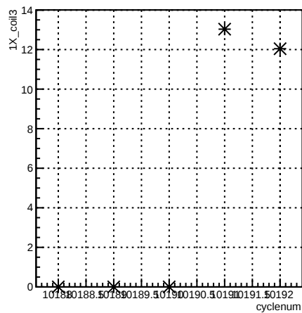
1X_coil3:cyclenum {run == 8023}
