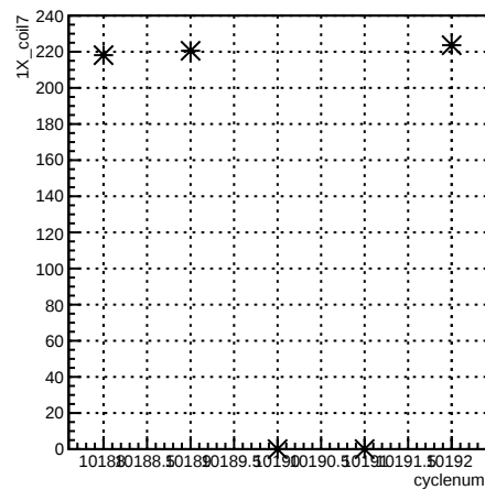
1X_coil7:cyclenum {run == 8023}
