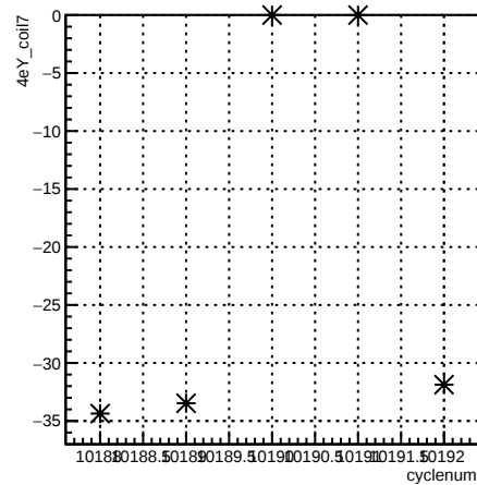
4eY_coil7:cyclenum {run == 8023}
