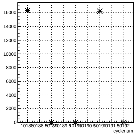
usl_coil6:cyclenum {run == 8023}
