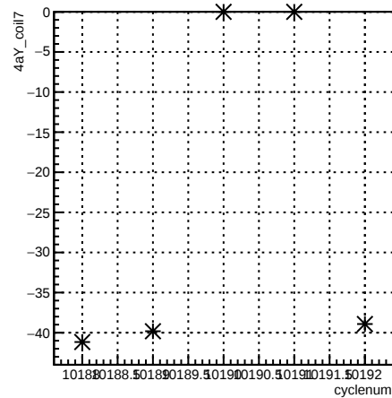
4aY_coil7:cyclenum {run == 8023}
