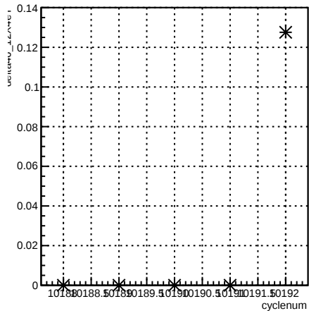
delta46_12X4eY:cyclenum {run == 8023}
