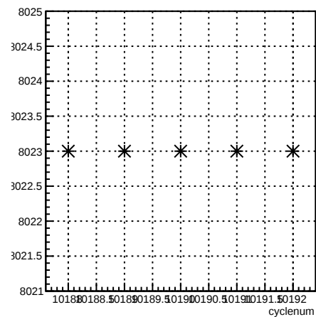
run:cyclenum {run == 8023}
