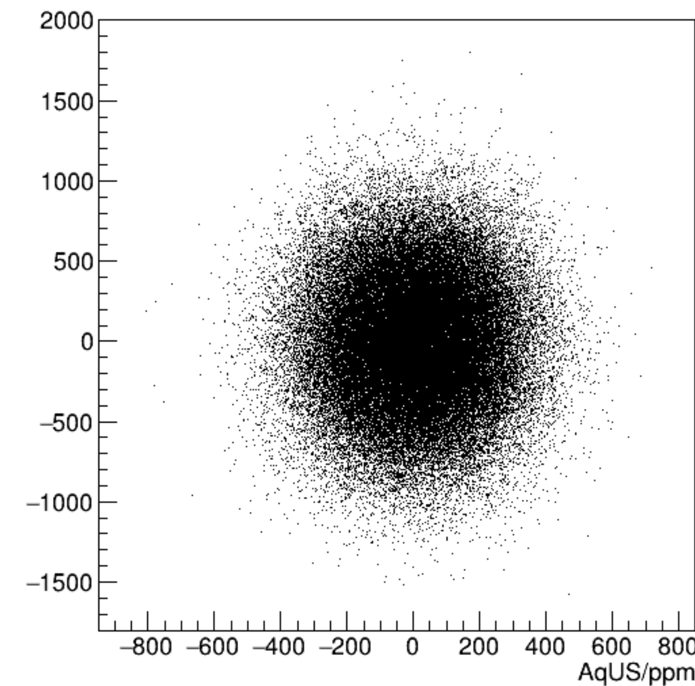
reg_asym_dsr/ppm:AqUS/ppm {ok_cut}
