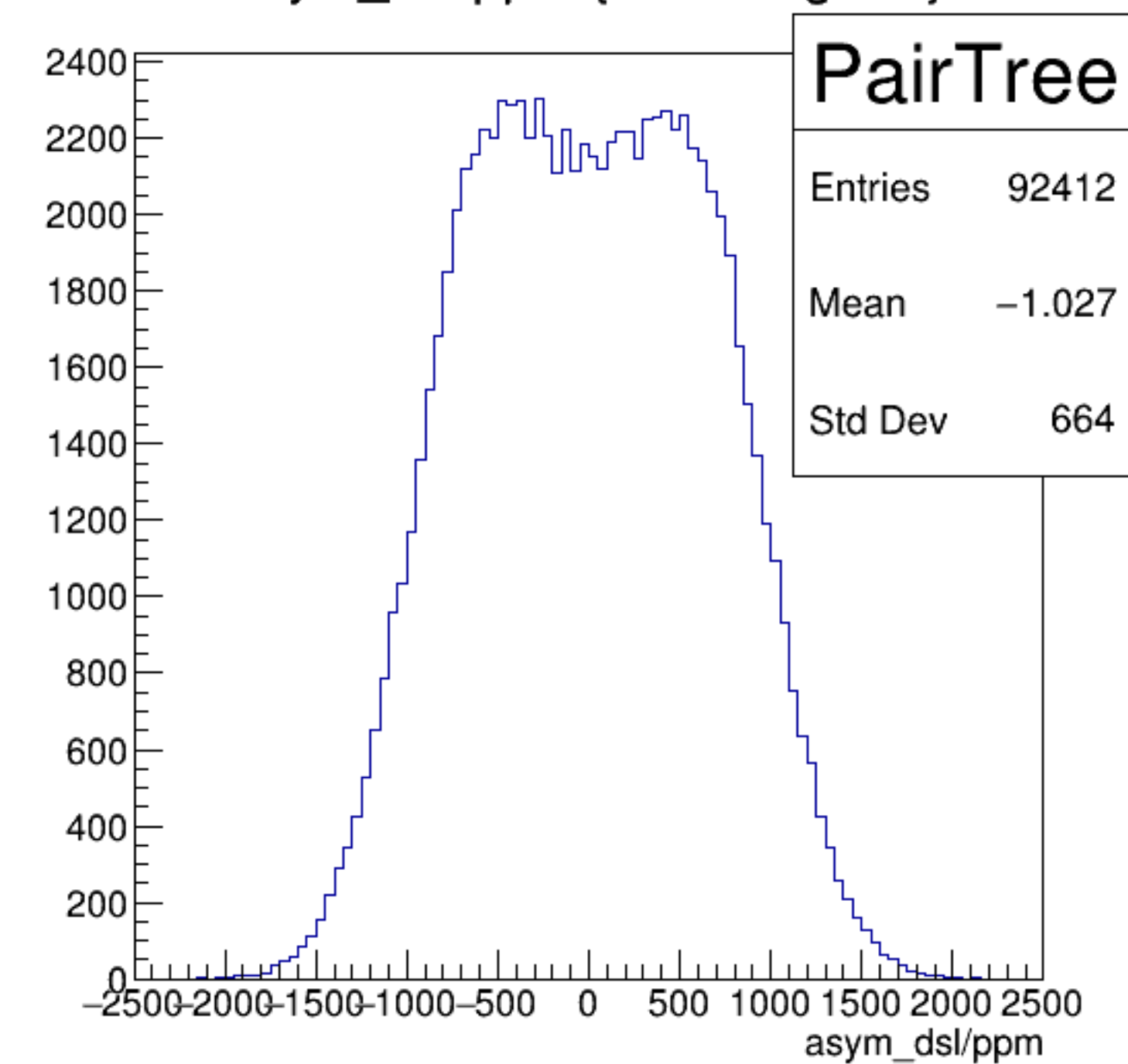
asym_dsl/ppm {ErrorFlag==0}
