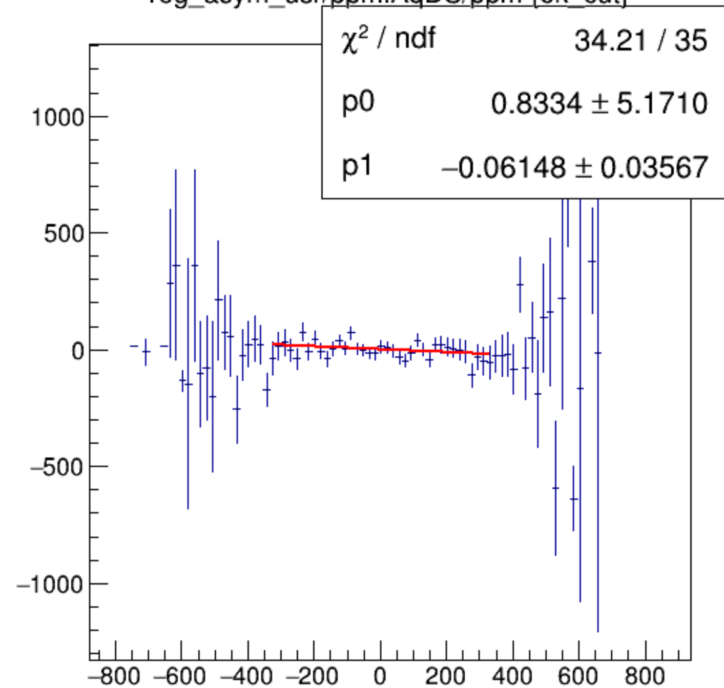
reg_asym_usr/ppm:AqDS/ppm {ok_cut}
