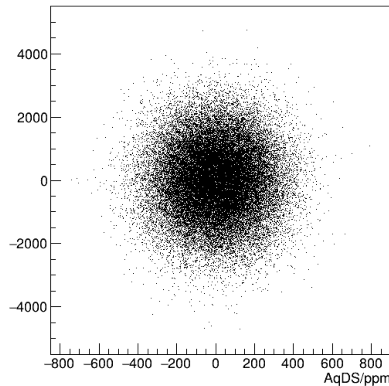
reg_asym_usr/ppm:AqDS/ppm {ok_cut}
