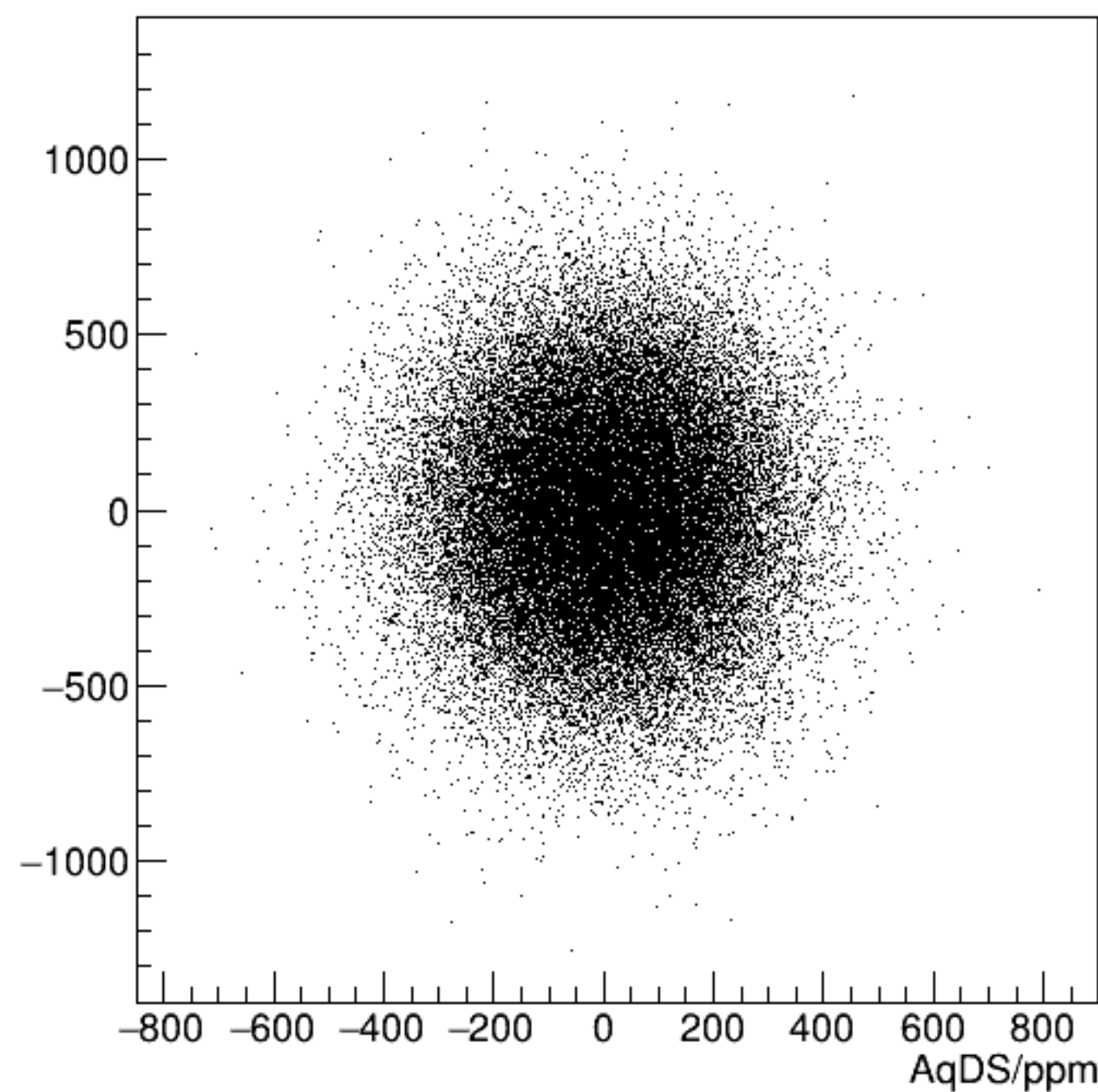
reg_asym_dsl/ppm:AqDS/ppm {ok_cut}
