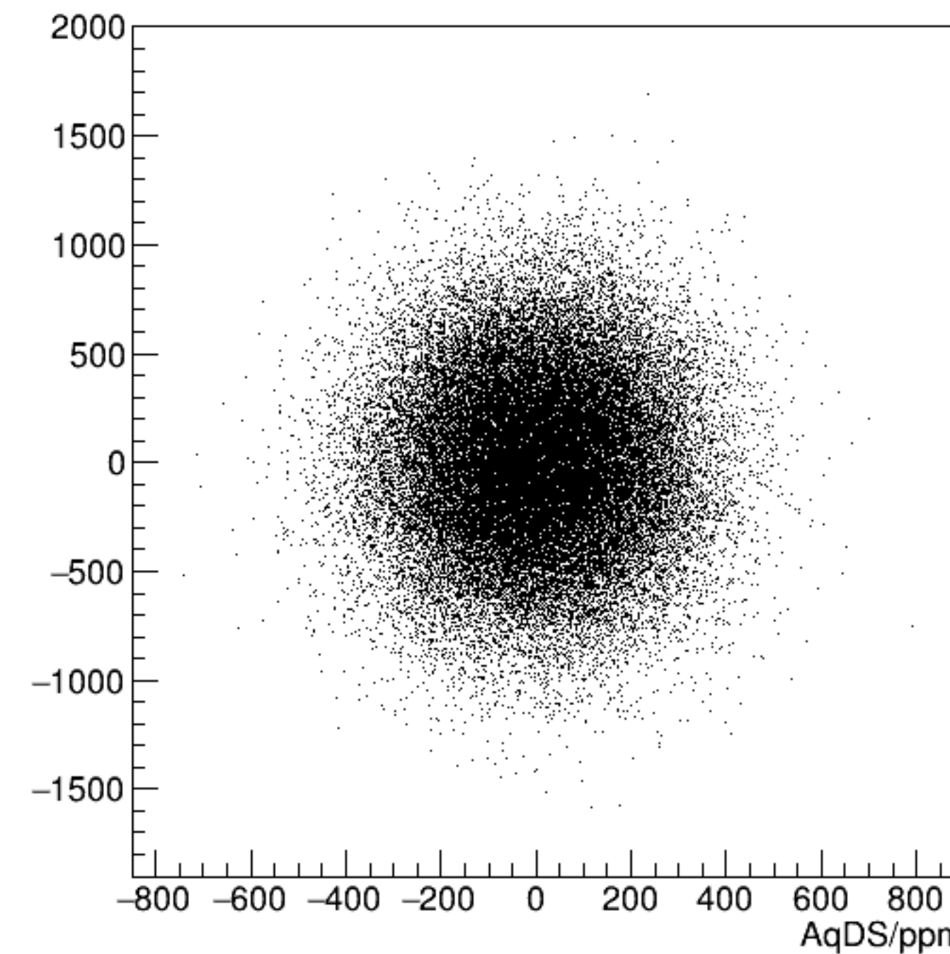
reg_asym_dsr/ppm:AqDS/ppm {ok_cut}
