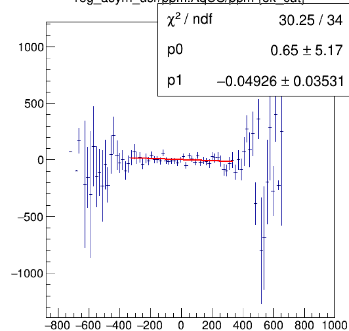
reg_asym_usr/ppm:AqUS/ppm {ok_cut}
