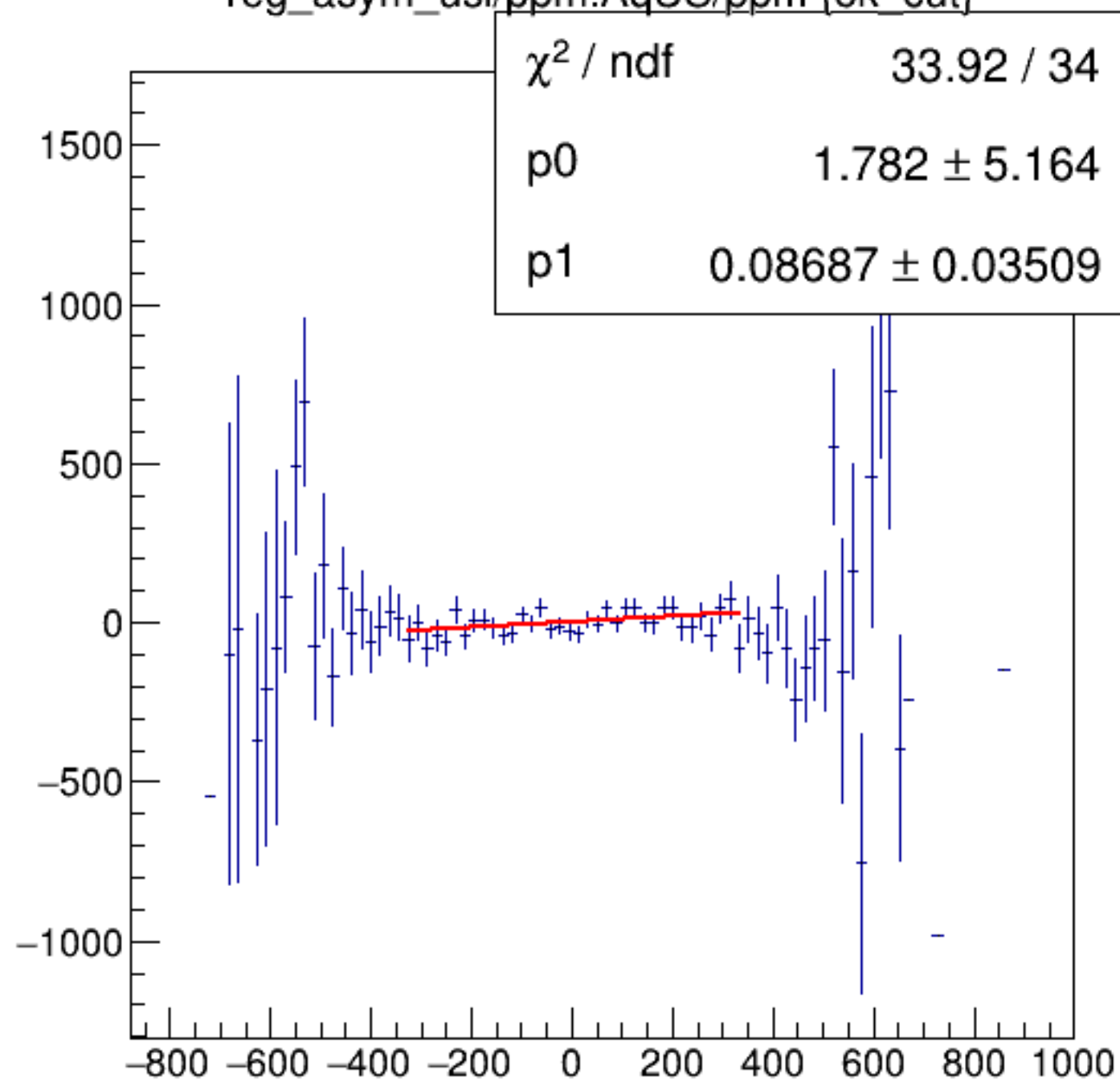
reg_asym_usl/ppm:AqUS/ppm {ok_cut}
