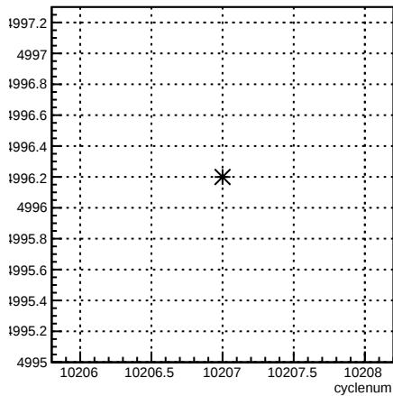
usl_coil7:cyclenum {run == 8027}
