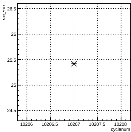
usl_4eY:cyclenum {run == 8027}
