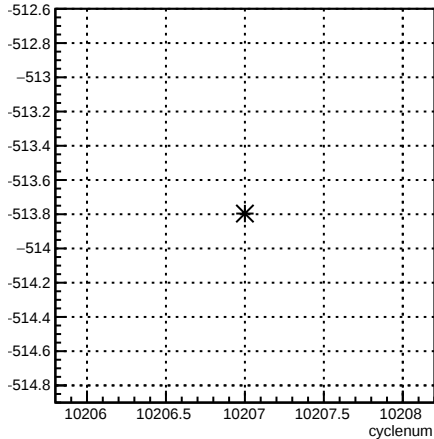
12X_coil7:cyclenum {run == 8027}
