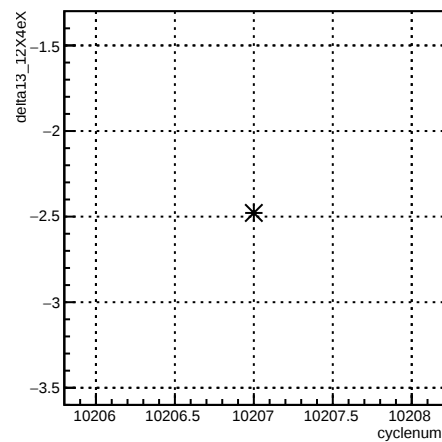
delta13_12X4eX:cyclenum {run == 8027}
