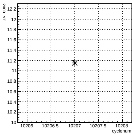
1X_coil3:cyclenum {run == 8027}
