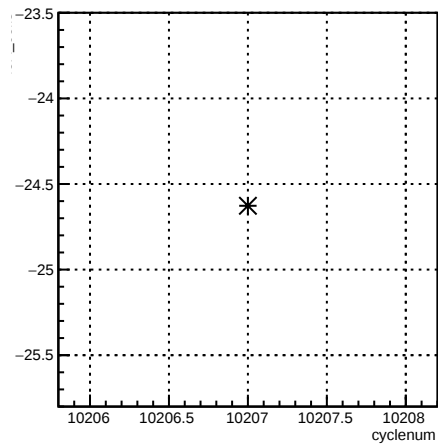
4eX_coil3:cyclenum {run == 8027}
