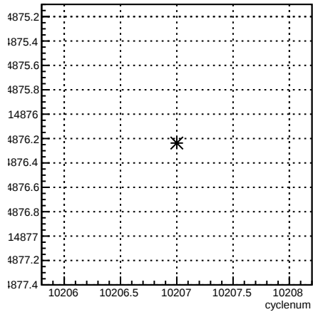
usr_coil6:cyclenum {run == 8027}
