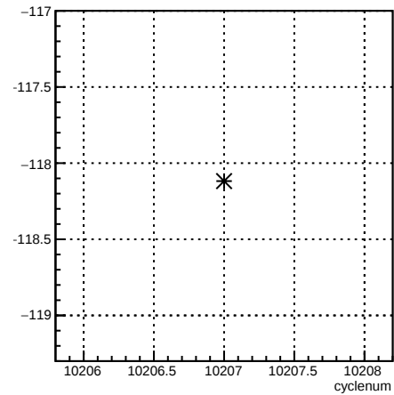
1X_coil1:cyclenum {run == 8027}
