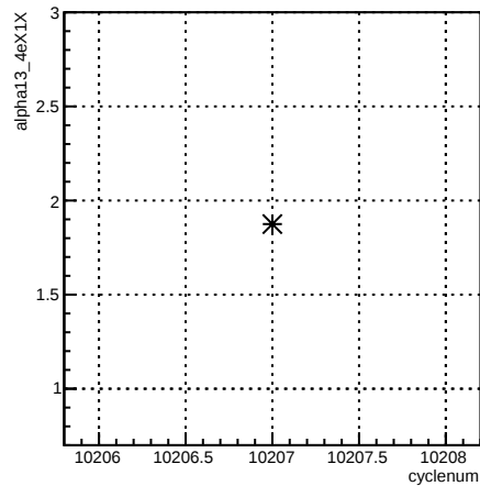
alpha13_4eX1X:cyclenum {run == 8027}
