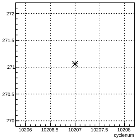
4eY_coil4:cyclenum {run == 8027}
