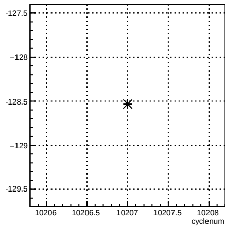
usr_4eY:cyclenum {run == 8027}
