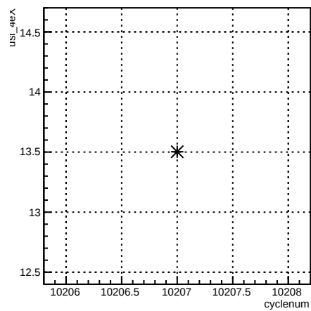
usl_4eX:cyclenum {run == 8027}
