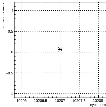
delta46_12X4eY:cyclenum {run == 8027}
