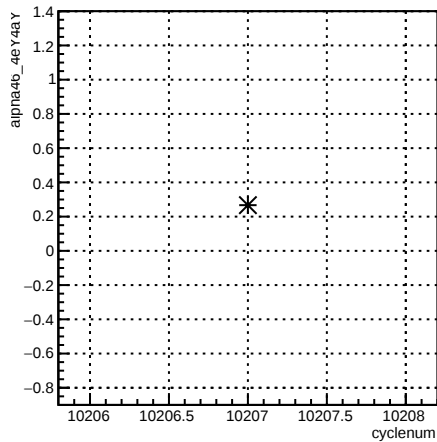
alpha46_4eY4aY:cyclenum {run == 8027}
