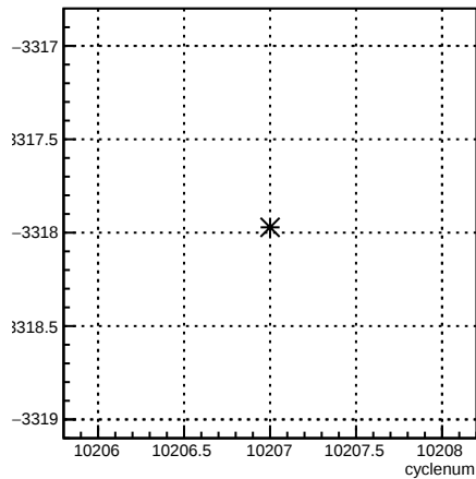
usl_coil6:cyclenum {run == 8027}
