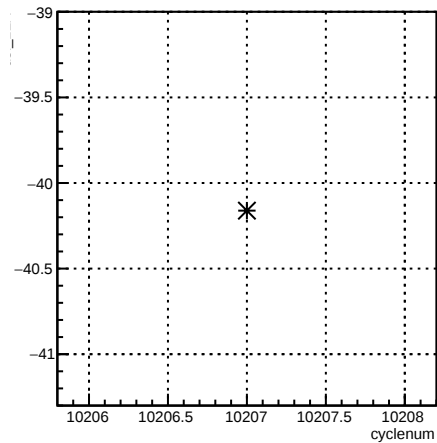
usl_12X:cyclenum {run == 8027}
