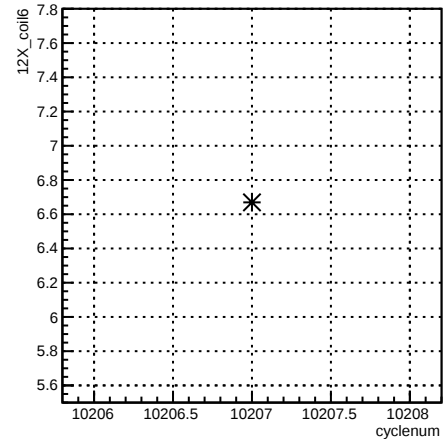
12X_coil6:cyclenum {run == 8027}
