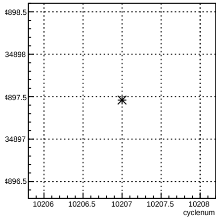
usr_coil7:cyclenum {run == 8027}
