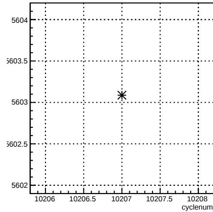
run:cyclenum {run == 8027}
