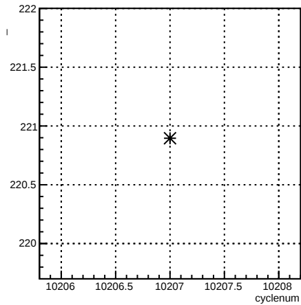
1X_coil7:cyclenum {run == 8027}
