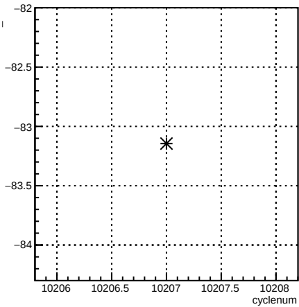
usl_1X:cyclenum {run == 8027}
