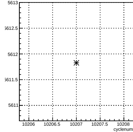
run:cyclenum {run == 8027}
