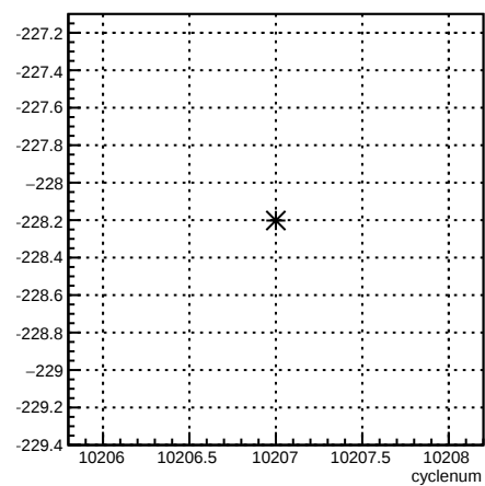
4eX_coil1:cyclenum {run == 8027}
