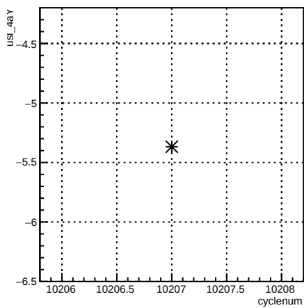
usl_4aY:cyclenum {run == 8027}
