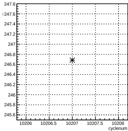
4eX_coil7:cyclenum {run == 8027}
