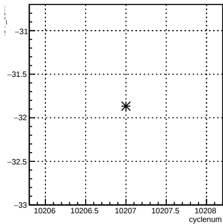
4eY_coil7:cyclenum {run == 8027}
