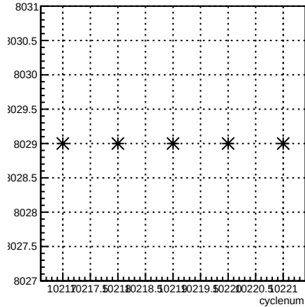
run:cyclenum {run == 8029}
