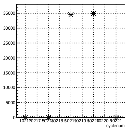
usr_coil7:cyclenum {run == 8029}
