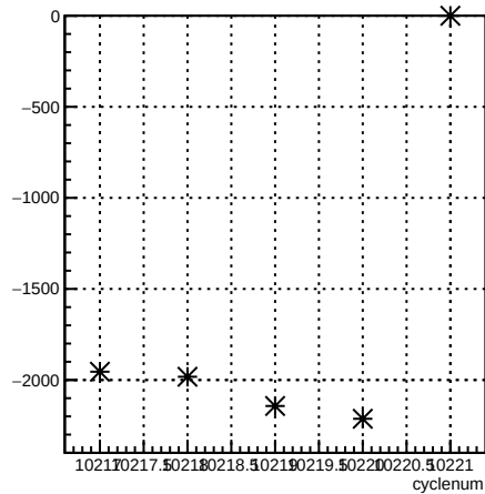
usr_coil3:cyclenum {run == 8029}
