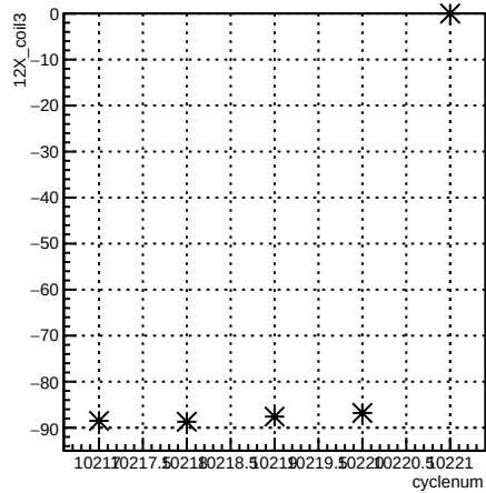
12X_coil3:cyclenum {run == 8029}
