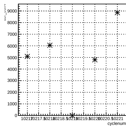
usr_coil4:cyclenum {run == 8029}
