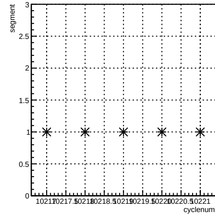
segment:cyclenum {run == 8029}
