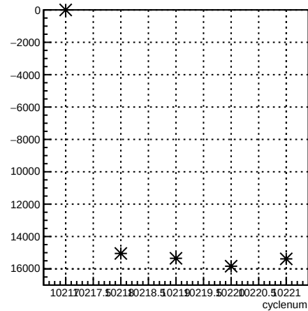
usr_coil1:cyclenum {run == 8029}
