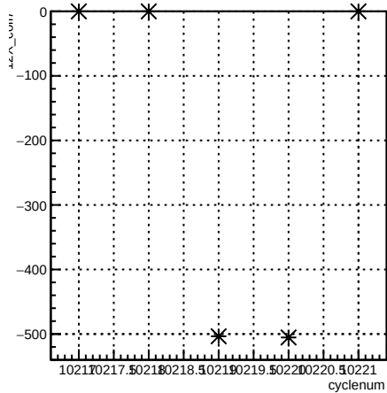
12X_coil7:cyclenum {run == 8029}
