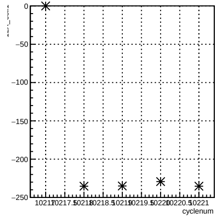
12X_coil1:cyclenum {run == 8029}
