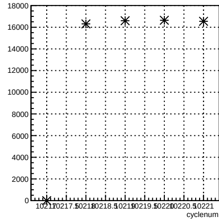
usl_coil1:cyclenum {run == 8029}
