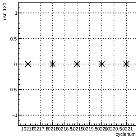
usr_12X:cyclenum {run == 8029}
