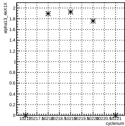
alpha13_4eX1X:cyclenum {run == 8029}
