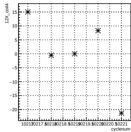
12X_coil4:cyclenum {run == 8029}
