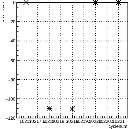
4eY_coil6:cyclenum {run == 8029}
