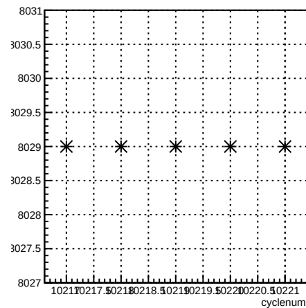
run:cyclenum {run == 8029}
