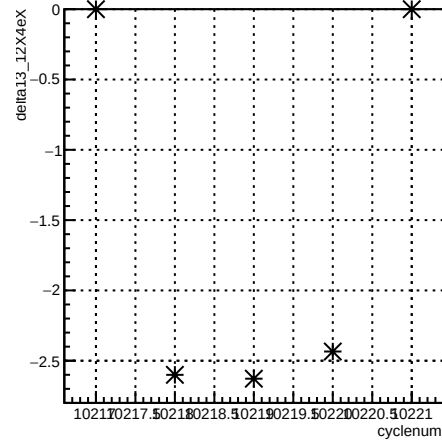
delta13_12X4eX:cyclenum {run == 8029}
