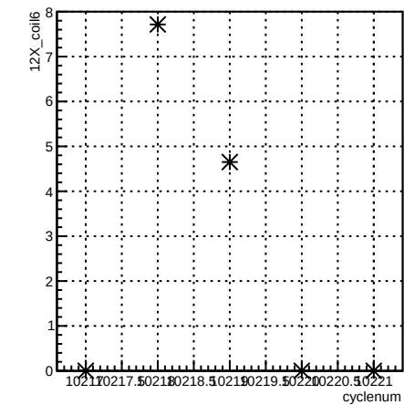
12X_coil6:cyclenum {run == 8029}
