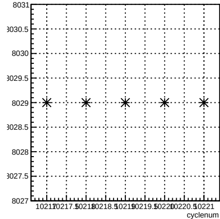
run:cyclenum {run == 8029}
