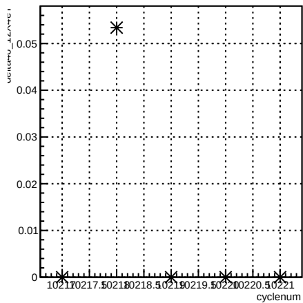
delta46_12X4eY:cyclenum {run == 8029}
