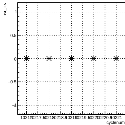
usr_4eY:cyclenum {run == 8029}
