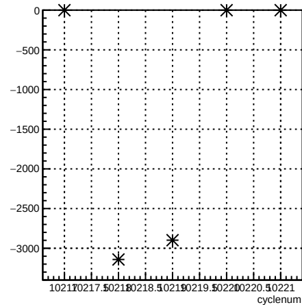
usr_coil6:cyclenum {run == 8029}
