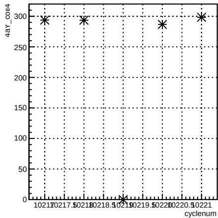
4eY_coil4:cyclenum {run == 8029}
