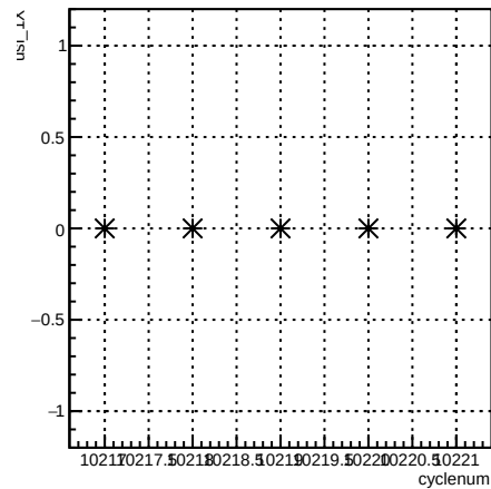
usl_4eY:cyclenum {run == 8029}
