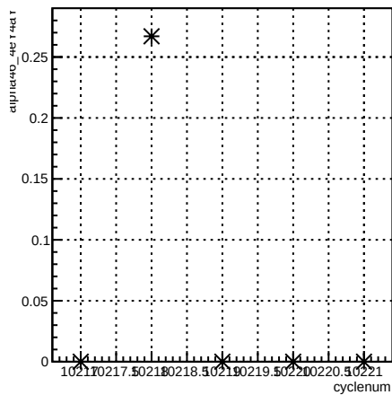
alpha46_4eY4aY:cyclenum {run == 8029}
