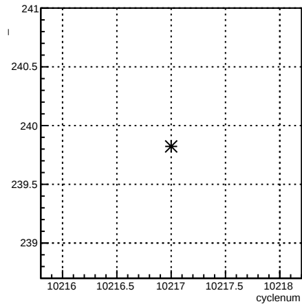
4eX_coil7:cyclenum {run == 8029}
