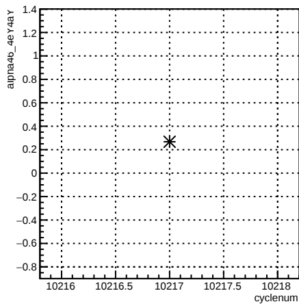
alpha46_4eY4aY:cyclenum {run == 8029}
