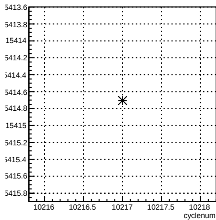
usr_coil1:cyclenum {run == 8029}
