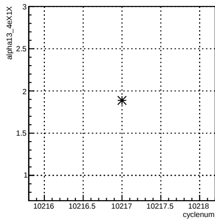
alpha13_4eX1X:cyclenum {run == 8029}
