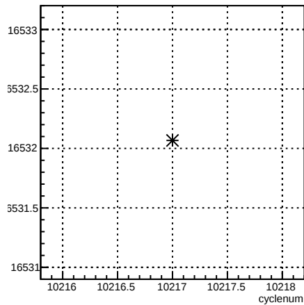
usl_coil6:cyclenum {run == 8029}
