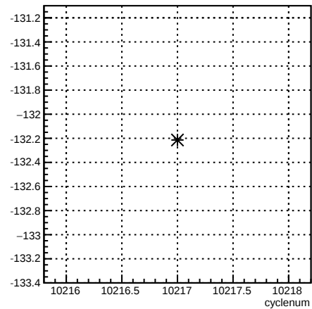
usr_4eY:cyclenum {run == 8029}
