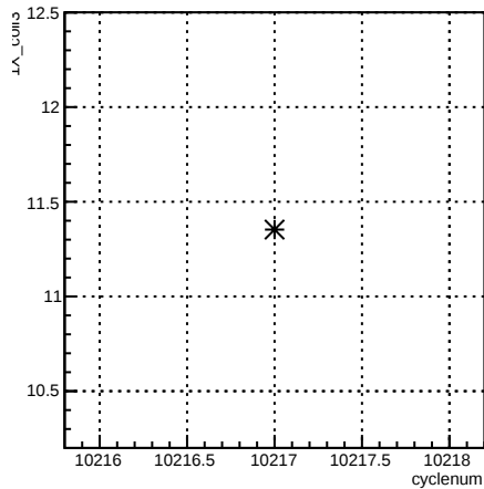
1X_coil3:cyclenum {run == 8029}
