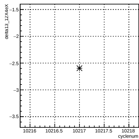
delta13_12X4eX:cyclenum {run == 8029}
