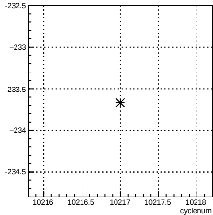
12X_coil1:cyclenum {run == 8029}
