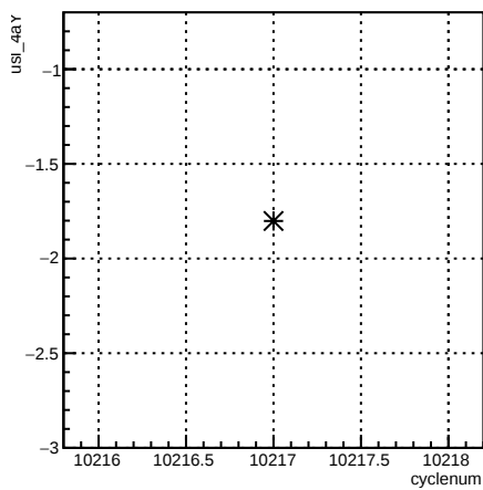
usl_4aY:cyclenum {run == 8029}
