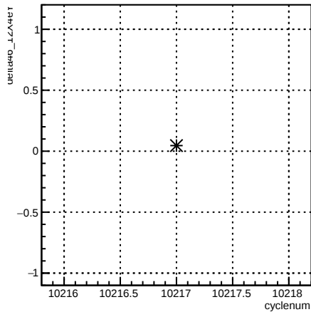
delta46_12X4eY:cyclenum {run == 8029}
