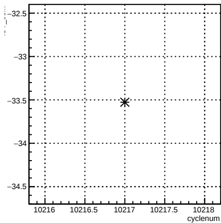
4eY_coil7:cyclenum {run == 8029}
