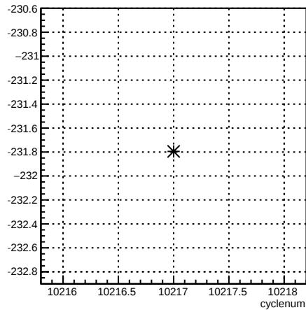
4eX_coil1:cyclenum {run == 8029}
