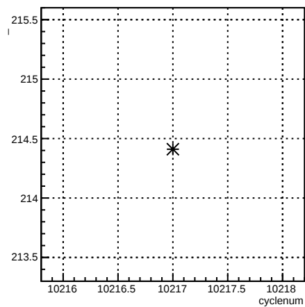
1X_coil7:cyclenum {run == 8029}
