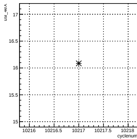
usl_4eX:cyclenum {run == 8029}
