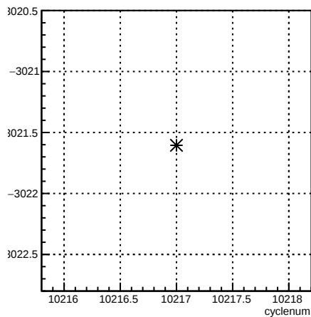
usr_coil6:cyclenum {run == 8029}
