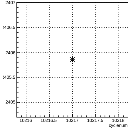
usl_coil7:cyclenum {run == 8029}
