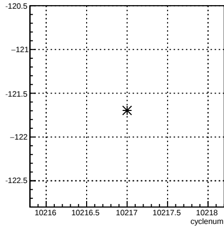
1X_coil1:cyclenum {run == 8029}
