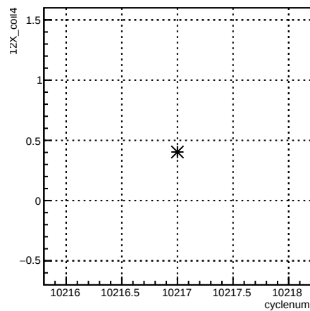
12X_coil4:cyclenum {run == 8029}
