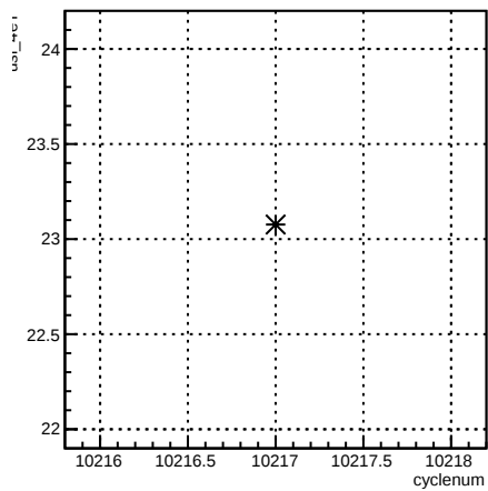
usl_4eY:cyclenum {run == 8029}
