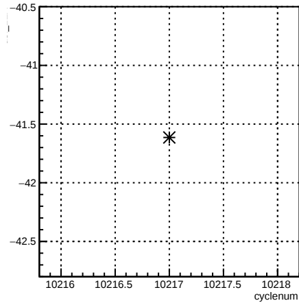
usl_12X:cyclenum {run == 8029}
