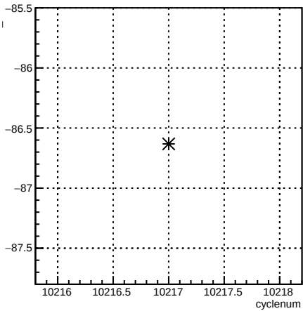
usl_1X:cyclenum {run == 8029}
