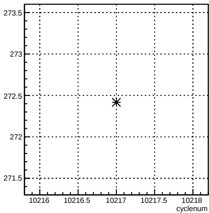
4eY_coil4:cyclenum {run == 8029}
