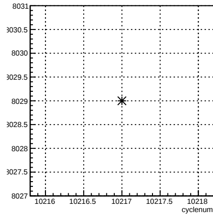
run:cyclenum {run == 8029}
