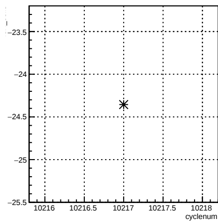
4eX_coil3:cyclenum {run == 8029}
