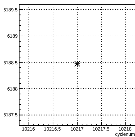
usr_coil4:cyclenum {run == 8029}
