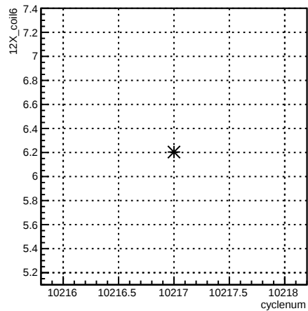
12X_coil6:cyclenum {run == 8029}
