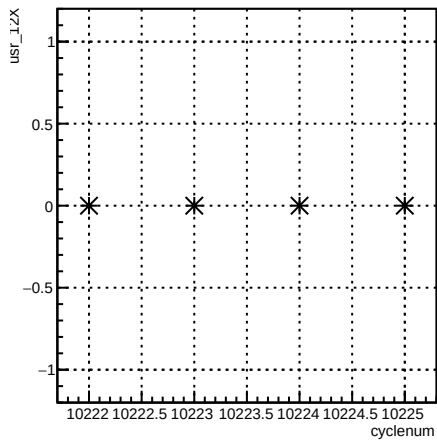
usr_12X:cyclenum {run == 8030}
