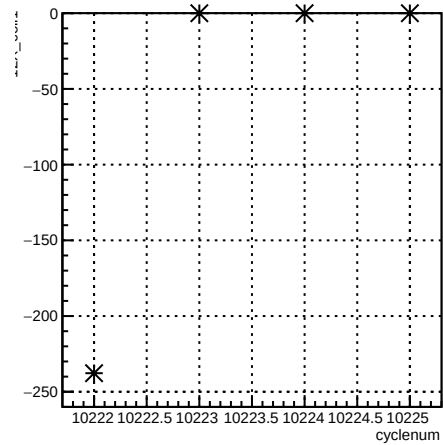
12X_coil1:cyclenum {run == 8030}
