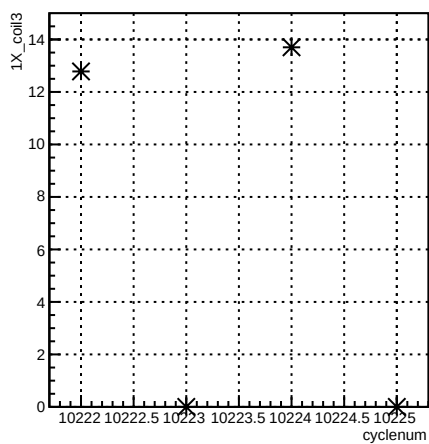
1X_coil3:cyclenum {run == 8030}
