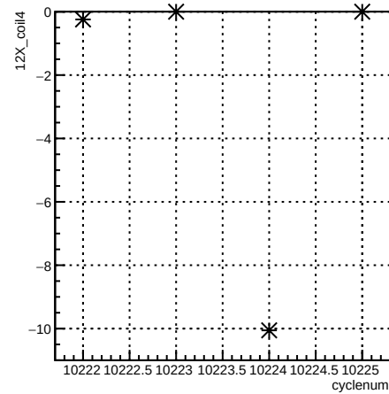
12X_coil4:cyclenum {run == 8030}
