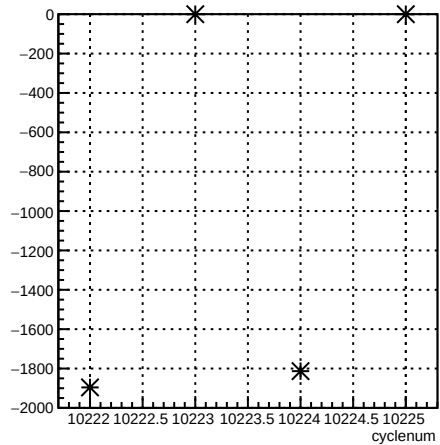
usr_coil3:cyclenum {run == 8030}
