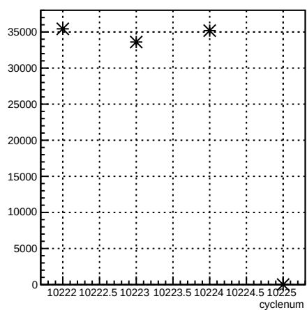
usr_coil7:cyclenum {run == 8030}
