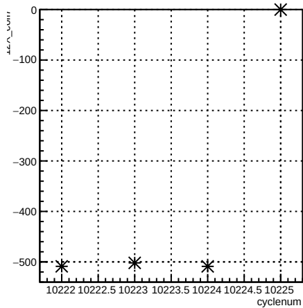
12X_coil7:cyclenum {run == 8030}
