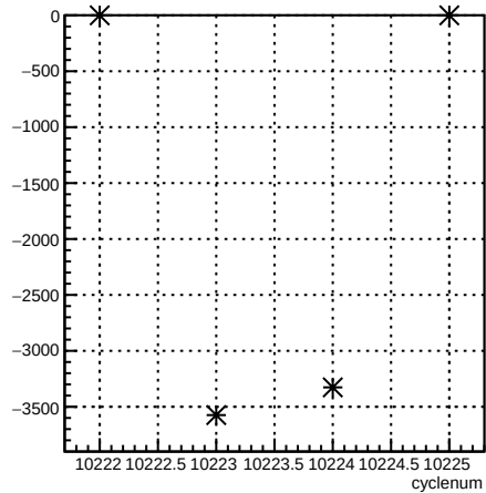
usl_coil6:cyclenum {run == 8030}
