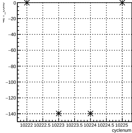
4eY_coil6:cyclenum {run == 8030}
