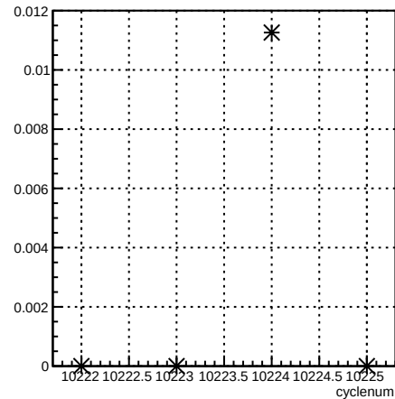
delta46_12X4eY:cyclenum {run == 8030}
