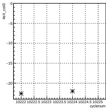
4eX_coil3:cyclenum {run == 8030}
