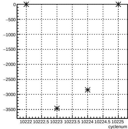
usr_coil6:cyclenum {run == 8030}
