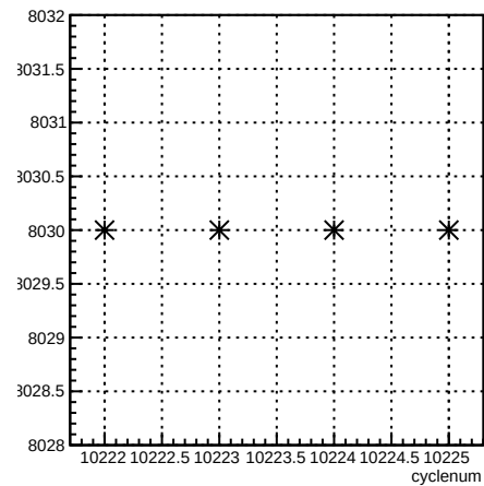
run:cyclenum {run == 8030}
