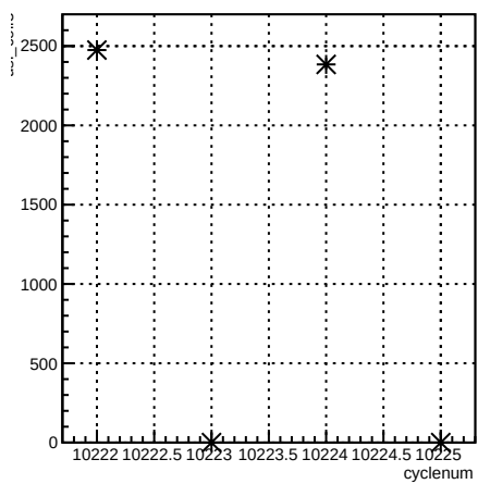
usl_coil3:cyclenum {run == 8030}
