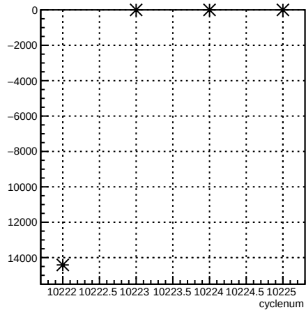
usr_coil1:cyclenum {run == 8030}
