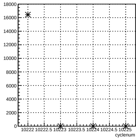
usl_coil1:cyclenum {run == 8030}
