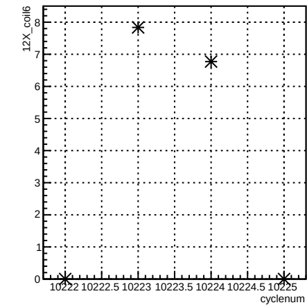
12X_coil6:cyclenum {run == 8030}
