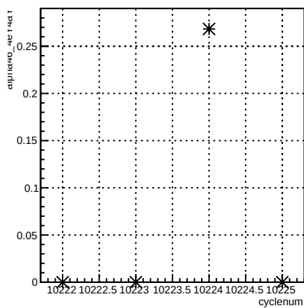
alpha46_4eY4aY:cyclenum {run == 8030}
