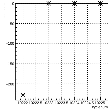
4eX_coil1:cyclenum {run == 8030}
