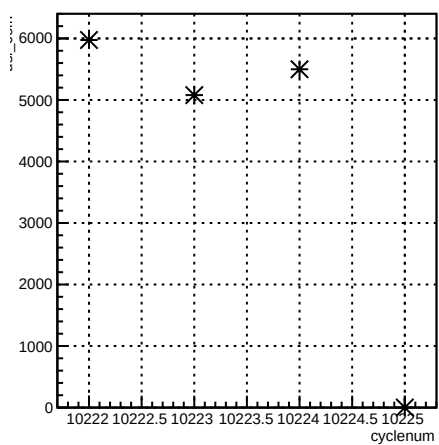
usl_coil7:cyclenum {run == 8030}
