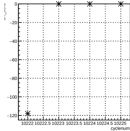
1X_coil1:cyclenum {run == 8030}
