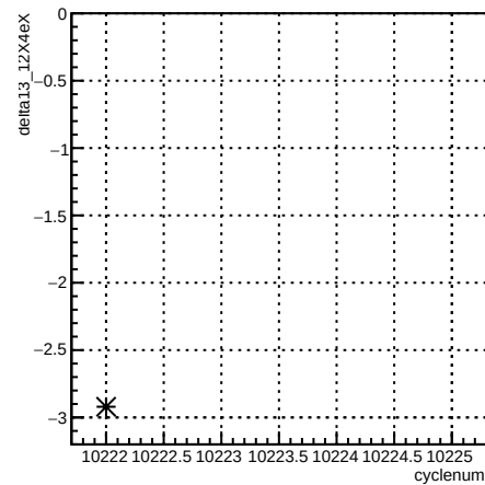
delta13_12X4eX:cyclenum {run == 8030}
