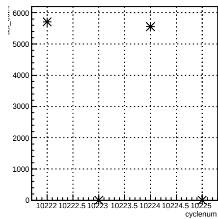
usl_coil4:cyclenum {run == 8030}
