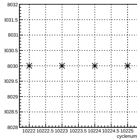
run:cyclenum {run == 8030}
