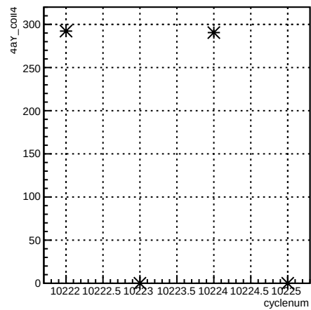
4aY_coil4:cyclenum {run == 8030}
