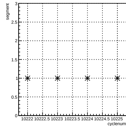
segment:cyclenum {run == 8030}
