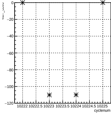
4aY_coil6:cyclenum {run == 8030}
