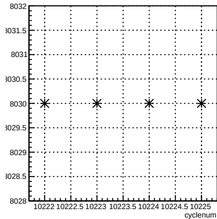
run:cyclenum {run == 8030}
