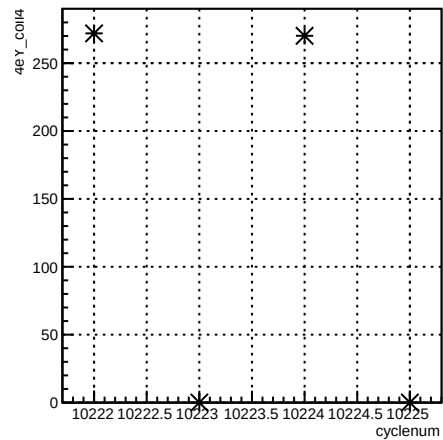
4eY_coil4:cyclenum {run == 8030}
