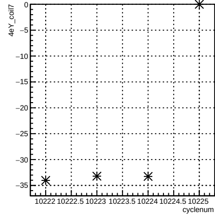
4eY_coil7:cyclenum {run == 8030}
