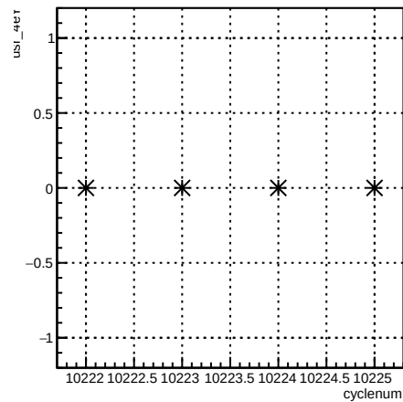
usr_4eY:cyclenum {run == 8030}
