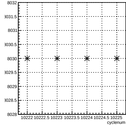
run:cyclenum {run == 8030}
