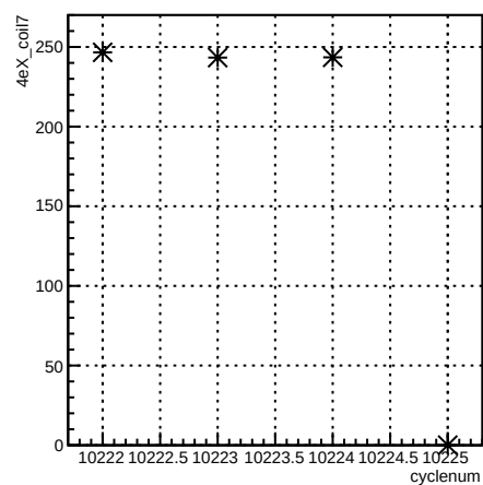
4eX_coil7:cyclenum {run == 8030}
