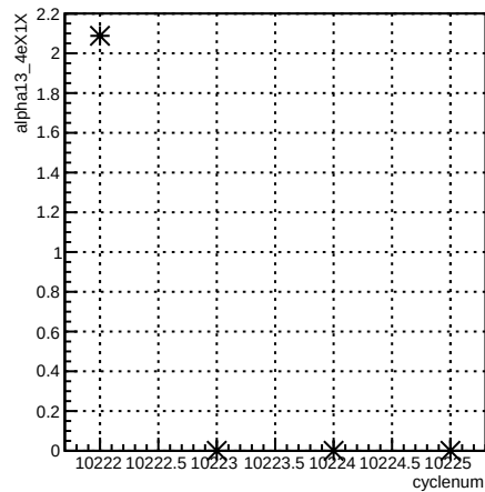
alpha13_4eX1X:cyclenum {run == 8030}
