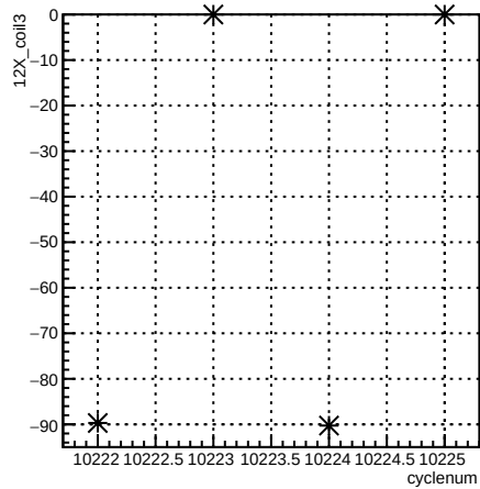
12X_coil3:cyclenum {run == 8030}
