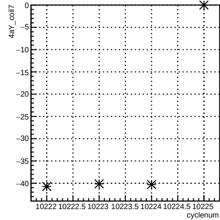
4aY_coil7:cyclenum {run == 8030}
