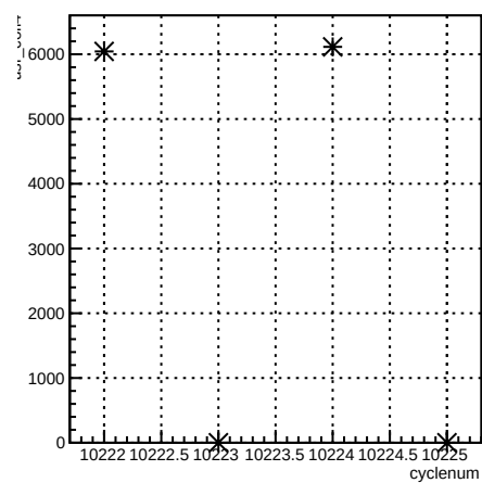
usr_coil4:cyclenum {run == 8030}
