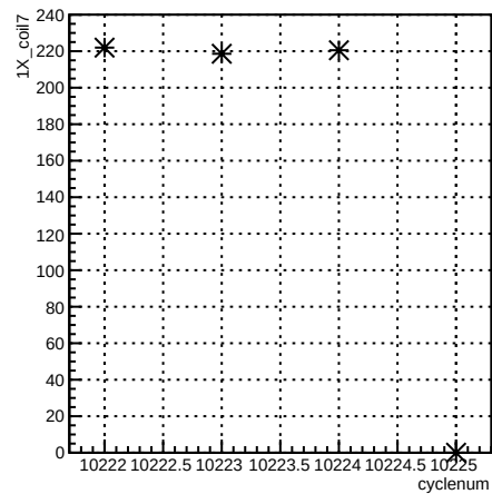
1X_coil7:cyclenum {run == 8030}
