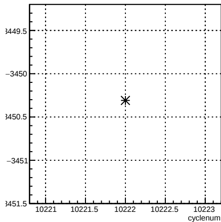
usl_coil6:cyclenum {run == 8030}
