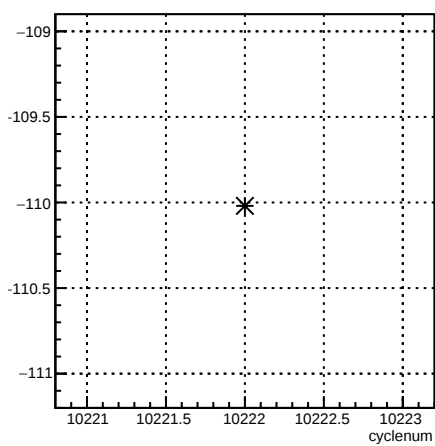
4aY_coil6:cyclenum {run == 8030}
