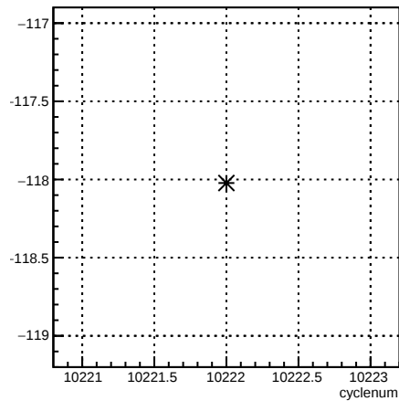
4eX_coil1:cyclenum {run == 8030}
