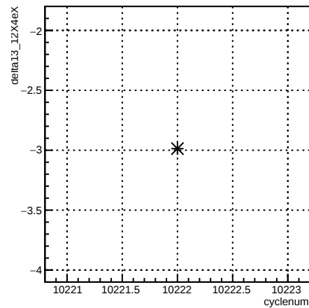
delta13_12X4eX:cyclenum {run == 8030}
