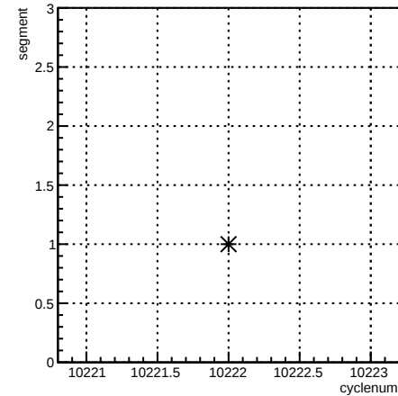
segment:cyclenum {run == 8030}
