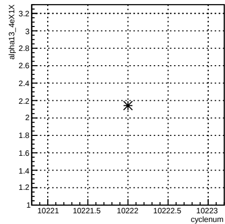
alpha13_4eX1X:cyclenum {run == 8030}
