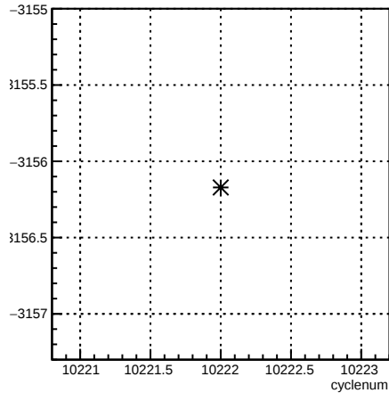
usr_coil6:cyclenum {run == 8030}
