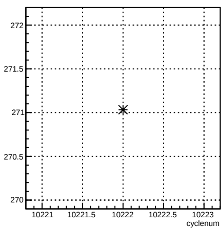
4eY_coil4:cyclenum {run == 8030}
