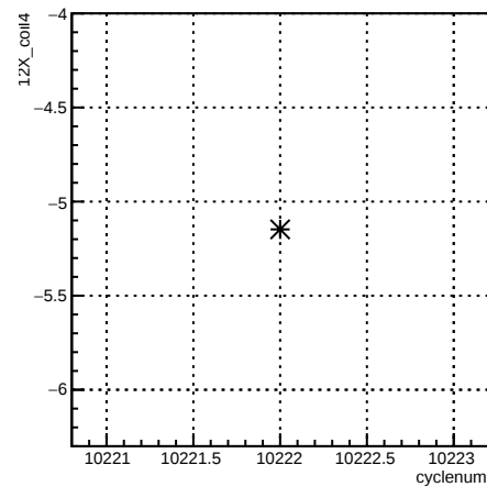
12X_coil4:cyclenum {run == 8030}
