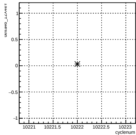
delta46_12X4eY:cyclenum {run == 8030}
