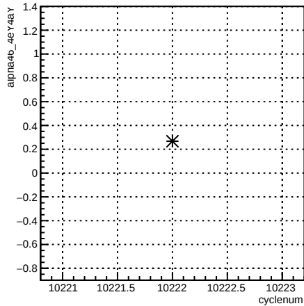
alpha46_4eY4aY:cyclenum {run == 8030}
