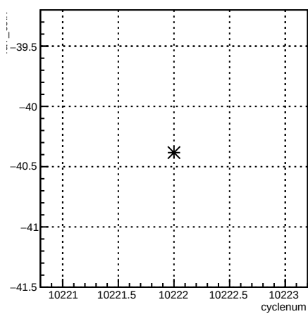
4aY_coil7:cyclenum {run == 8030}
