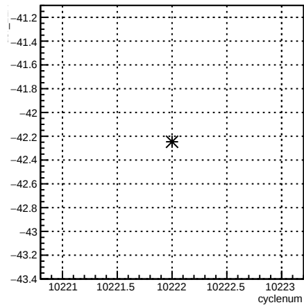
usr_12X:cyclenum {run == 8030}
