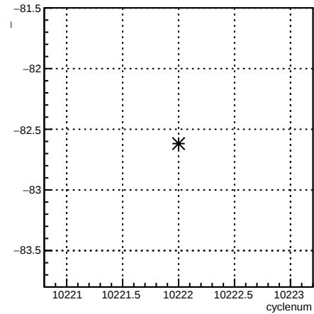
usl_1X:cyclenum {run == 8030}
