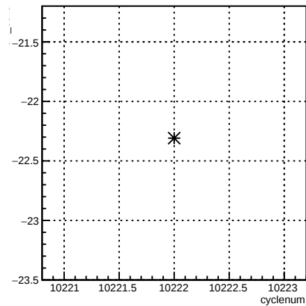
4eX_coil3:cyclenum {run == 8030}
