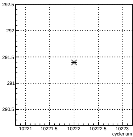
4aY_coil4:cyclenum {run == 8030}
