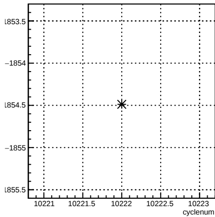
usr_coil7:cyclenum {run == 8030}
