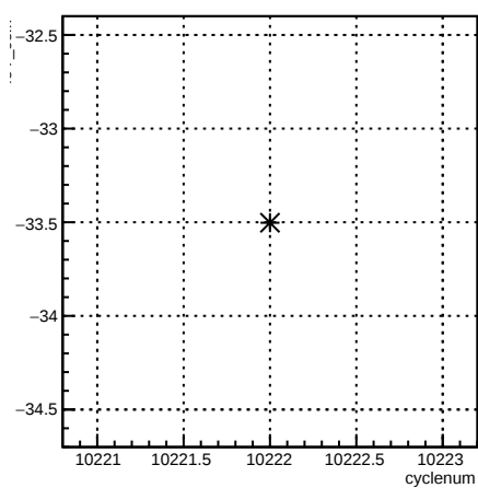
4eY_coil7:cyclenum {run == 8030}
