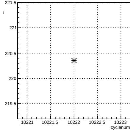
4eX_coil7:cyclenum {run == 8030}
