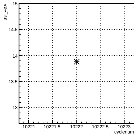
usl_4eX:cyclenum {run == 8030}
