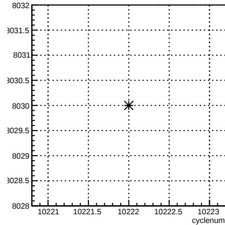
run:cyclenum {run == 8030}
