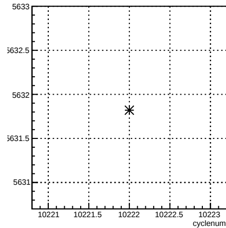
usl_coil4:cyclenum {run == 8030}
