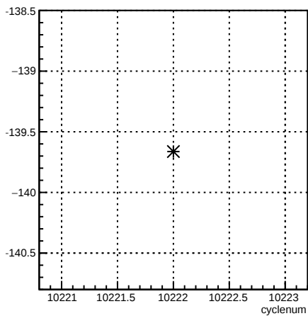
4eY_coil6:cyclenum {run == 8030}
