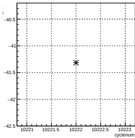
usl_12X:cyclenum {run == 8030}
