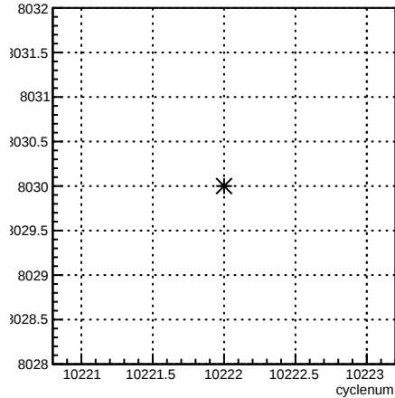
run:cyclenum {run == 8030}
