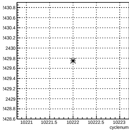
usl_coil7:cyclenum {run == 8030}
