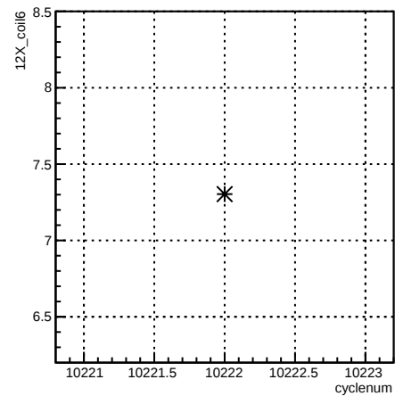
12X_coil6:cyclenum {run == 8030}
