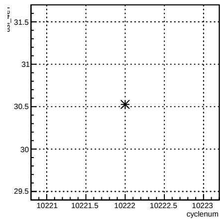
usl_4eY:cyclenum {run == 8030}
