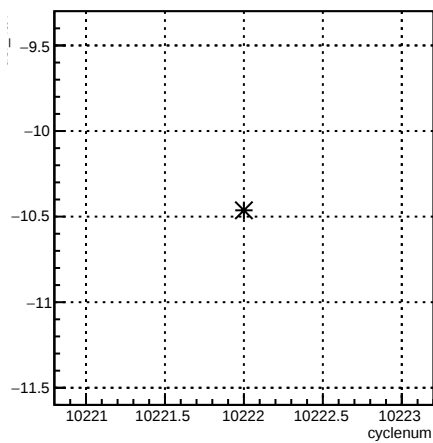
usl_4aY:cyclenum {run == 8030}
