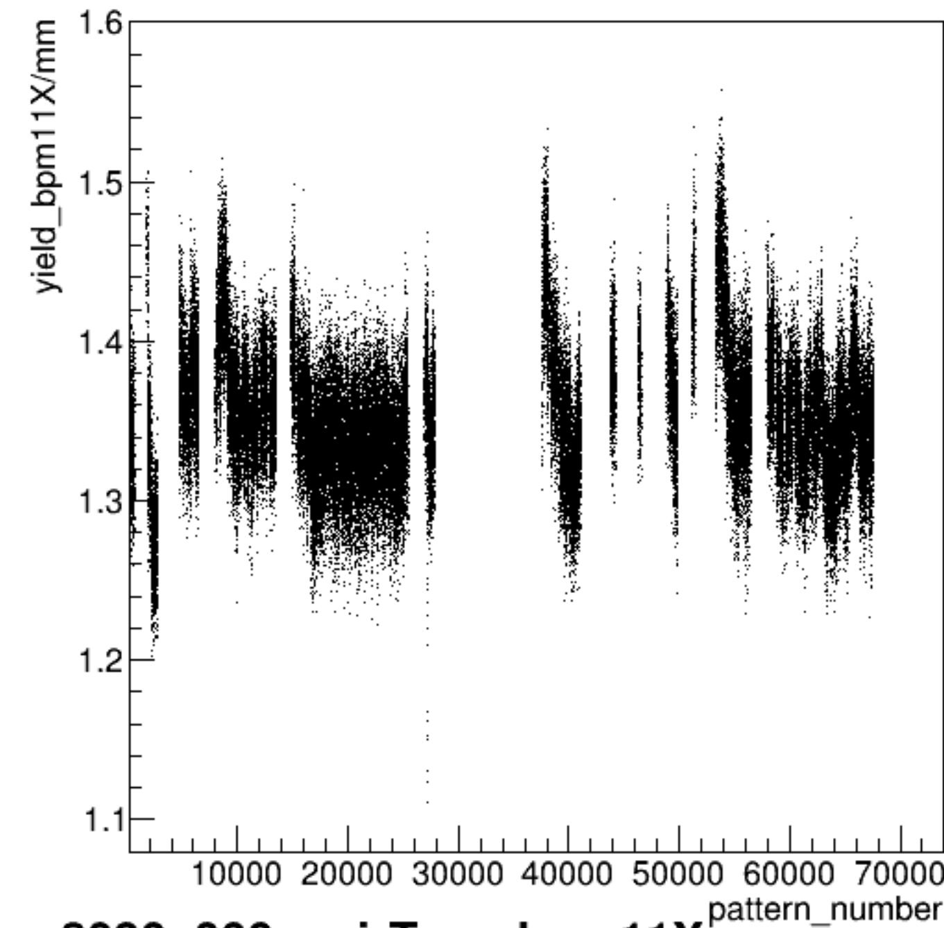
yield_bpm11X/mm:pattern_number {ErrorFlag==0}
