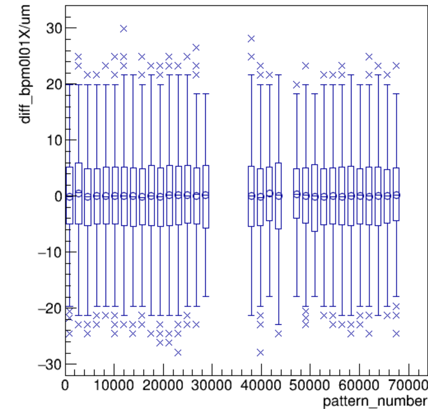
diff_bpm0l01X/um:pattern_number {ErrorFlag==0}
