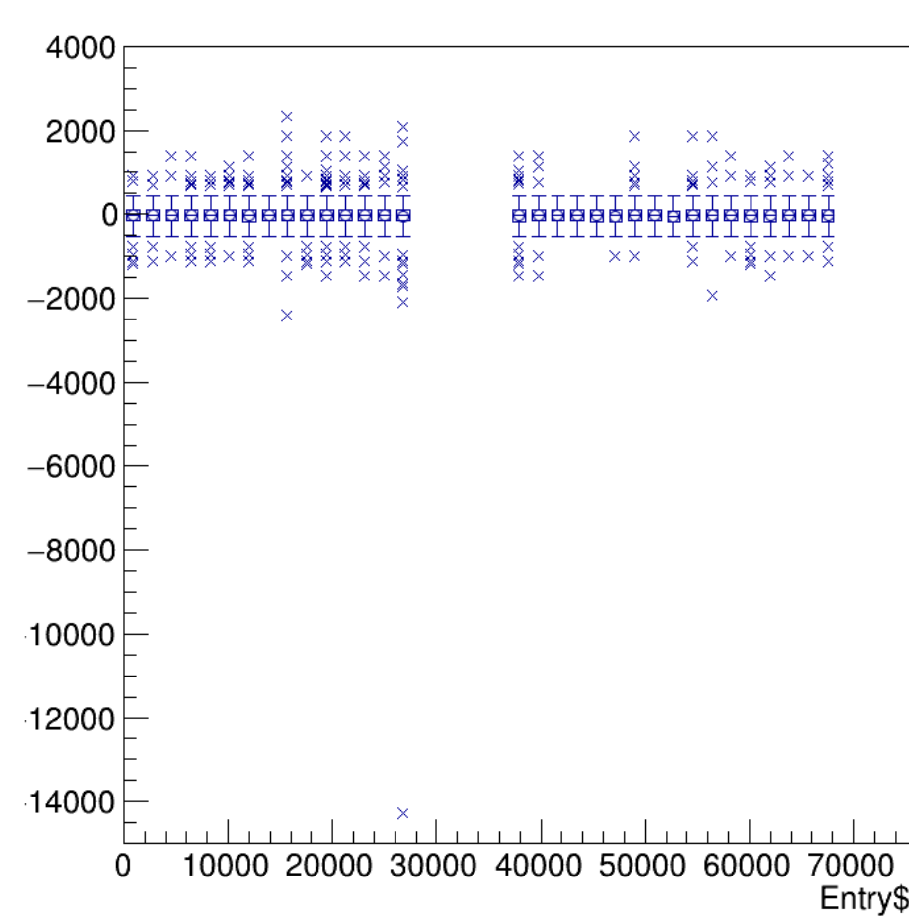
asym_bpm2i02WS/ppm:Entry$ {ErrorFlag==0}
