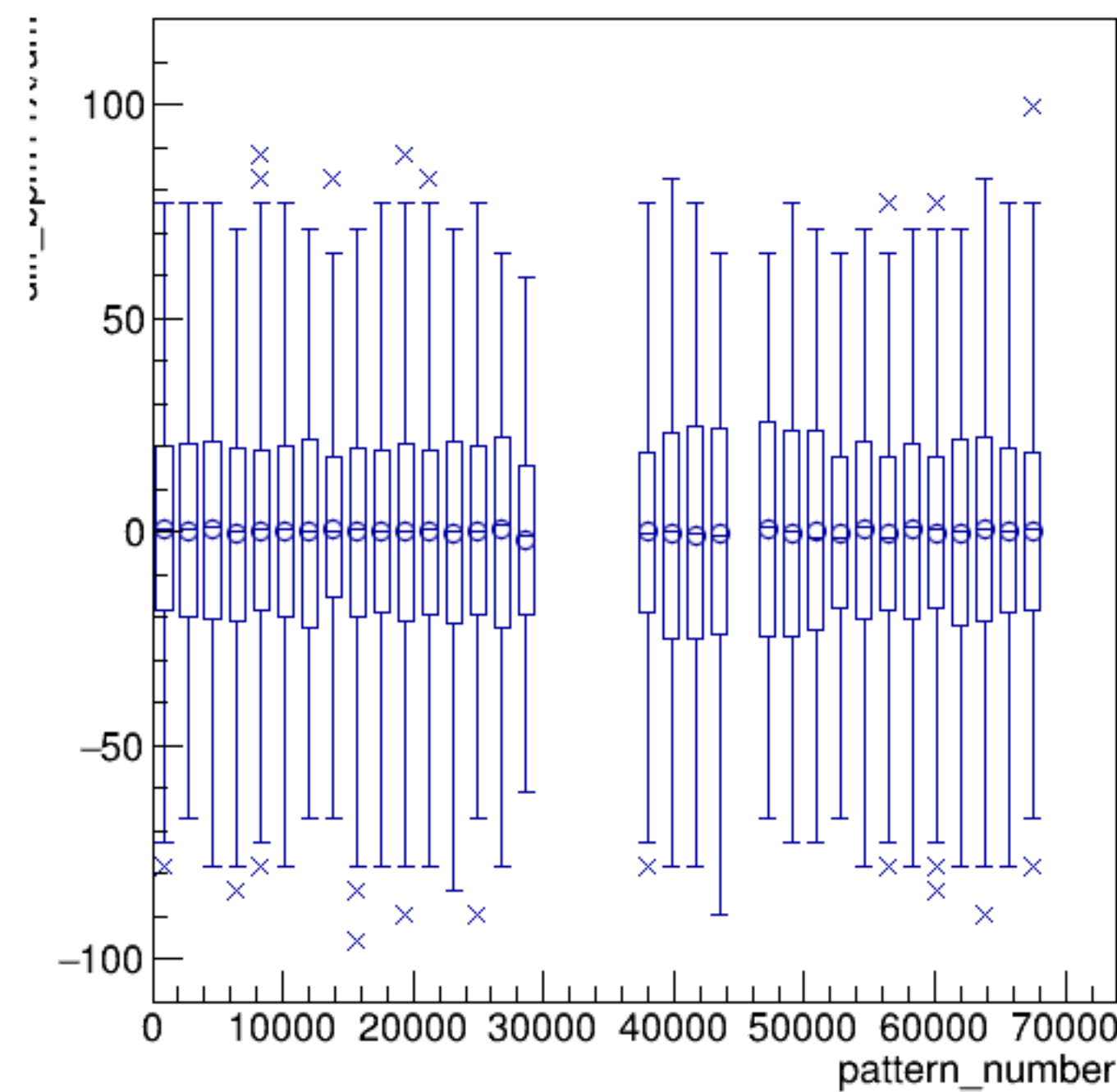
diff_bpm11X/um:pattern_number {ErrorFlag==0}
