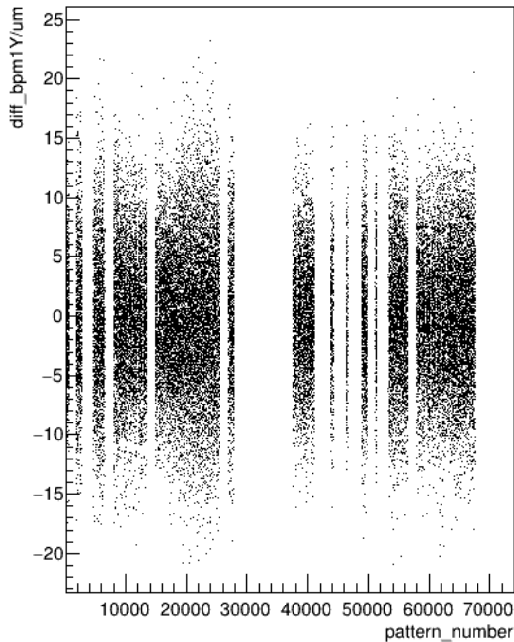
diff_bpm1Y/um:pattern_number {ErrorFlag==0}
