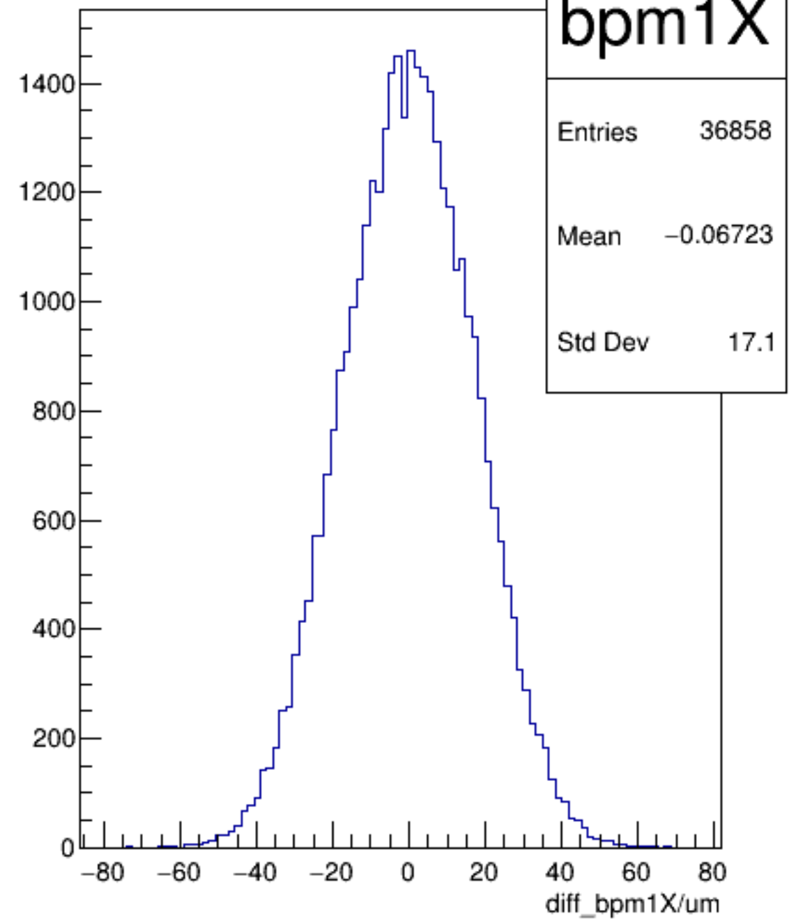
diff_bpm1X/um {ErrorFlag==0}
