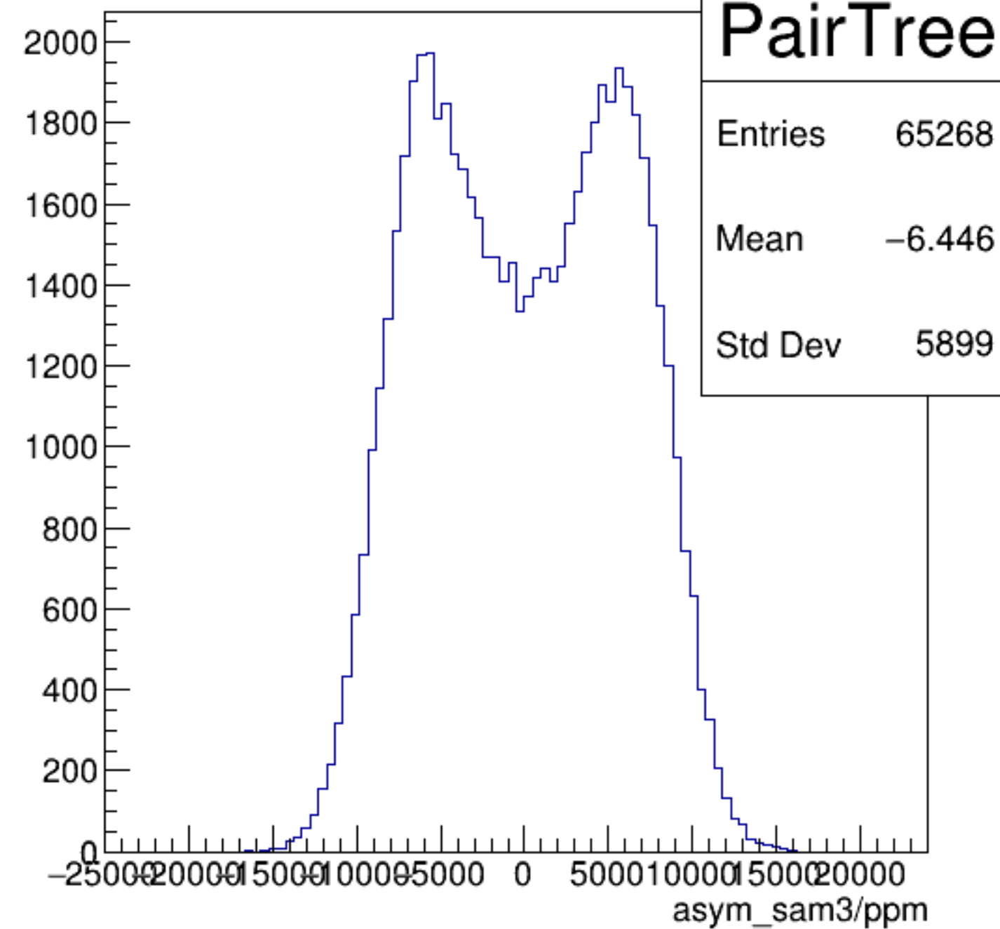
asym_sam3/ppm {ErrorFlag==0}
