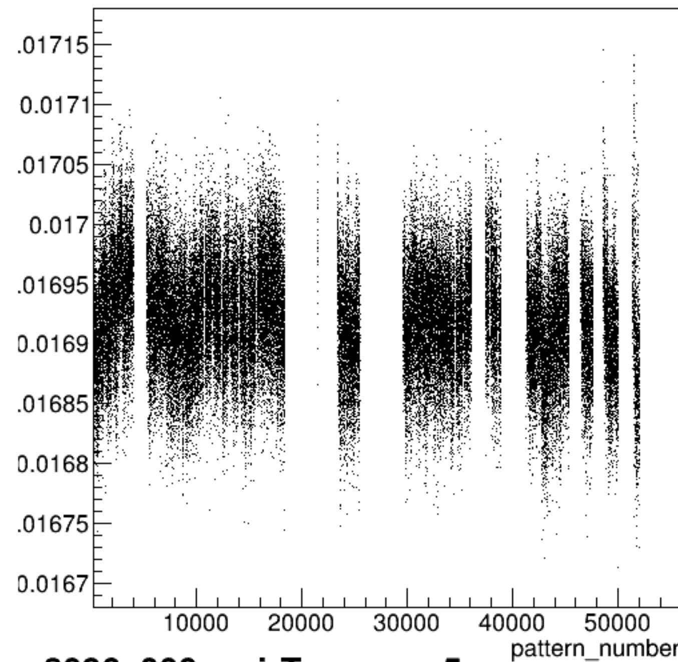
yield_sam5:pattern_number {ErrorFlag==0}
