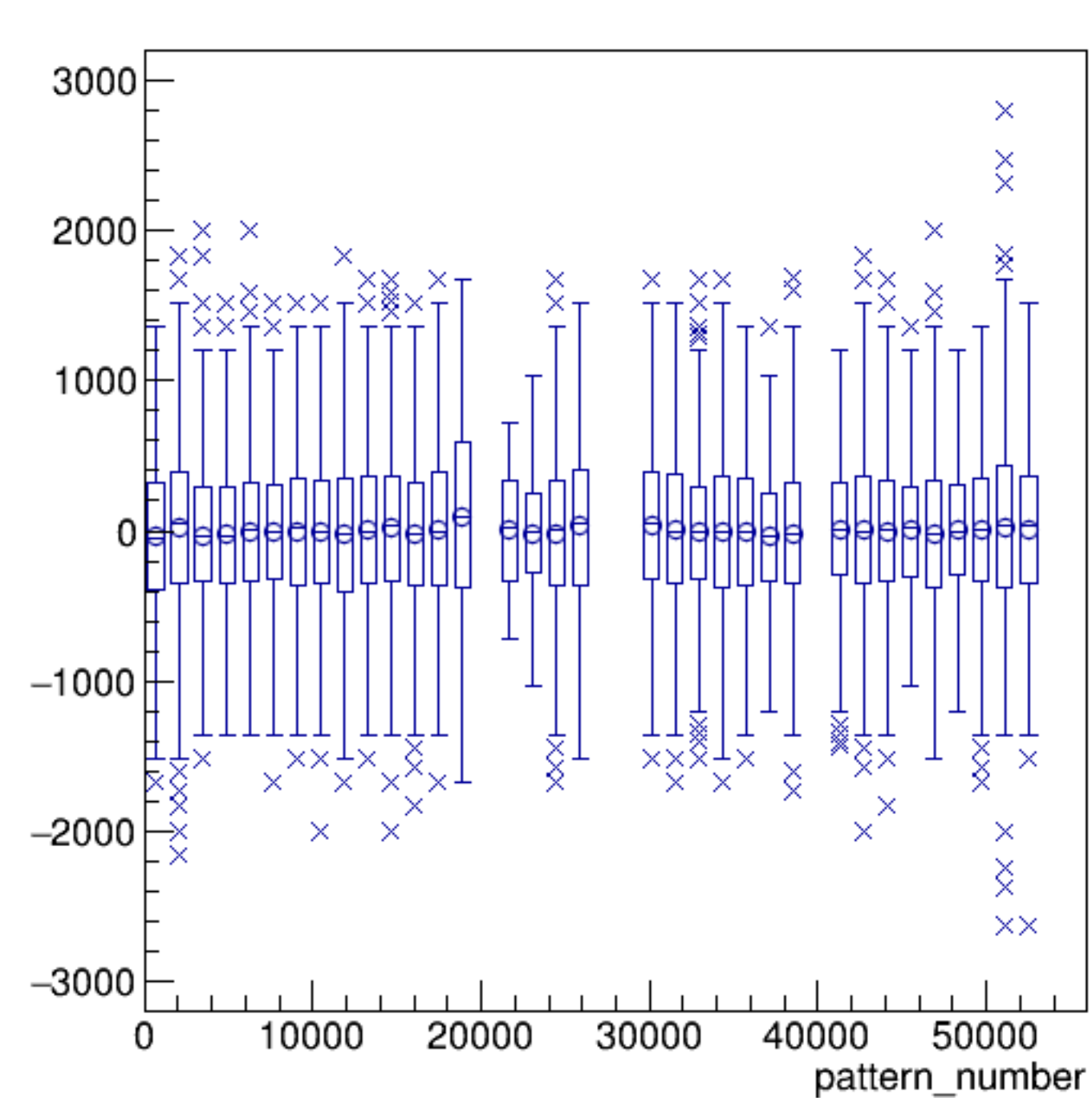
asym_sam8/ppm:pattern_number {ErrorFlag==0}
