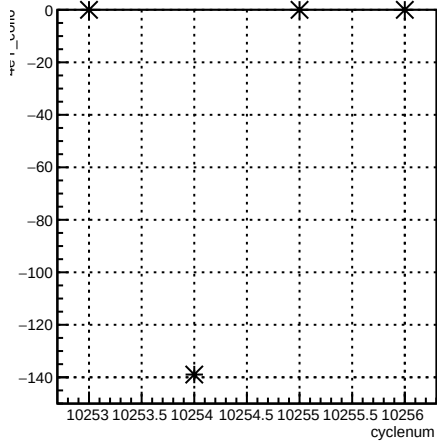
4eY_coil6:cyclenum {run == 8040}
