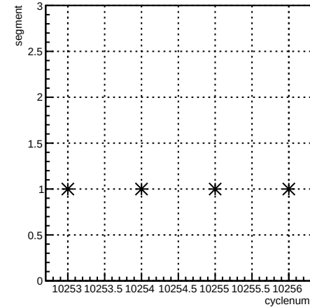
segment:cyclenum {run == 8040}
