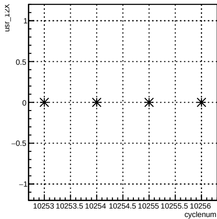
usr_12X:cyclenum {run == 8040}
