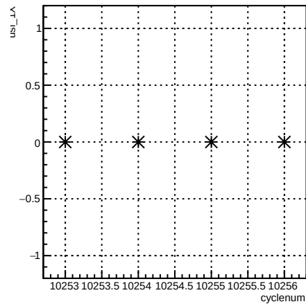
usl_4eY:cyclenum {run == 8040}
