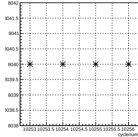
run:cyclenum {run == 8040}
