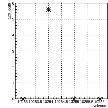
12X_coil6:cyclenum {run == 8040}
