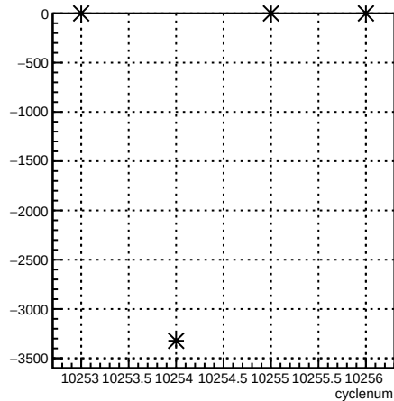
usr_coil6:cyclenum {run == 8040}
