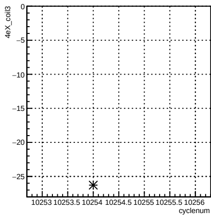
4eX_coil3:cyclenum {run == 8040}
