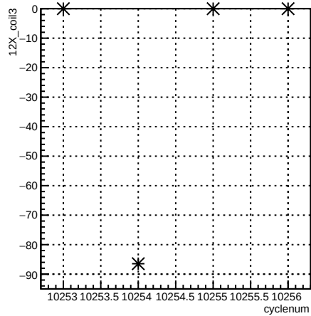
12X_coil3:cyclenum {run == 8040}
