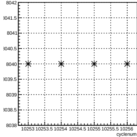
run:cyclenum {run == 8040}
