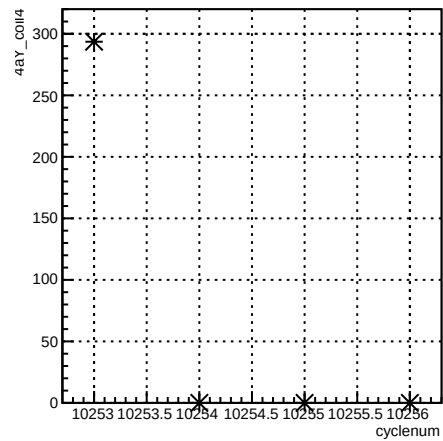
4eY_coil4:cyclenum {run == 8040}
