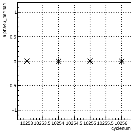
alpha46_4eY4aY:cyclenum {run == 8040}
