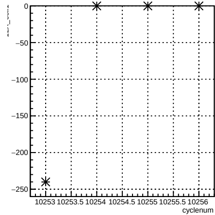
12X_coil1:cyclenum {run == 8040}
