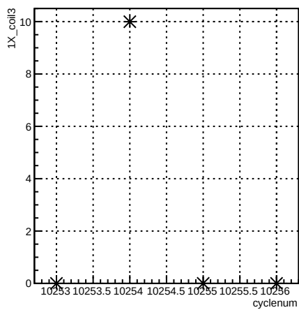
1X_coil3:cyclenum {run == 8040}
