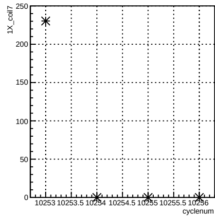
1X_coil7:cyclenum {run == 8040}
