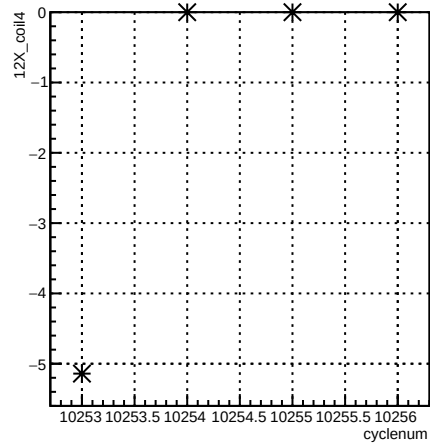
12X_coil4:cyclenum {run == 8040}
