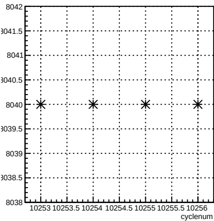
run:cyclenum {run == 8040}
