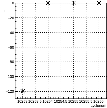
1X_coil1:cyclenum {run == 8040}
