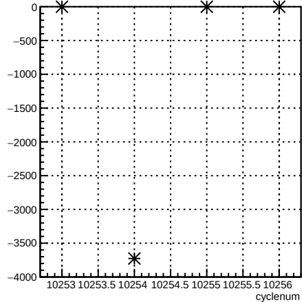
usl_coil6:cyclenum {run == 8040}
