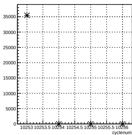
usr_coil7:cyclenum {run == 8040}
