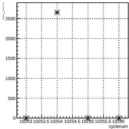
usl_coil7:cyclenum {run == 8040}
