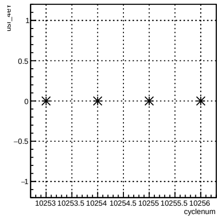
usr_4eY:cyclenum {run == 8040}
