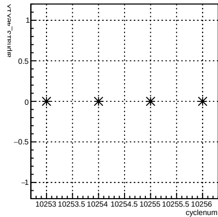
alpha13_4eX1X:cyclenum {run == 8040}
