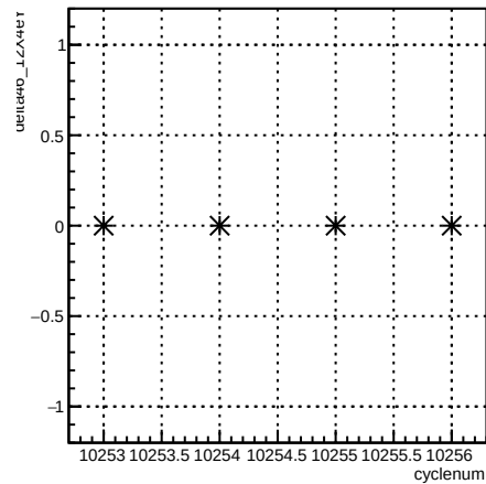
delta46_12X4eY:cyclenum {run == 8040}
