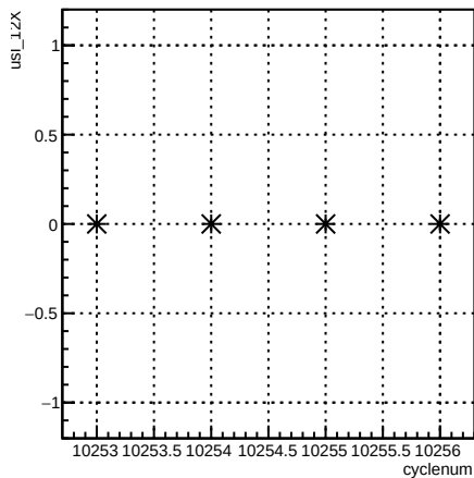
usl_12X:cyclenum {run == 8040}
