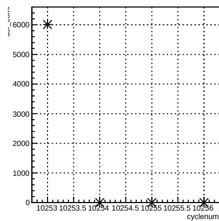
usr_coil4:cyclenum {run == 8040}
