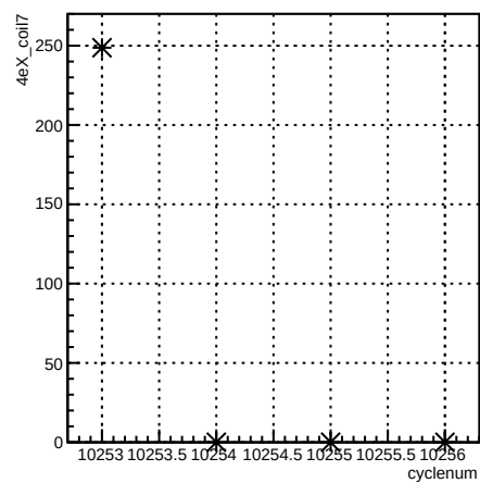
4eX_coil7:cyclenum {run == 8040}
