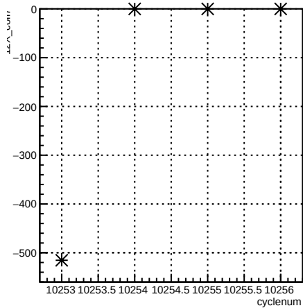
12X_coil7:cyclenum {run == 8040}
