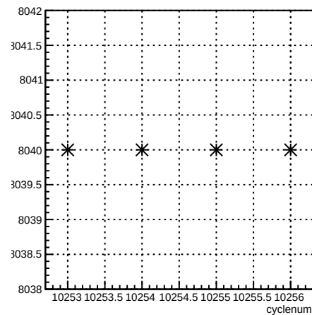
run:cyclenum {run == 8040}
