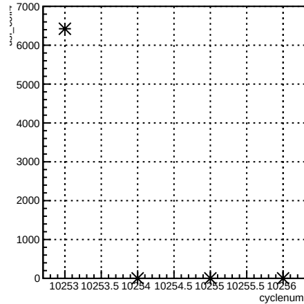
run:cyclenum {run == 8040}
