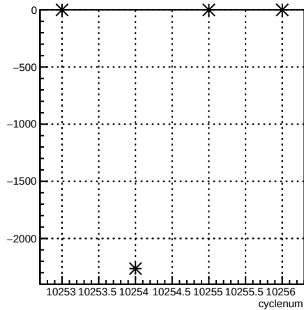
usr_coil3:cyclenum {run == 8040}
