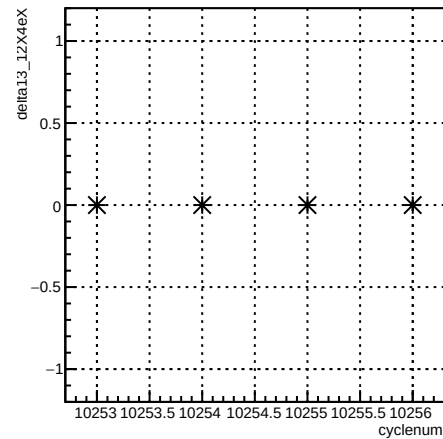
delta13_12X4eX:cyclenum {run == 8040}
