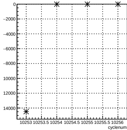
usr_coil1:cyclenum {run == 8040}
