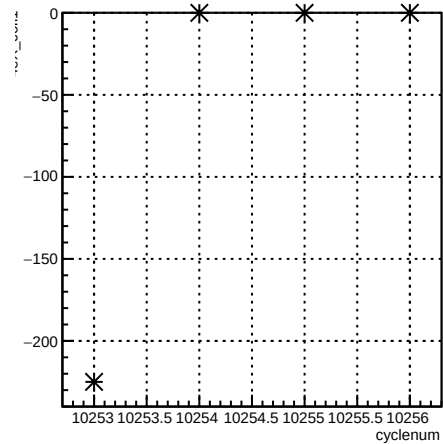
4eX_coil1:cyclenum {run == 8040}
