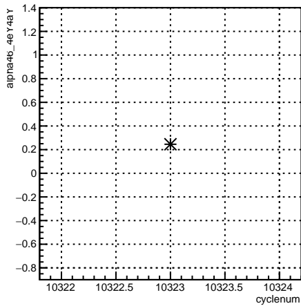
alpha46_4eY4aY:cyclenum {run == 8100}
