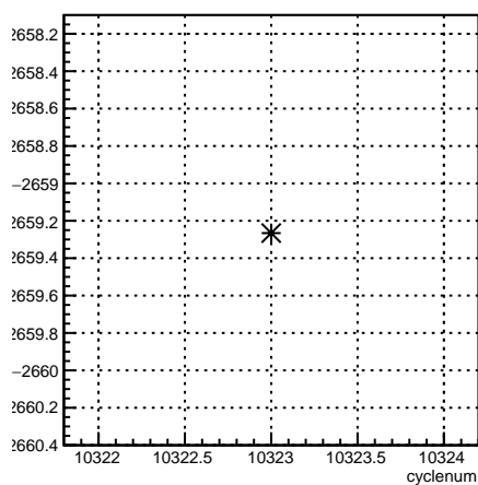
usl_coil6:cyclenum {run == 8100}
