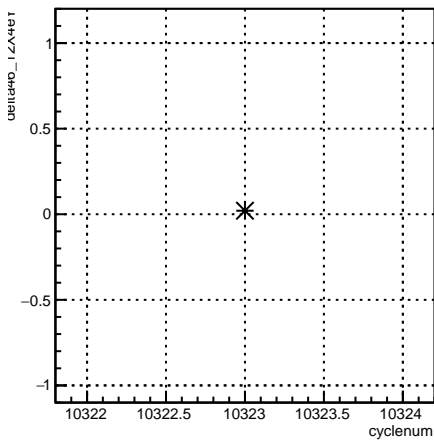
delta46_12X4eY:cyclenum {run == 8100}
