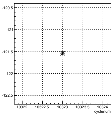
4aY_coil6:cyclenum {run == 8100}
