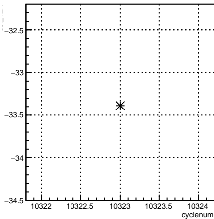
usl_12X:cyclenum {run == 8100}
