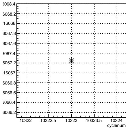
usl_coil1:cyclenum {run == 8100}
