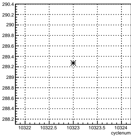
4aY_coil4:cyclenum {run == 8100}
