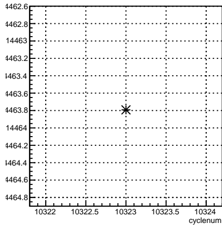
usr_coil1:cyclenum {run == 8100}
