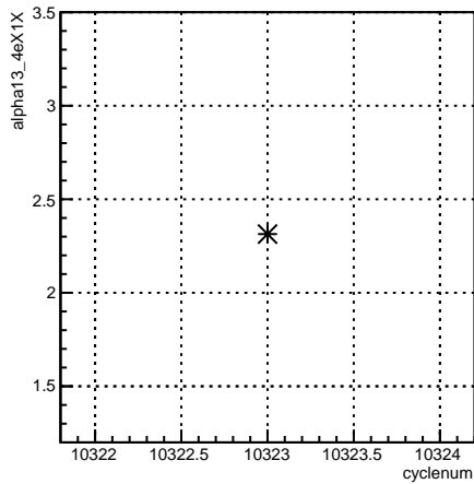
alpha13_4eX1X:cyclenum {run == 8100}
