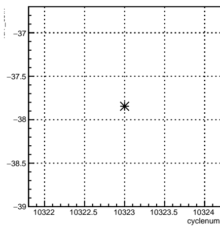
4aY_coil7:cyclenum {run == 8100}
