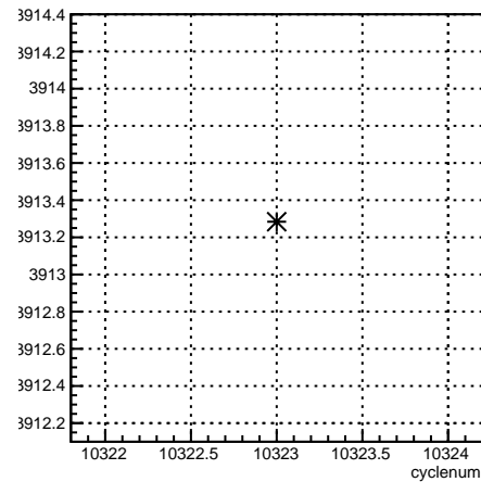
usl_coil4:cyclenum {run == 8100}
