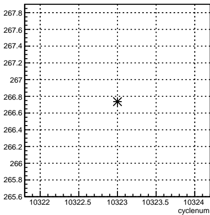
4eY_coil4:cyclenum {run == 8100}
