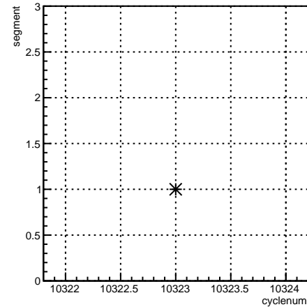
segment:cyclenum {run == 8100}
