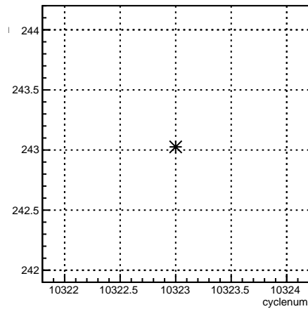
4eX_coil7:cyclenum {run == 8100}
