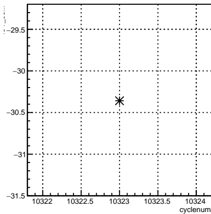
4eY_coil7:cyclenum {run == 8100}
