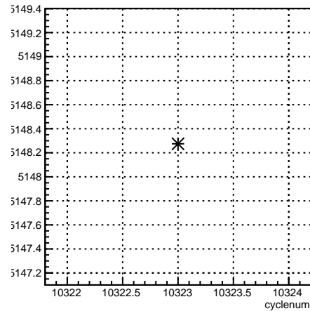
usr_coil4:cyclenum {run == 8100}
