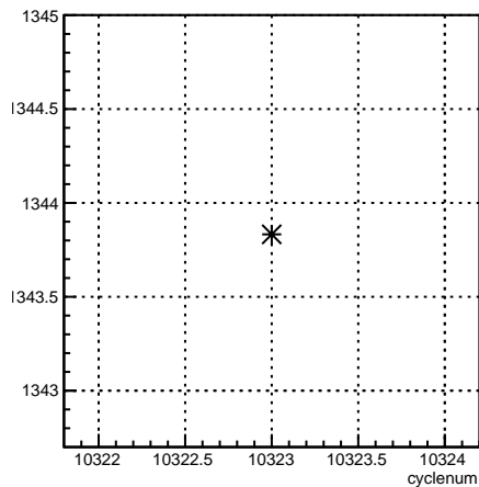
usl_coil7:cyclenum {run == 8100}
