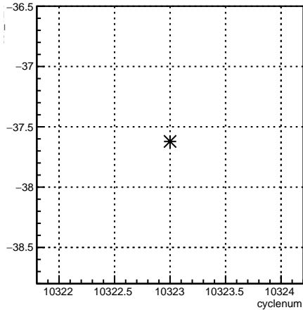
usr_12X:cyclenum {run == 8100}
