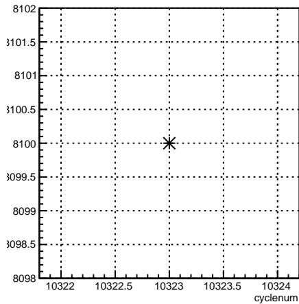
run:cyclenum {run == 8100}
