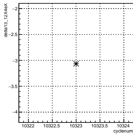
delta13_12X4eX:cyclenum {run == 8100}
