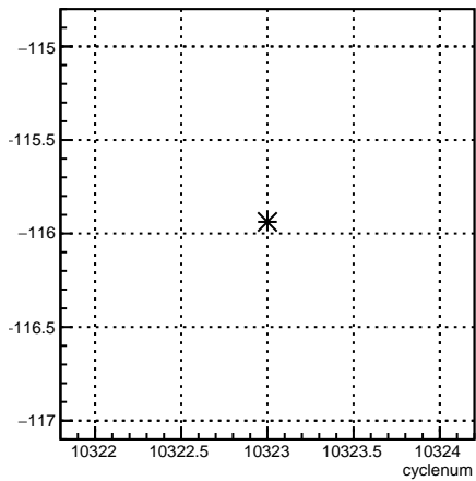
usr_4eY:cyclenum {run == 8100}
