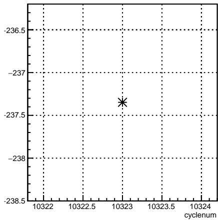
12X_coil6:cyclenum {run == 8100}
