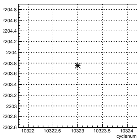
usl_coil3:cyclenum {run == 8100}
