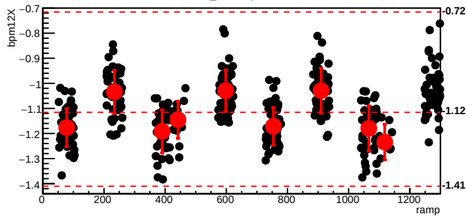
bmod_trim2,cyc=10327
