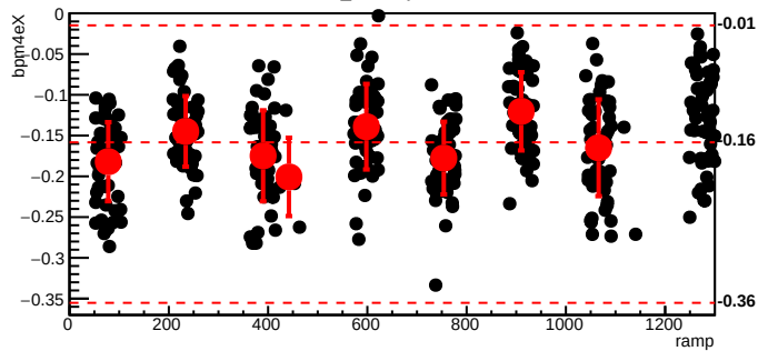
bmod_trim6,cyc=10327
