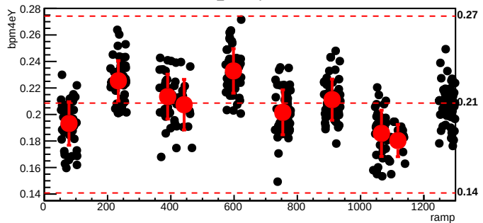
bmod_trim3,cyc=10327
