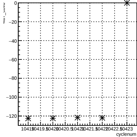
4eY_coil6:cyclenum {run == 8125}
