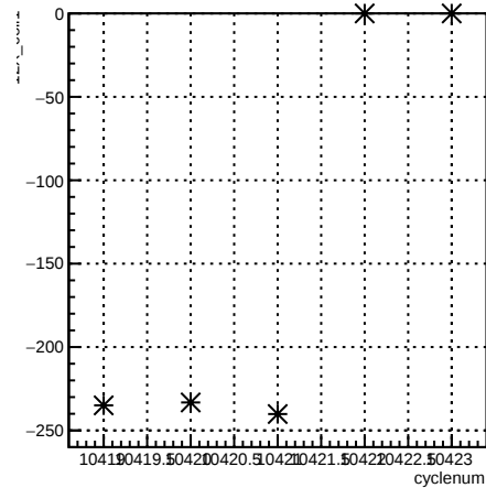
12X_coil1:cyclenum {run == 8125}
