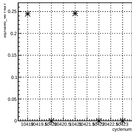
alpha46_4eY4aY:cyclenum {run == 8125}
