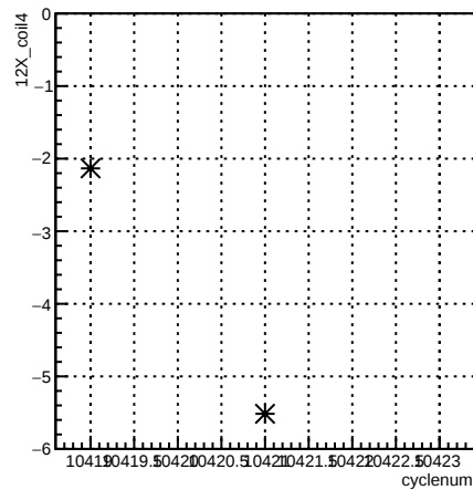
12X_coil4:cyclenum {run == 8125}
