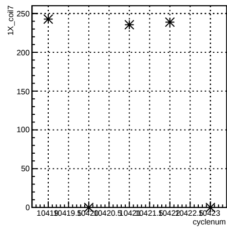
1X_coil7:cyclenum {run == 8125}
