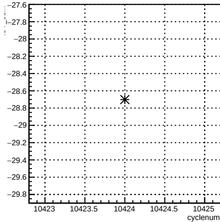
4eY_coil7:cyclenum {run == 8126}
