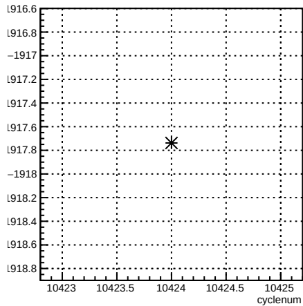
usr_coil3:cyclenum {run == 8126}
