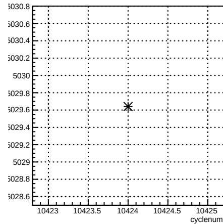
usr_coil4:cyclenum {run == 8126}
