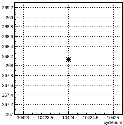
4eY_coil4:cyclenum {run == 8126}
