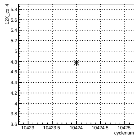
12X_coil4:cyclenum {run == 8126}
