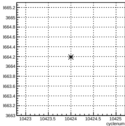
usl_coil7:cyclenum {run == 8126}
