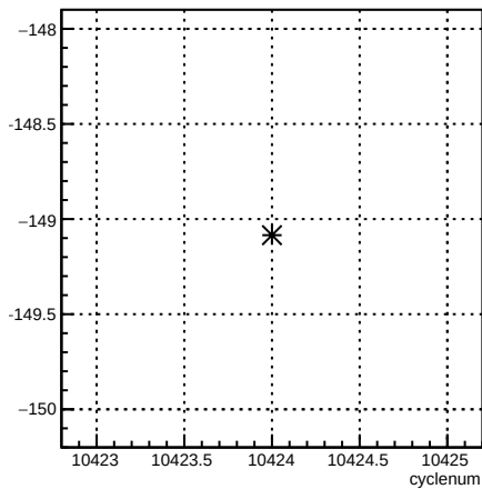
4eY_coil6:cyclenum {run == 8126}
