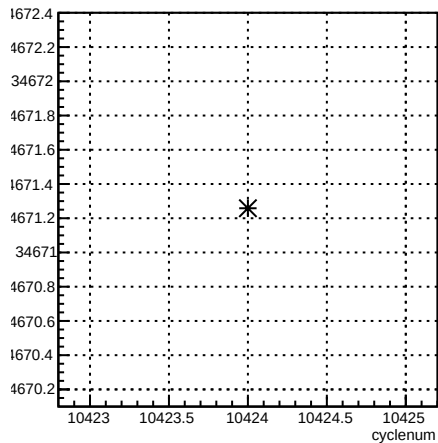
usr_coil7:cyclenum {run == 8126}
