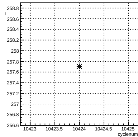
4eX_coil7:cyclenum {run == 8126}
