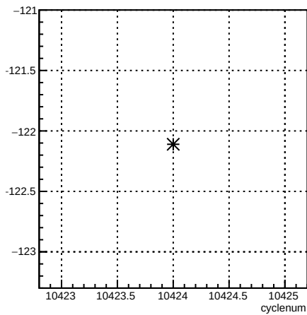
4aY_coil6:cyclenum {run == 8126}
