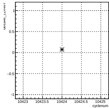
delta46_12X4eY:cyclenum {run == 8126}
