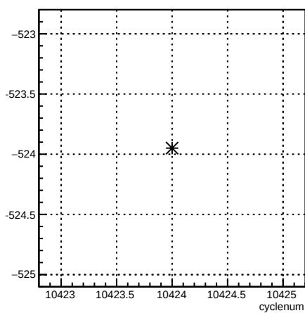
12X_coil7:cyclenum {run == 8126}
