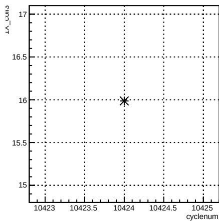
1X_coil3:cyclenum {run == 8126}
