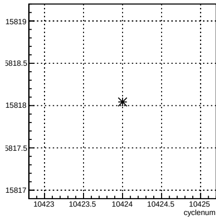
usl_coil6:cyclenum {run == 8126}
