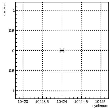
usr_4eY:cyclenum {run == 8126}
