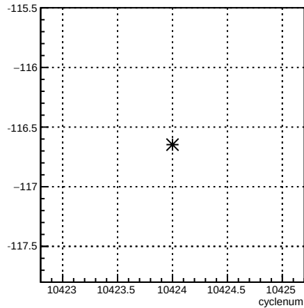
1X_coil1:cyclenum {run == 8126}
