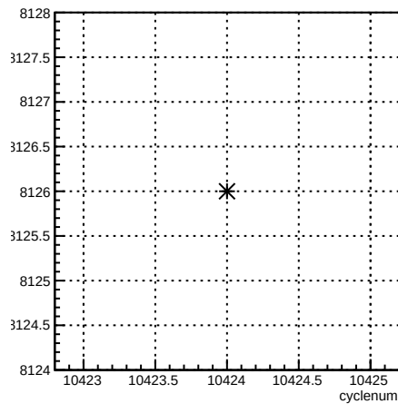
run:cyclenum {run == 8126}
