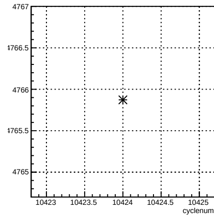
usl_coil4:cyclenum {run == 8126}
