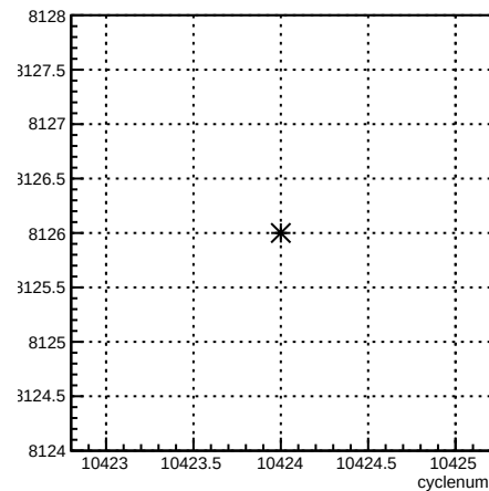
run:cyclenum {run == 8126}
