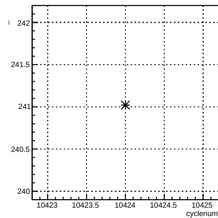
1X_coil7:cyclenum {run == 8126}
