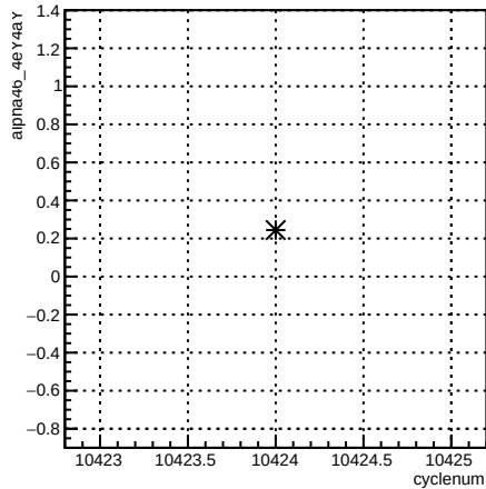
alpha46_4eY4aY:cyclenum {run == 8126}
