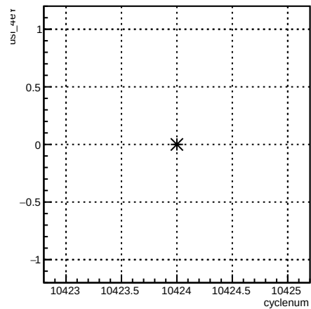
usl_4eY:cyclenum {run == 8126}
