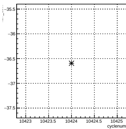
4aY_coil7:cyclenum {run == 8126}
