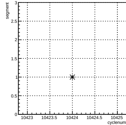
segment:cyclenum {run == 8126}
