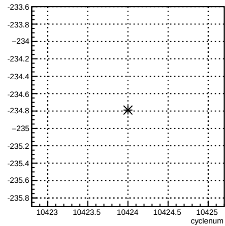
12X_coil1:cyclenum {run == 8126}
