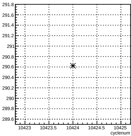
4aY_coil4:cyclenum {run == 8126}
