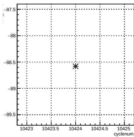
12X_coil3:cyclenum {run == 8126}
