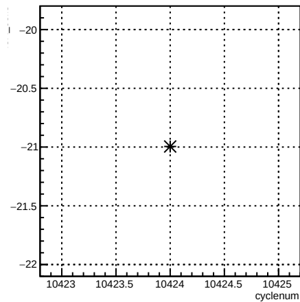
4eX_coil3:cyclenum {run == 8126}
