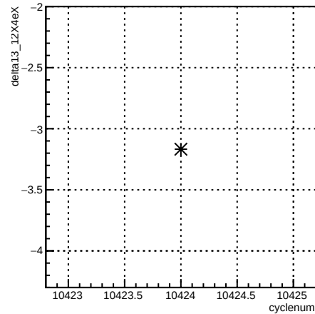
delta13_12X4eX:cyclenum {run == 8126}
