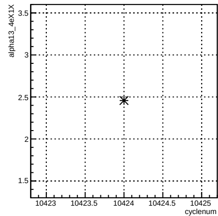
alpha13_4eX1X:cyclenum {run == 8126}
