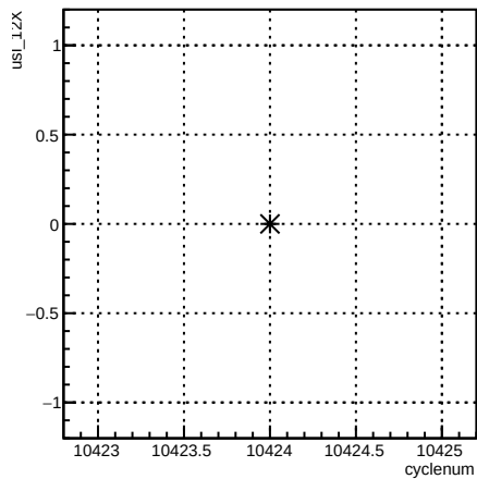
usl_12X:cyclenum {run == 8126}
