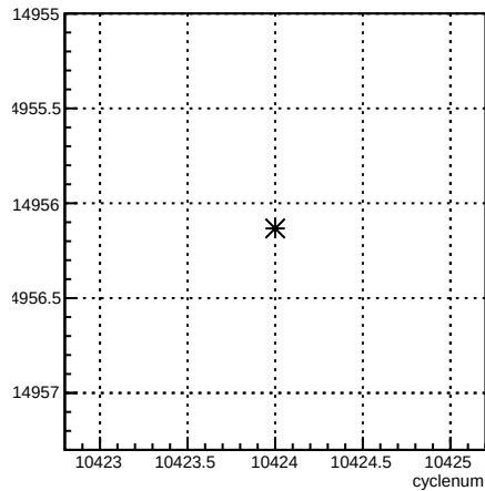
usr_coil1:cyclenum {run == 8126}
