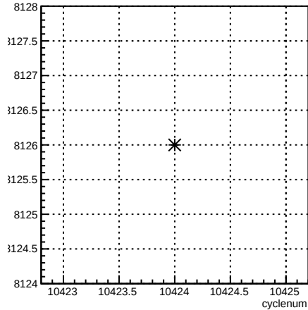
run:cyclenum {run == 8126}
