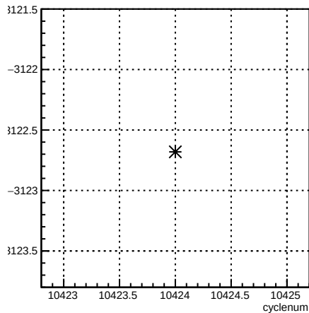
usr_coil6:cyclenum {run == 8126}
