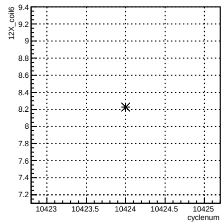
12X_coil6:cyclenum {run == 8126}
