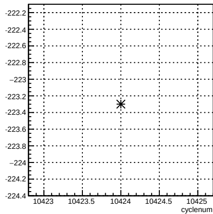
4eX_coil1:cyclenum {run == 8126}
