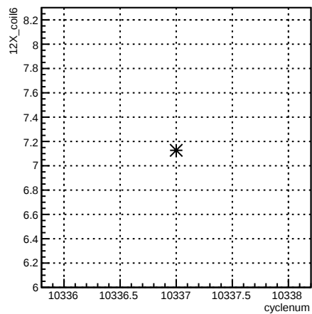
12X_coil6:cyclenum {run == 8103}
