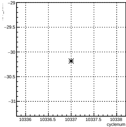
4eY_coil7:cyclenum {run == 8103}
