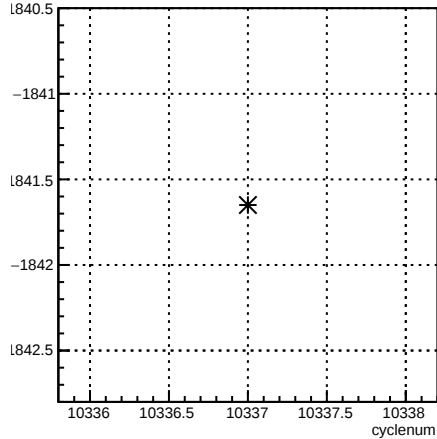
usr_coil3:cyclenum {run == 8103}
