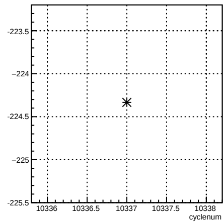
4eX_coil1:cyclenum {run == 8103}
