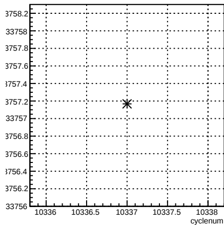
usr_coil7:cyclenum {run == 8103}
