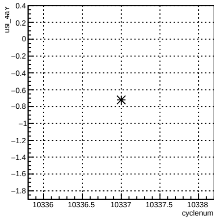
usl_4aY:cyclenum {run == 8103}
