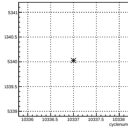
usr_coil4:cyclenum {run == 8103}
