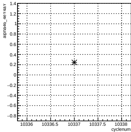
alpha46_4eY4aY:cyclenum {run == 8103}
