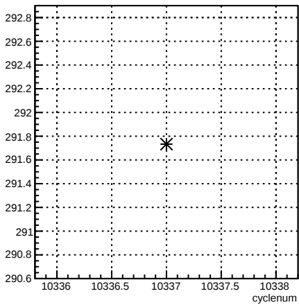
4eY_coil4:cyclenum {run == 8103}
