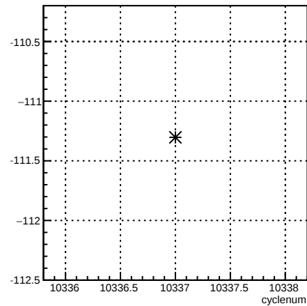
usr_4eY:cyclenum {run == 8103}
