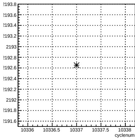
usl_coil3:cyclenum {run == 8103}
