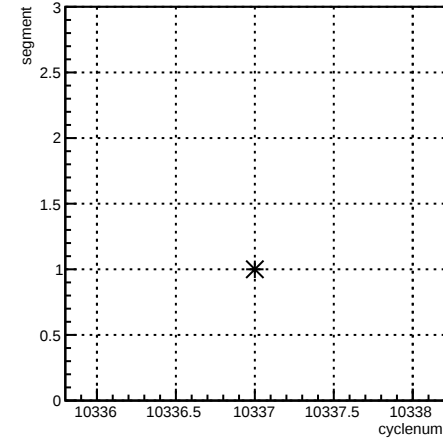
segment:cyclenum {run == 8103}
