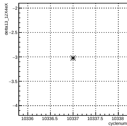
delta13_12X4eX:cyclenum {run == 8103}
