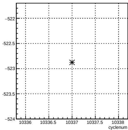
12X_coil7:cyclenum {run == 8103}
