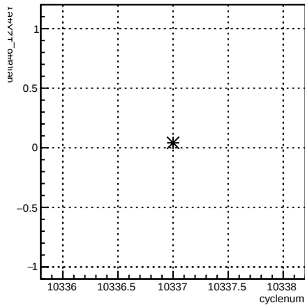
delta46_12X4eY:cyclenum {run == 8103}
