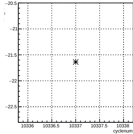
4eX_coil3:cyclenum {run == 8103}
