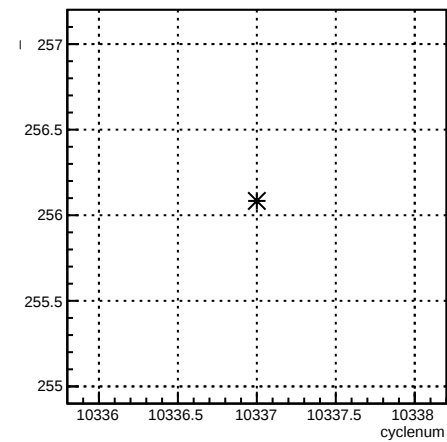
4eX_coil7:cyclenum {run == 8103}
