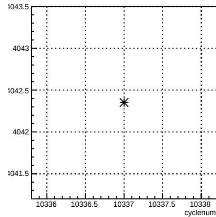
usl_coil4:cyclenum {run == 8103}
