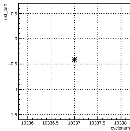
usl_4eX:cyclenum {run == 8103}
