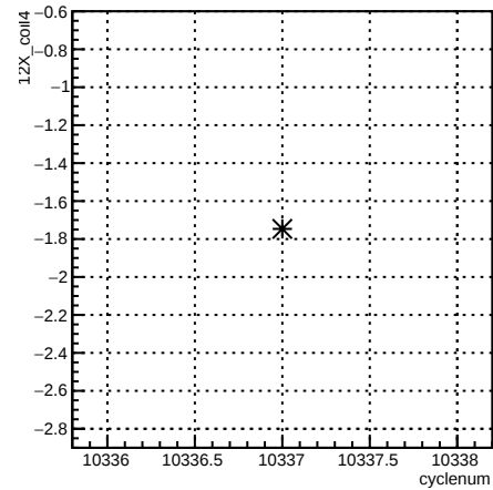
12X_coil4:cyclenum {run == 8103}
