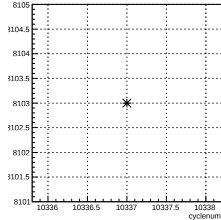
run:cyclenum {run == 8103}
