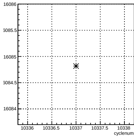
usl_coil1:cyclenum {run == 8103}
