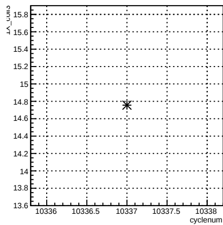
1X_coil3:cyclenum {run == 8103}
