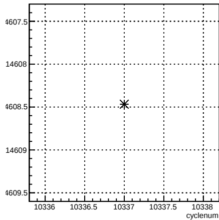
usr_coil1:cyclenum {run == 8103}
