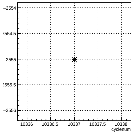
usl_coil6:cyclenum {run == 8103}
