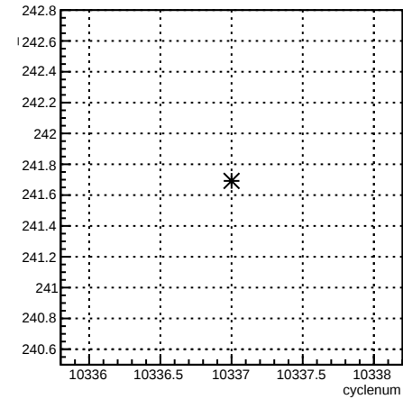
1X_coil7:cyclenum {run == 8103}
