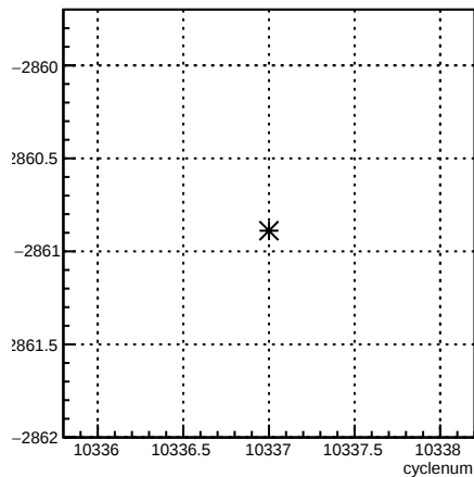
usr_coil6:cyclenum {run == 8103}
