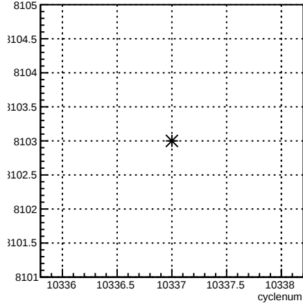
run:cyclenum {run == 8103}
