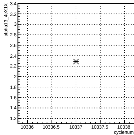
alpha13_4eX1X:cyclenum {run == 8103}
