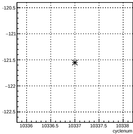
4eY_coil6:cyclenum {run == 8103}
