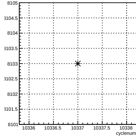
run:cyclenum {run == 8103}
