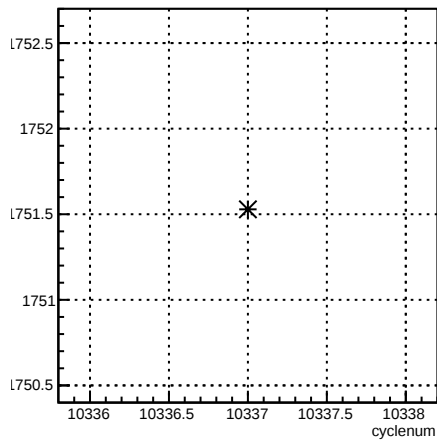
usl_coil7:cyclenum {run == 8103}
