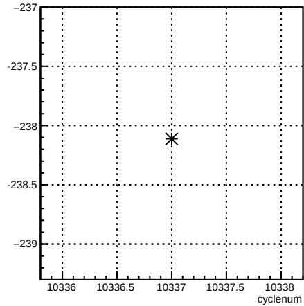
12X_coil1:cyclenum {run == 8103}
