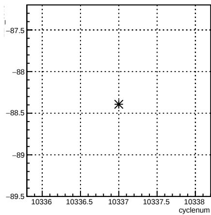
12X_coil3:cyclenum {run == 8103}
