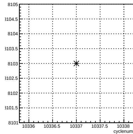
run:cyclenum {run == 8103}
