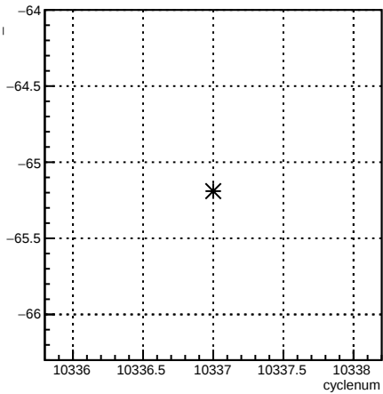
usl_1X:cyclenum {run == 8103}
