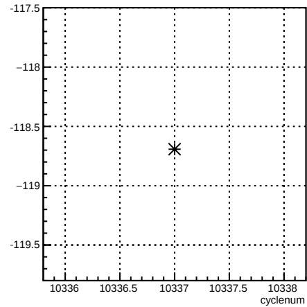
1X_coil1:cyclenum {run == 8103}
