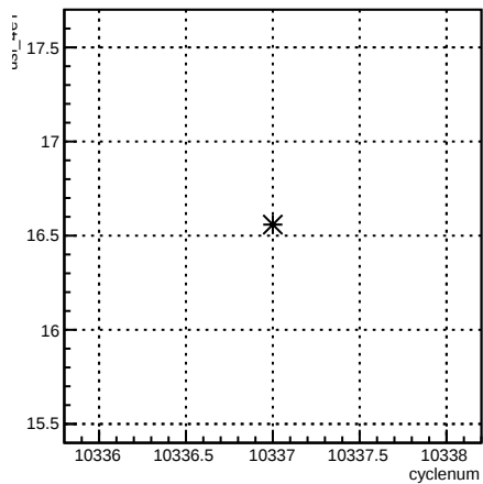
usl_4eY:cyclenum {run == 8103}
