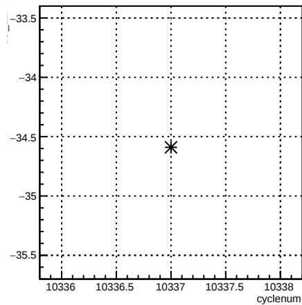
usl_12X:cyclenum {run == 8103}
