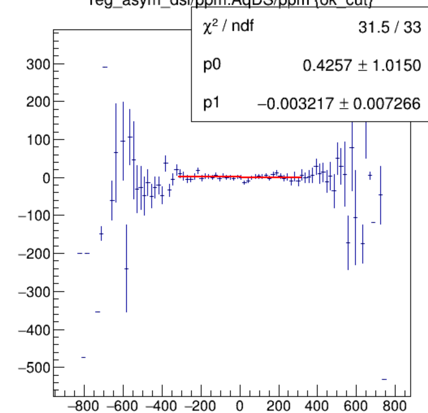
reg_asym_dsl/ppm:AqDS/ppm {ok_cut}
