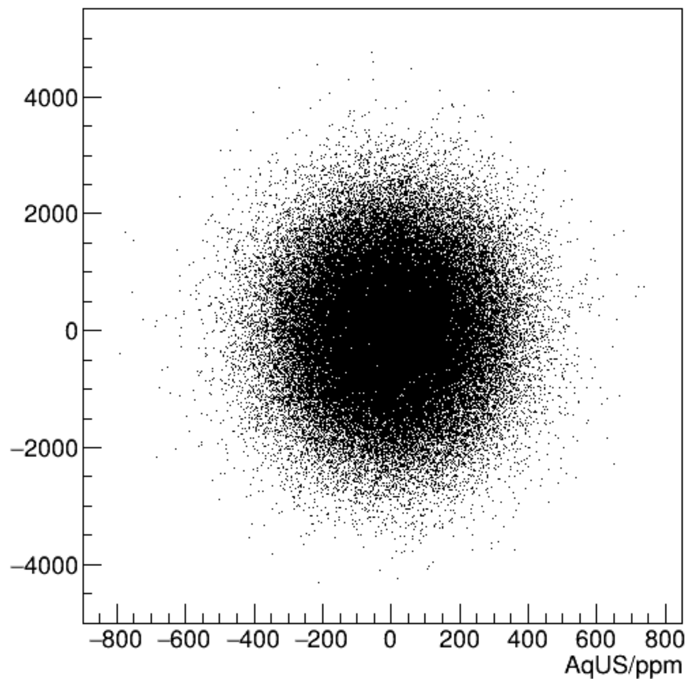
reg_asym_usl/ppm:AqUS/ppm {ok_cut}
