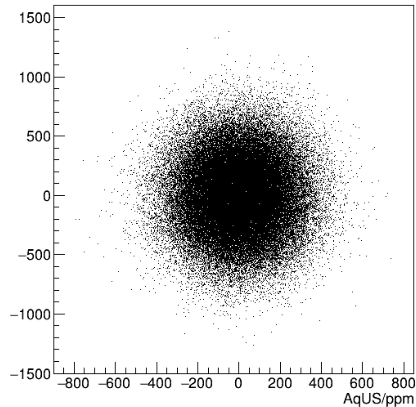
reg_asym_dsl/ppm:AqUS/ppm {ok_cut}
