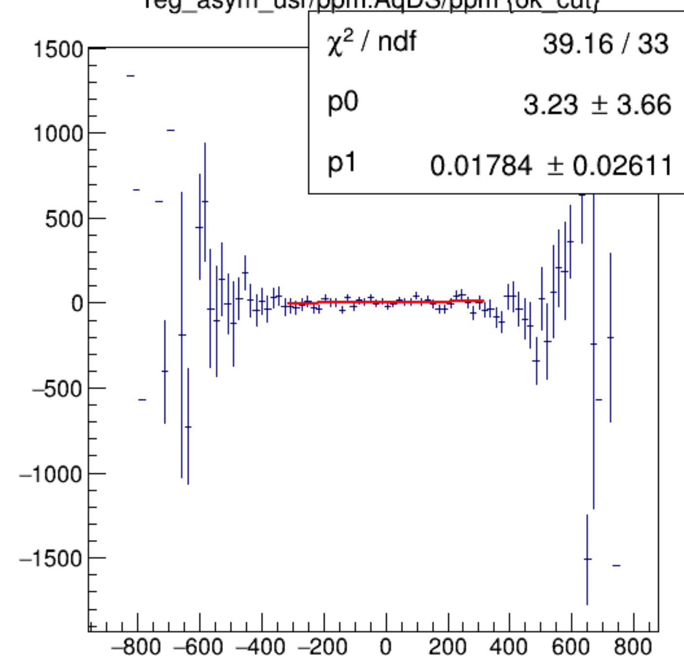
reg_asym_usr/ppm:AqDS/ppm {ok_cut}
