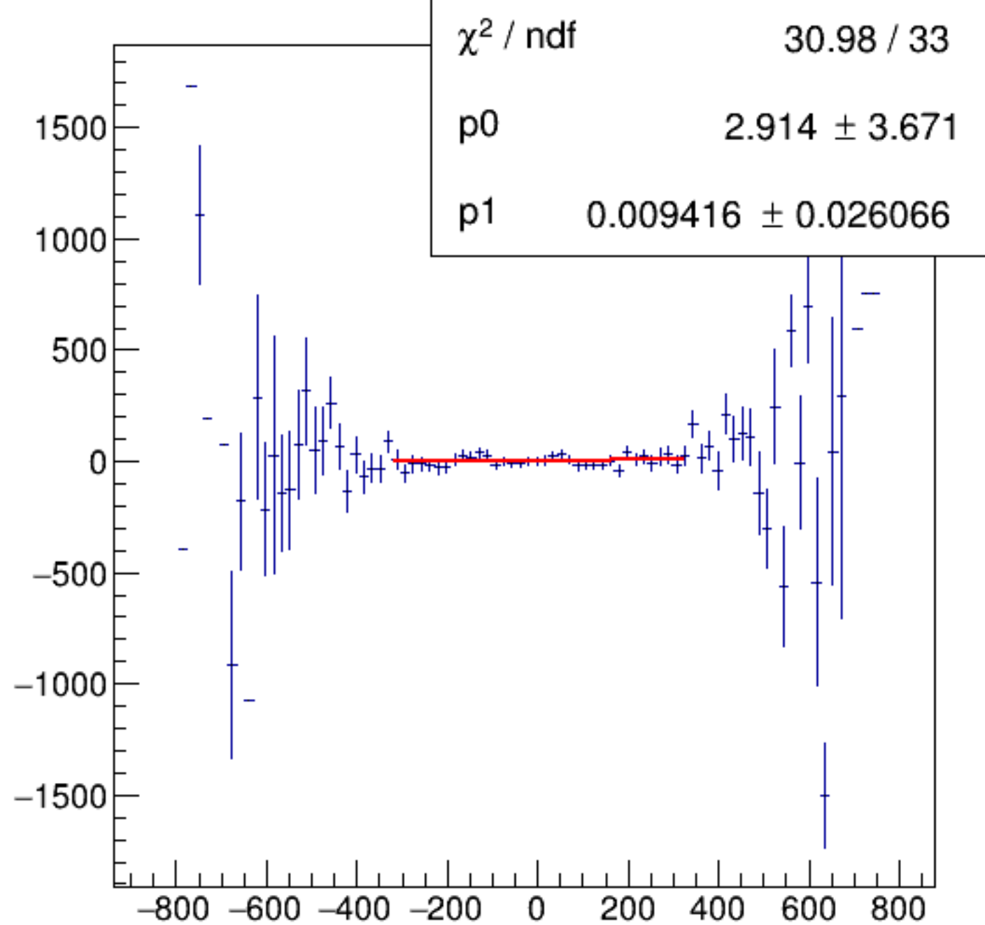
reg_asym_usl/ppm:AqUS/ppm {ok_cut}
