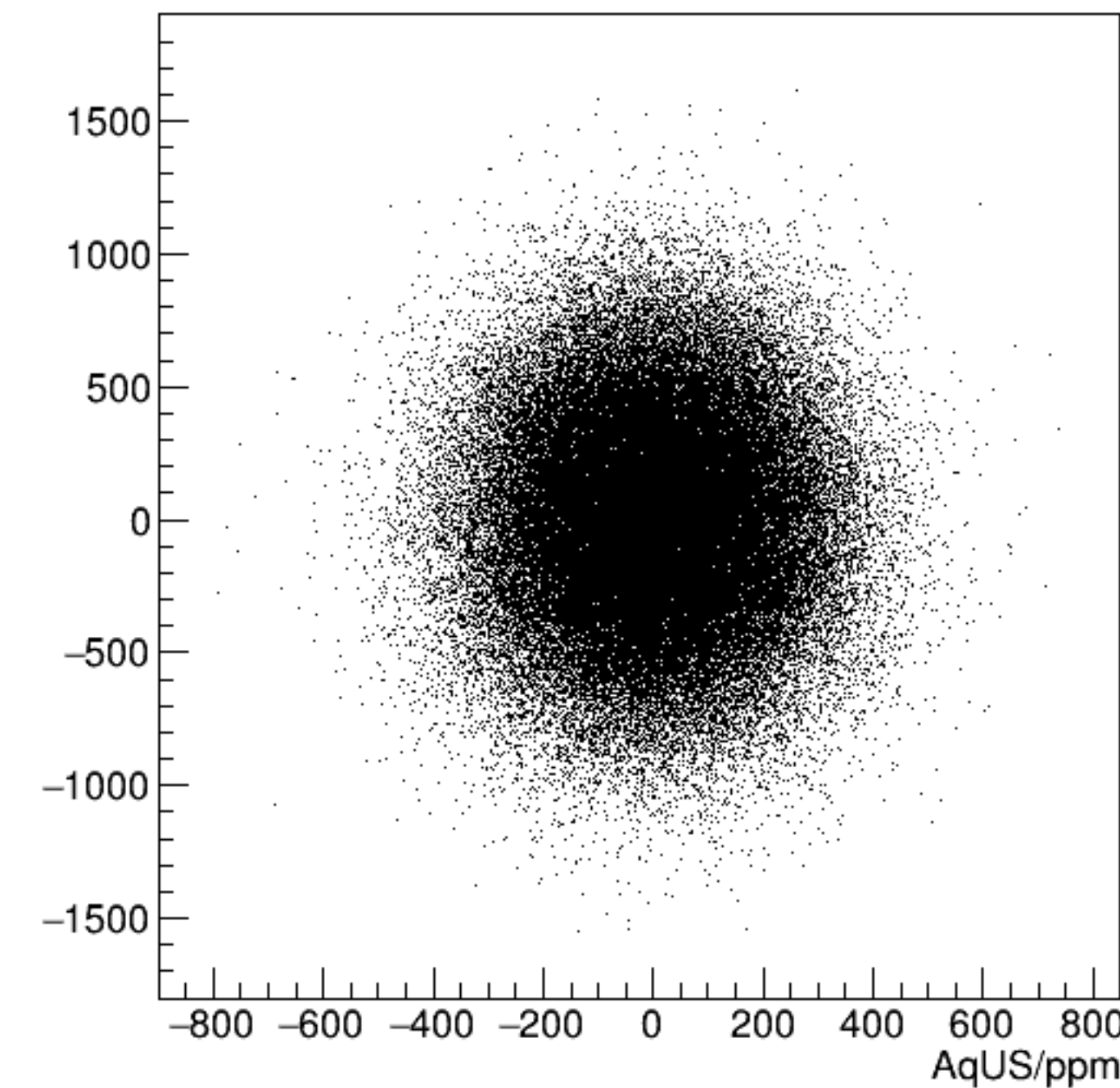
reg_asym_dsr/ppm:AqUS/ppm {ok_cut}
