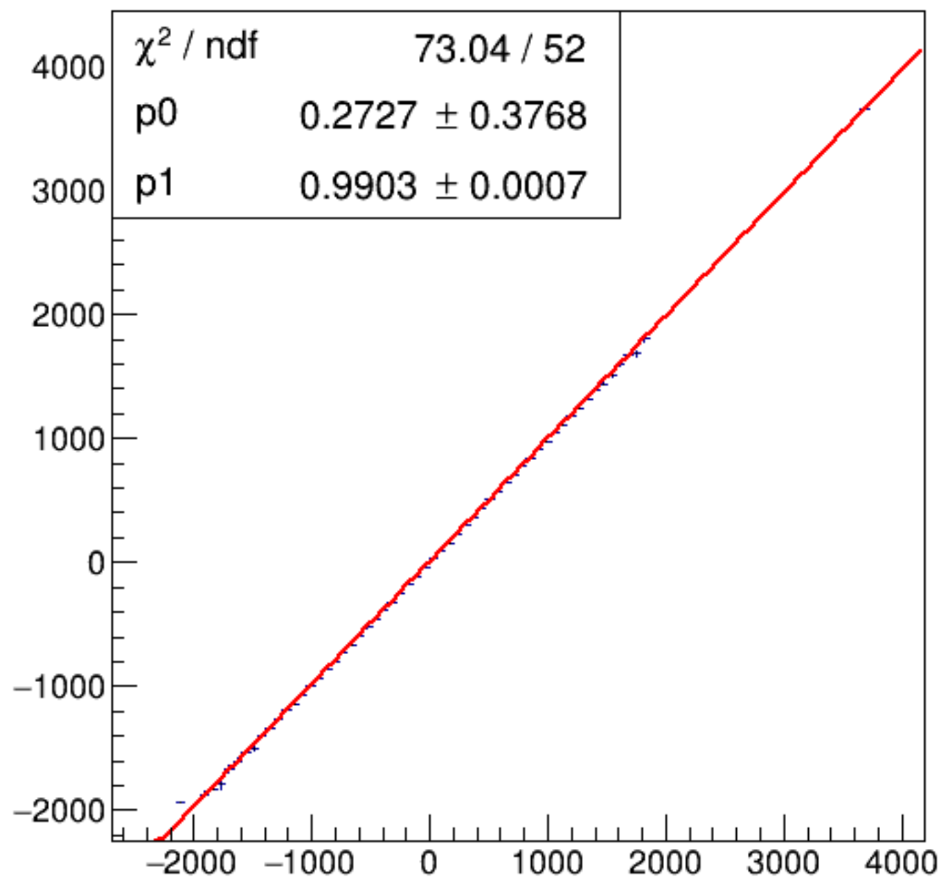
run8109_000_asym_bcm_dg_us_vs_asym_bcm_an_ds3_pr.png
