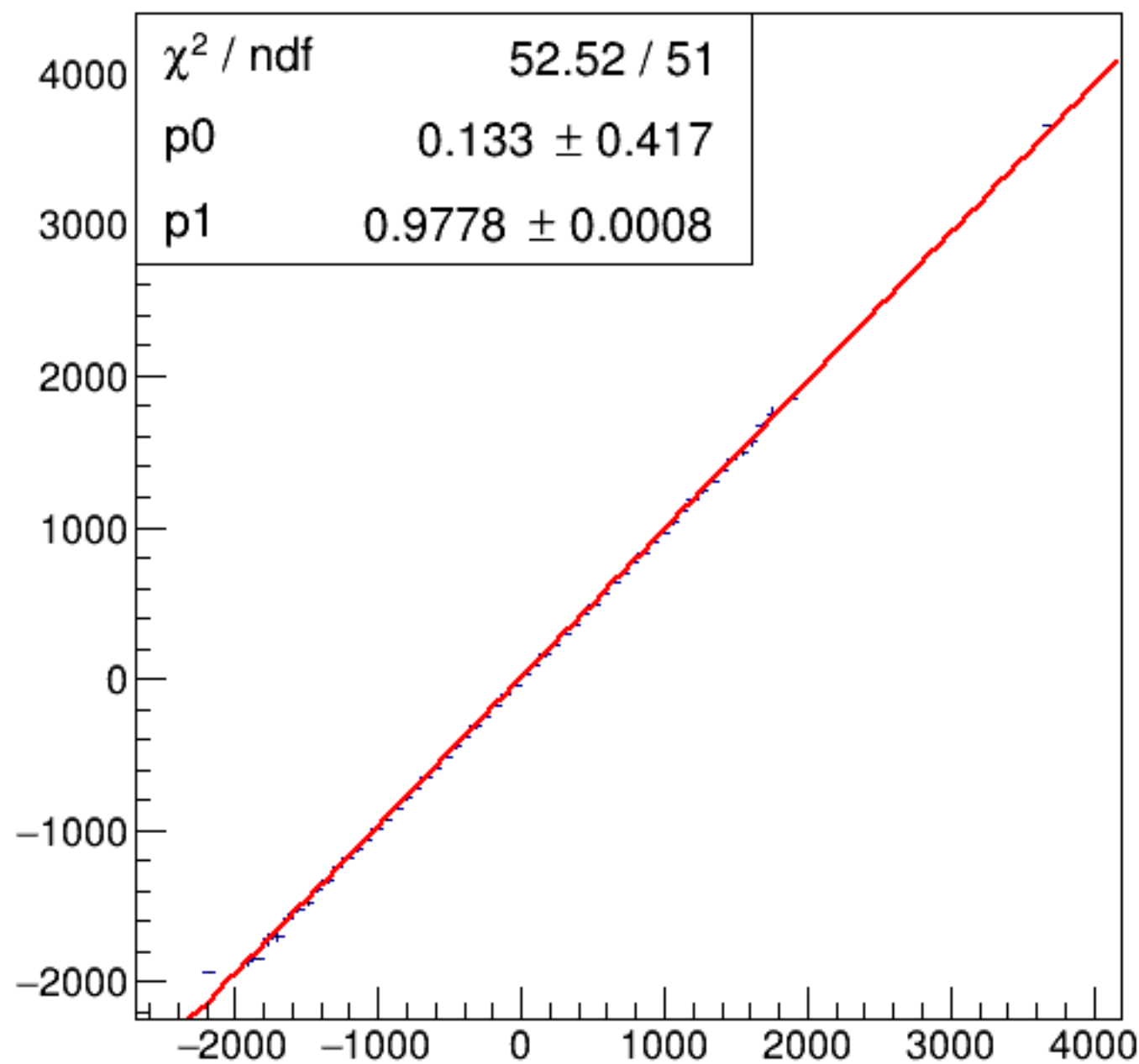
run8109_000_asym_bcm_dg_us_vs_asym_bcm_dg_ds_pr.png
