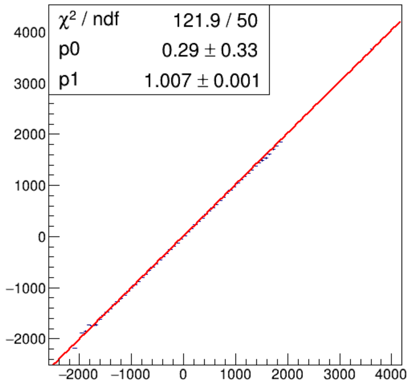
run8109_000_asym_bcm_dg_ds_vs_asym_bcm_an_us_pr.png
