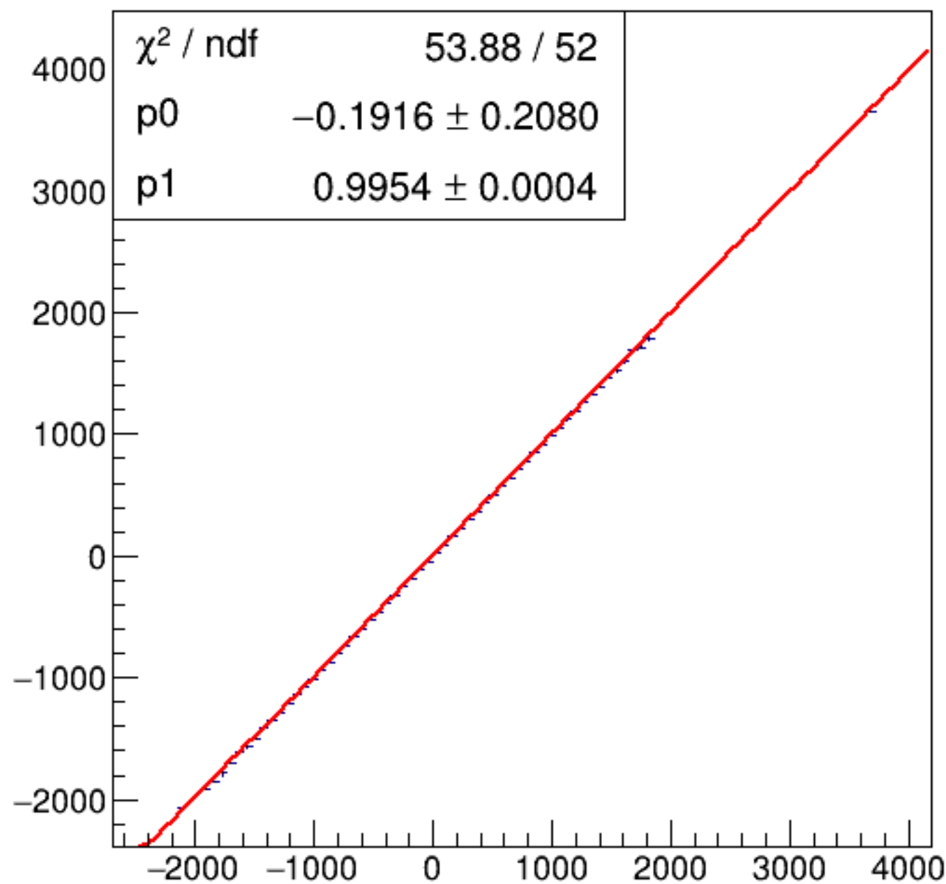
run8109_000_asym_bcm_an_us_vs_asym_bcm_an_ds3_pr.png
