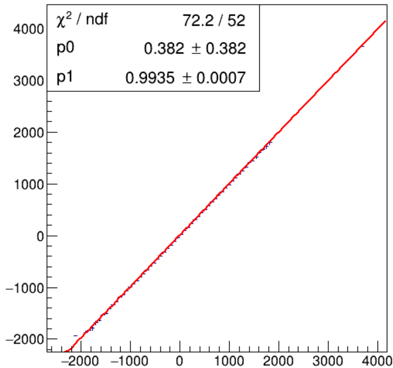
run8109_000_asym_bcm_dg_us_vs_asym_bcm_an_ds_pr.png
