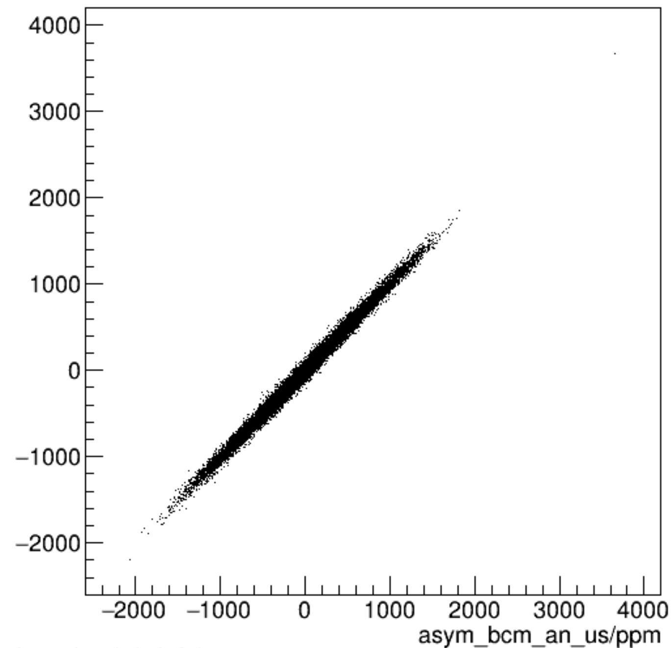
run8109_000_asym_bcm_dg_ds_vs_asym_bcm_an_us_pr.png
