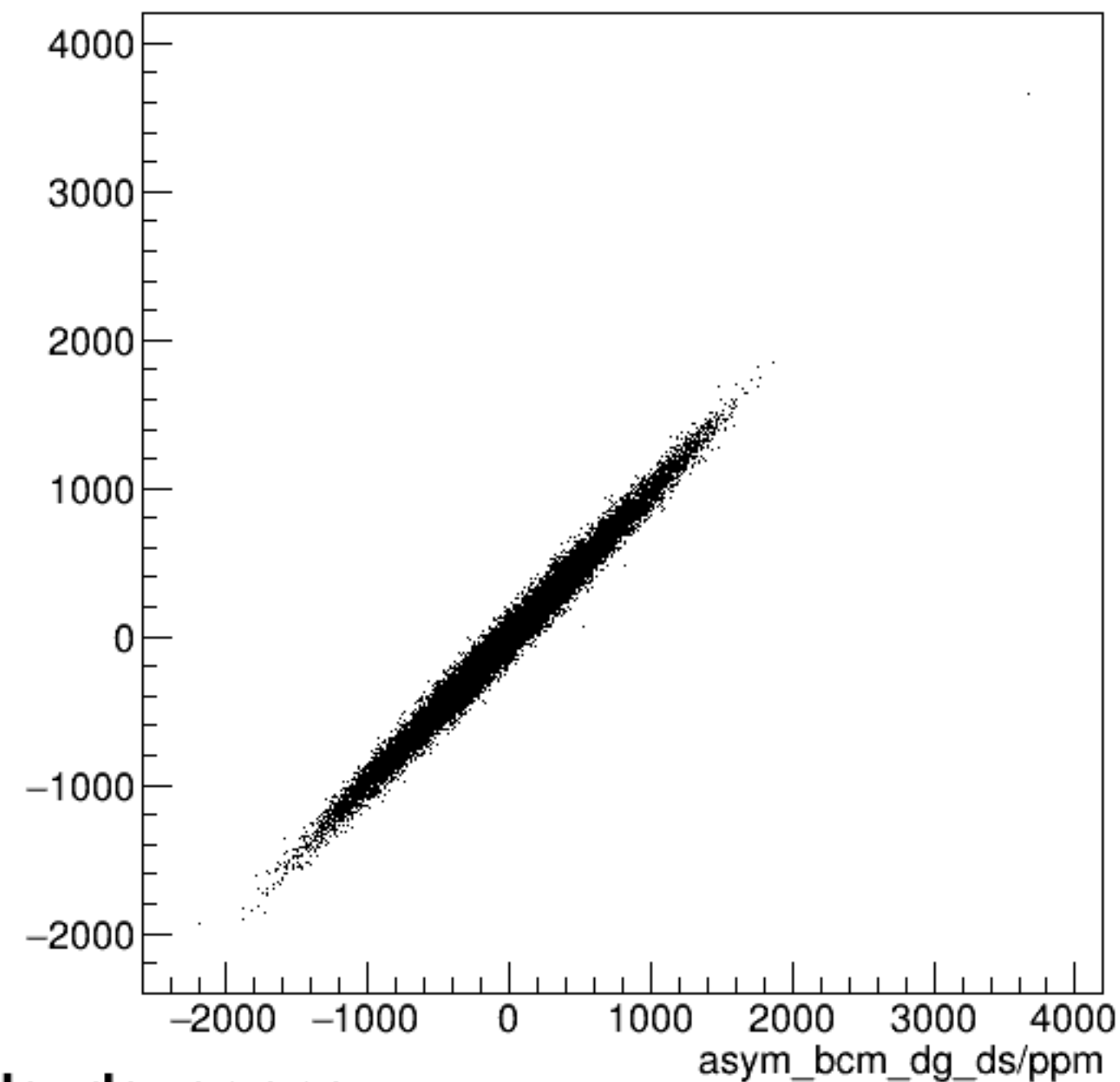
run8109_000_asym_bcm_dg_us_vs_asym_bcm_dg_ds_pr.png
