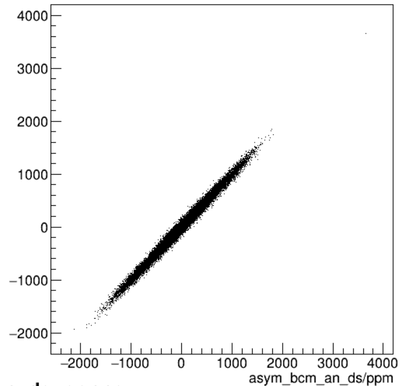
run8109_000_asym_bcm_dg_us_vs_asym_bcm_an_ds_pr.png
