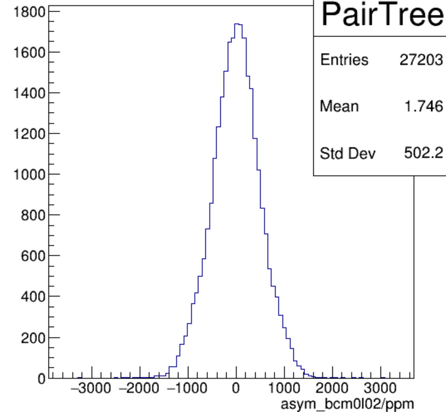
asym_bcm0l02/ppm {ErrorFlag==0}
