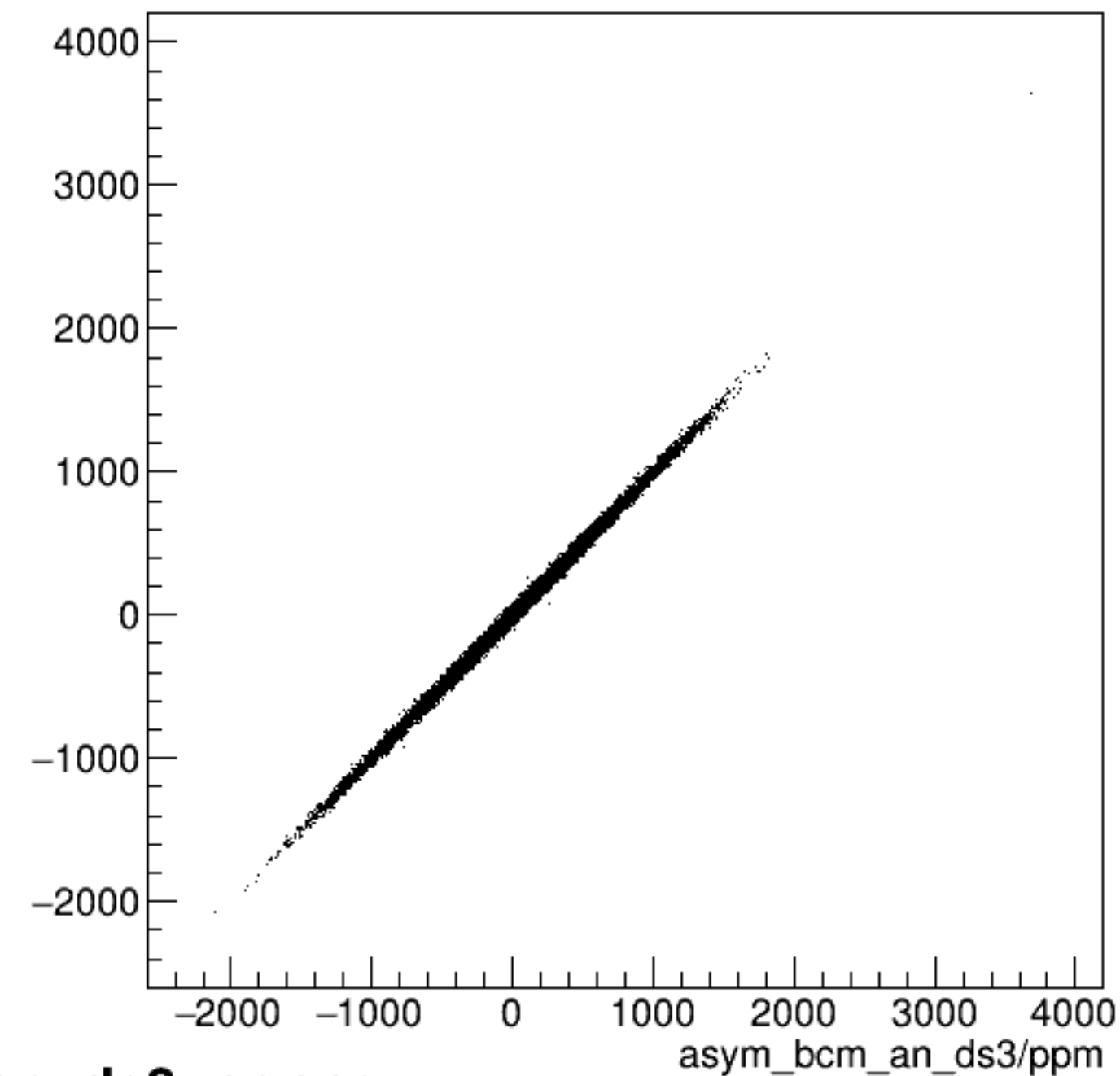
run8109_000_asym_bcm_an_us_vs_asym_bcm_an_ds3_pr.png
