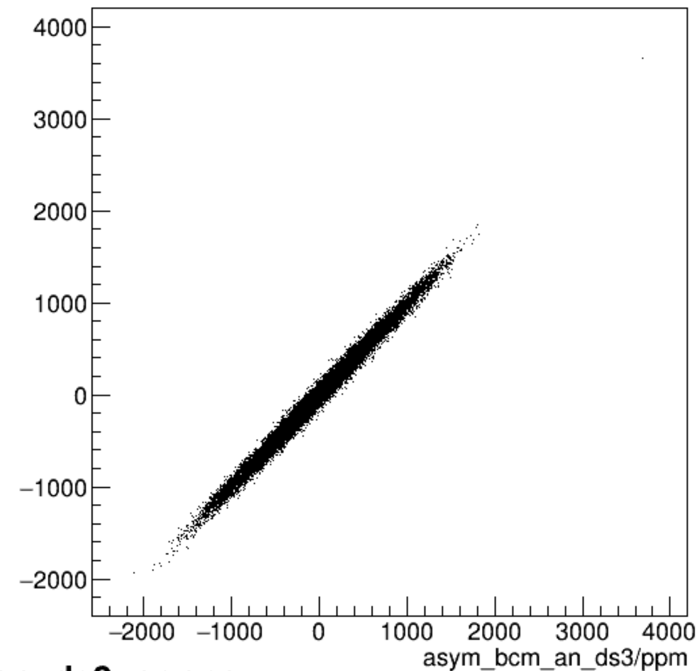
run8109_000_asym_bcm_dg_us_vs_asym_bcm_an_ds3_pr.png
