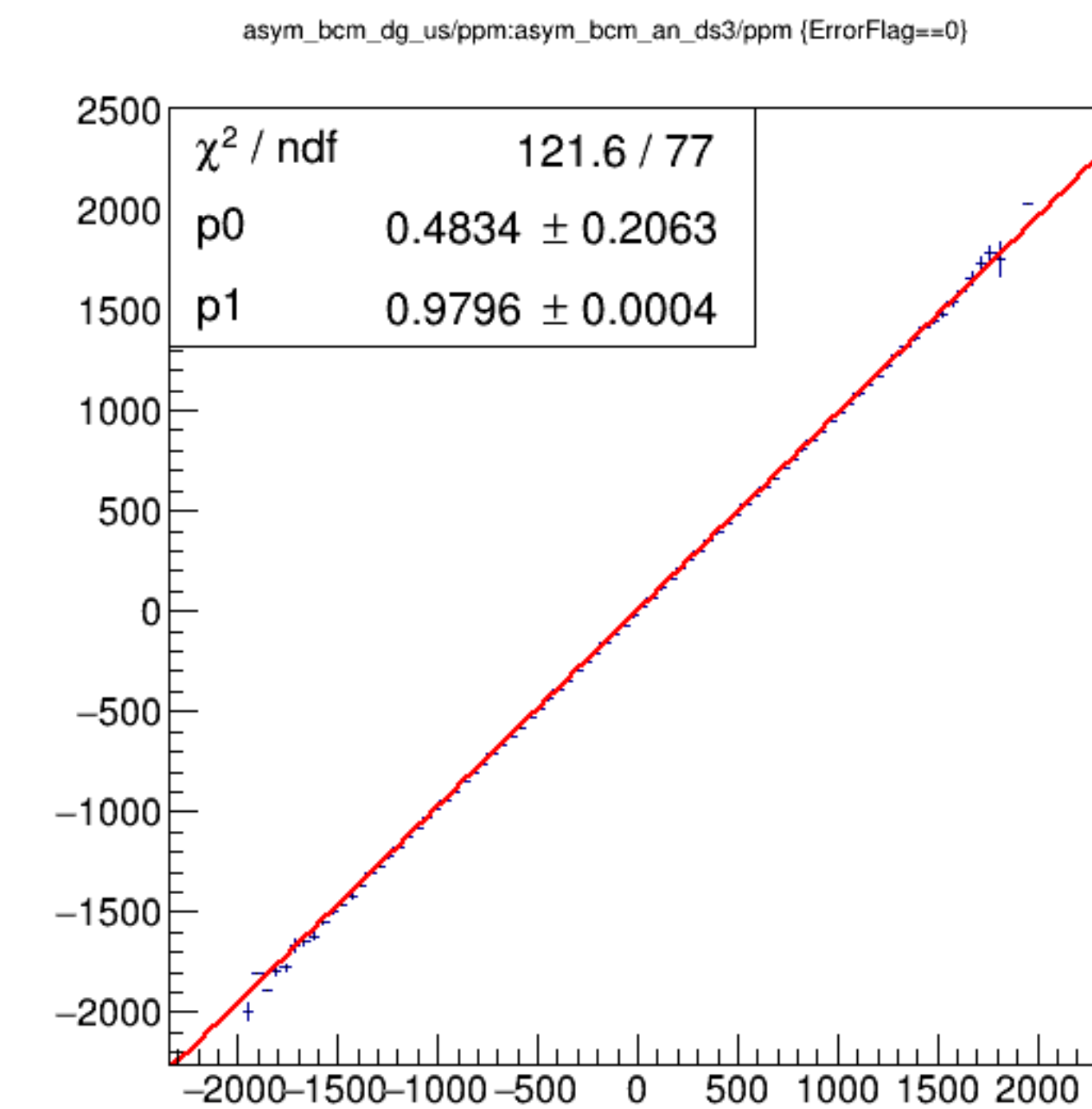
run8117_000_asym_bcm_dg_us_vs_asym_bcm_an_ds3_pr.png
