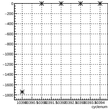
usr_coil3:cyclenum {run == 8118}
