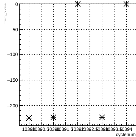
4eX_coil1:cyclenum {run == 8118}
