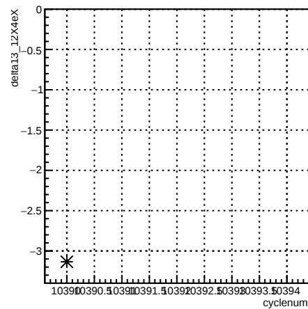
delta13_12X4eX:cyclenum {run == 8118}
