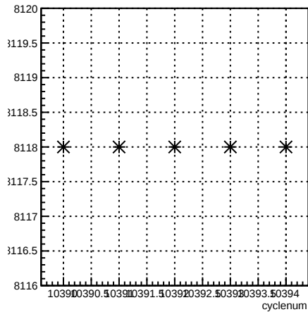
run:cyclenum {run == 8118}
