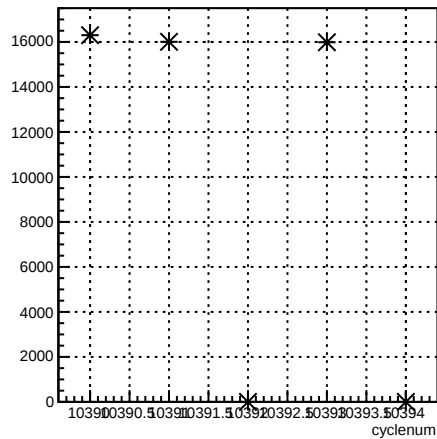
usl_coil6:cyclenum {run == 8118}
