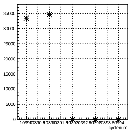
usr_coil7:cyclenum {run == 8118}
