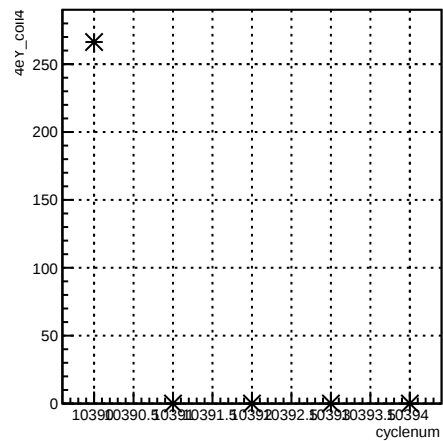
4eY_coil4:cyclenum {run == 8118}
