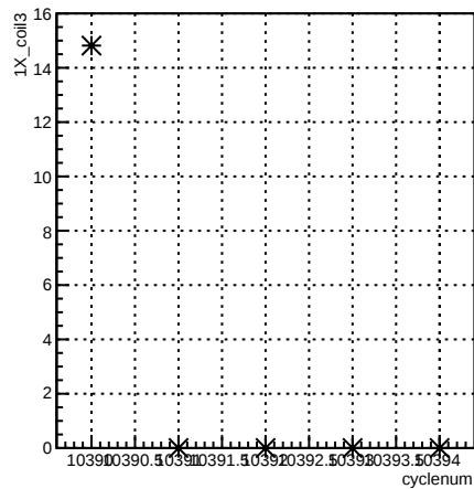
1X_coil3:cyclenum {run == 8118}
