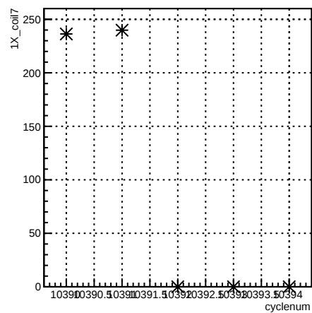
1X_coil7:cyclenum {run == 8118}
