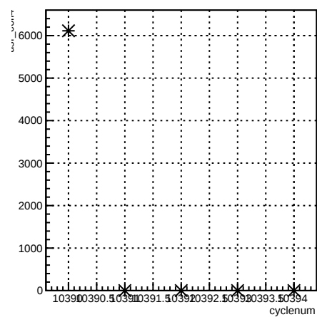
usr_coil4:cyclenum {run == 8118}
