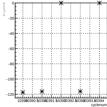
1X_coil1:cyclenum {run == 8118}
