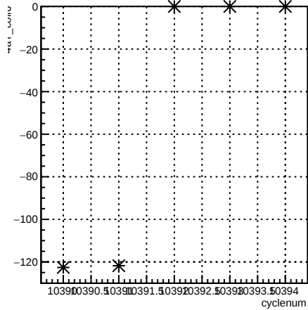
4eY_coil6:cyclenum {run == 8118}
