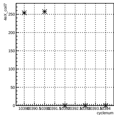
4eX_coil7:cyclenum {run == 8118}
