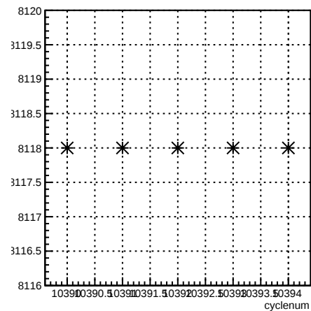
run:cyclenum {run == 8118}
