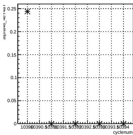
alpha46_4eY4aY:cyclenum {run == 8118}
