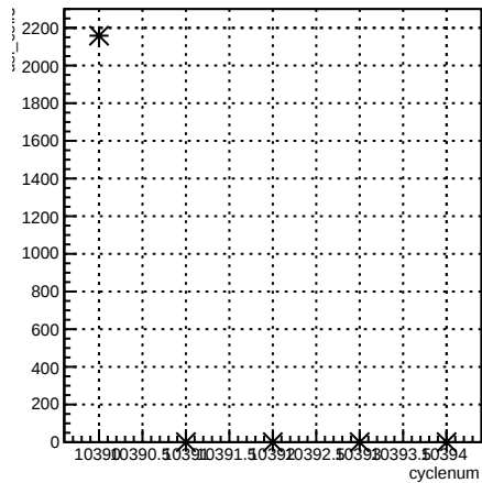
usl_coil7:cyclenum {run == 8118}
