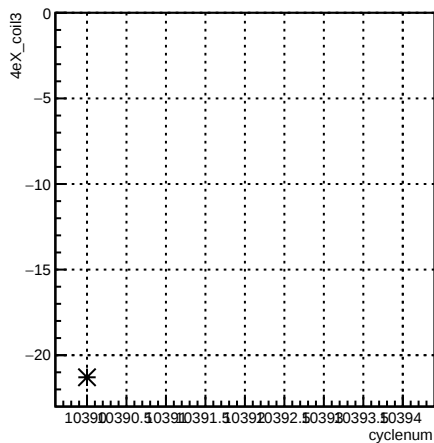
4eX_coil3:cyclenum {run == 8118}
