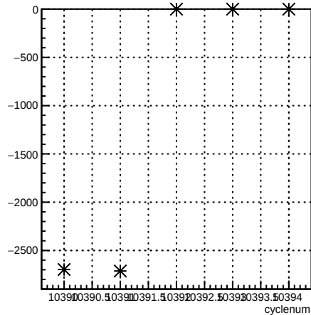
usl_coil6:cyclenum {run == 8118}
