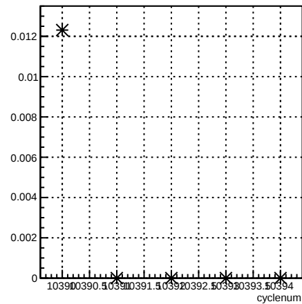
delta46_12X4eY:cyclenum {run == 8118}
