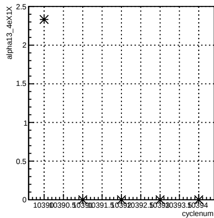
alpha13_4eX1X:cyclenum {run == 8118}
