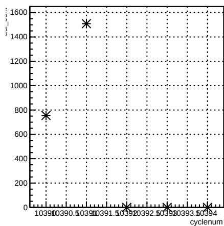
usl_coil7:cyclenum {run == 8118}
