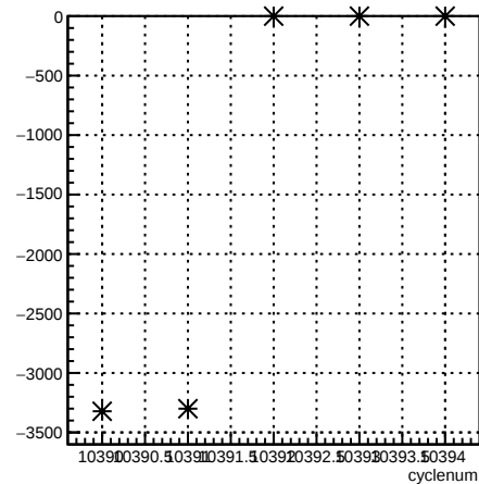
usr_coil6:cyclenum {run == 8118}
