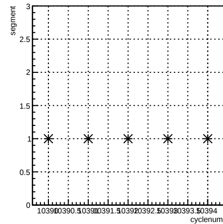
segment:cyclenum {run == 8118}
