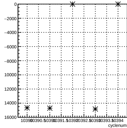
usr_coil1:cyclenum {run == 8118}
