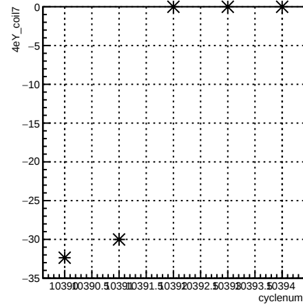
4eY_coil7:cyclenum {run == 8118}
