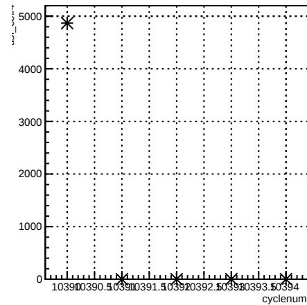
run:cyclenum {run == 8118}
