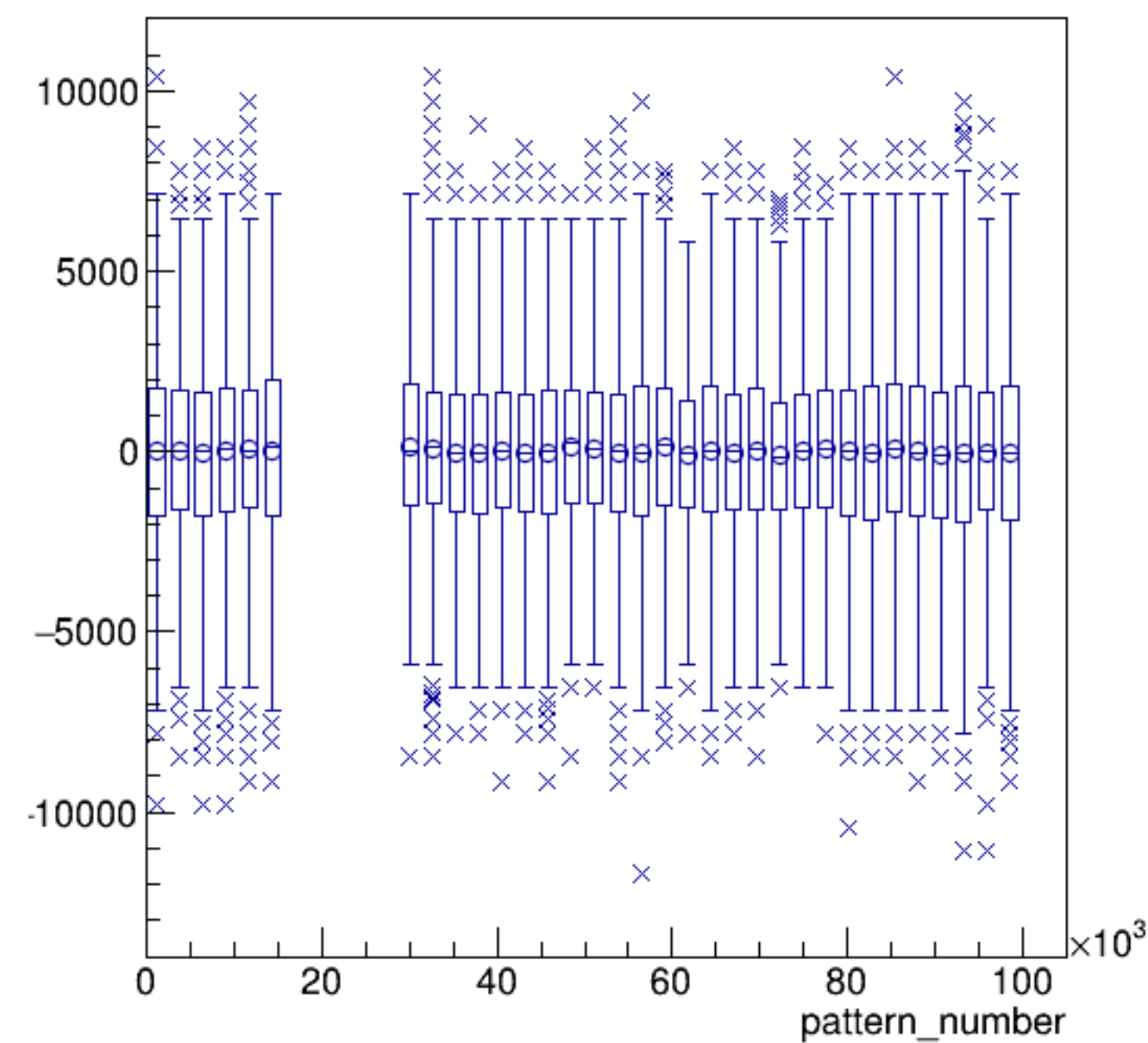
asym_sam3/ppm:pattern_number {ErrorFlag==0}
