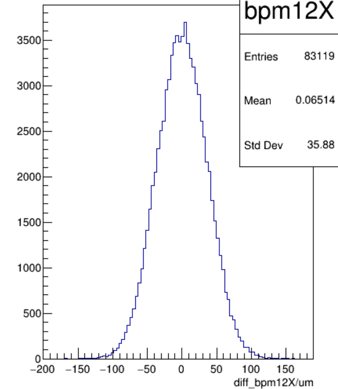
diff_bpm12X/um {ErrorFlag==0}
