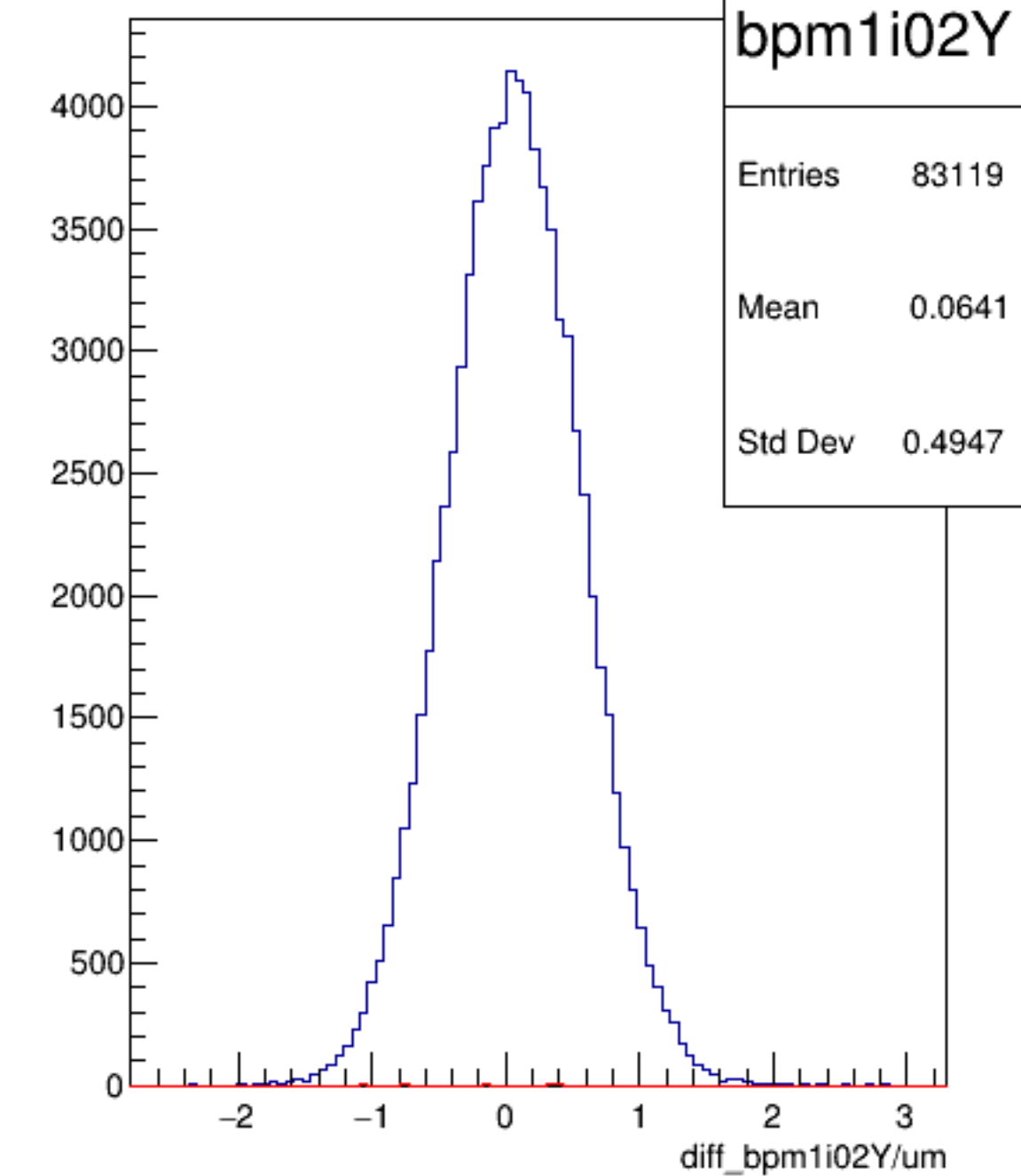
diff_bpm1i02Y/um {ErrorFlag==0}
