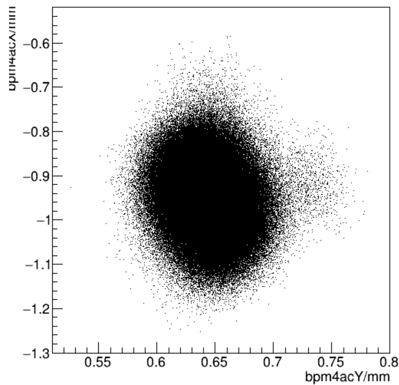
bpm4acX/mm:bpm4acY/mm {ErrorFlag==0}
