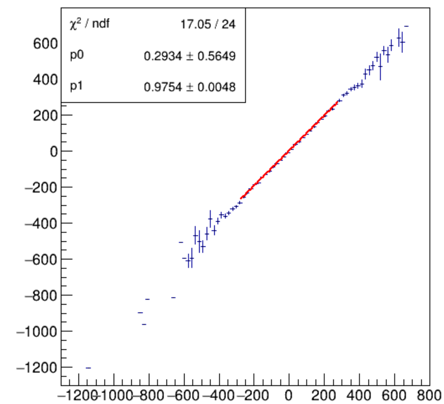
asym_bpm16WS/ppm:Aq/ppm {ErrorFlag==0}
