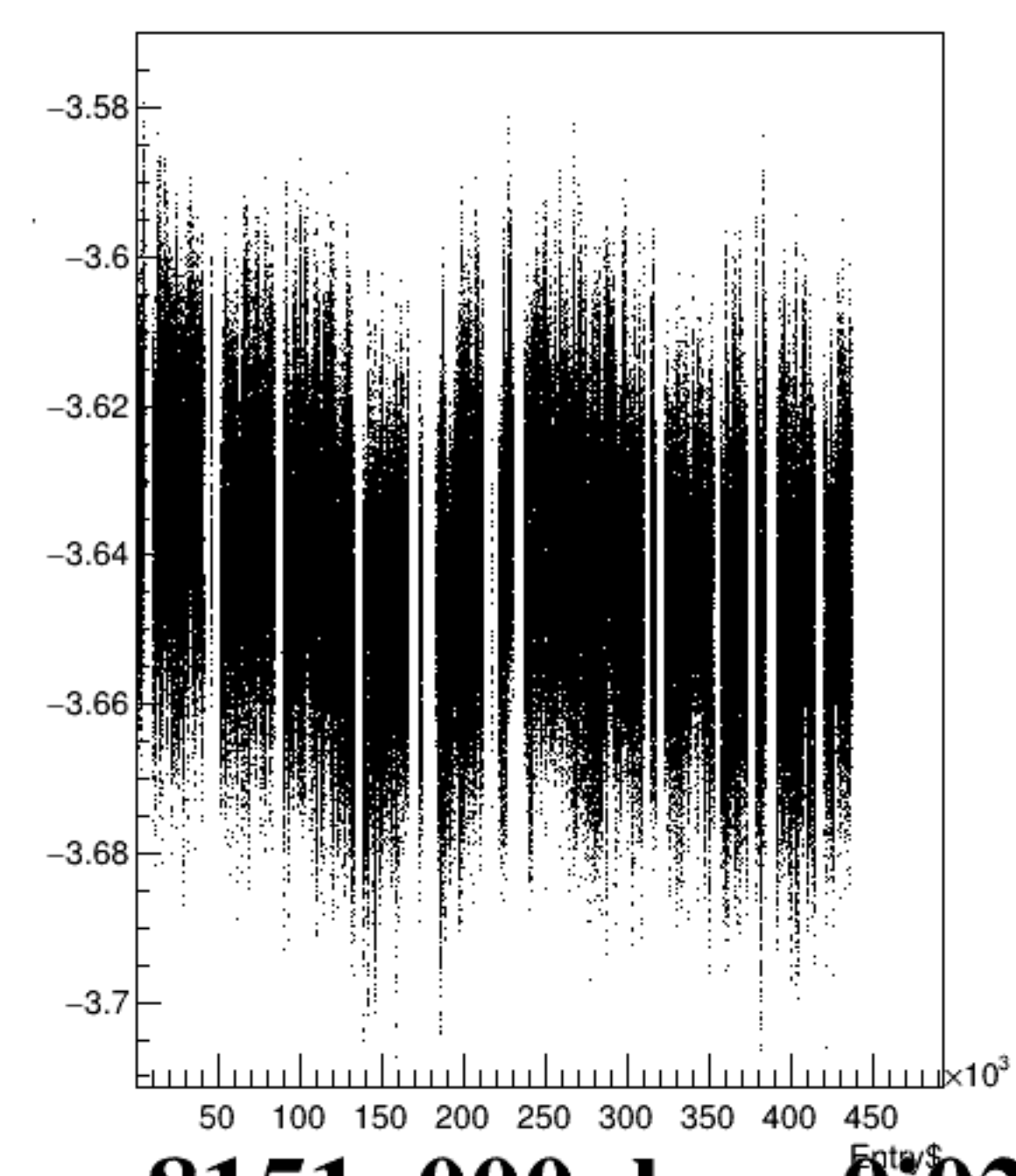
bpm0i02Y/mm:Entry$ {ErrorFlag==0}
