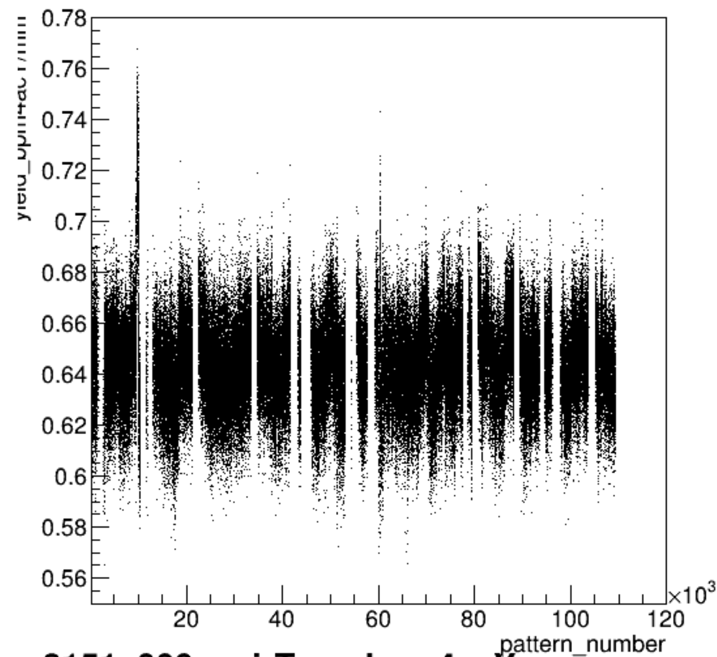
yield_bpm4acY/mm:pattern_number {ErrorFlag==0}
