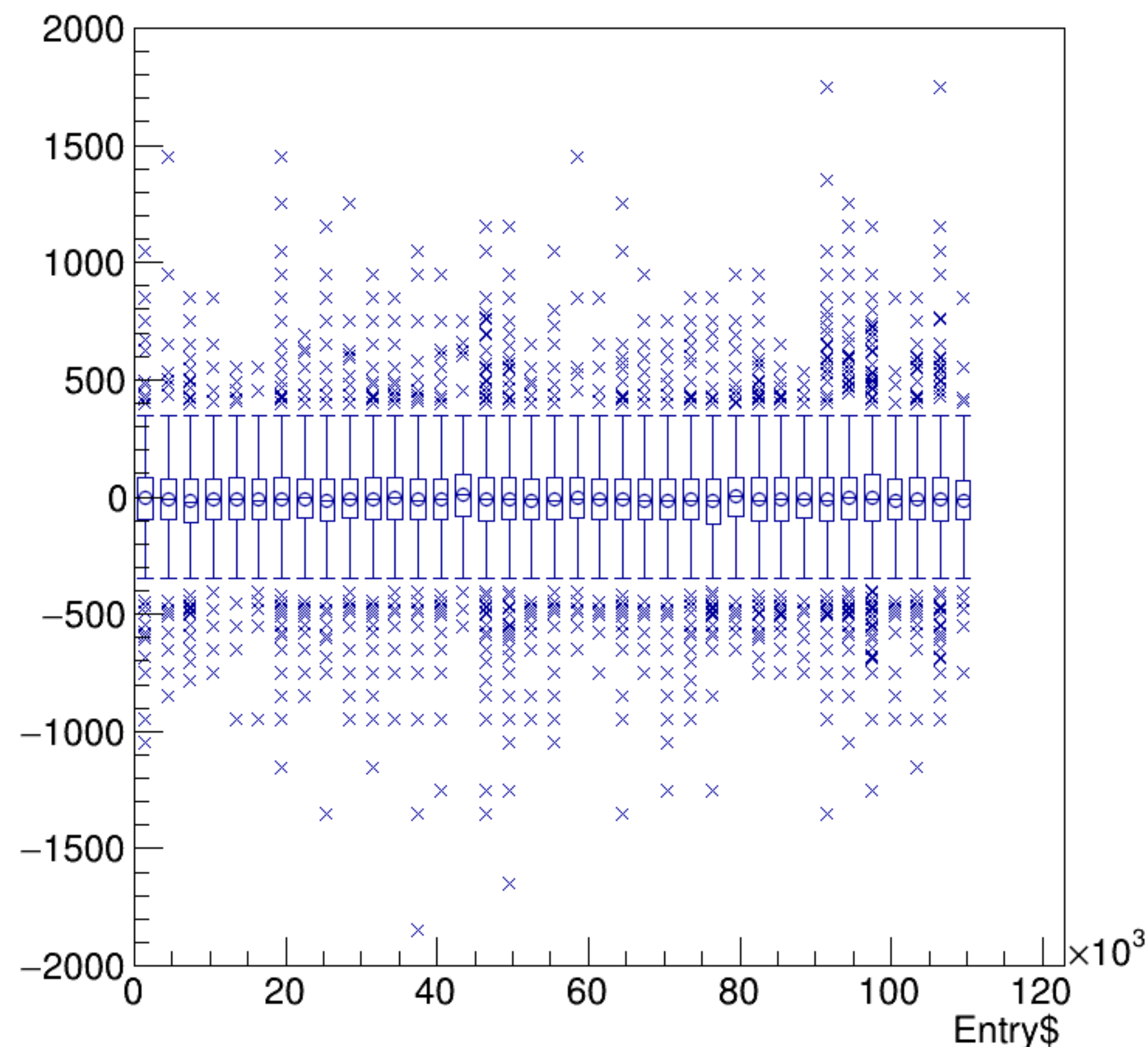
asym_bpm2i01WS/ppm:Entry$ {ErrorFlag==0}
