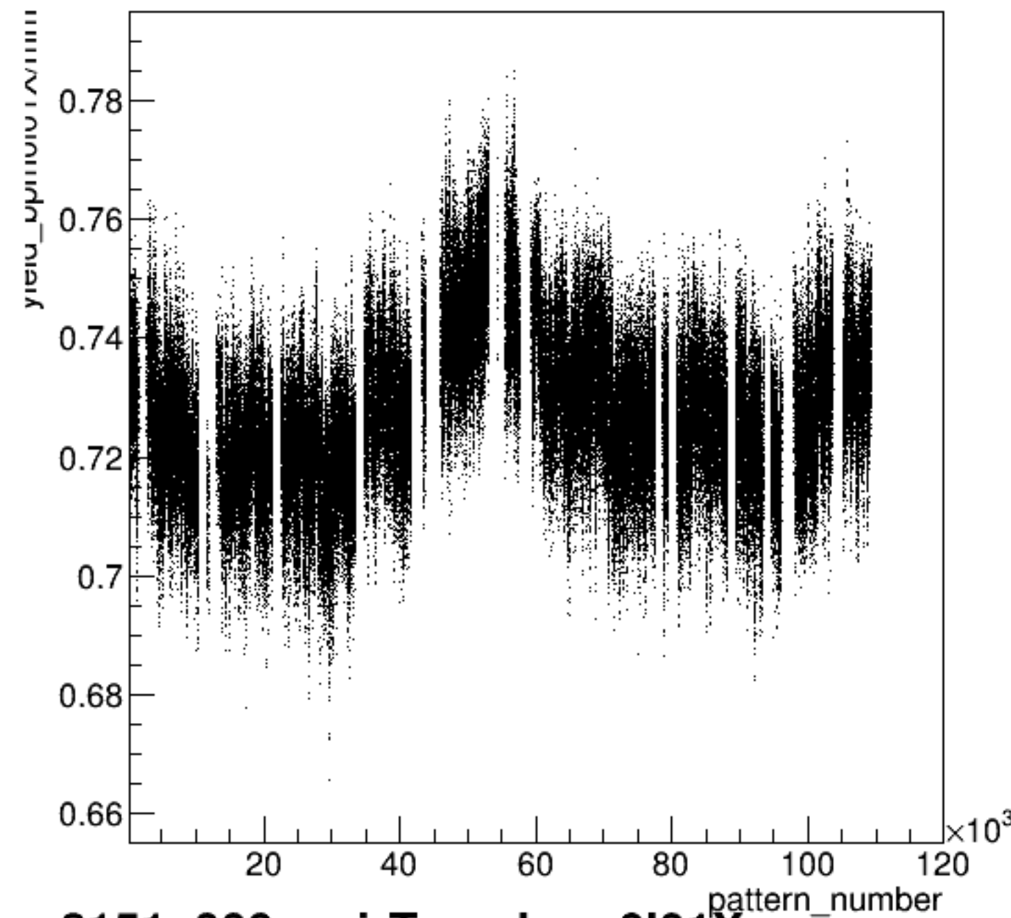
yield_bpm0l01X/mm:pattern_number {ErrorFlag==0}
