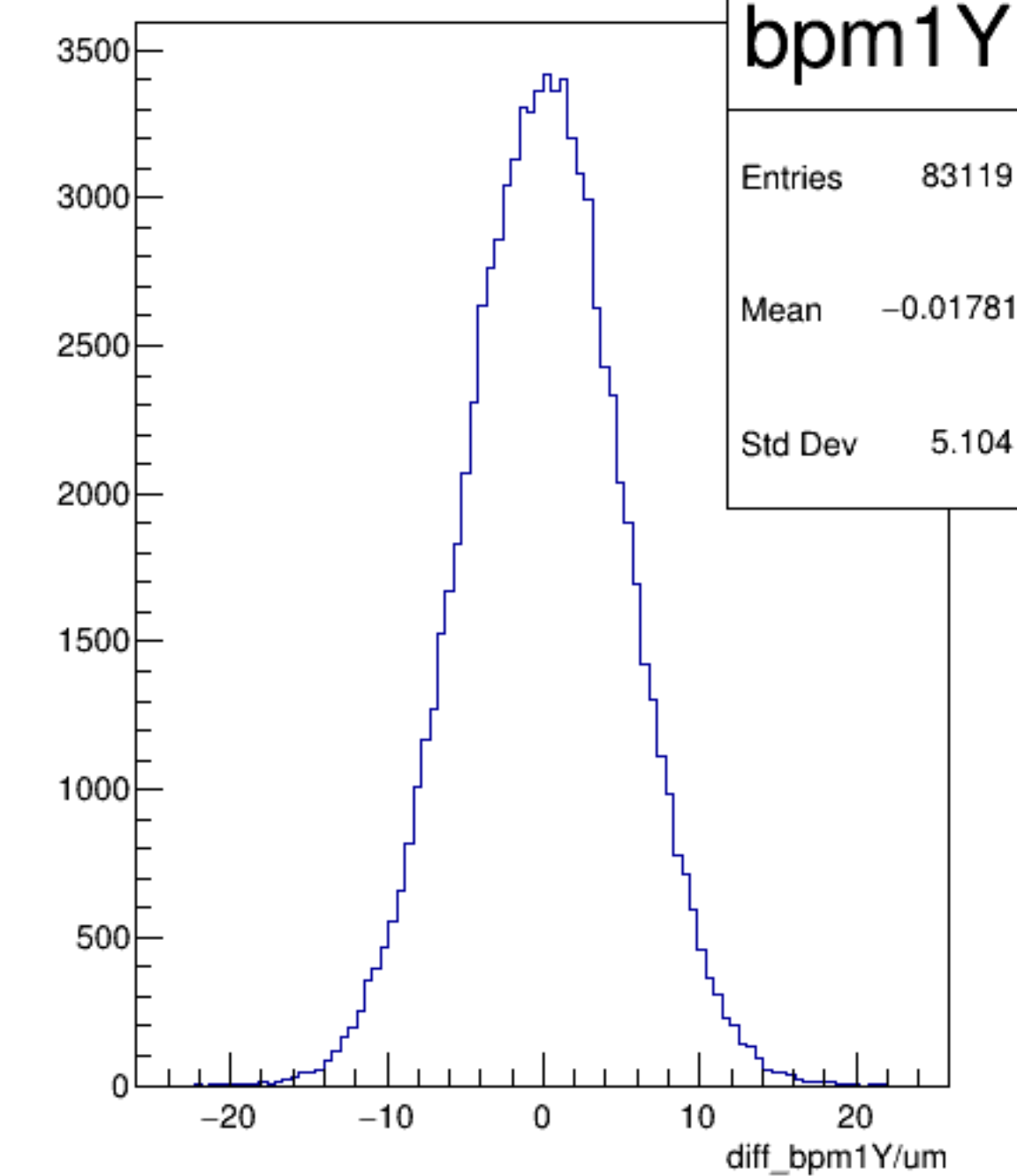
diff_bpm1Y/um {ErrorFlag==0}
