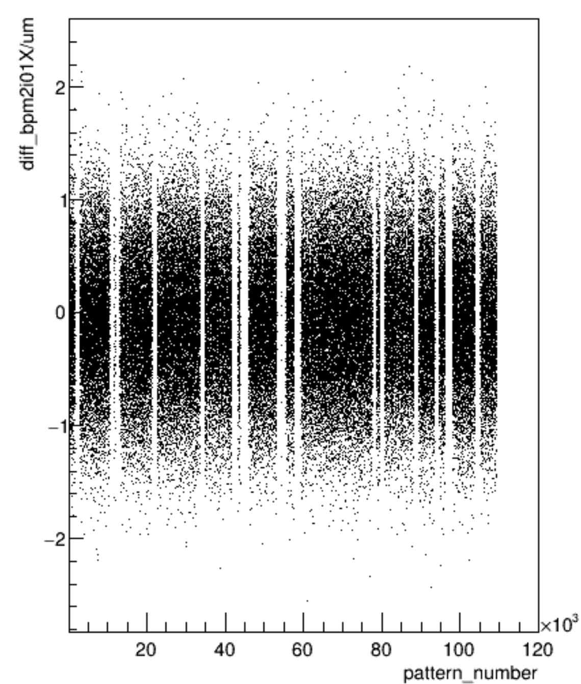
diff_bpm2i01X/um:pattern_number {ErrorFlag==0}
