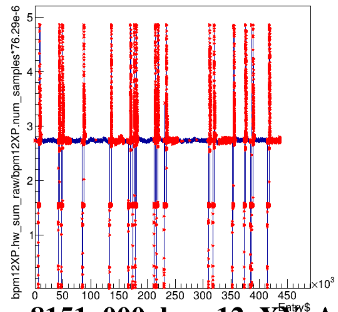
bpm12XP.hw_sum_raw/bpm12XP.num_samples*76.29e-6:Entry$
