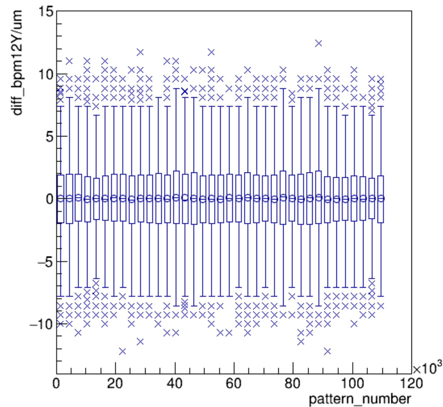
diff_bpm12Y/um:pattern_number {ErrorFlag==0}
