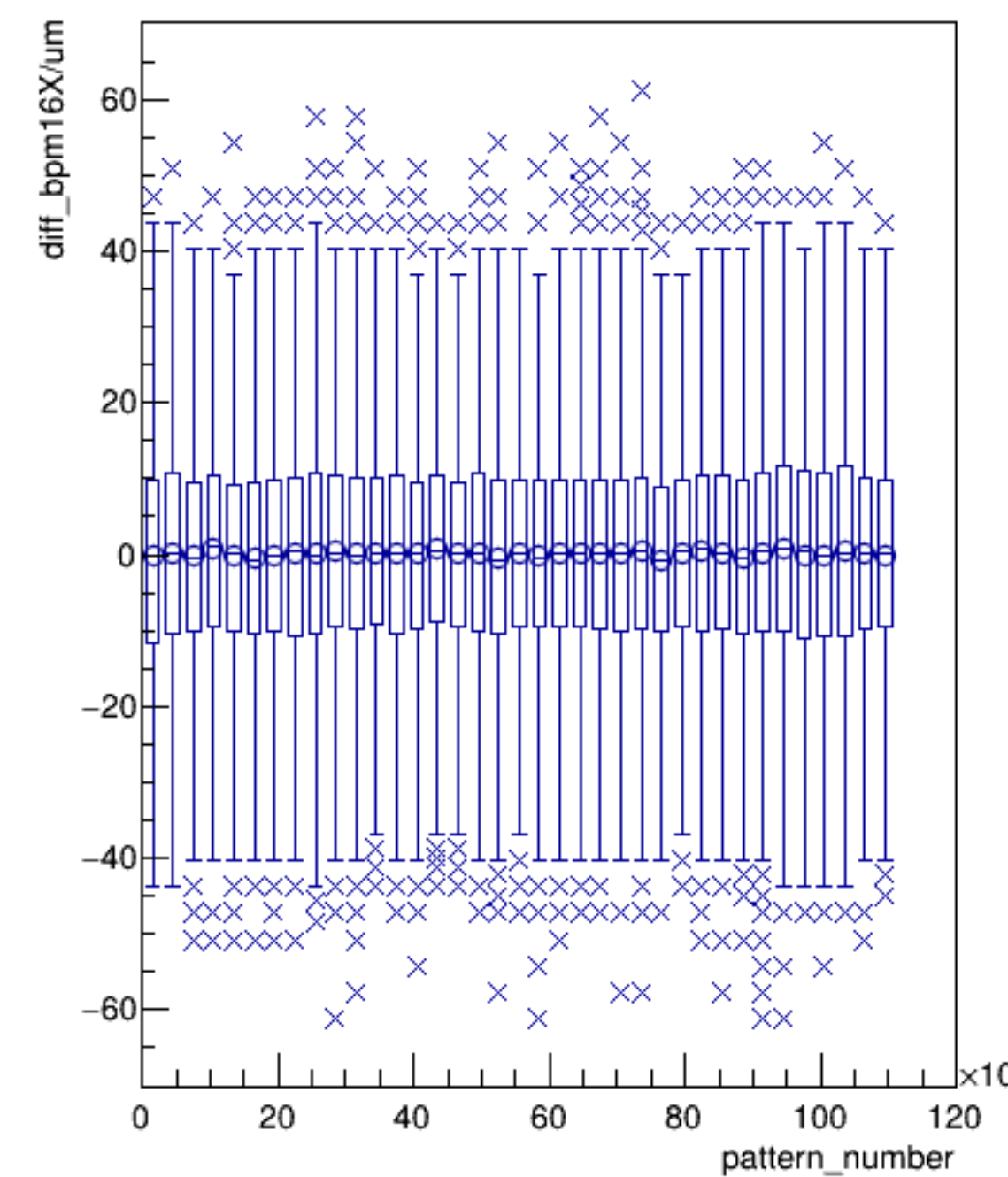
diff_bpm16X/um:pattern_number {ErrorFlag==0}
