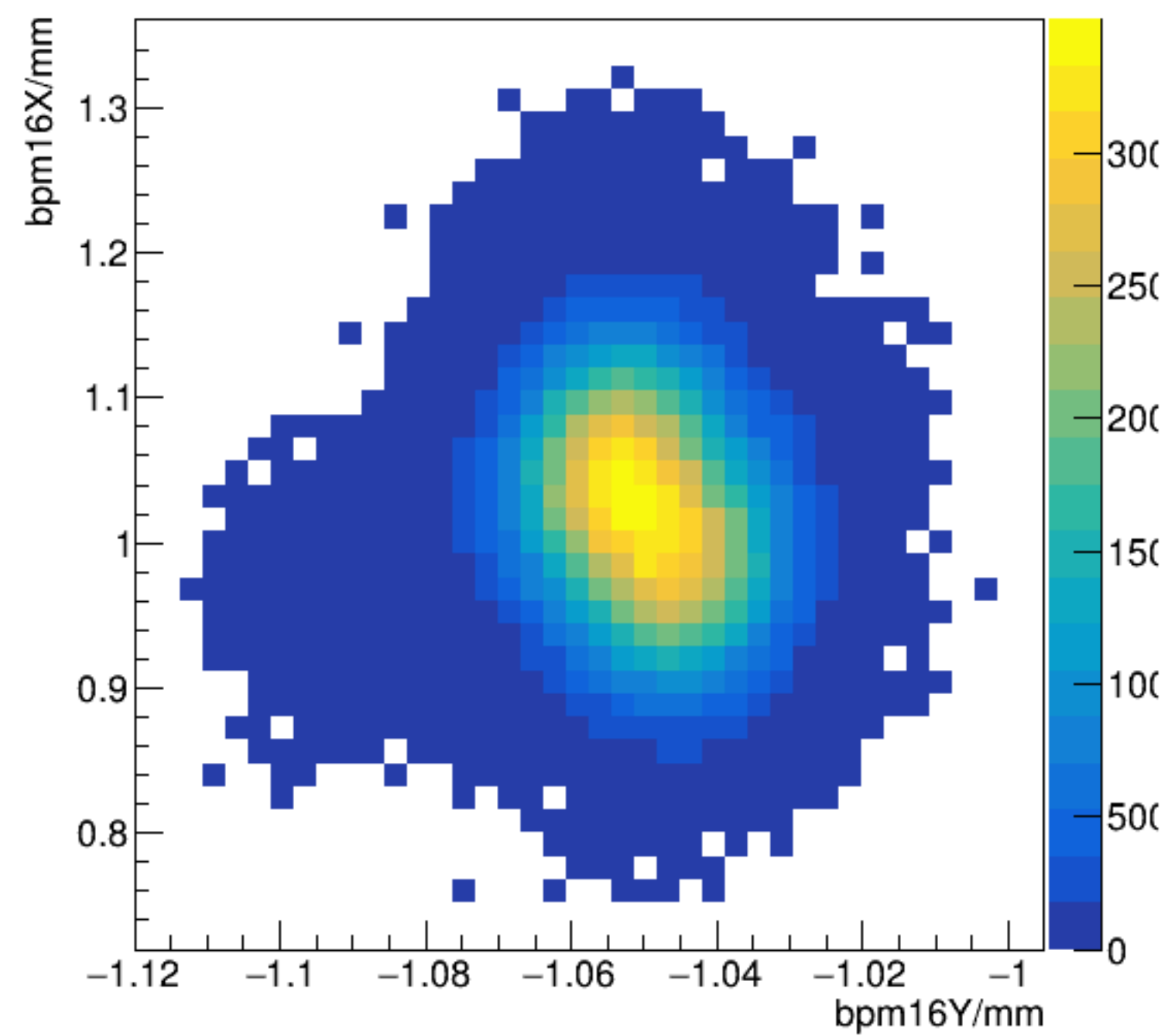
bpm16X/mm:bpm16Y/mm {ErrorFlag==0}
