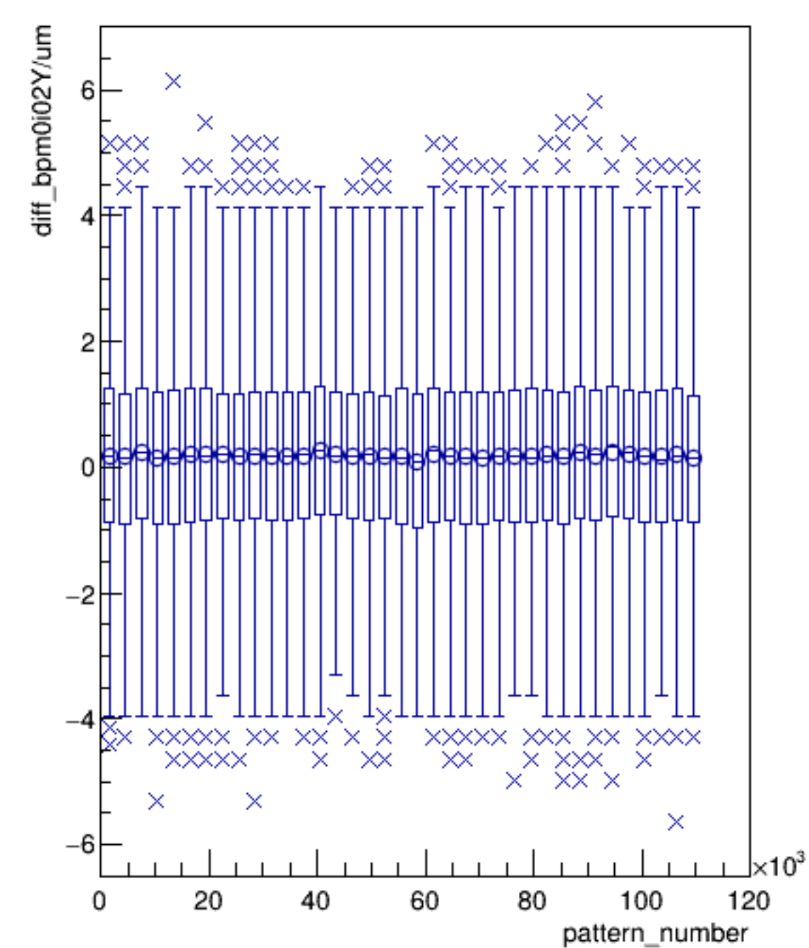
diff_bpm0i02Y/um:pattern_number (ErrorFlag==0)
