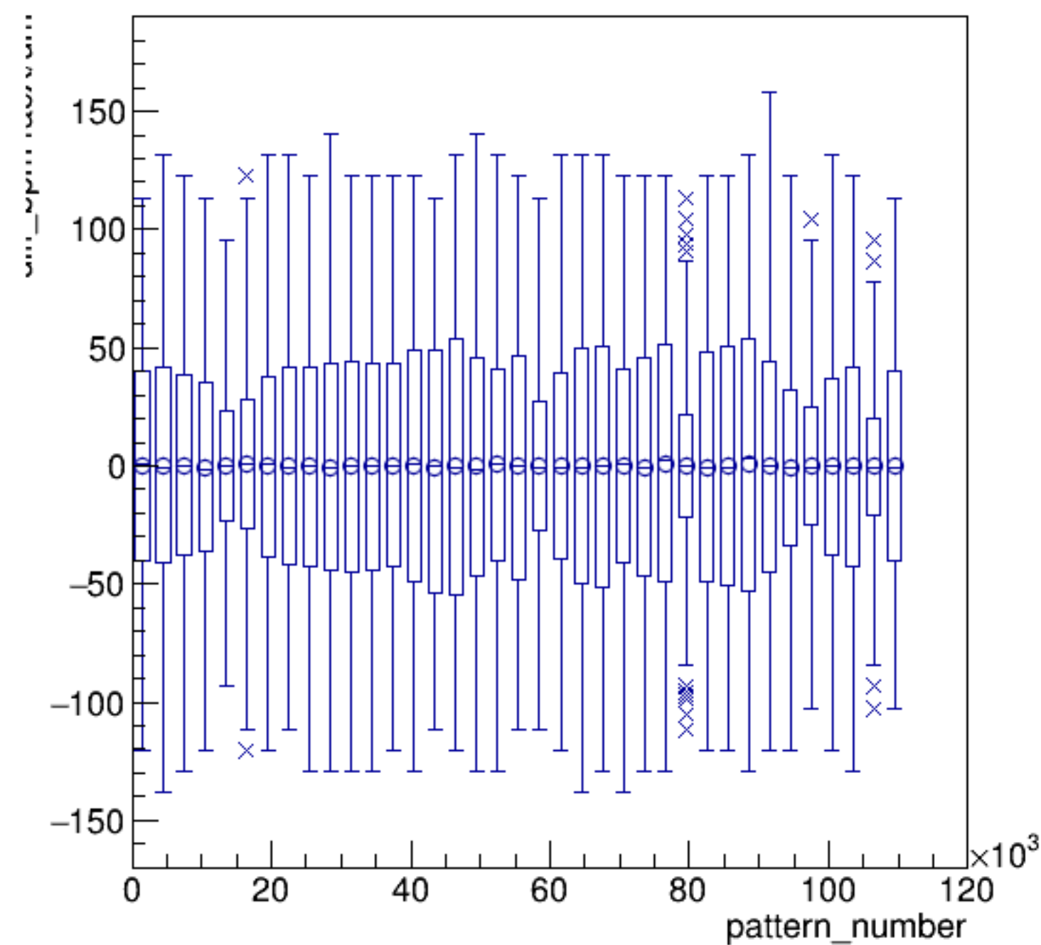
diff_bpm4acX/um:pattern_number {ErrorFlag==0}
