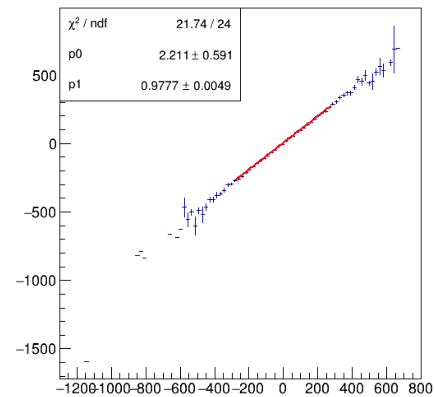
asym_bpm0l01WS/ppm:Aq/ppm {ErrorFlag==0}
