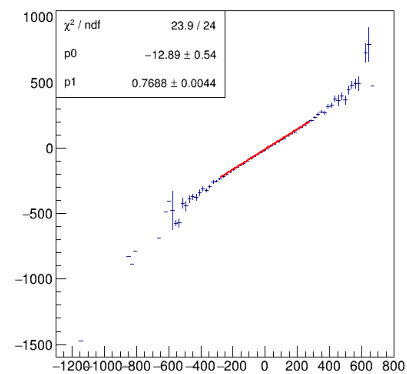
asym_bpm0i02WS/ppm:Aq/ppm {ErrorFlag==0}
