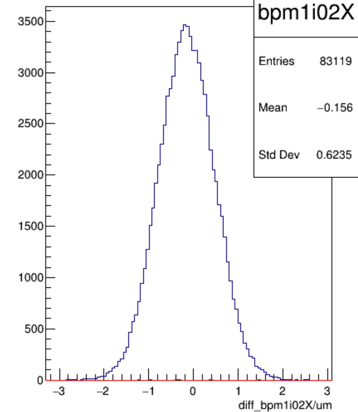
diff_bpm1i02X/um {ErrorFlag==0}
