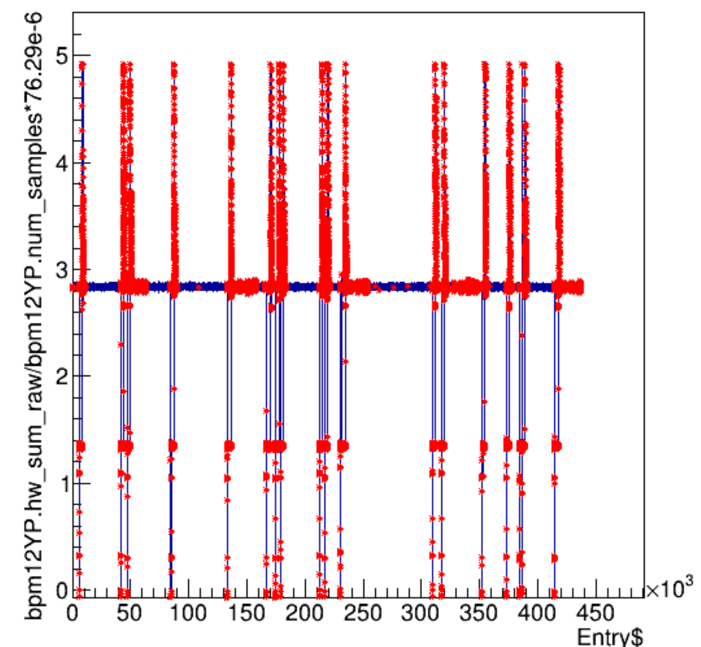
bpm12YP.hw_sum_raw/bpm12YP.num_samples*76.29e-6:Entry$
