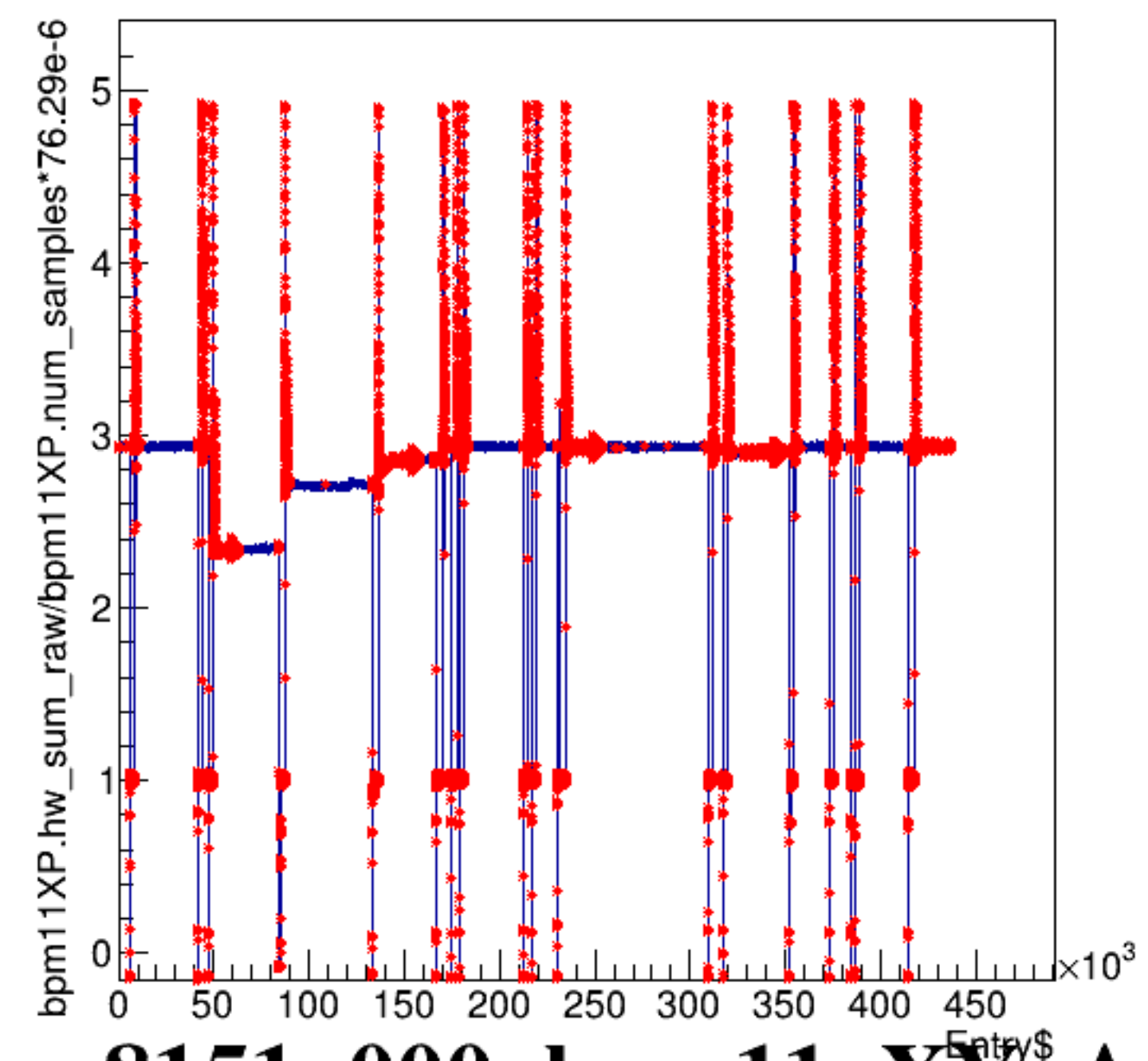
bpm11XP.hw_sum_raw/bpm11XP.num_samples*76.29e-6:Entry$
