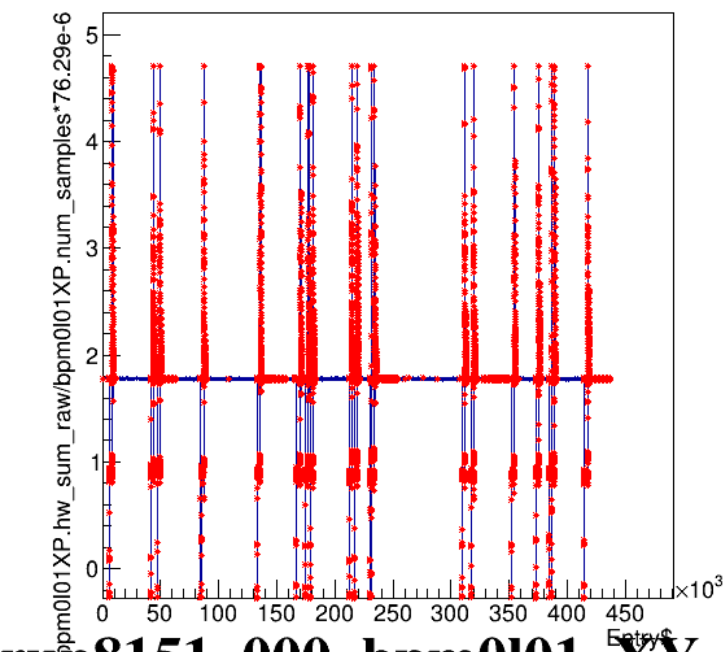
bpm0l01XP.hw_sum_raw/bpm0l01XP.num_samples*76.29e-6:Entry$
