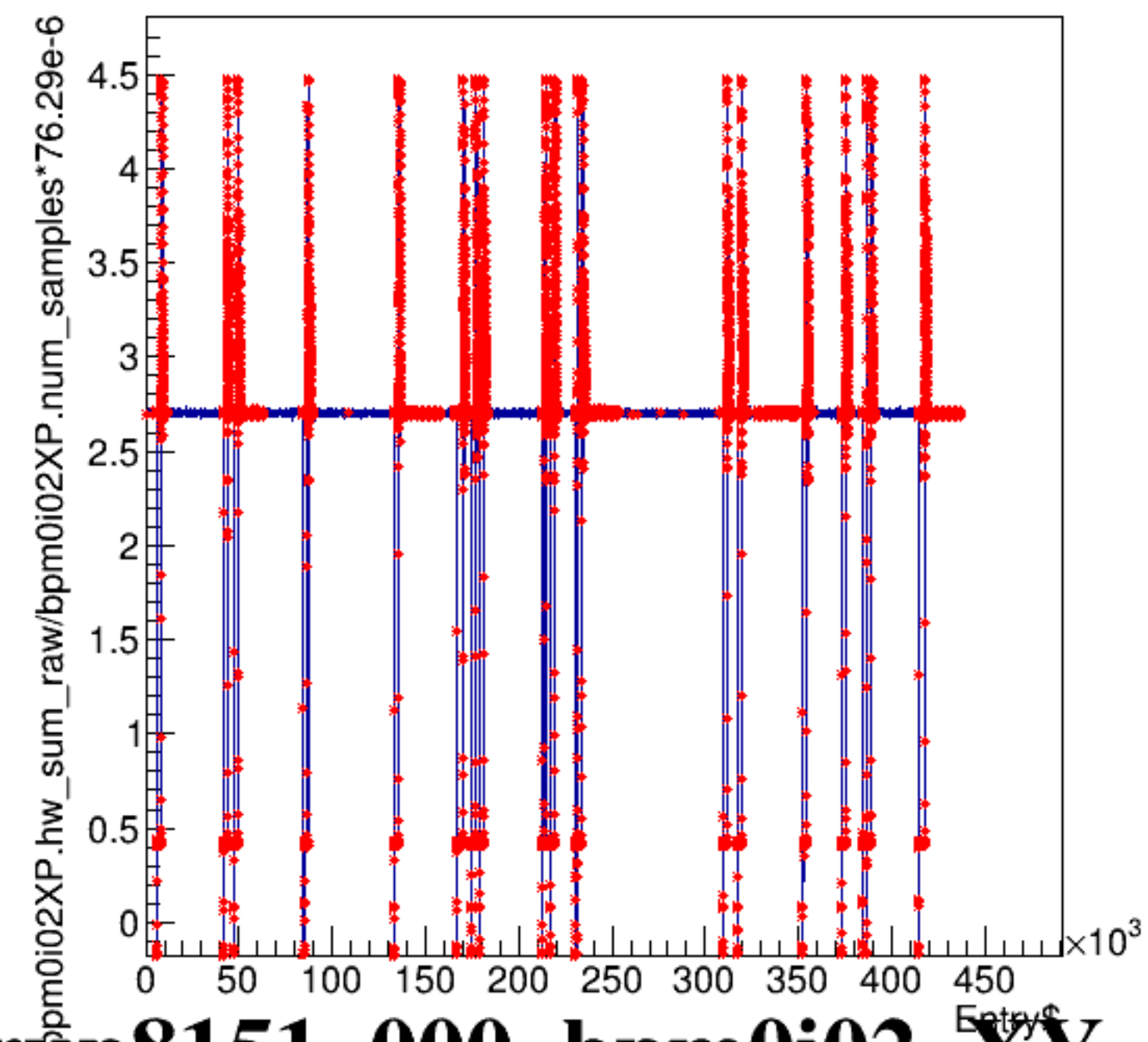
bpm0i02XP.hw_sum_raw/bpm0i02XP.num_samples*76.29e-6:Entry$
