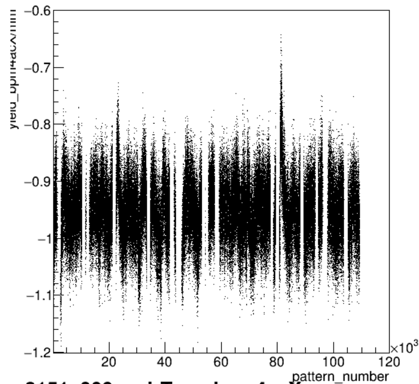
yield_bpm4acX/mm:pattern_number {ErrorFlag==0}
