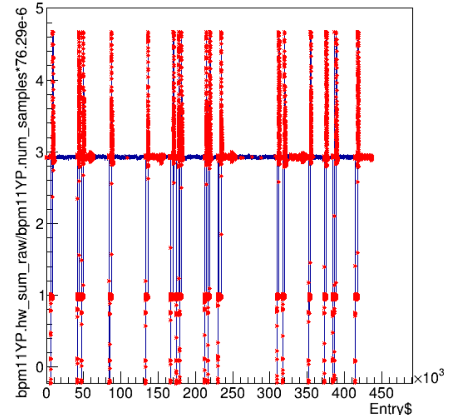
bpm11YP.hw_sum_raw/bpm11YP.num_samples*76.29e-6:Entry$
