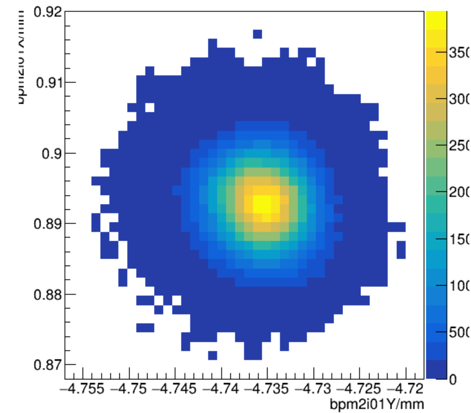
bpm2i01X/mm:bpm2i01Y/mm {ErrorFlag==0}
