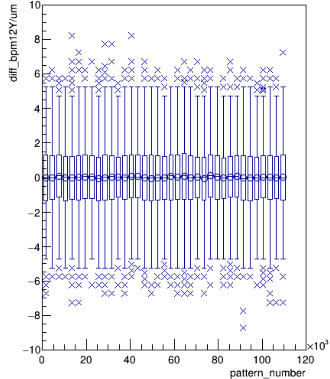
diff_bpm12Y/um:pattern_number (ErrorFlag==0)
