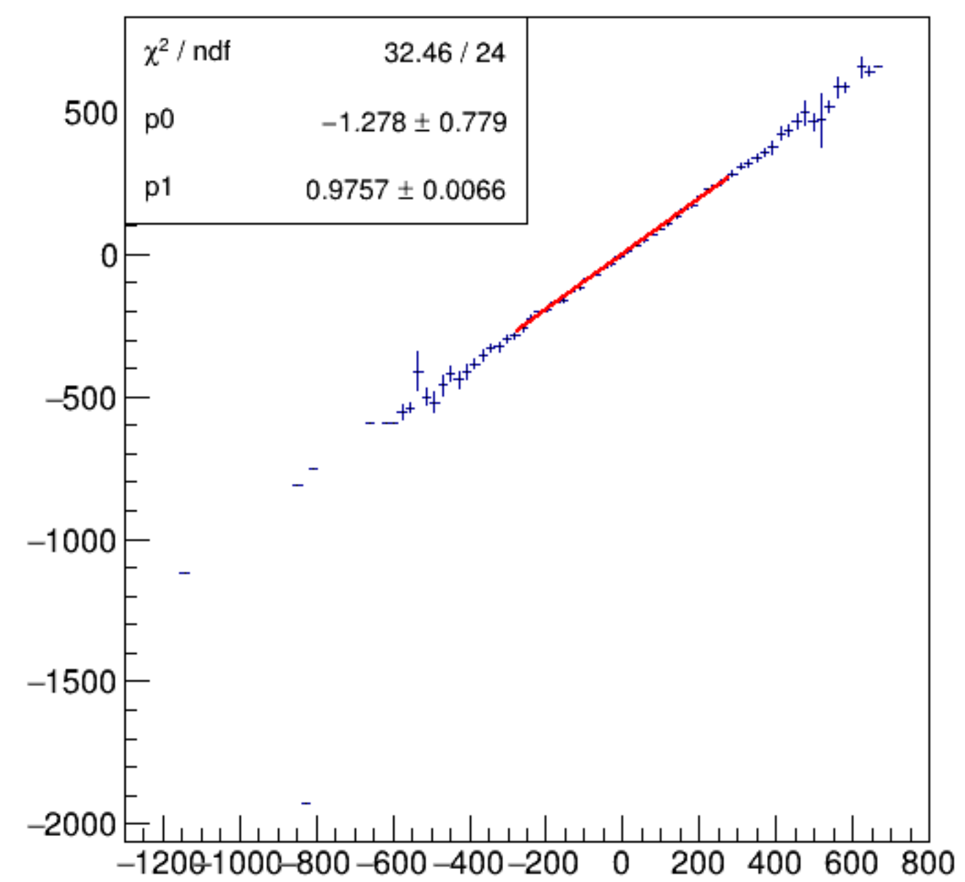
asym_bpm4acWS/ppm:Aq/ppm {ErrorFlag==0}
