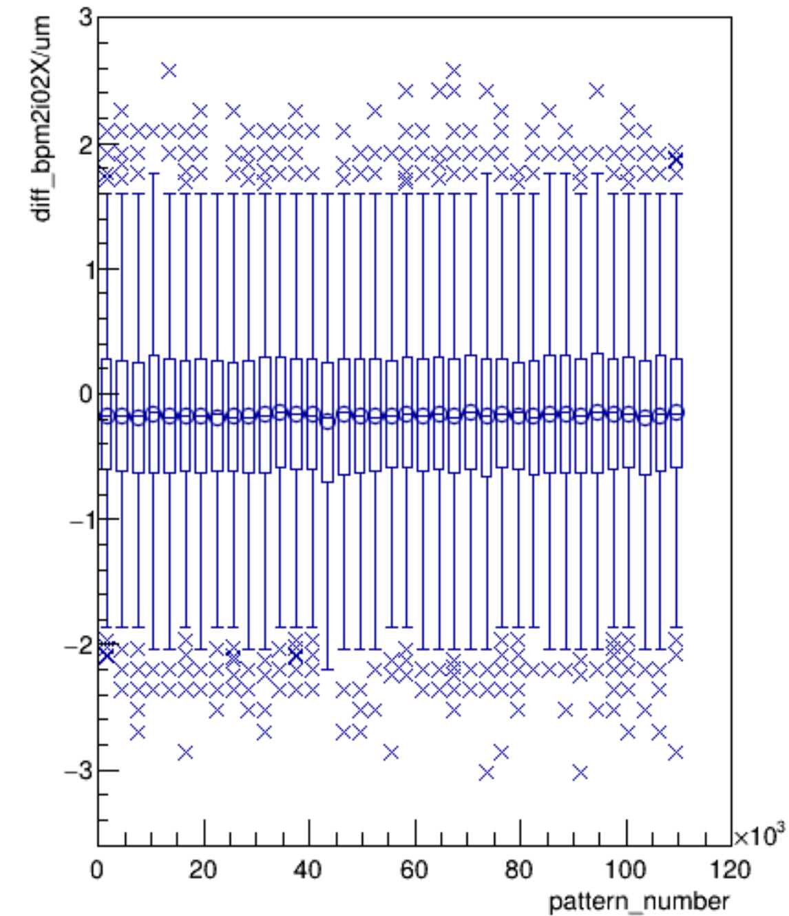
diff_bpm2i02X/um:pattern_number (ErrorFlag==0)
