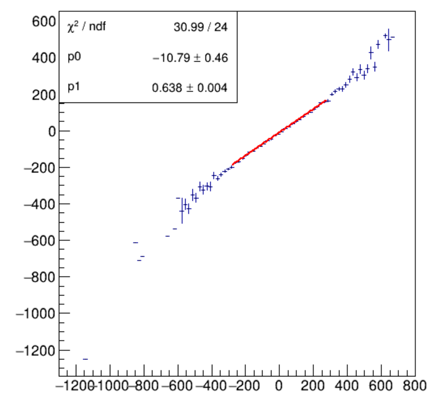
asym_bpm2i01WS/ppm:Aq/ppm {ErrorFlag==0}
