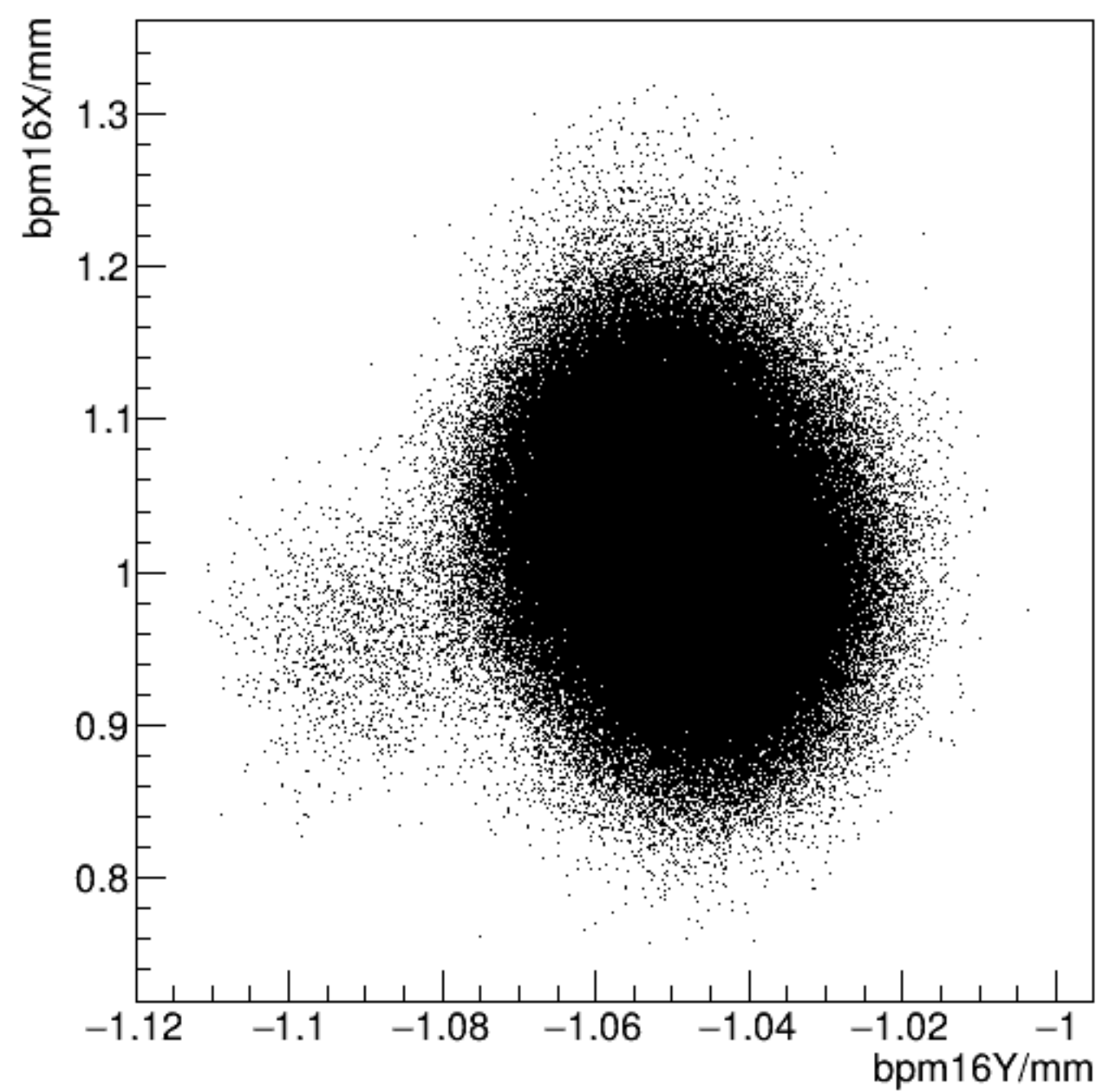
bpm16X/mm:bpm16Y/mm {ErrorFlag==0}
