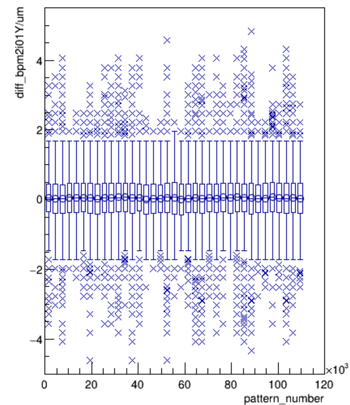
diff_bpm2i01Y/um:pattern_number {ErrorFlag==0}
