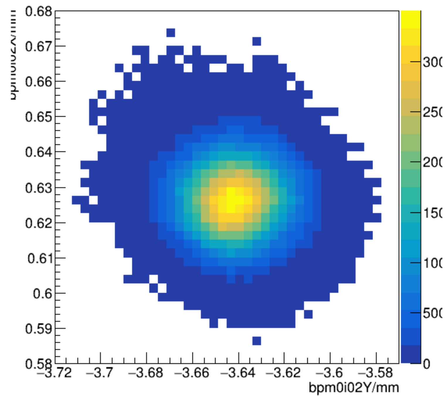
bpm0i02X/mm:bpm0i02Y/mm {ErrorFlag==0}
