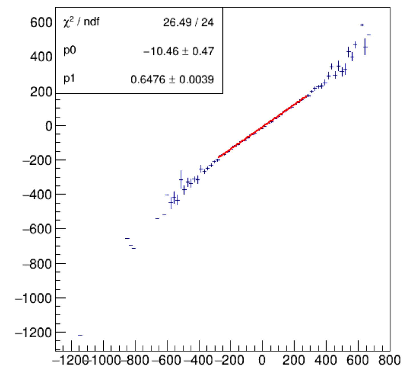
asym_bpm2i02WS/ppm:Aq/ppm {ErrorFlag==0}
