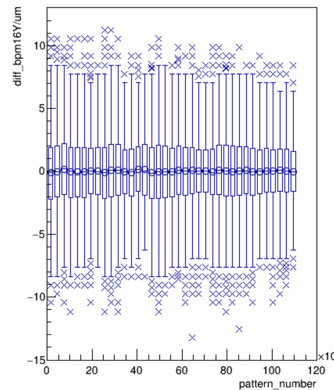
diff_bpm16Y/um:pattern_number {ErrorFlag==0}
