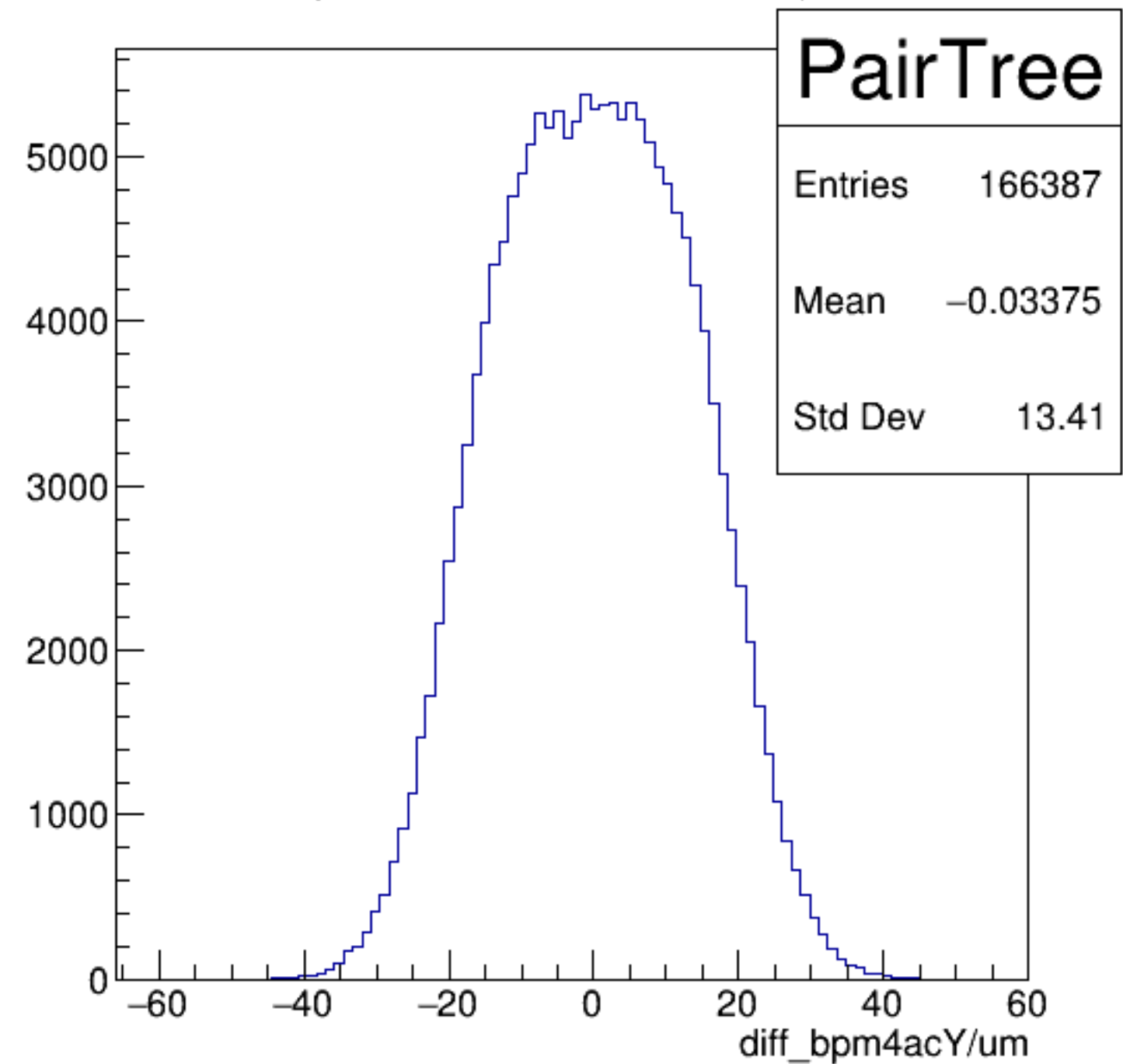
diff_bpm4acY/um {ErrorFlag==0}
