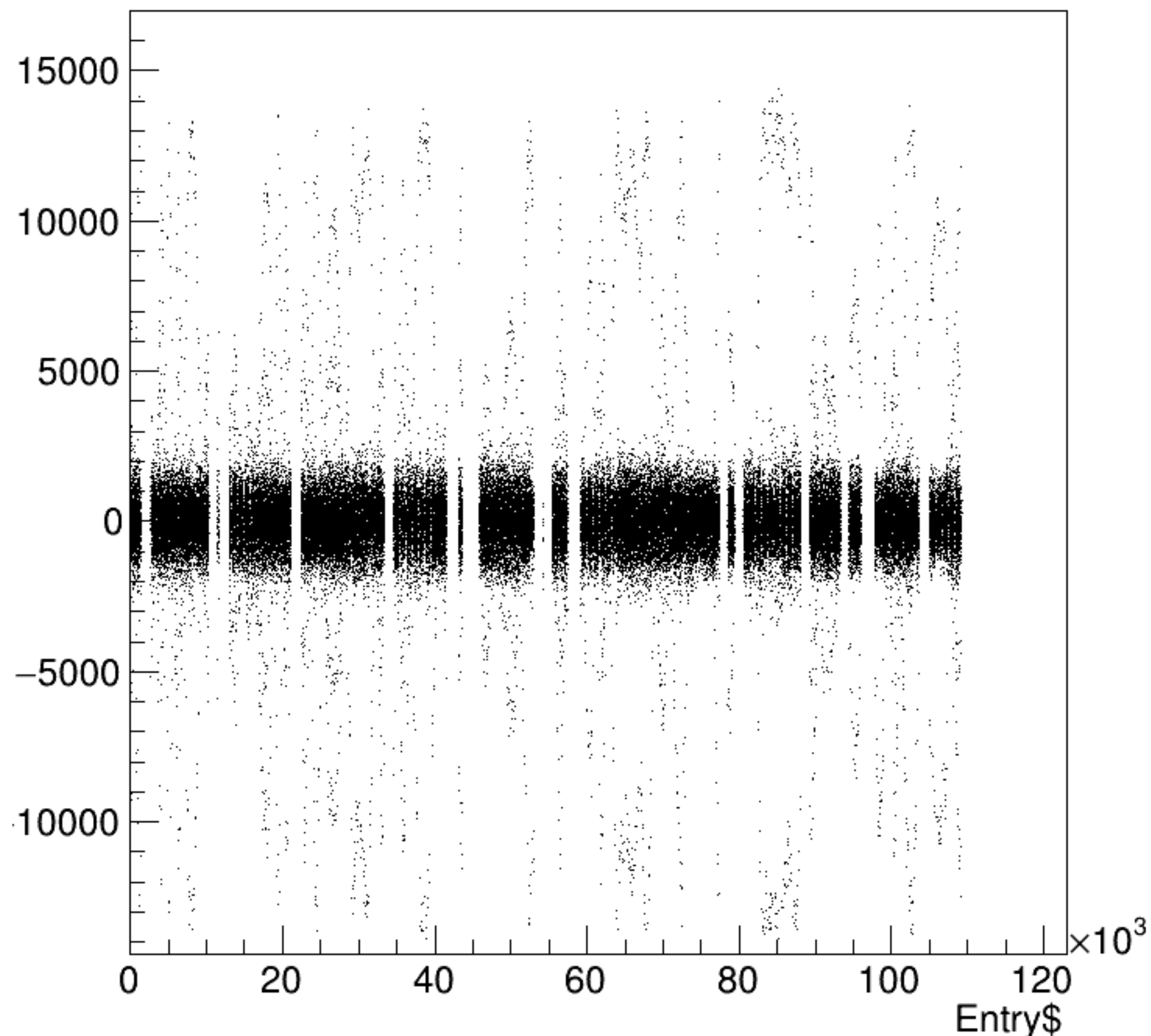
asym_bpm0i07WS/ppm:Entry$ {ErrorFlag==0}
