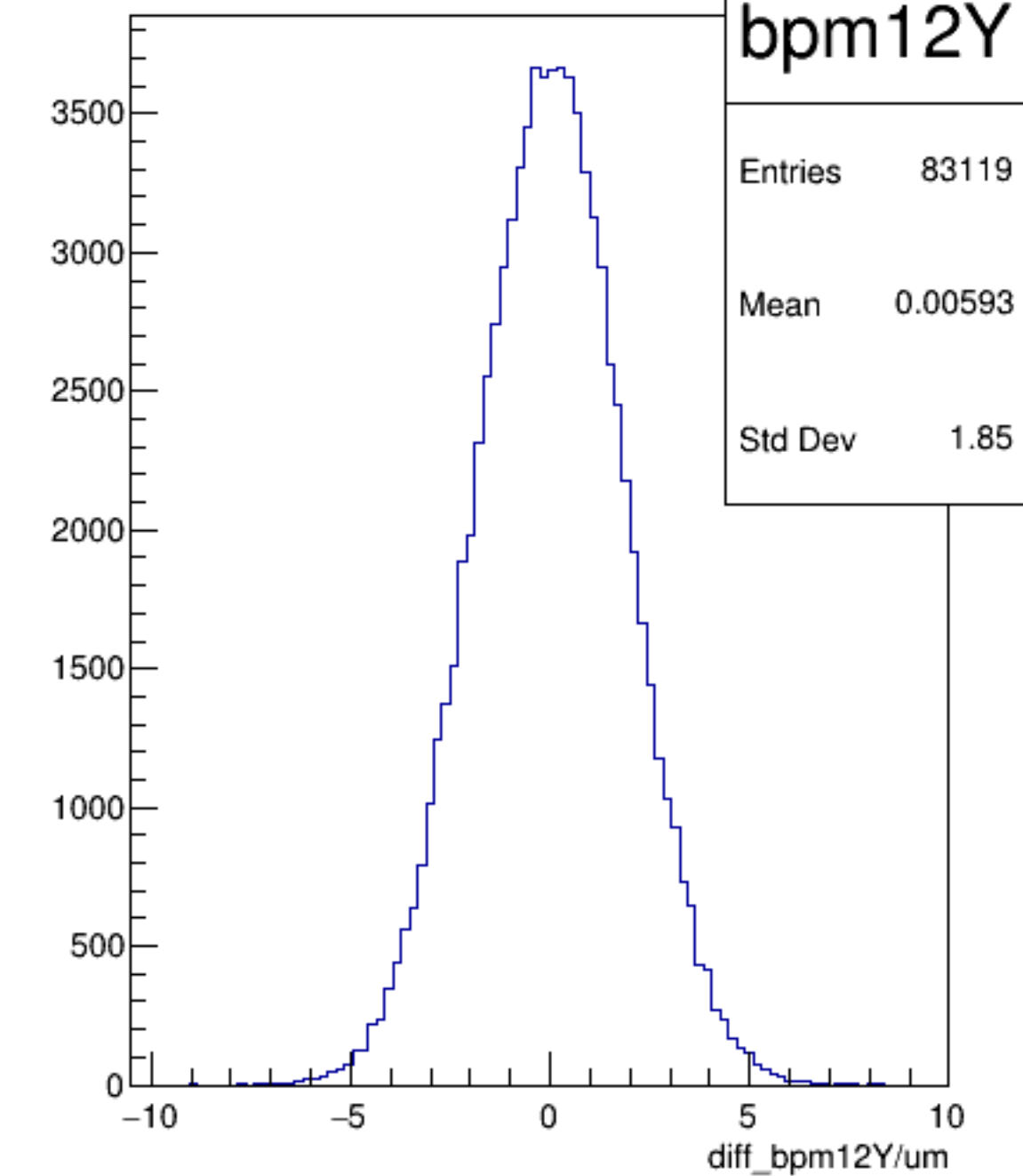
diff_bpm12Y/um {ErrorFlag==0}
