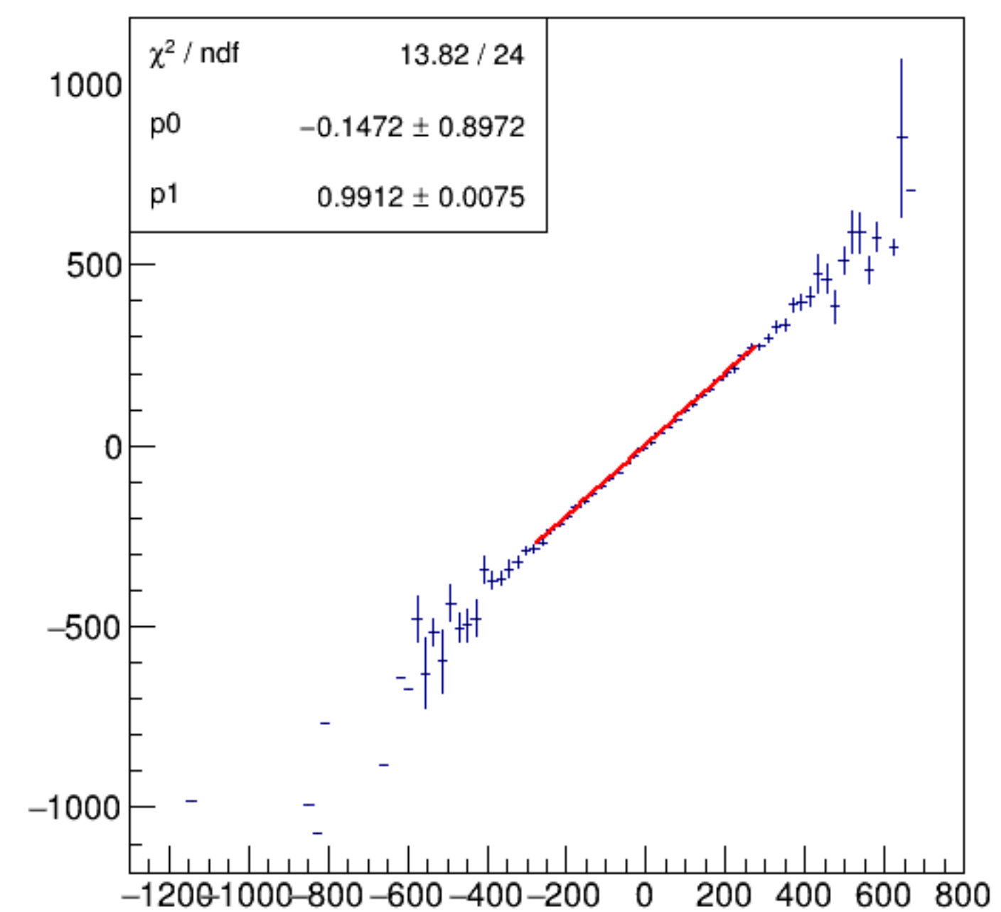
asym_bpm12WS/ppm:Aq/ppm {ErrorFlag==0}
