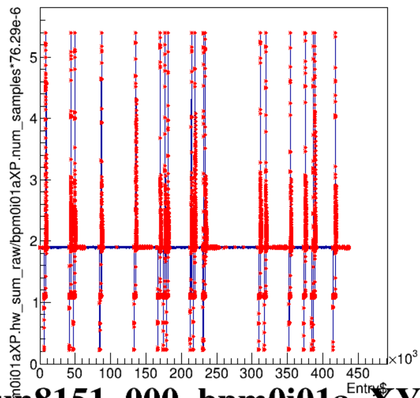
bpm0i01aXP.hw_sum_raw/bpm0i01aXP.num_samples*76.29e-6:Entry$
