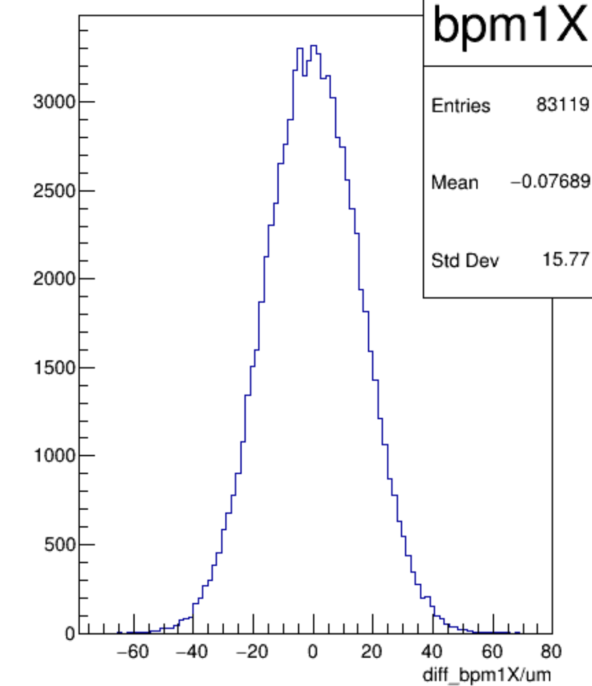
diff_bpm1X/um {ErrorFlag==0}
