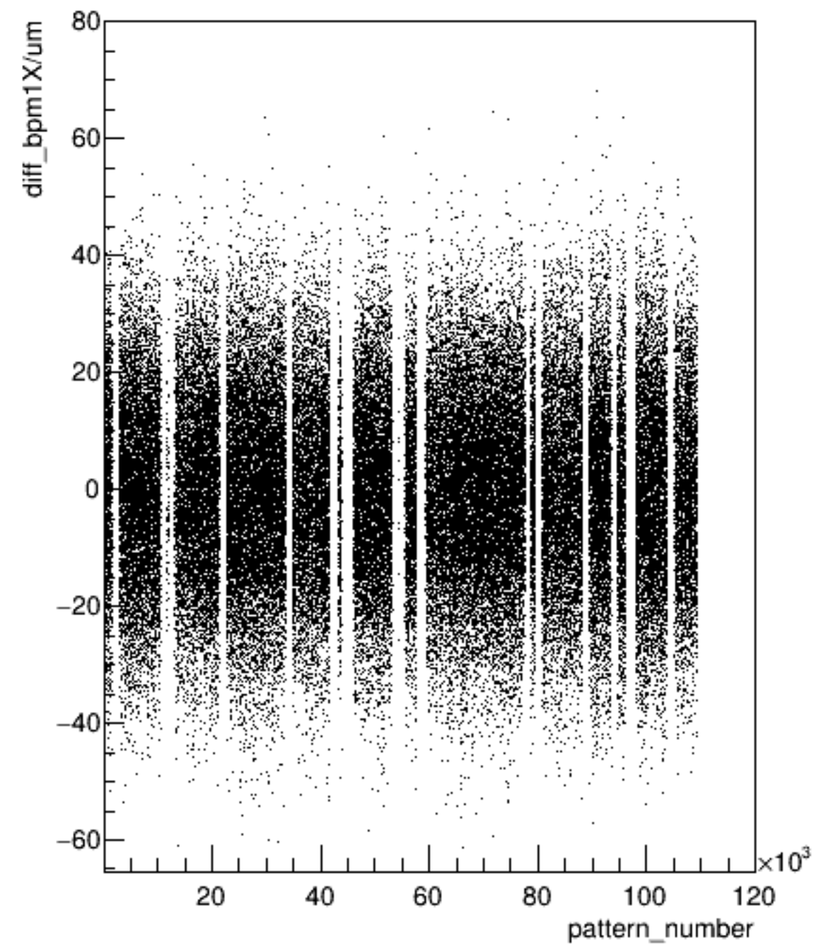
diff_bpm1X/um:pattern_number {ErrorFlag==0}
