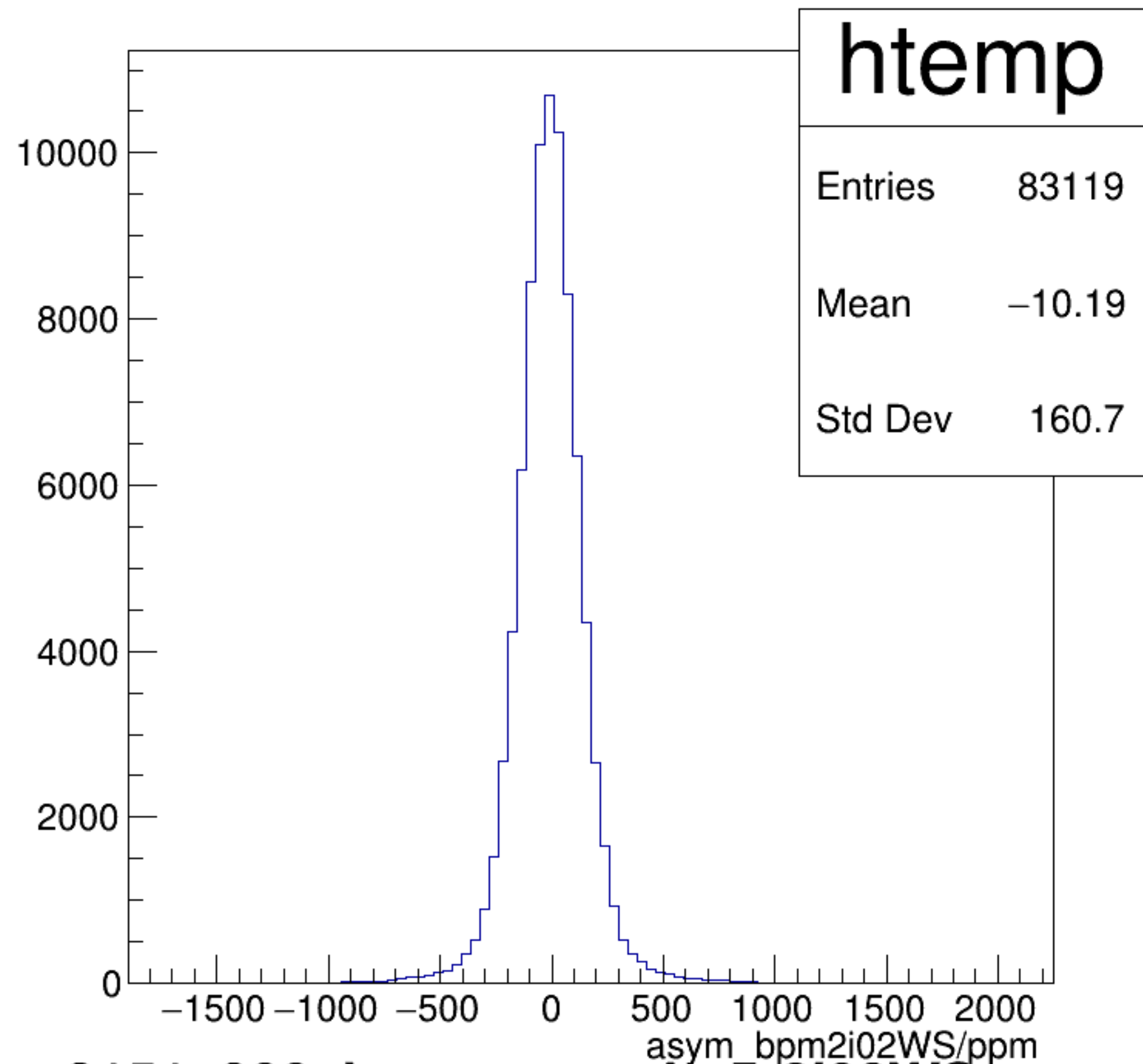
run8151_000_bpm_asym_bpm2i02WS.png
