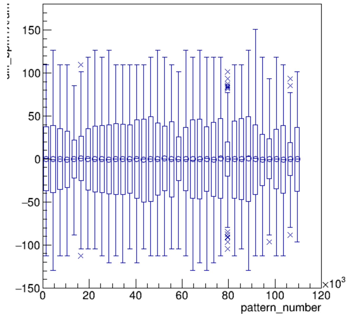
diff_bpm1X/um:pattern_number {ErrorFlag==0}
