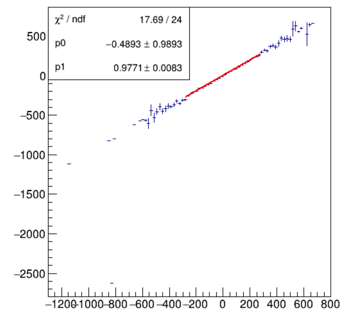
asym_bpm4ecWS/ppm:Aq/ppm {ErrorFlag==0}
