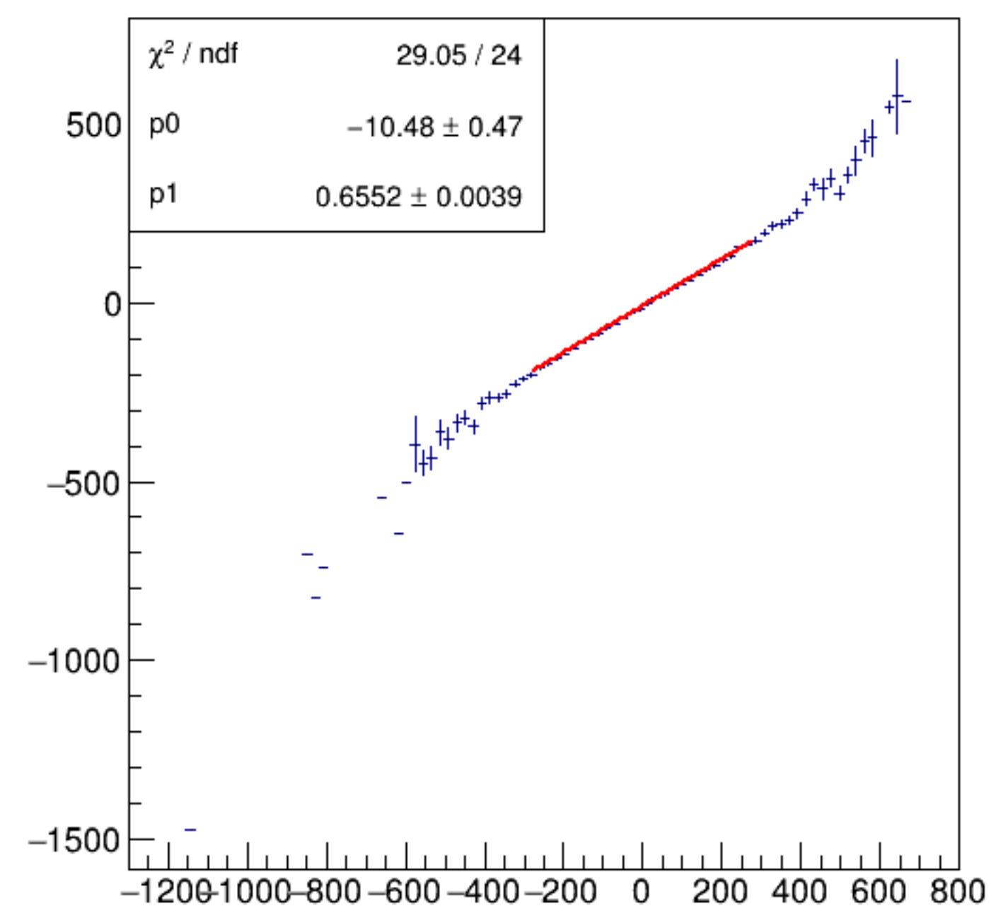
asym_bpm1i02WS/ppm:Aq/ppm {ErrorFlag==0}
