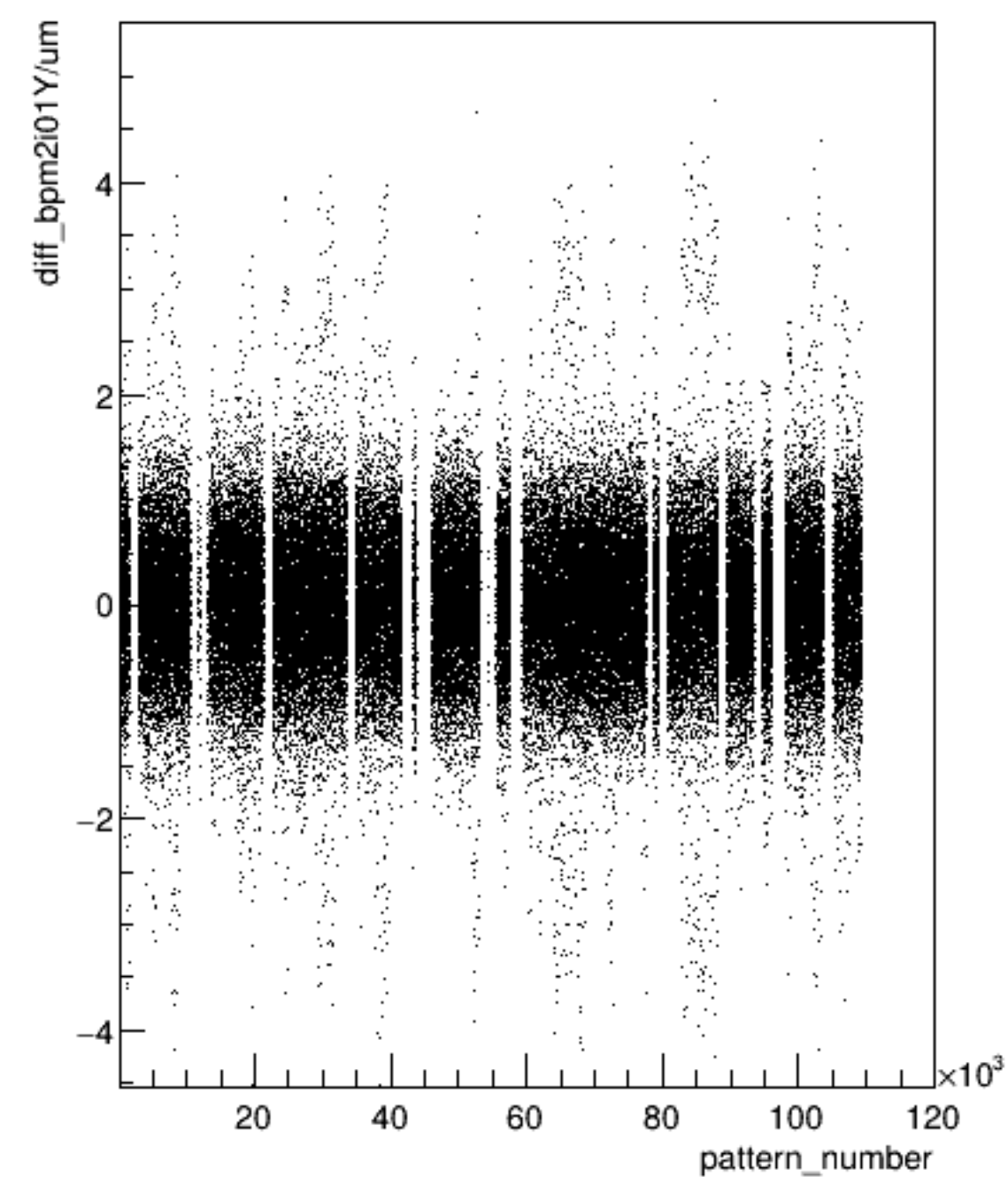
diff_bpm2i01Y/um:pattern_number {ErrorFlag==0}
