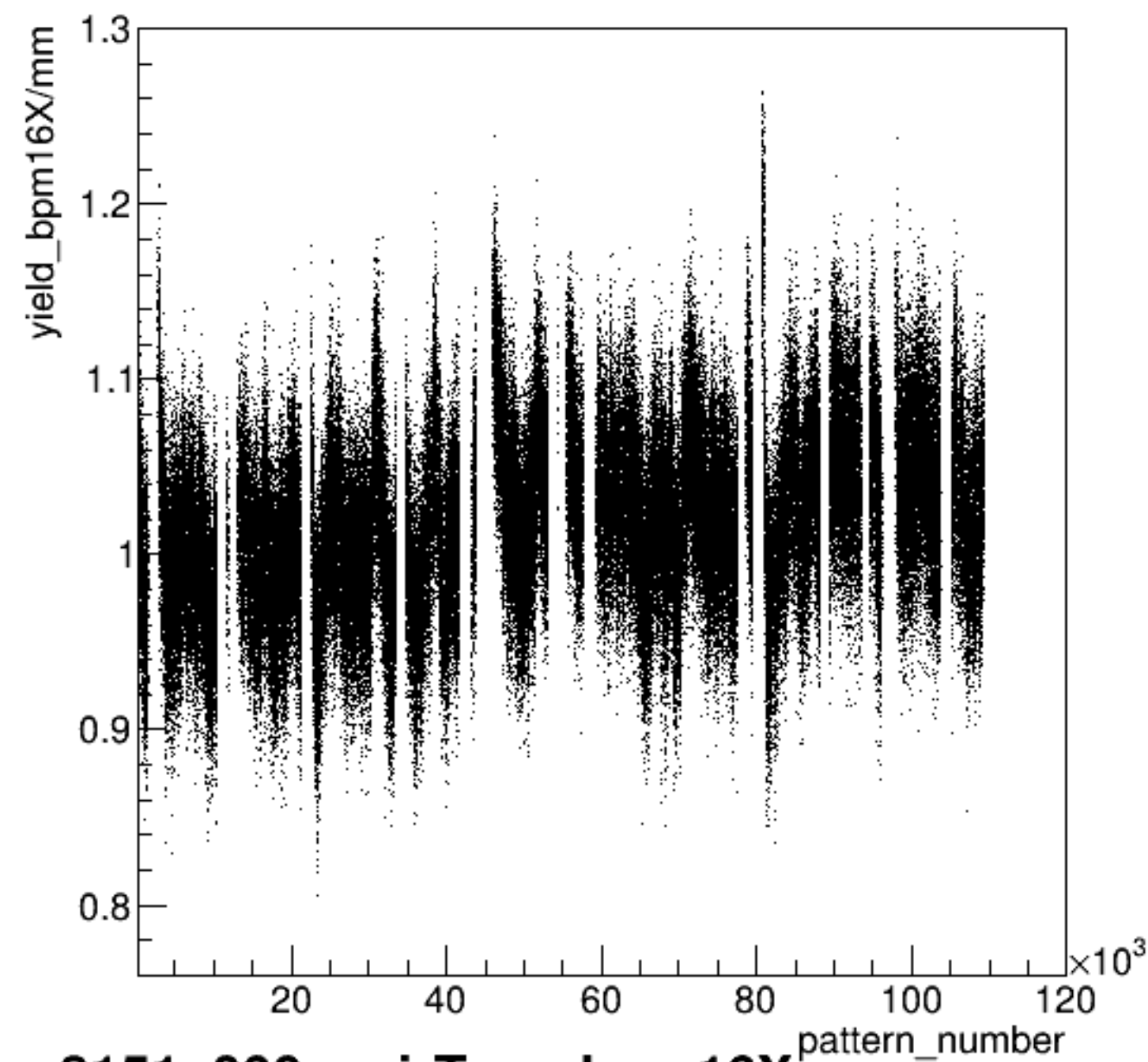
yield_bpm16X/mm:pattern_number {ErrorFlag==0}
