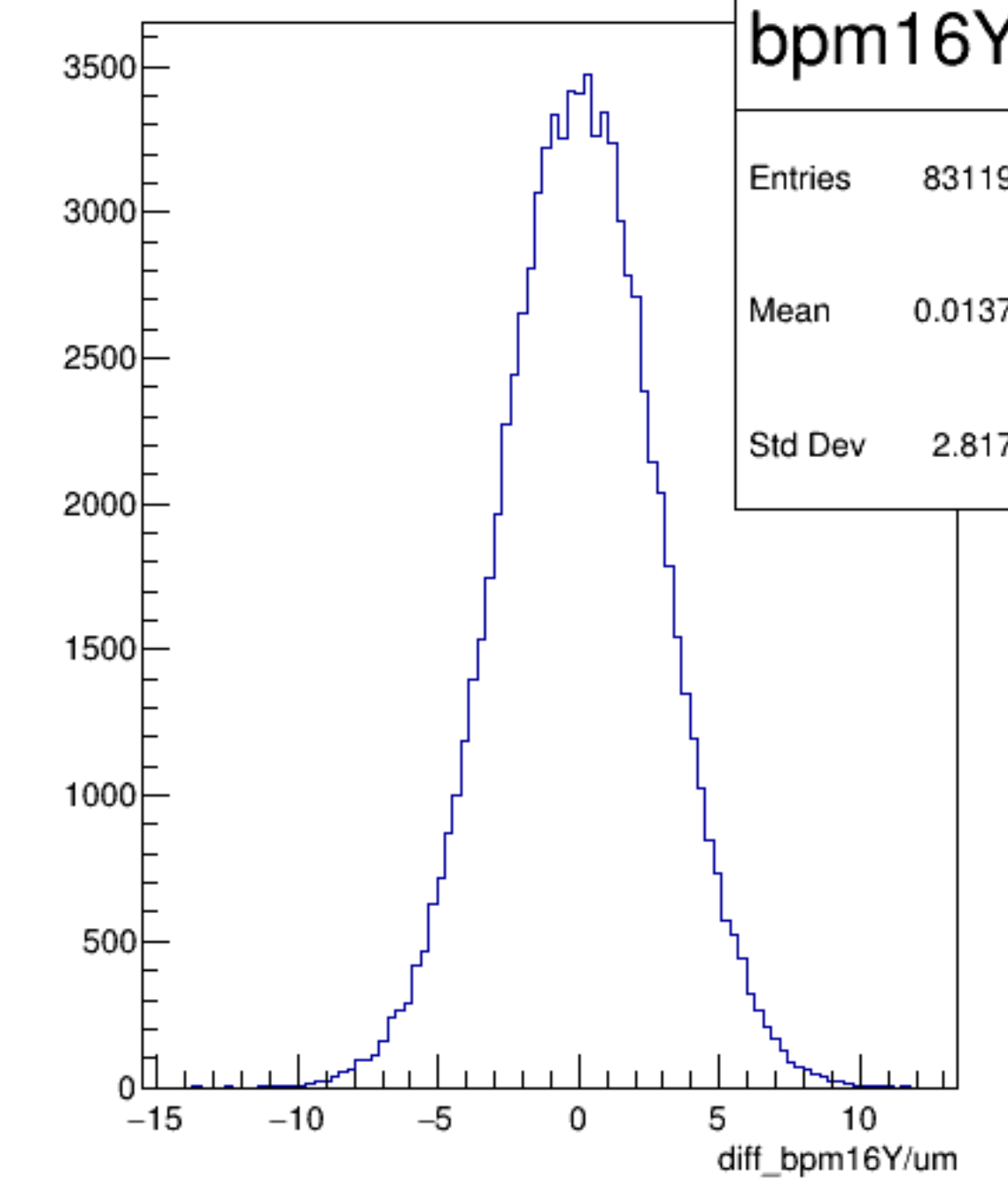
diff_bpm16Y/um {ErrorFlag==0}
