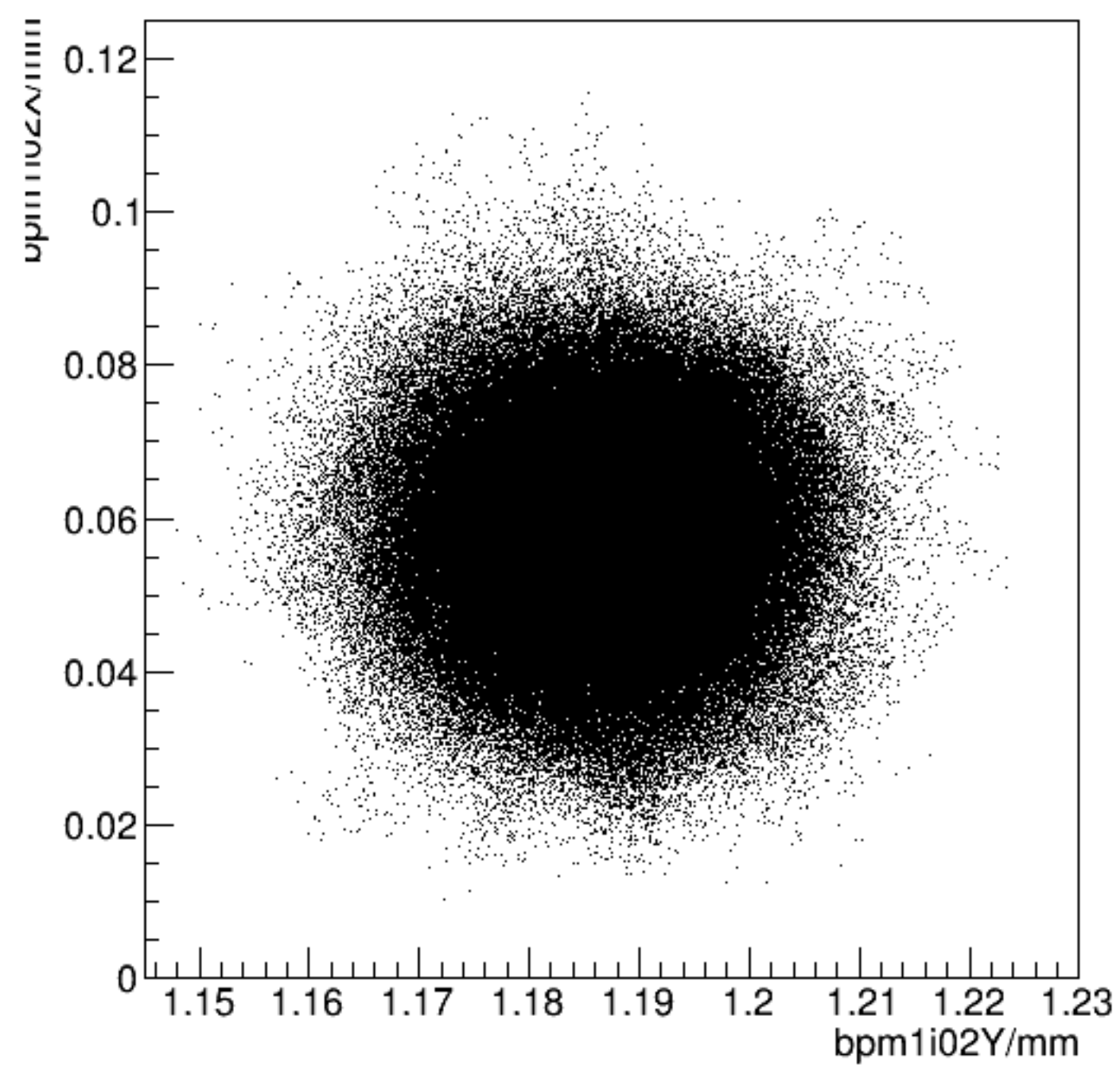
bpm1i02X/mm:bpm1i02Y/mm {ErrorFlag==0}
