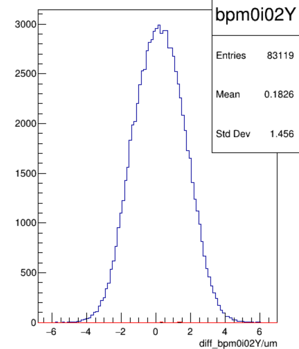
diff_bpm0i02Y/um {ErrorFlag==0}
