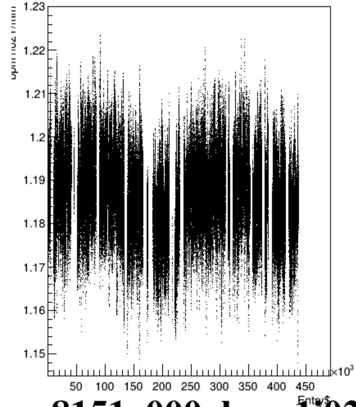
bpm1i02Y/mm:Entry$ {ErrorFlag==0}
