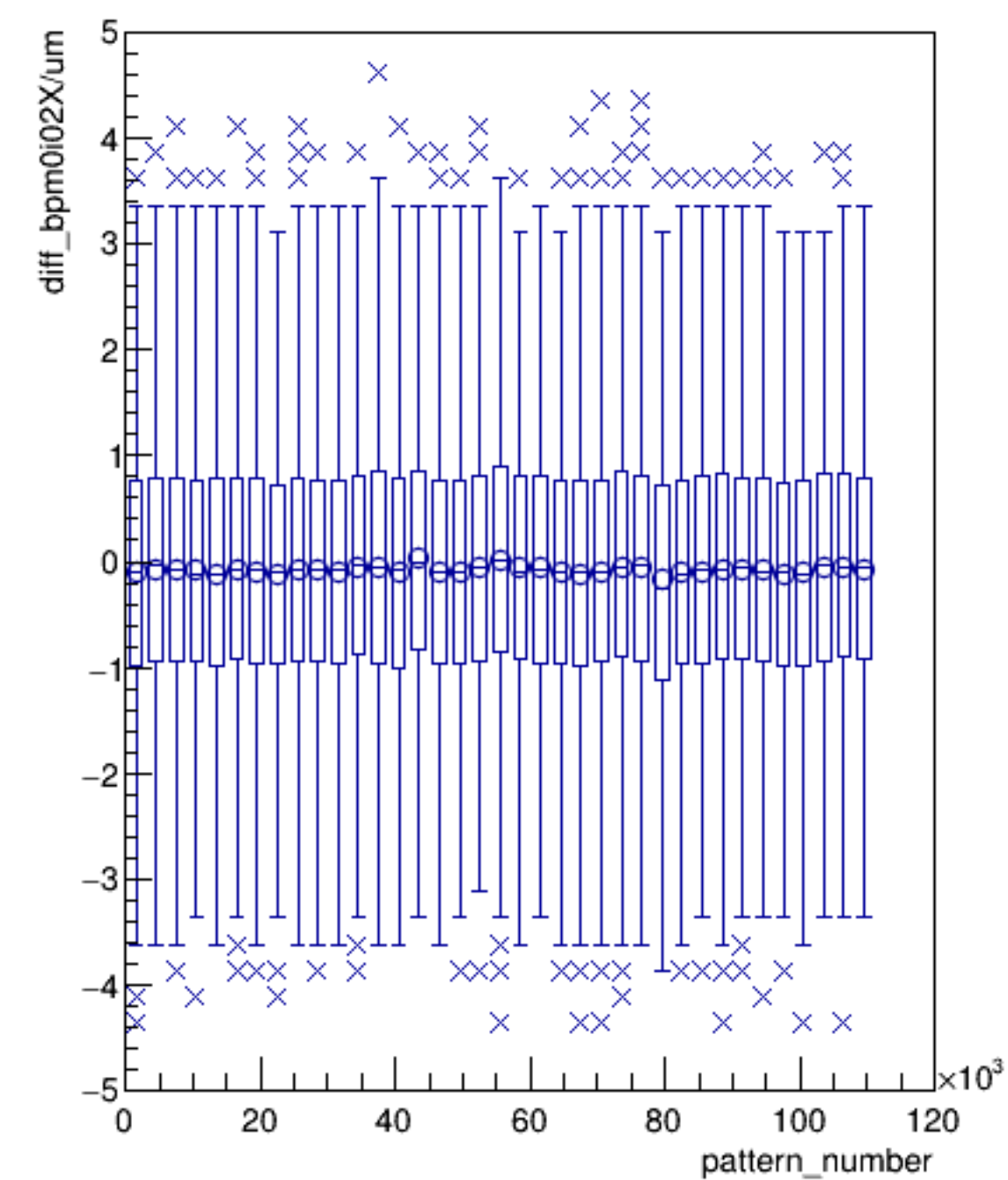
diff_bpm0i02X/um:pattern_number (ErrorFlag==0)
