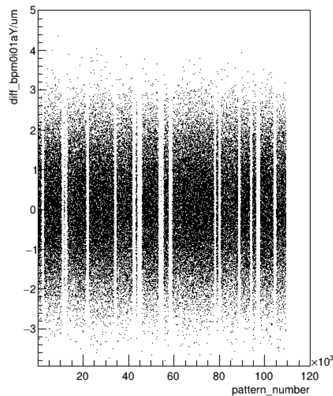
diff_bpm0i01aY/um:pattern_number (ErrorFlag==0)
