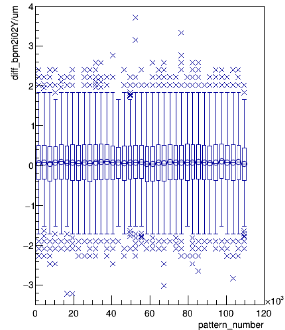
diff_bpm2i02Y/um:pattern_number (ErrorFlag==0)
