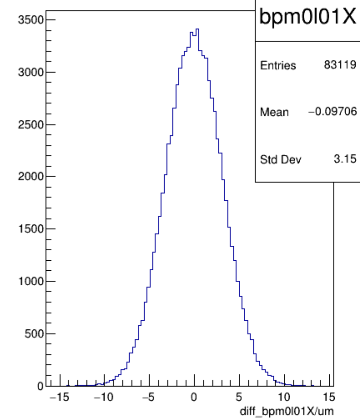
diff_bpm0l01X/um {ErrorFlag==0}
