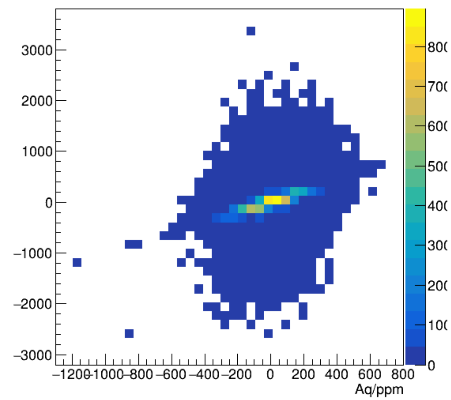
asym_bpm4ecWS/ppm:Aq/ppm {ErrorFlag==0}
