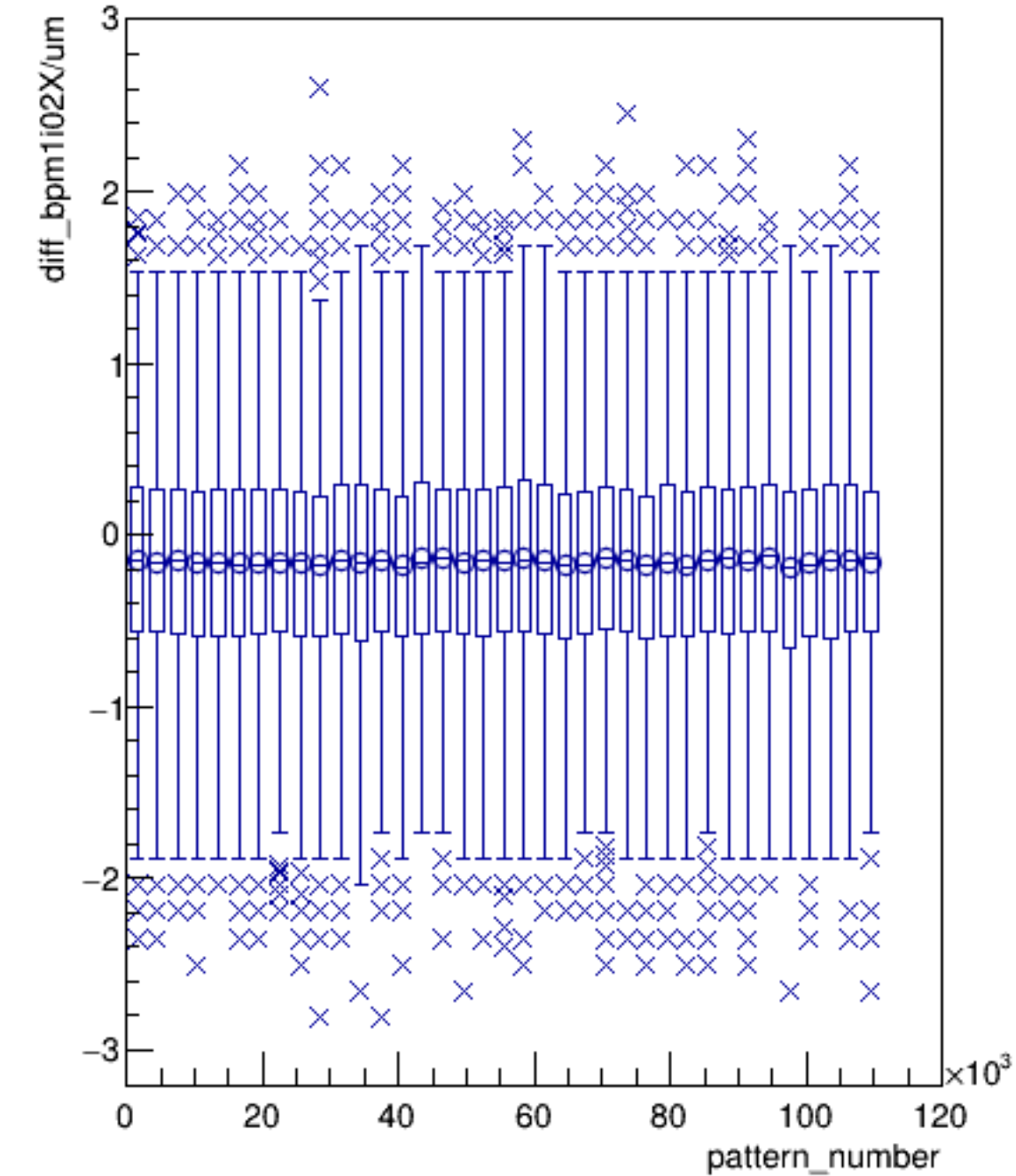
diff_bpm1i02X/um:pattern_number (ErrorFlag==0)
