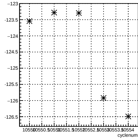
1X_coil1:cyclenum {run == 8156}
