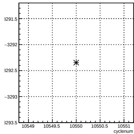
usr_coil6:cyclenum {run == 8156}
