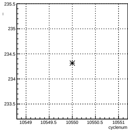
4eX_coil7:cyclenum {run == 8156}
