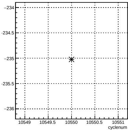
12X_coil6:cyclenum {run == 8156}
