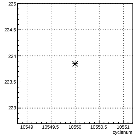
1X_coil7:cyclenum {run == 8156}
