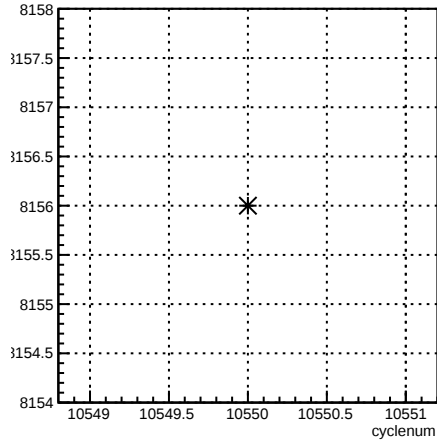
run:cyclenum {run == 8156}
