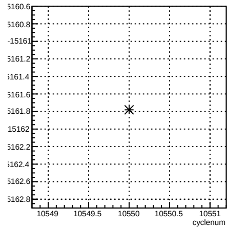
usr_coil1:cyclenum {run == 8156}
