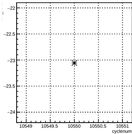
4eX_coil3:cyclenum {run == 8156}
