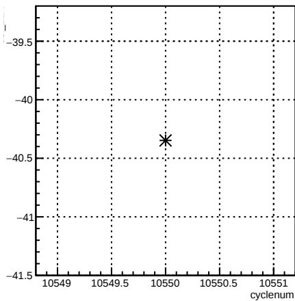
usl_12X:cyclenum {run == 8156}
