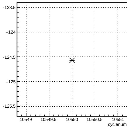
4eX_coil1:cyclenum {run == 8156}
