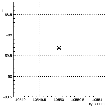
12X_coil7:cyclenum {run == 8156}
