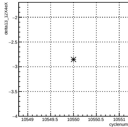
delta13_12X4eX:cyclenum {run == 8156}
