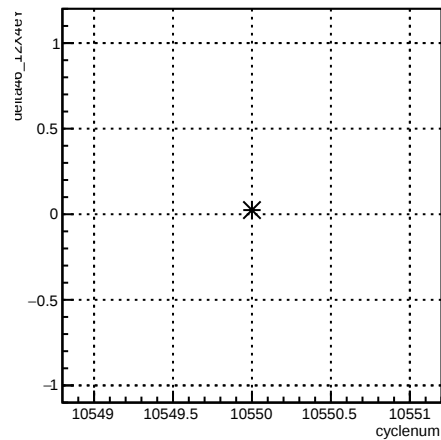
delta46_12X4eY:cyclenum {run == 8156}
