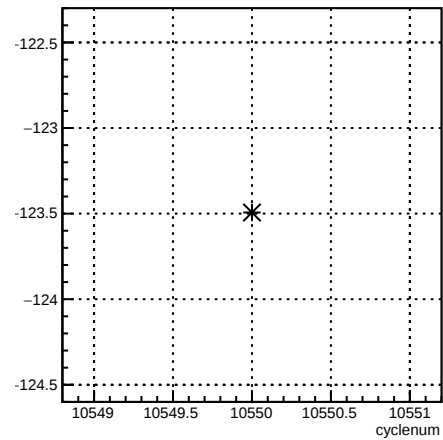
usr_4eY:cyclenum {run == 8156}
