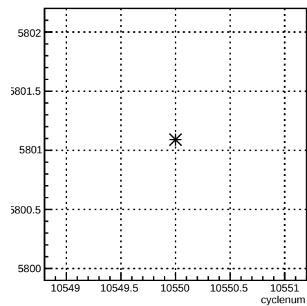
usr_coil4:cyclenum {run == 8156}
