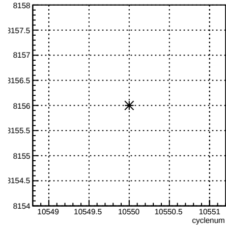
run:cyclenum {run == 8156}
