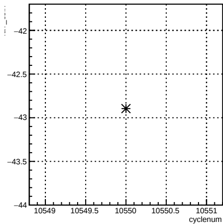
4eY_coil7:cyclenum {run == 8156}
