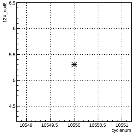
12X_coil6:cyclenum {run == 8156}
