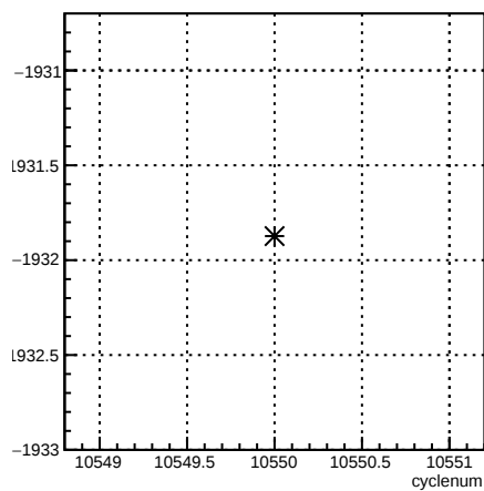
usr_coil3:cyclenum {run == 8156}
