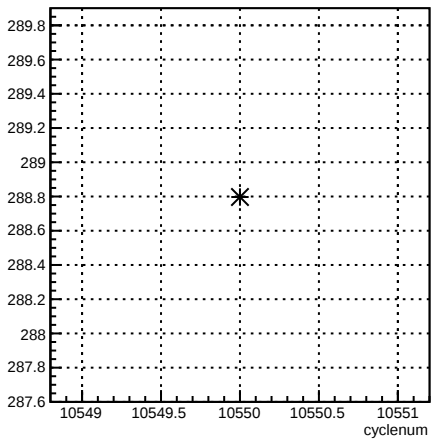
4eY_coil4:cyclenum {run == 8156}
