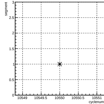
segment:cyclenum {run == 8156}
