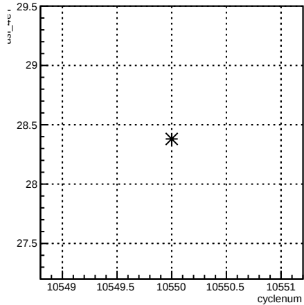
usl_4eY:cyclenum {run == 8156}
