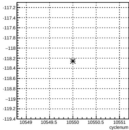
4eY_coil6:cyclenum {run == 8156}
