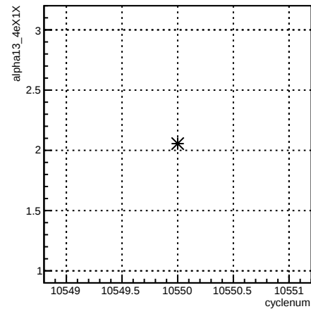
alpha13_4eX1X:cyclenum {run == 8156}
