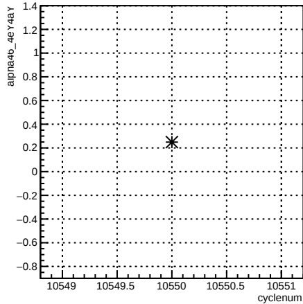
alpha46_4eY4aY:cyclenum {run == 8156}
