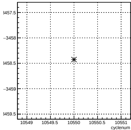
usl_coil6:cyclenum {run == 8156}
