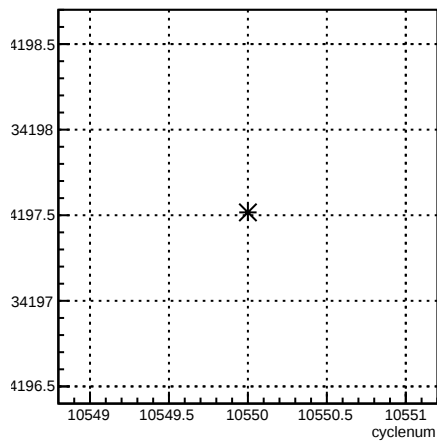
usr_coil7:cyclenum {run == 8156}
