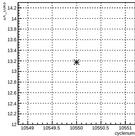
4eX_coil3:cyclenum {run == 8156}
