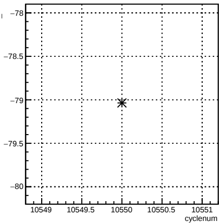
usl_4eY:cyclenum {run == 8156}
