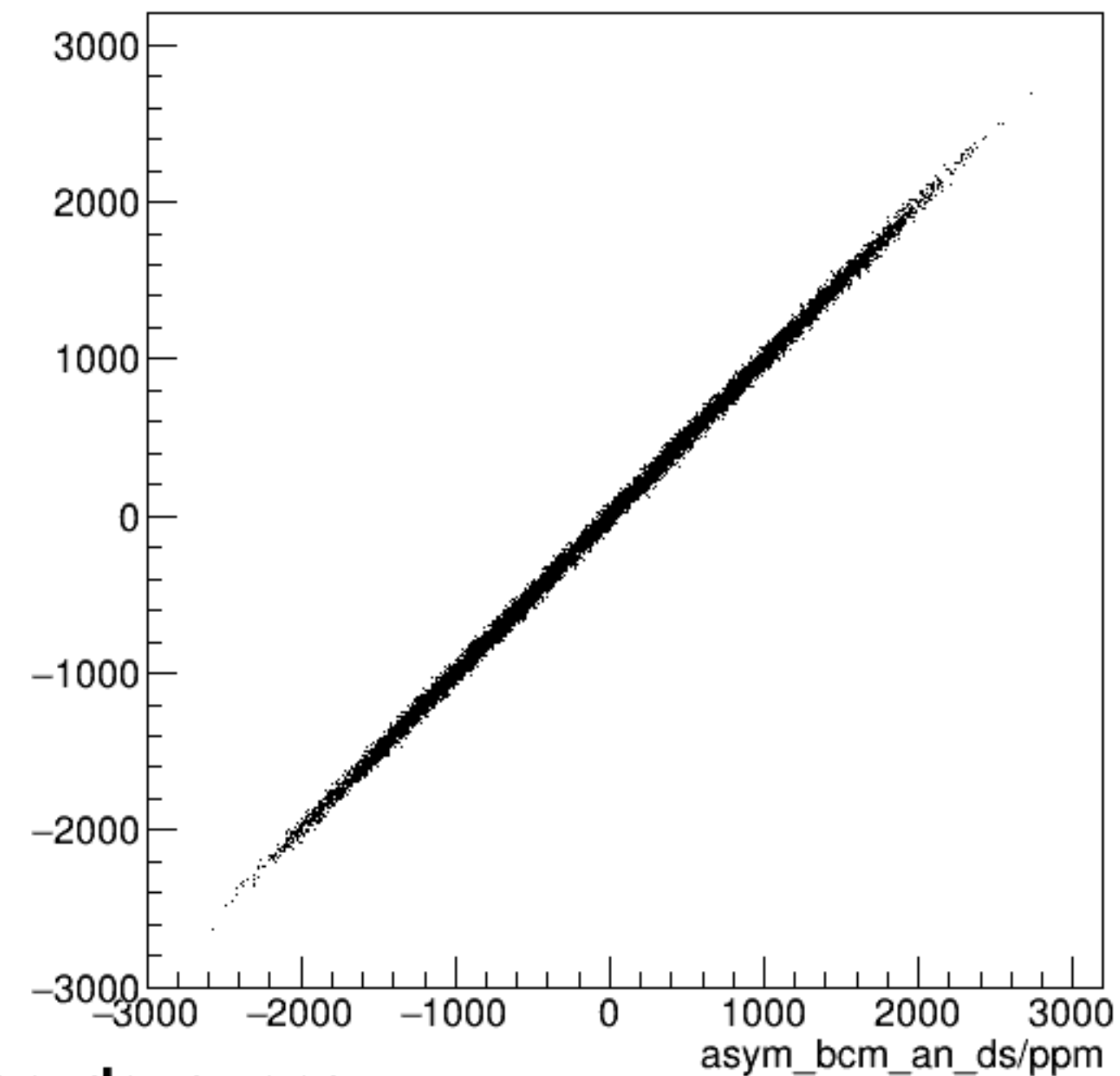
run8189_000_asym_bcm_an_us_vs_asym_bcm_an_ds_pr.png
