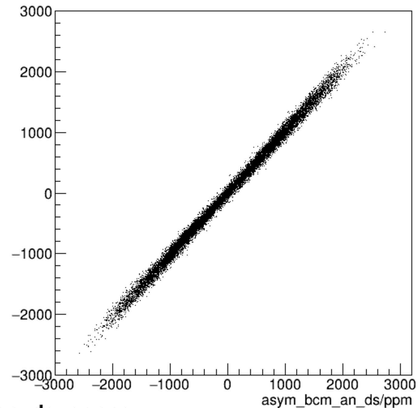
run8189_000_asym_bcm_dg_us_vs_asym_bcm_an_ds_pr.png
