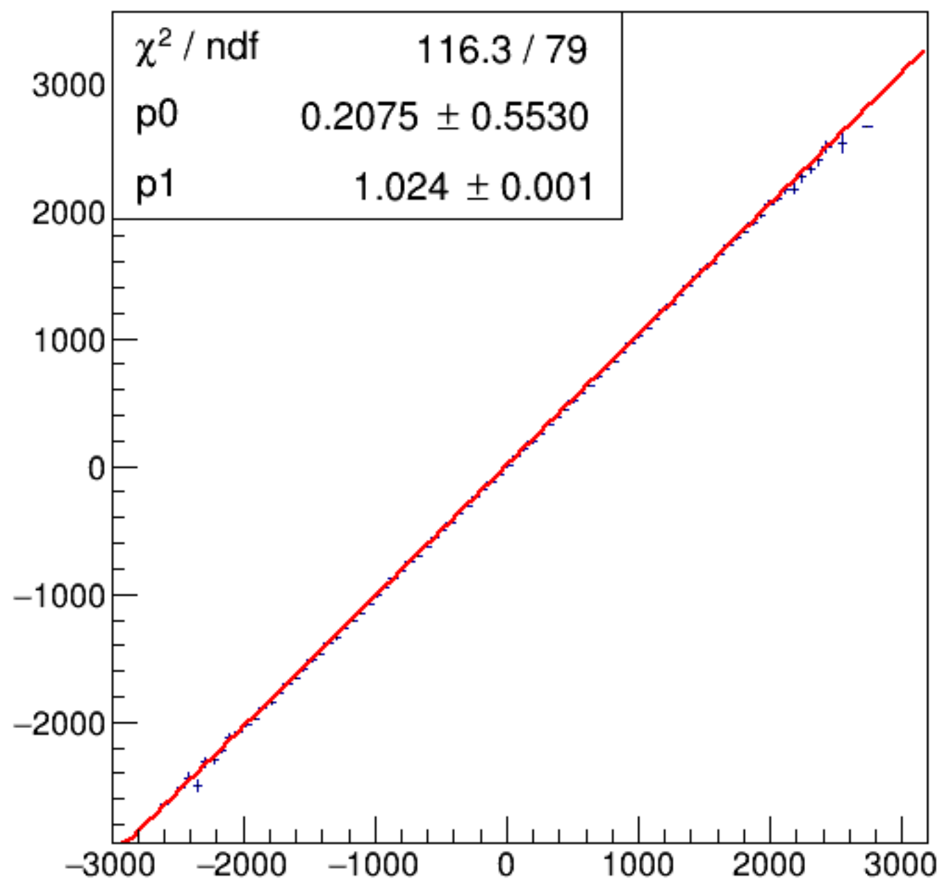
run8189_000_asym_bcm_dg_us_vs_asym_bcm_an_ds_pr.png
