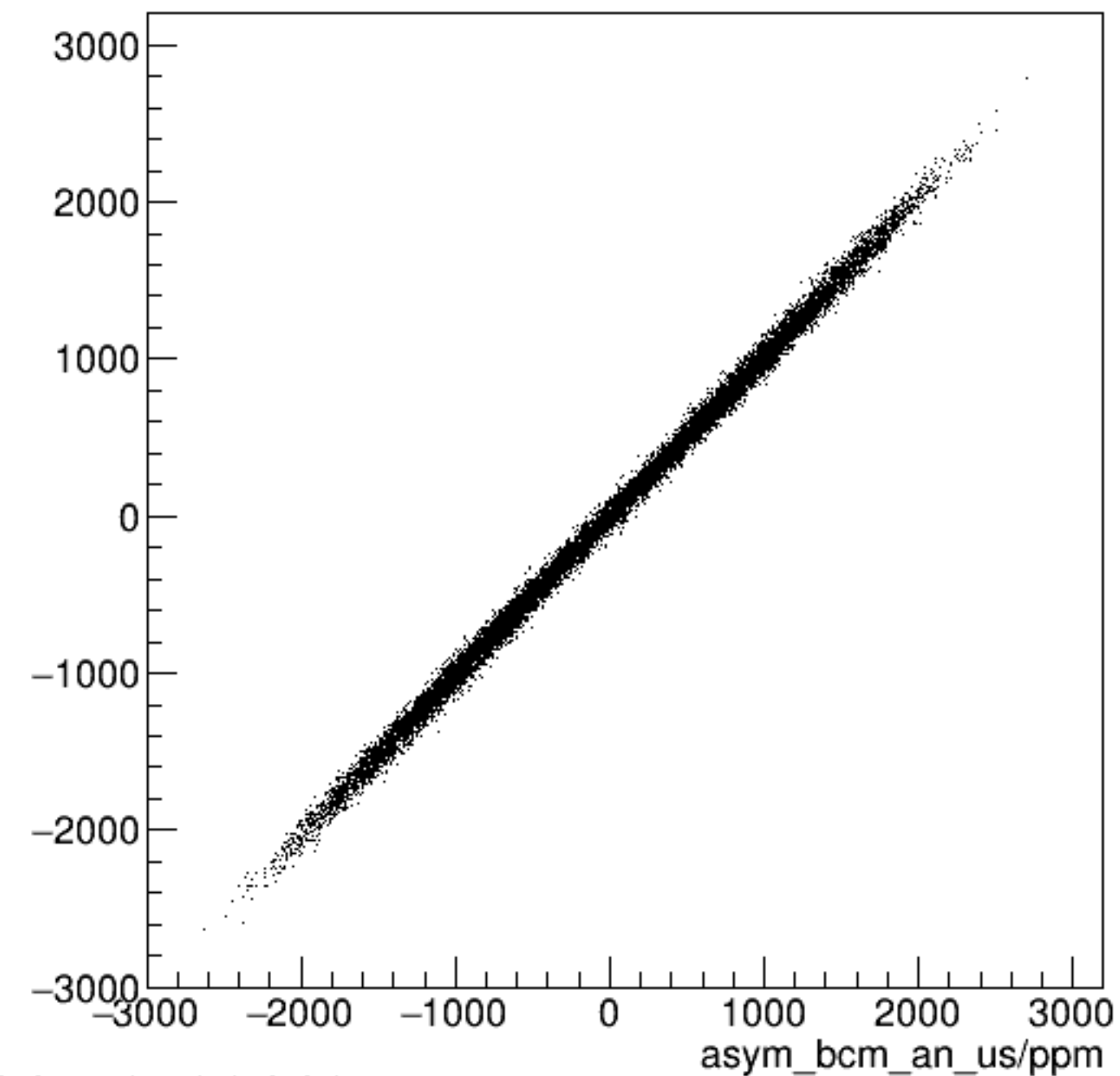
run8189_000_asym_bcm_dg_ds_vs_asym_bcm_an_us_pr.png
