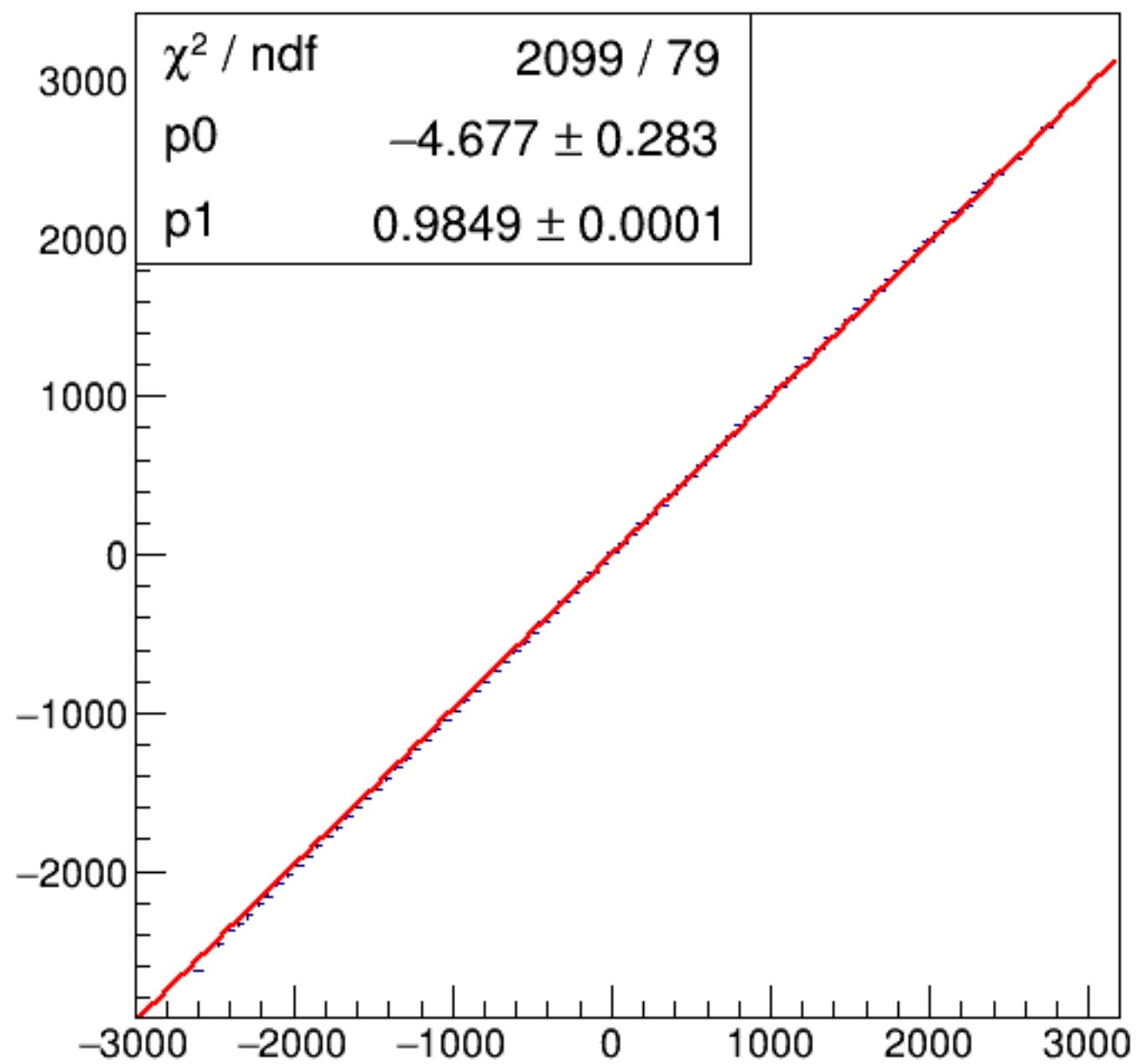
run8189_000_asym_bcm_an_us_vs_asym_bcm_an_ds_pr.png
