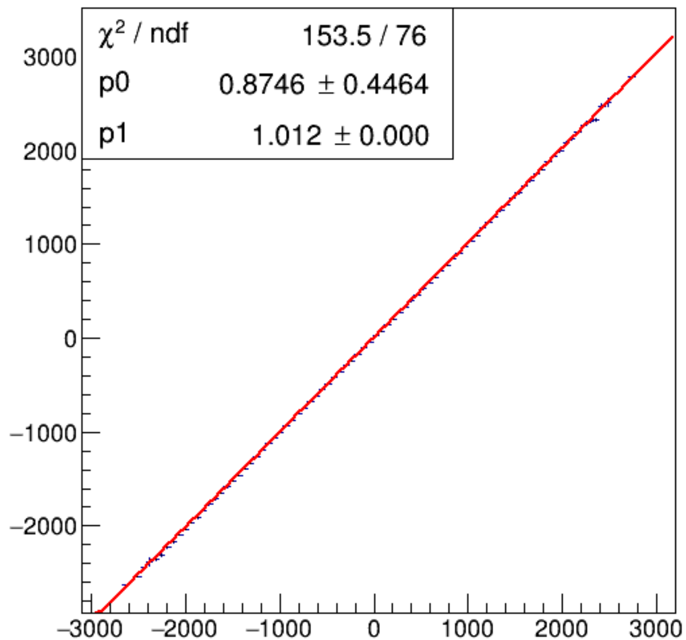
run8189_000_asym_bcm_dg_ds_vs_asym_bcm_an_us_pr.png
