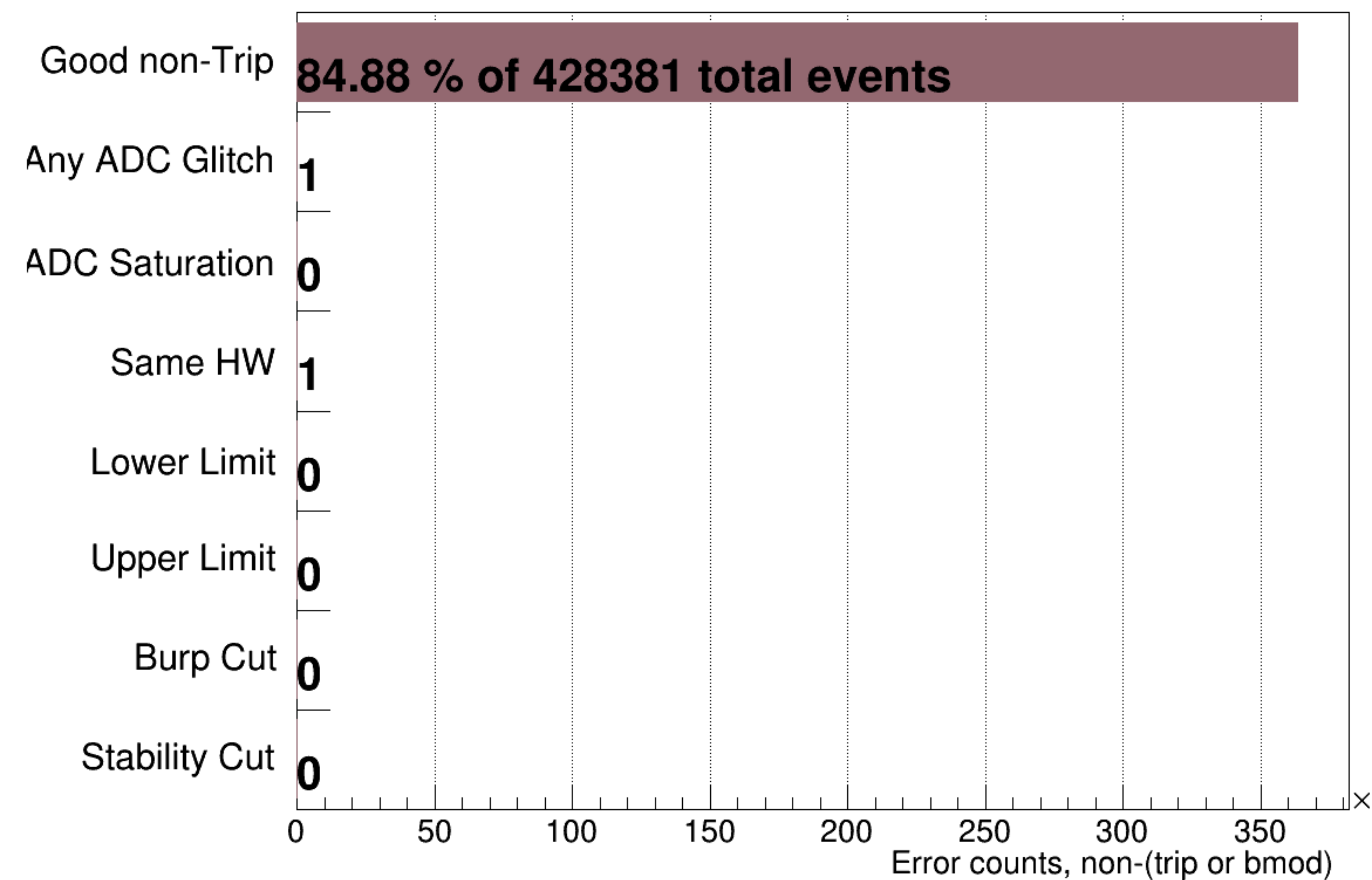
sam6's Device Error Counter &amp; Not (Trip || BMOD)
