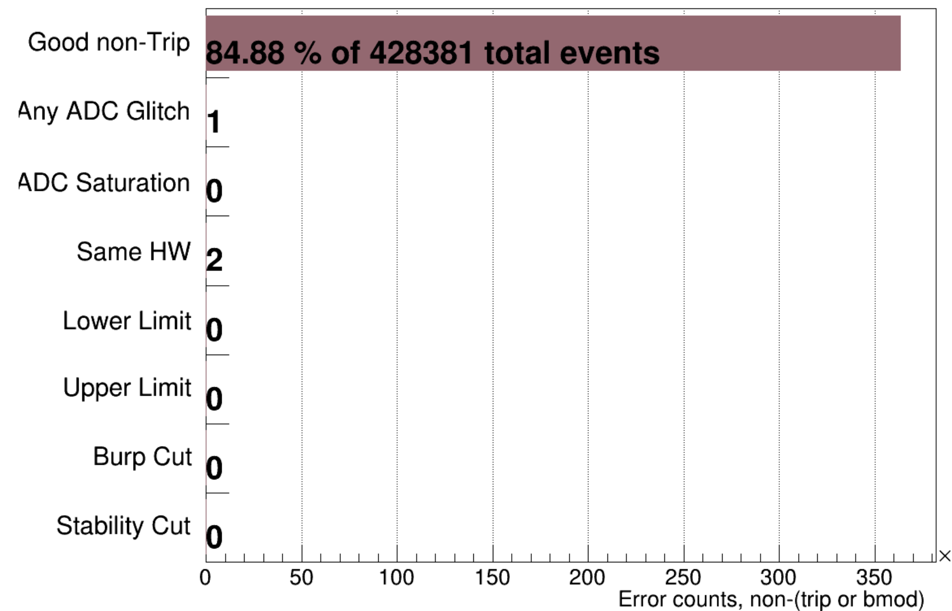
sam7's Device Error Counter &amp; Not (Trip || BMOD)
