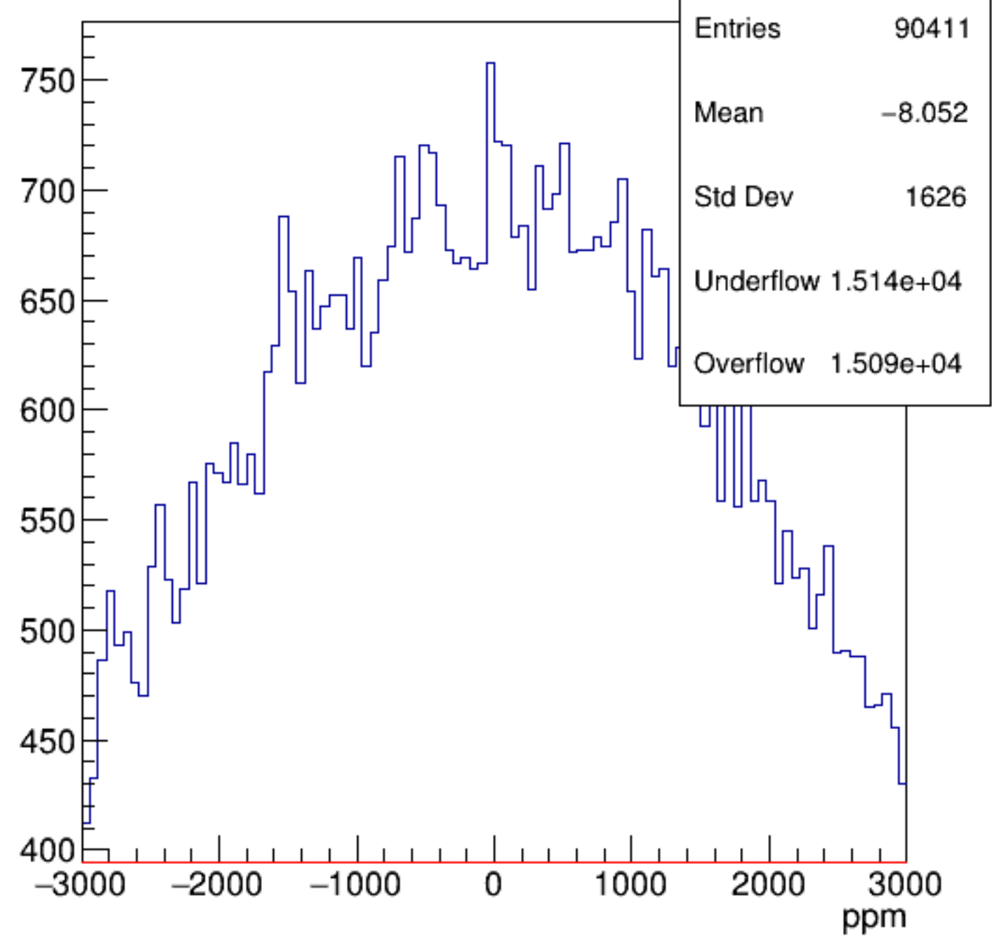
asym_sam3
