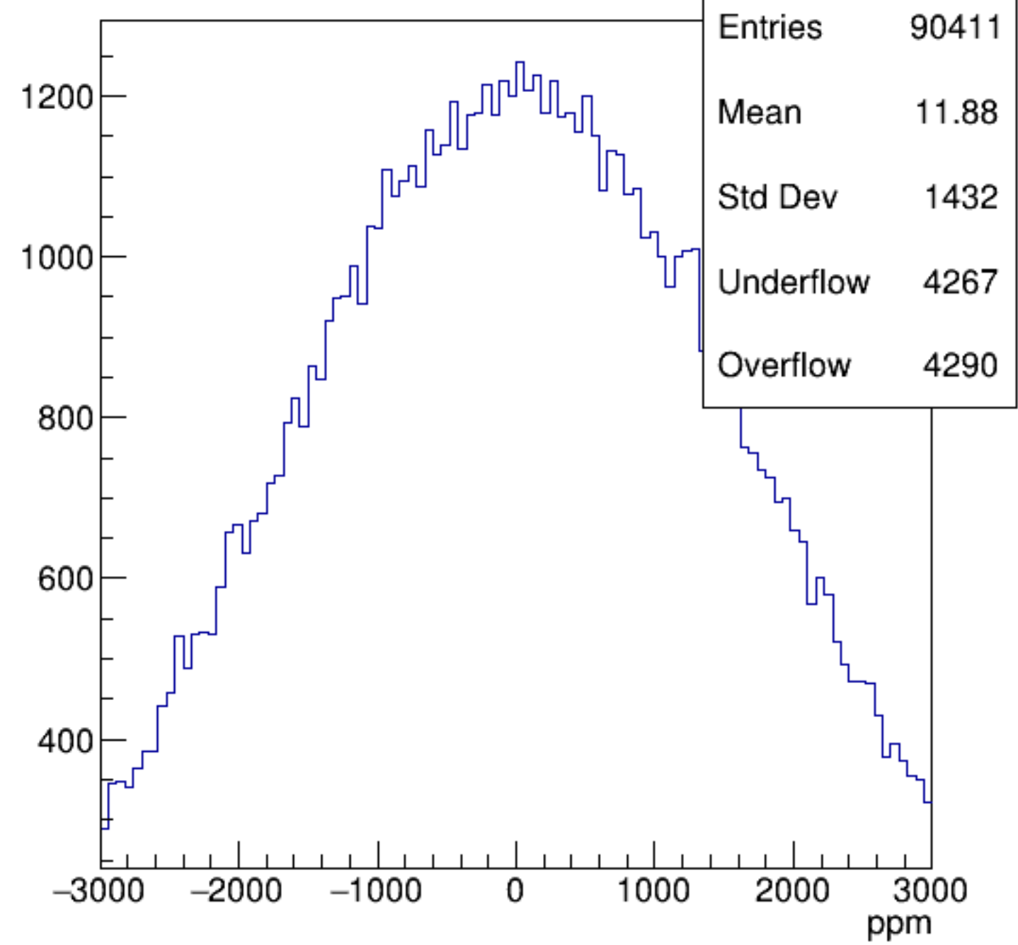
asym_sam6
