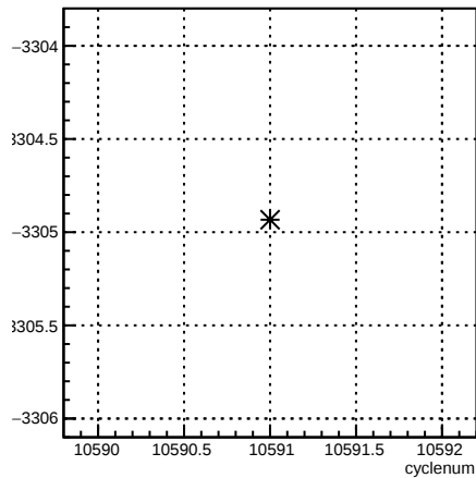
usr_coil6:cyclenum {run == 8167}
