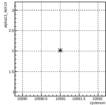
alpha13_4eX1X:cyclenum {run == 8167}
