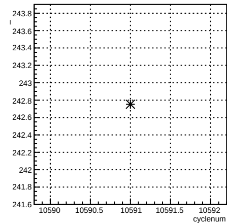
4eX_coil7:cyclenum {run == 8167}
