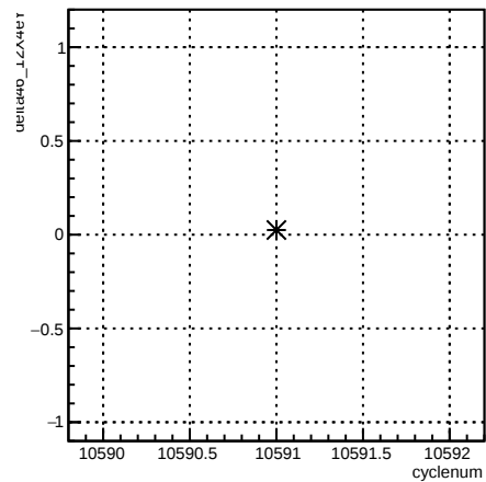
delta46_12X4eY:cyclenum {run == 8167}
