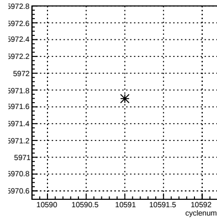
usr_coil4:cyclenum {run == 8167}
