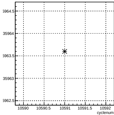
usr_coil7:cyclenum {run == 8167}
