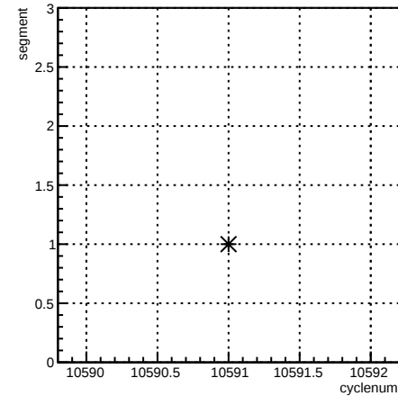
segment:cyclenum {run == 8167}
