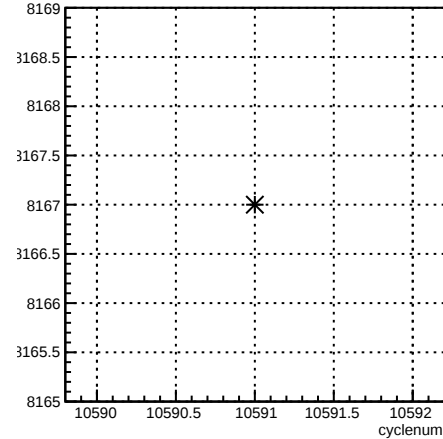
run:cyclenum {run == 8167}
