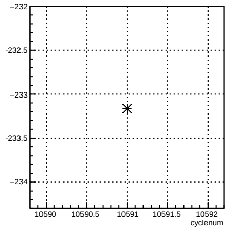
12X_coil1:cyclenum {run == 8167}
