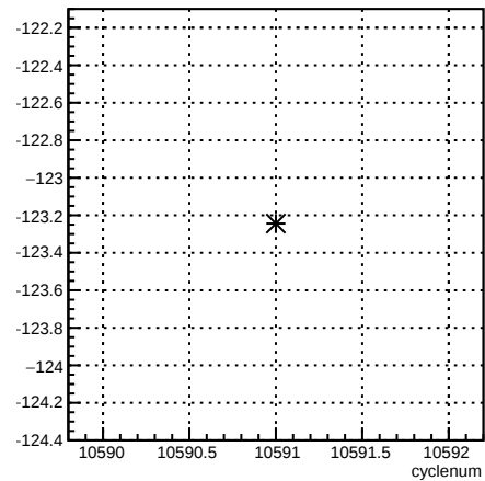
4eX_coil1:cyclenum {run == 8167}
