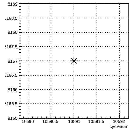
run:cyclenum {run == 8167}
