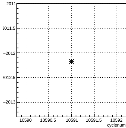
usr_coil3:cyclenum {run == 8167}
