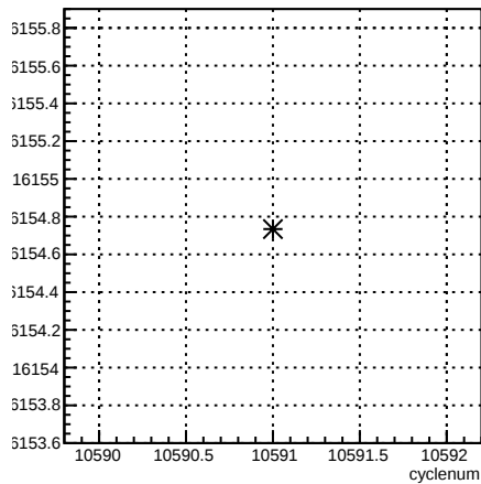
usl_coil6:cyclenum {run == 8167}
