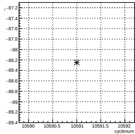
usl_4eY:cyclenum {run == 8167}
