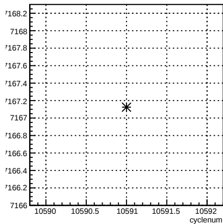
usl_coil7:cyclenum {run == 8167}
