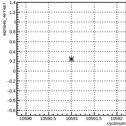
alpha46_4eY4aY:cyclenum {run == 8167}
