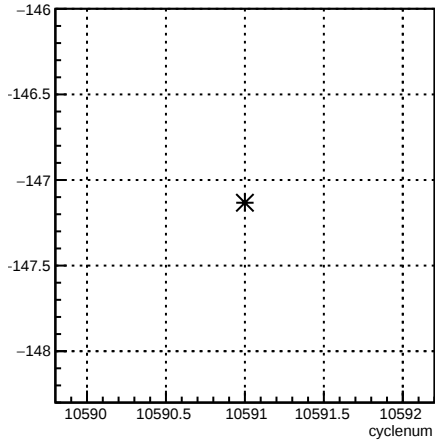
4eY_coil6:cyclenum {run == 8167}
