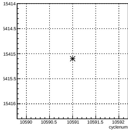
usr_coil1:cyclenum {run == 8167}
