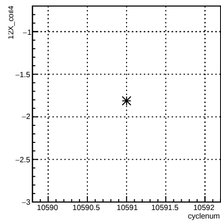
12X_coil4:cyclenum {run == 8167}
