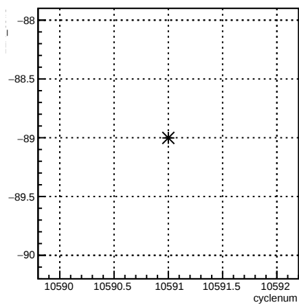
12X_coil3:cyclenum {run == 8167}
