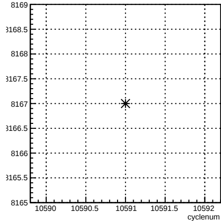
run:cyclenum {run == 8167}
