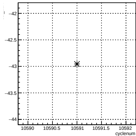
usl_12X:cyclenum {run == 8167}
