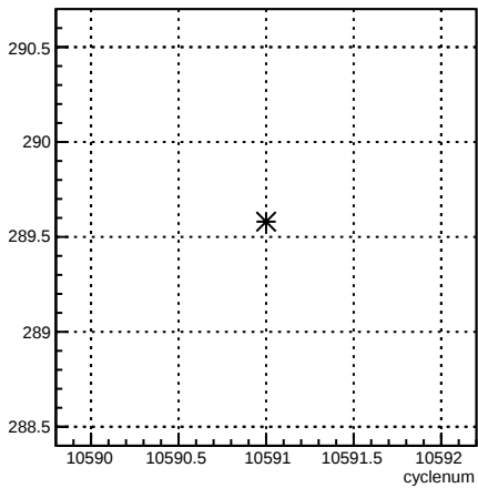
4eY_coil4:cyclenum {run == 8167}
