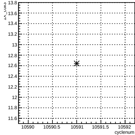
4eX_coil3:cyclenum {run == 8167}
