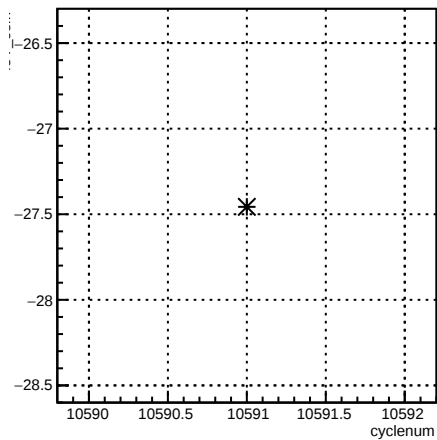
4eY_coil7:cyclenum {run == 8167}
