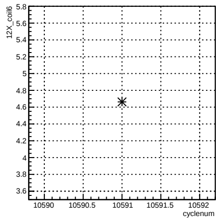
12X_coil6:cyclenum {run == 8167}
