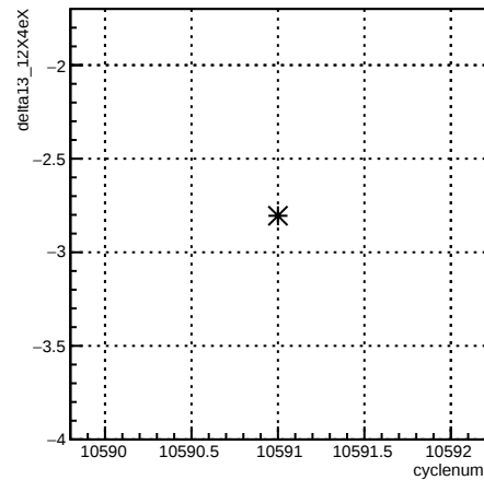
delta13_12X4eX:cyclenum {run == 8167}
