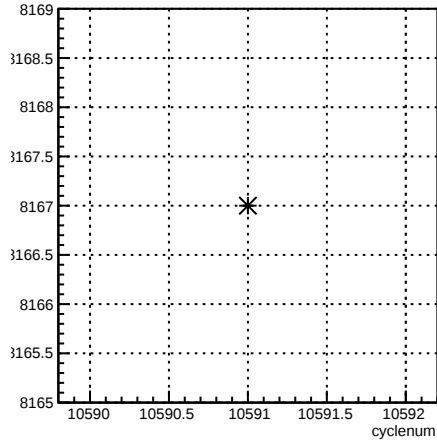
run:cyclenum {run == 8167}
