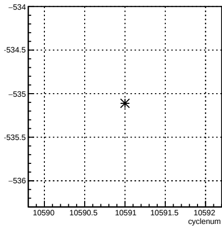
12X_coil7:cyclenum {run == 8167}
