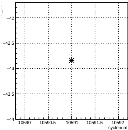
usr_12X:cyclenum {run == 8167}
