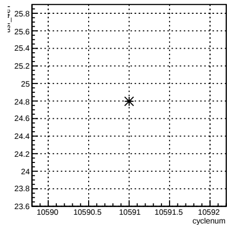
usr_4eY:cyclenum {run == 8167}
