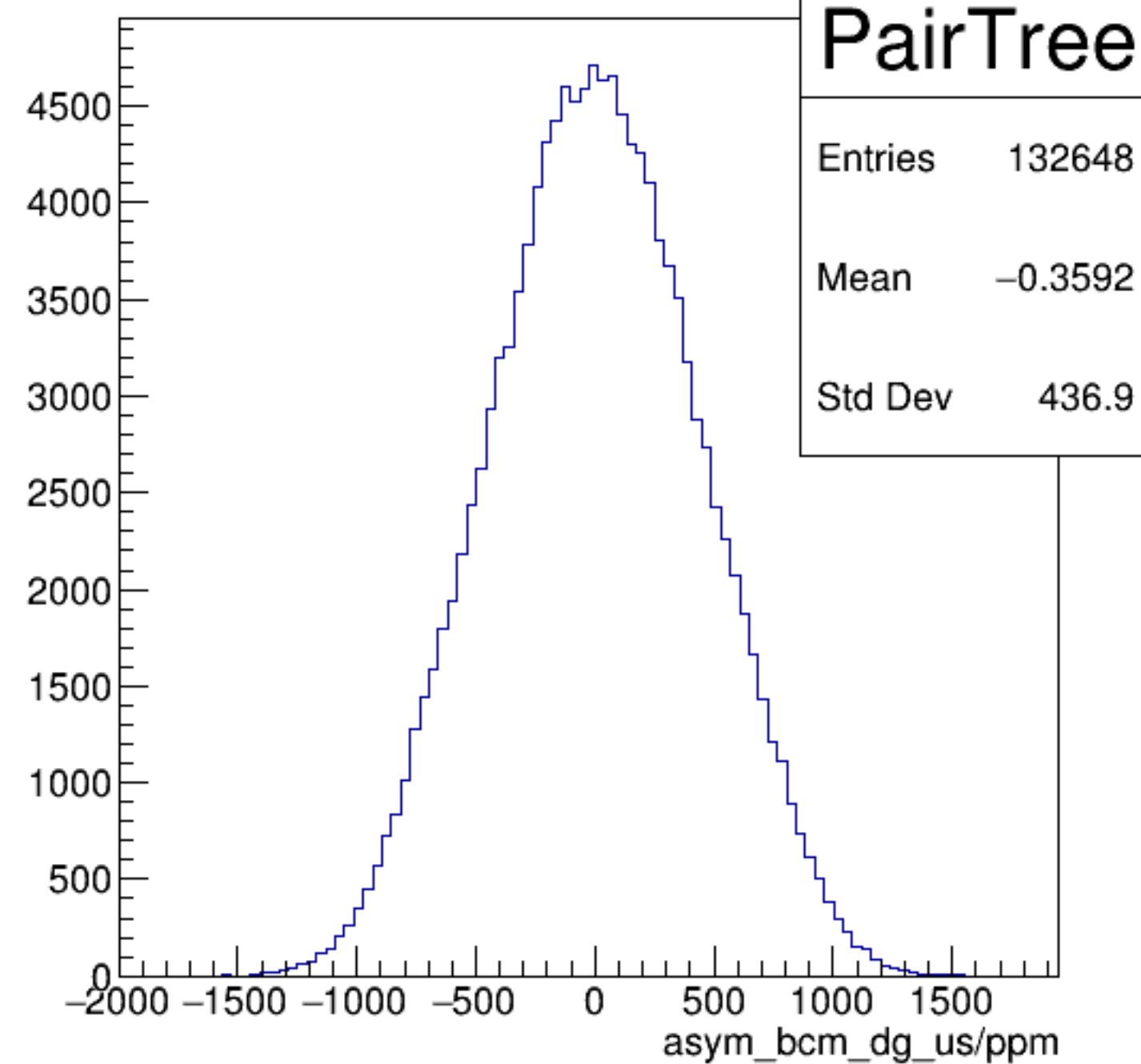
asym_bcm_dg_us/ppm {ErrorFlag==0}
