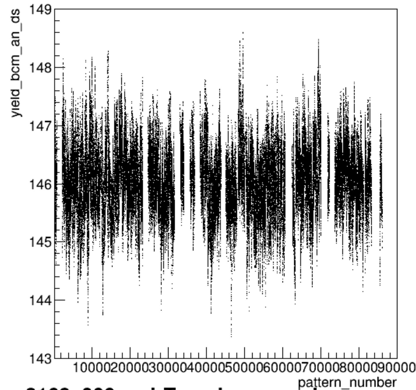
yield_bcm_an_ds:pattern_number {ErrorFlag==0}
