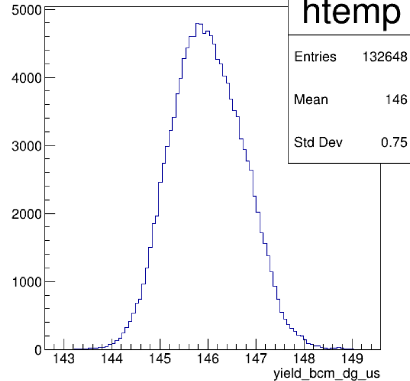
yield_bcm_dg_us {ErrorFlag==0}
