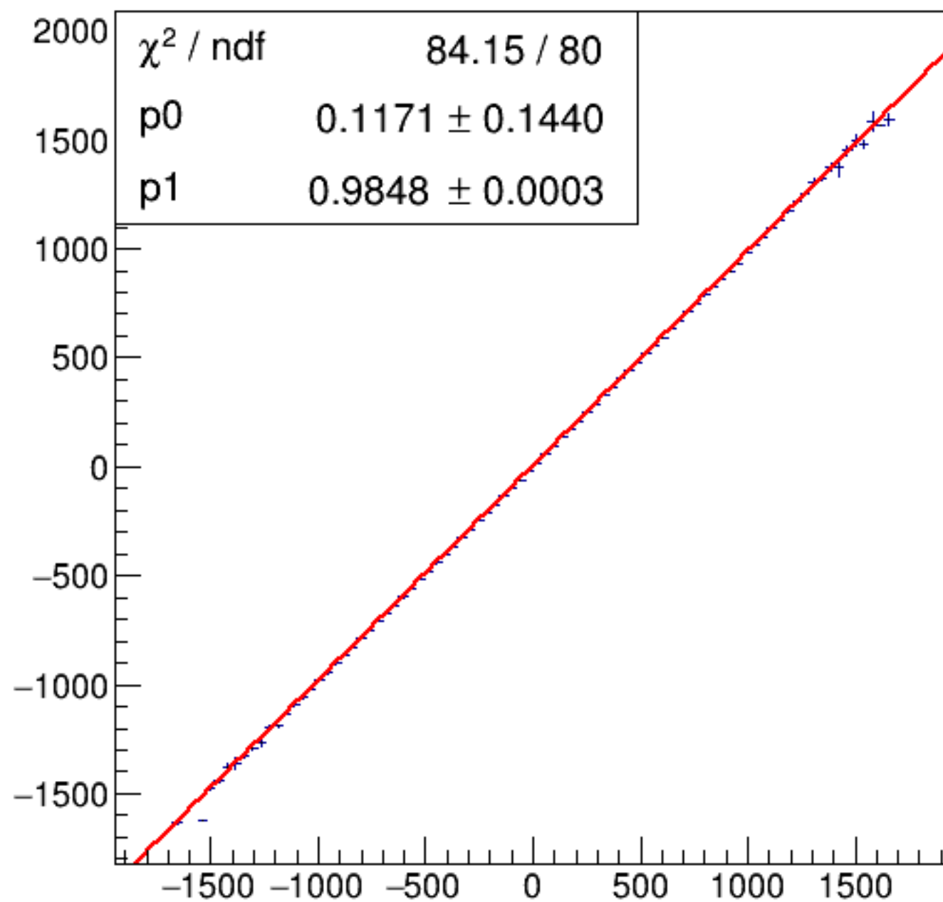
run8168_000_asym_bcm_dg_ds_vs_asym_bcm_an_us_pr.png
