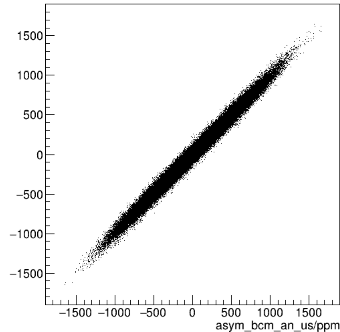
run8168_000_asym_bcm_dg_ds_vs_asym_bcm_an_us_pr.png
