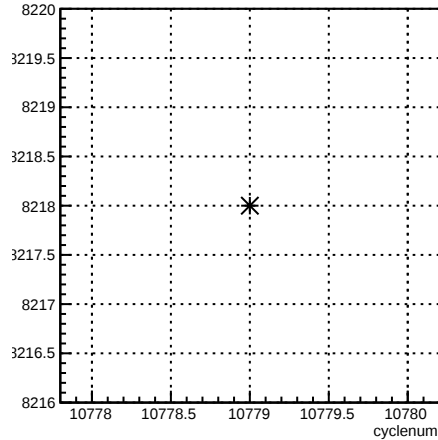
run:cyclenum {run == 8218}
