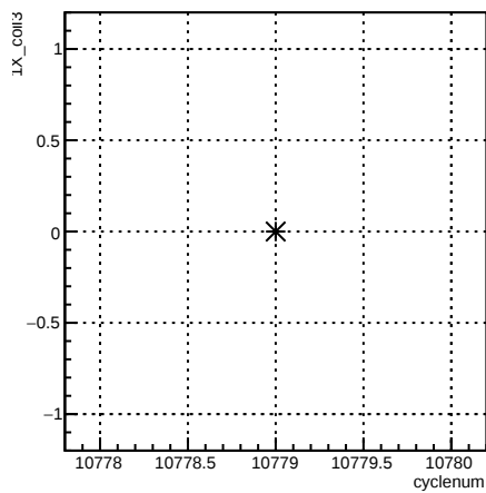
1X_coil3:cyclenum {run == 8218}
