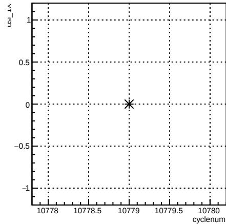
usl_4eY:cyclenum {run == 8218}
