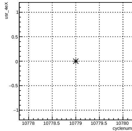
run:cyclenum {run == 8218}
