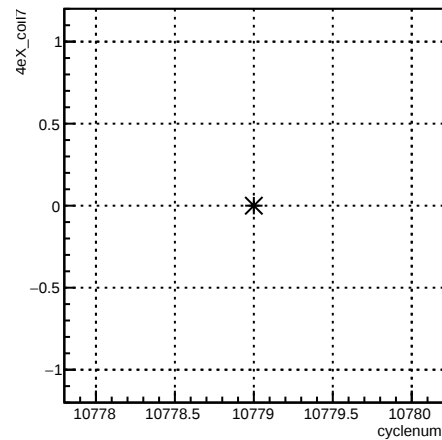
4eX_coil7:cyclenum {run == 8218}
