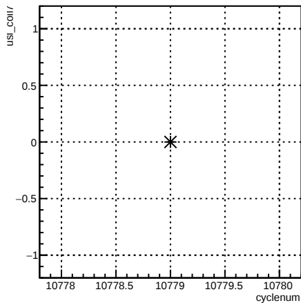
usl_coil7:cyclenum {run == 8218}
