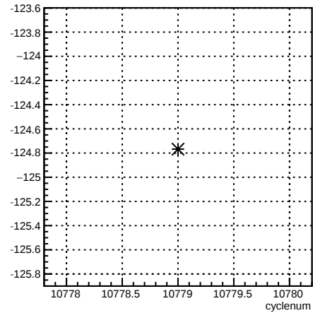
1X_coil1:cyclenum {run == 8218}
