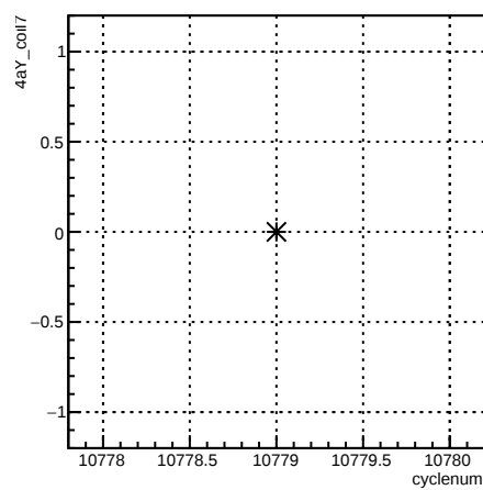
4aY_coil7:cyclenum {run == 8218}
