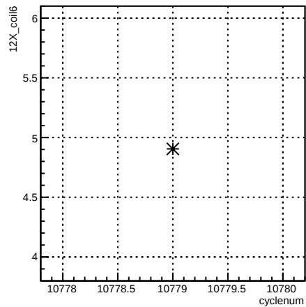
12X_coil6:cyclenum {run == 8218}
