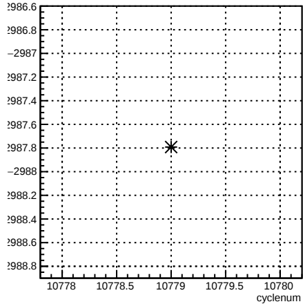
usr_coil6:cyclenum {run == 8218}
