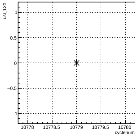
usl_12X:cyclenum {run == 8218}
