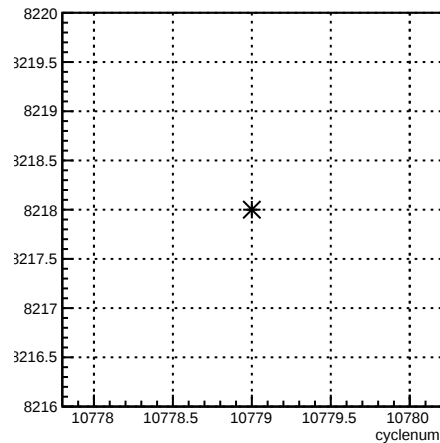
run:cyclenum {run == 8218}
