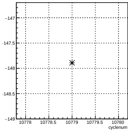
4eY_coil6:cyclenum {run == 8218}
