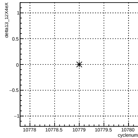
delta13_12X4eX:cyclenum {run == 8218}
