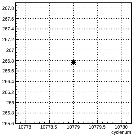
4eY_coil4:cyclenum {run == 8218}
