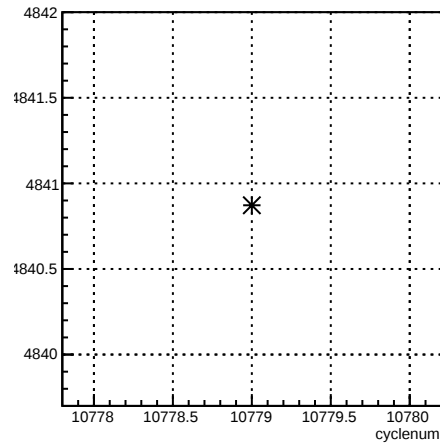
usl_coil4:cyclenum {run == 8218}
