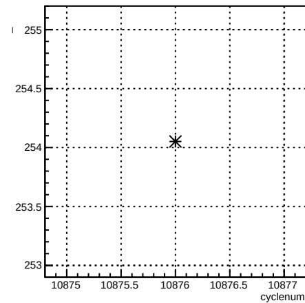
4eX_coil7:cyclenum {run == 8238}
