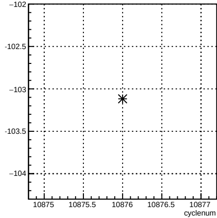
4eY_coil6:cyclenum {run == 8238}
