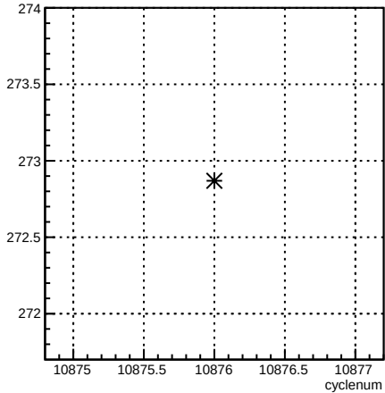
4eY_coil4:cyclenum {run == 8238}
