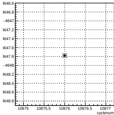
usl_coil6:cyclenum {run == 8238}
