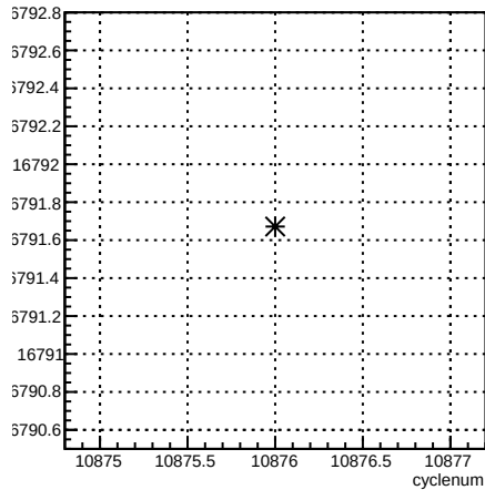
usl_coil1:cyclenum {run == 8238}
