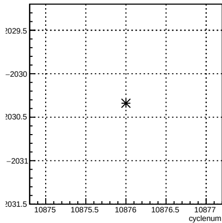
usr_coil3:cyclenum {run == 8238}
