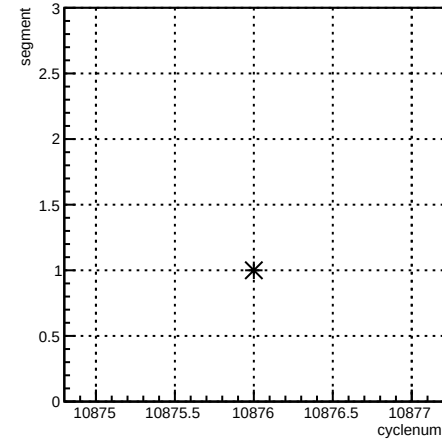
segment:cyclenum {run == 8238}
