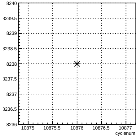
run:cyclenum {run == 8238}
