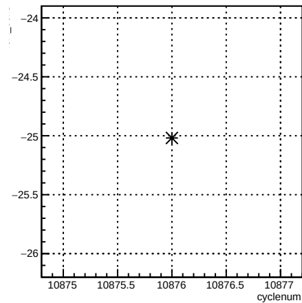
4eX_coil3:cyclenum {run == 8238}
