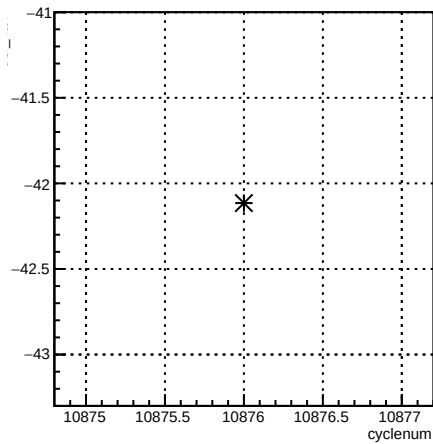
usl_4aY:cyclenum {run == 8238}
