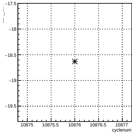
12X_coil4:cyclenum {run == 8238}
