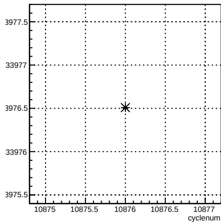
usr_coil7:cyclenum {run == 8238}
