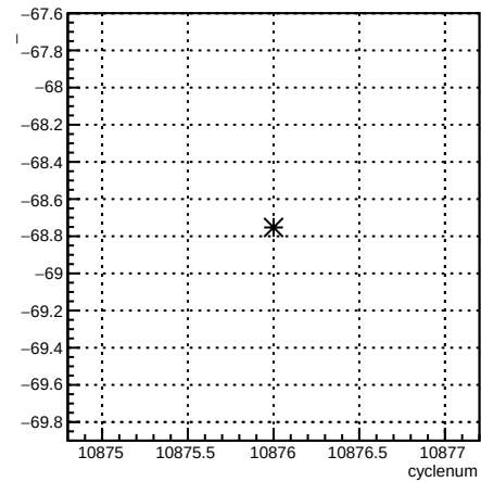
usl_1X:cyclenum {run == 8238}
