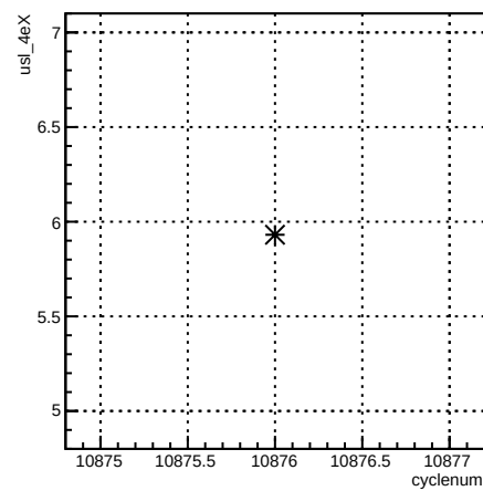
usl_4eX:cyclenum {run == 8238}
