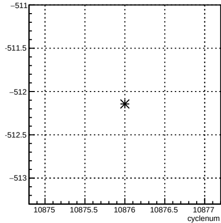
12X_coil7:cyclenum {run == 8238}
