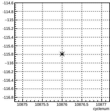
usr_1X:cyclenum {run == 8238}
