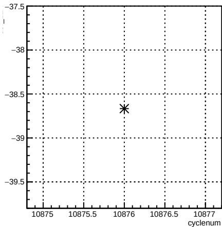
usr_12X:cyclenum {run == 8238}
