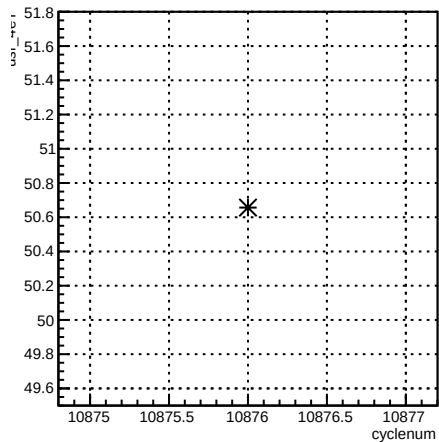
usr_4eY:cyclenum {run == 8238}
