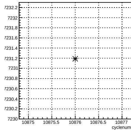
usr_coil4:cyclenum {run == 8238}
