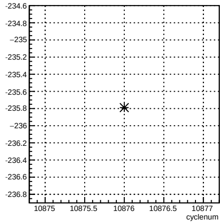
12X_coil1:cyclenum {run == 8238}
