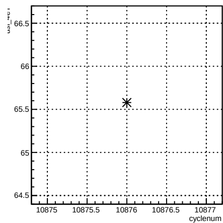
usl_4eY:cyclenum {run == 8238}
