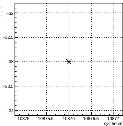
usr_4aY:cyclenum {run == 8238}
