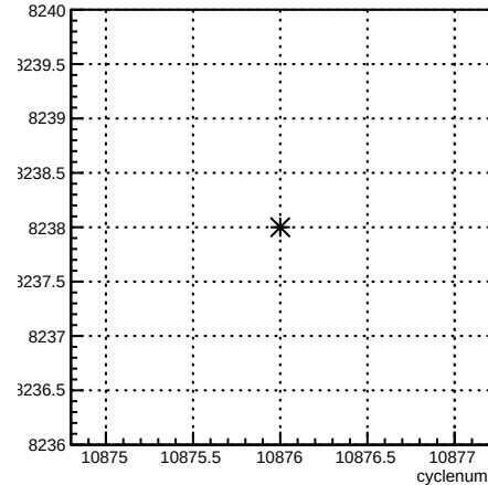
run:cyclenum {run == 8238}
