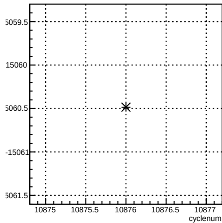
usr_coil1:cyclenum {run == 8238}
