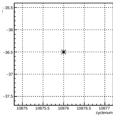
usl_12X:cyclenum {run == 8238}
