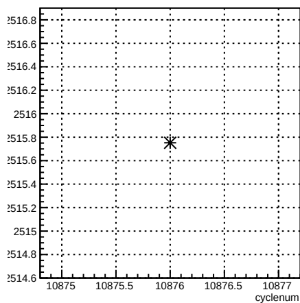
usl_coil7:cyclenum {run == 8238}
