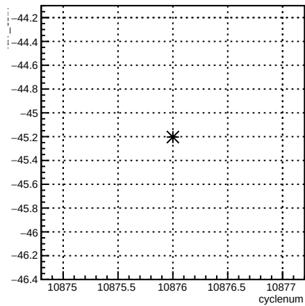
4eY_coil7:cyclenum {run == 8238}
