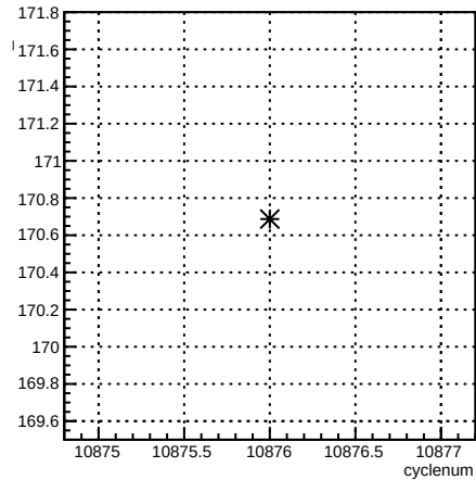
usr_4eX:cyclenum {run == 8238}
