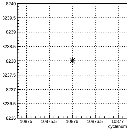
run:cyclenum {run == 8238}
