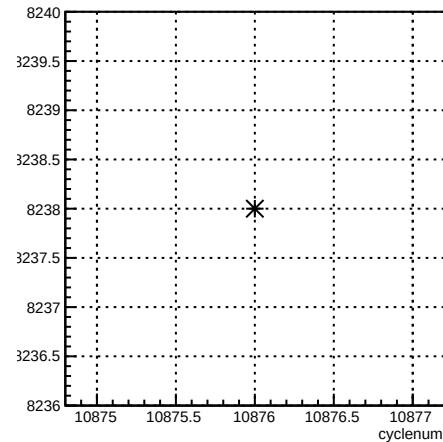
run:cyclenum {run == 8238}
