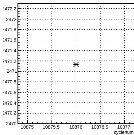
usl_coil3:cyclenum {run == 8238}
