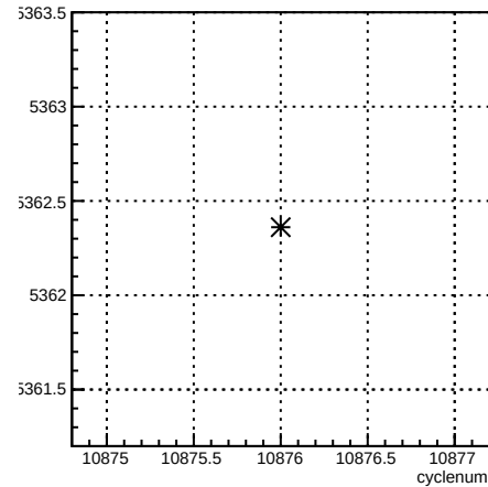
usl_coil4:cyclenum {run == 8238}
