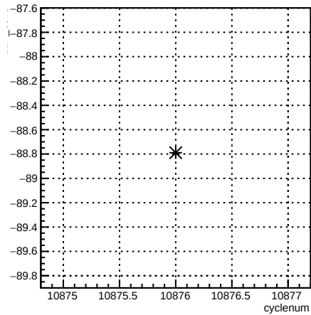
12X_coil3:cyclenum {run == 8238}
