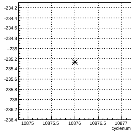
4eX_coil1:cyclenum {run == 8238}
