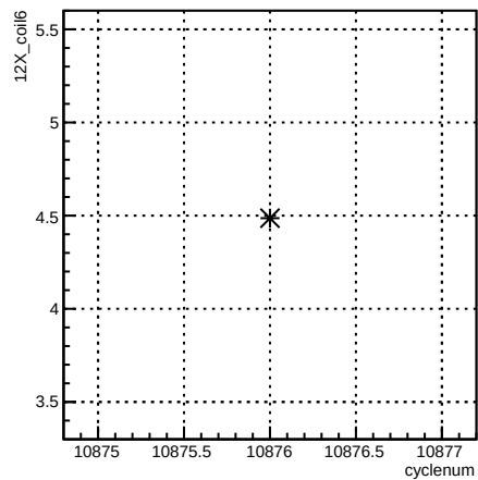
12X_coil6:cyclenum {run == 8238}
