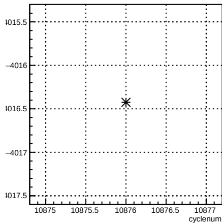
usr_coil6:cyclenum {run == 8238}
