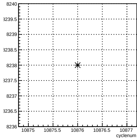
run:cyclenum {run == 8238}
