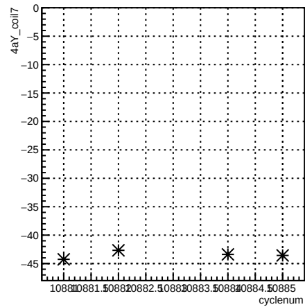
4aY_coil7:cyclenum {run == 8239}
