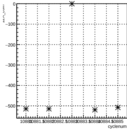
12X_coil7:cyclenum {run == 8239}
