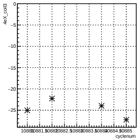
4eX_coil3:cyclenum {run == 8239}
