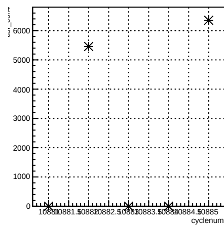
usr_coil4:cyclenum {run == 8239}
