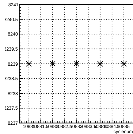
run:cyclenum {run == 8239}
