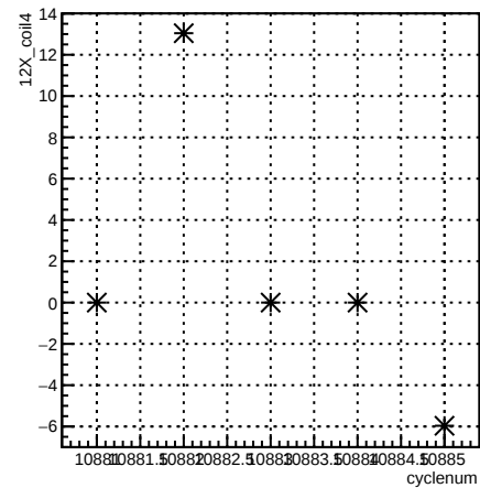
12X_coil4:cyclenum {run == 8239}
