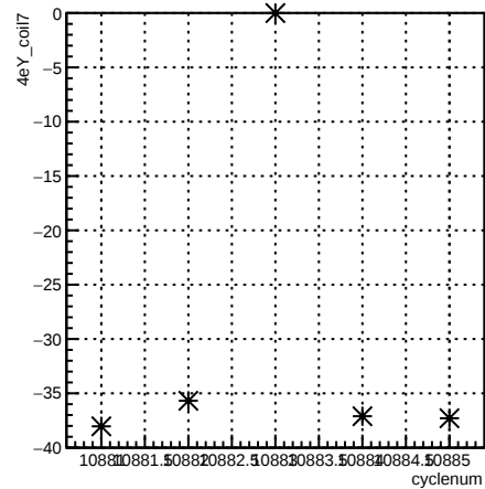
4eY_coil7:cyclenum {run == 8239}
