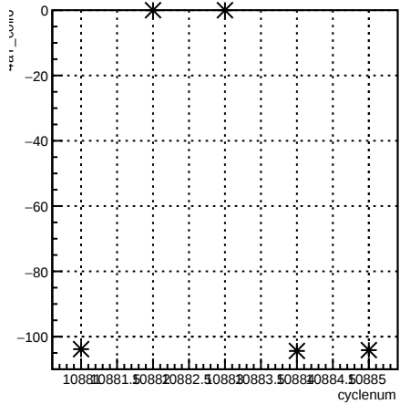
4aY_coil6:cyclenum {run == 8239}
