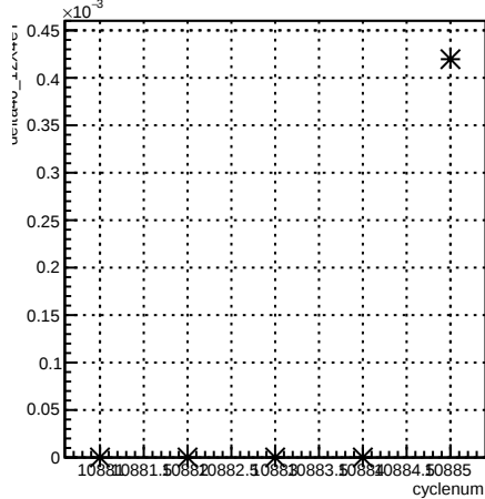
delta46_12X4eY:cyclenum {run == 8239}
