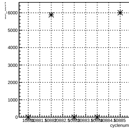
run:cyclenum {run == 8239}
