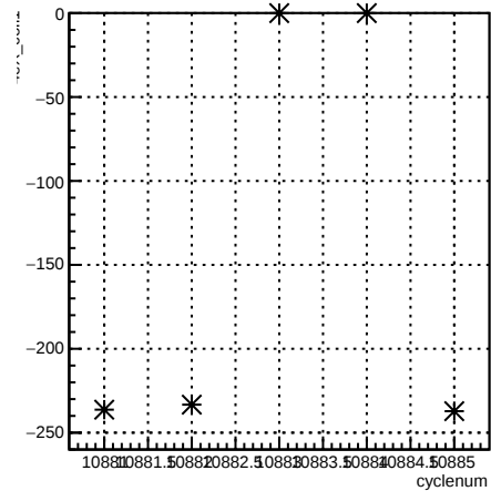
4eX_coil1:cyclenum {run == 8239}
