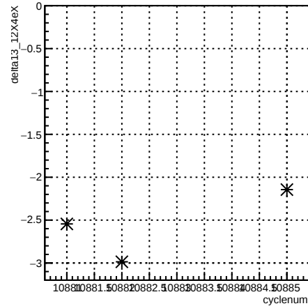
delta13_12X4eX:cyclenum {run == 8239}
