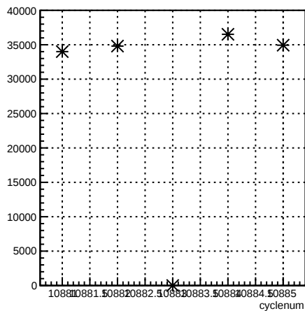
usr_coil7:cyclenum {run == 8239}
