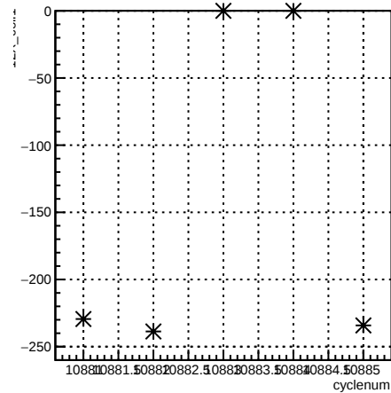
12X_coil1:cyclenum {run == 8239}
