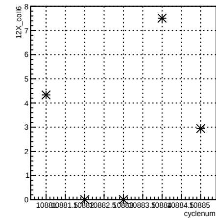
12X_coil6:cyclenum {run == 8239}
