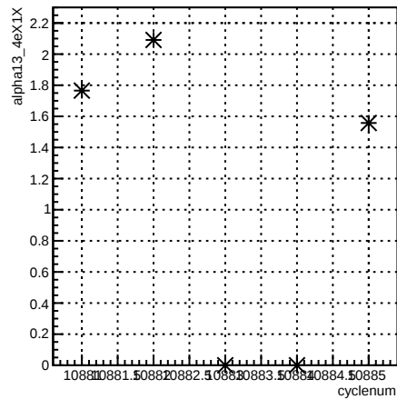
alpha13_4eX1X:cyclenum {run == 8239}
