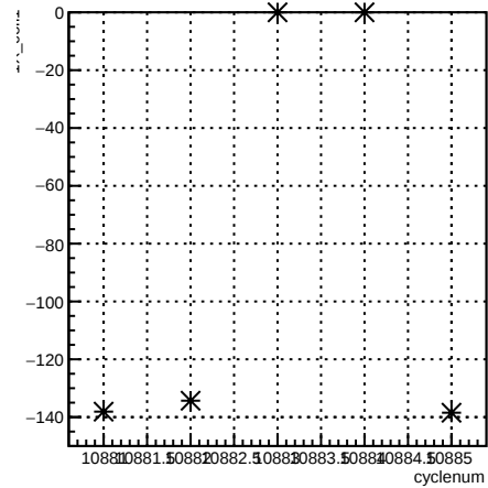
1X_coil1:cyclenum {run == 8239}
