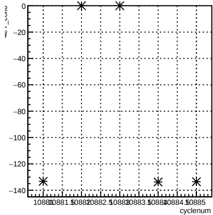
4eY_coil6:cyclenum {run == 8239}
