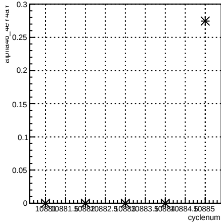
alpha46_4eY4aY:cyclenum {run == 8239}
