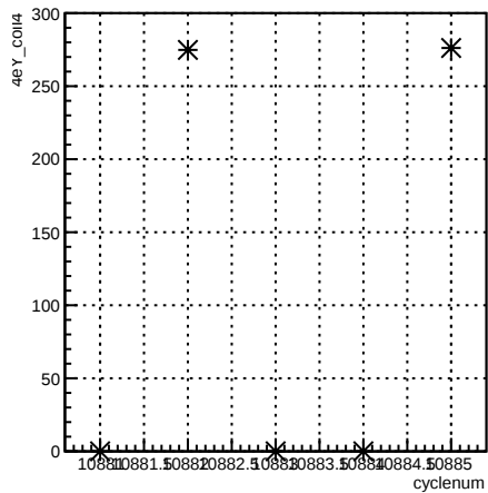
4eY_coil4:cyclenum {run == 8239}
