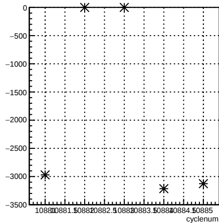
usr_coil6:cyclenum {run == 8239}
