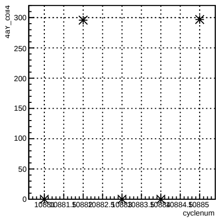
4aY_coil4:cyclenum {run == 8239}
