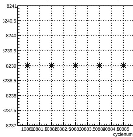
run:cyclenum {run == 8239}
