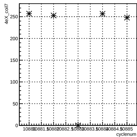
4eX_coil7:cyclenum {run == 8239}
