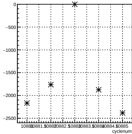
usr_coil3:cyclenum {run == 8239}
