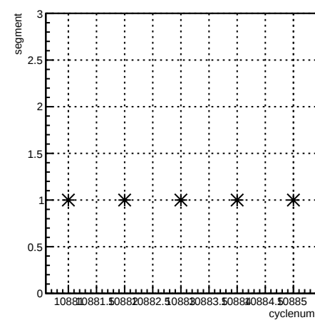
segment:cyclenum {run == 8239}
