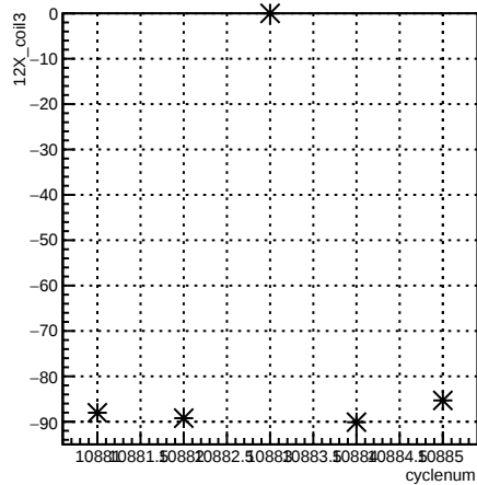
12X_coil3:cyclenum {run == 8239}
