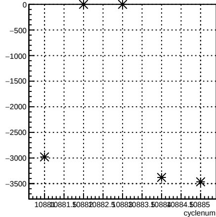
usl_coil6:cyclenum {run == 8239}
