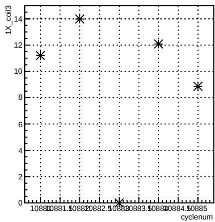
1X_coil3:cyclenum {run == 8239}
