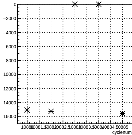
usr_coil1:cyclenum {run == 8239}
