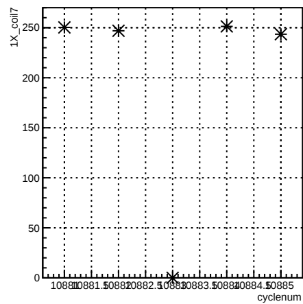
1X_coil7:cyclenum {run == 8239}
